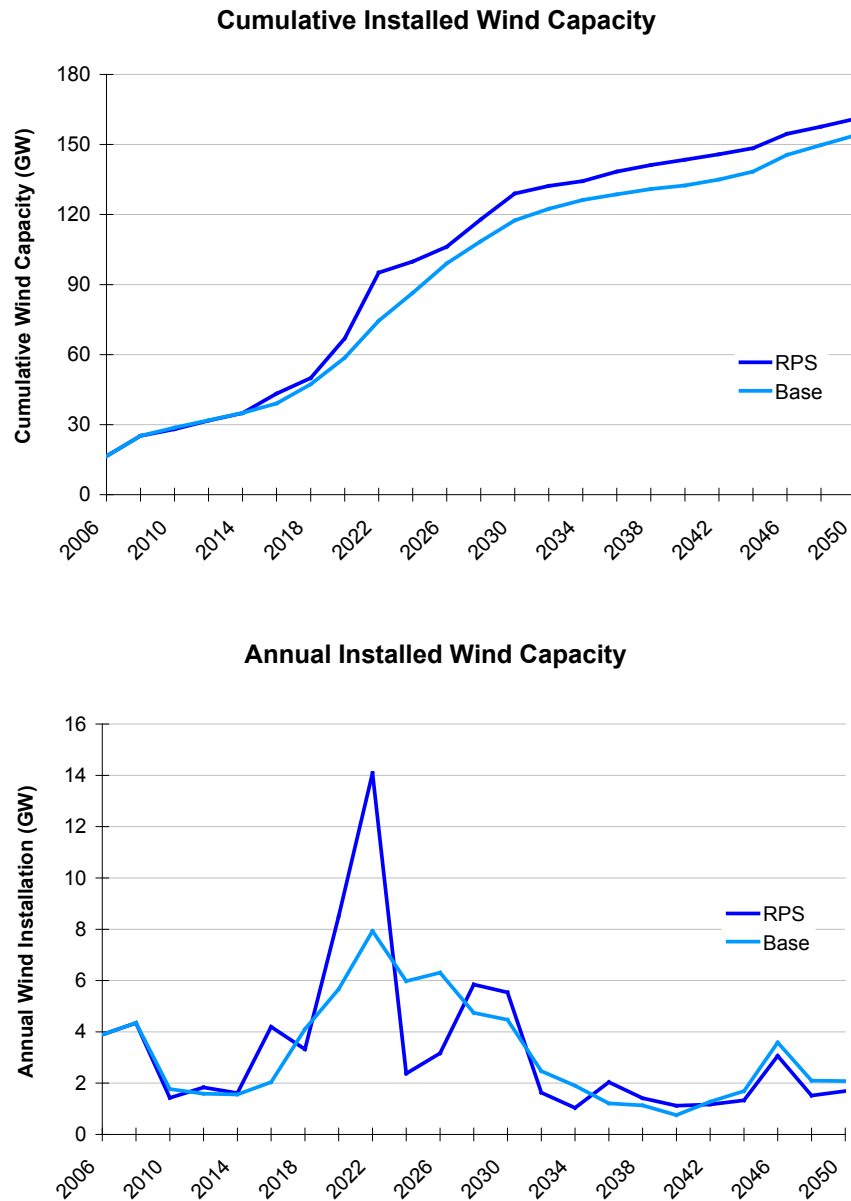
Figure 6. Cumulative and annual installations of wind power
