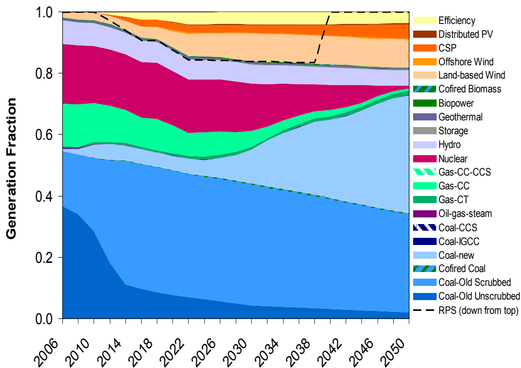
Figure 2. Contributions to meeting total load in the RPS case
