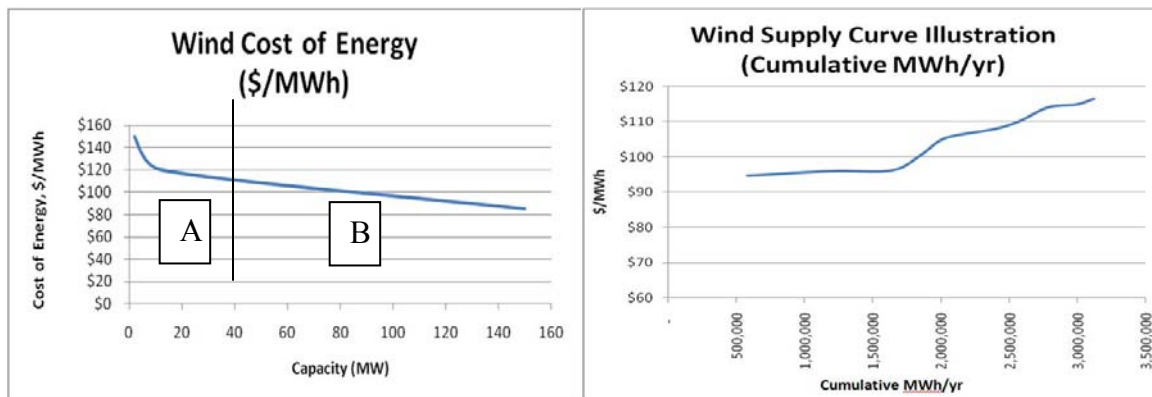
Figure 1. Adapted from a Competitive Renewable Energy Zone in a study of California's Renewable Energy Transmission Initiative (Black and Veatch 2009)
