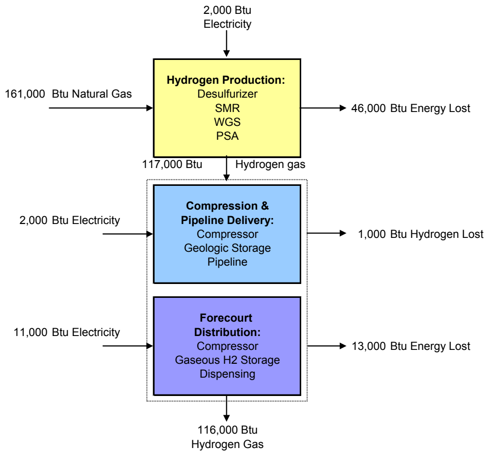
Figure 2.4.5. Flow diagram and energy balance of central natural gas–pipeline delivery pathway
