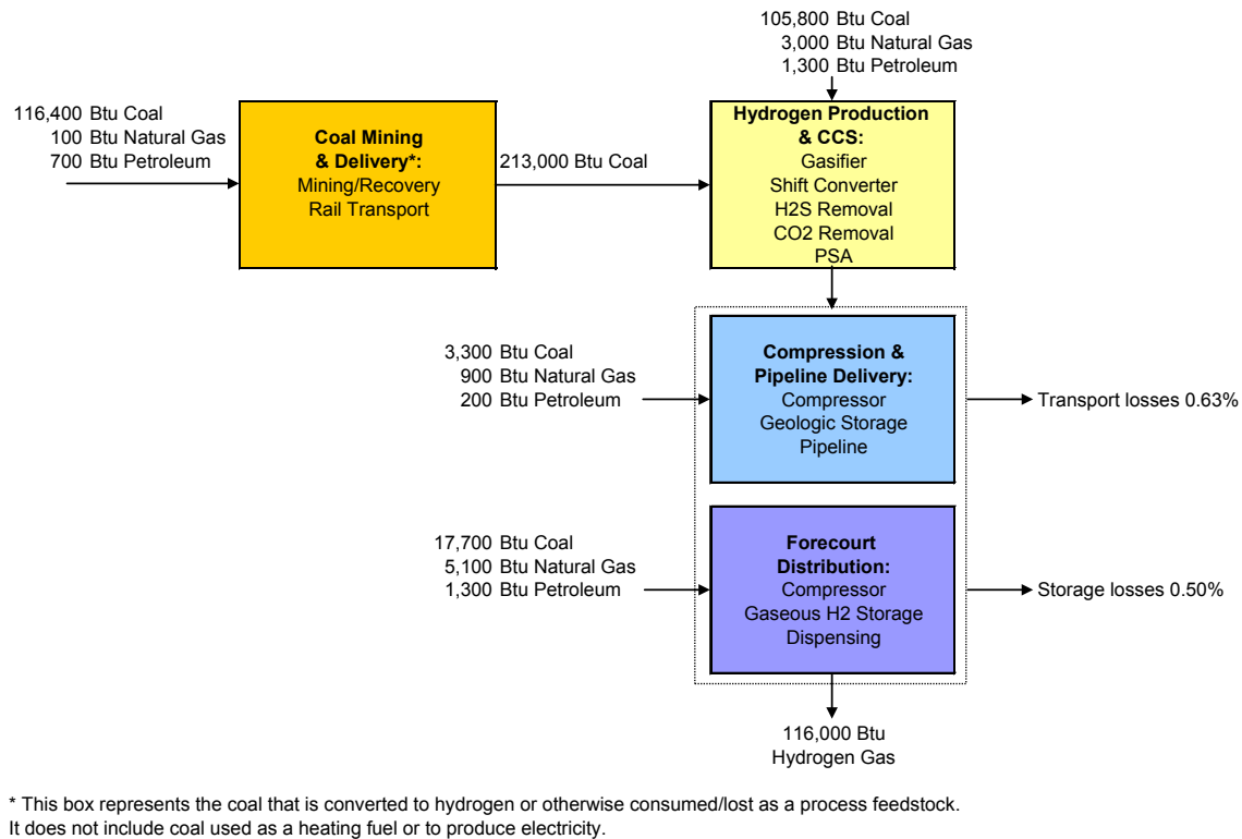
Figure 9.7.5. WTW energy inputs to deliver 116,000 Btu hydrogen to a vehicle using central coal with CCS–pipeline delivery pathway
