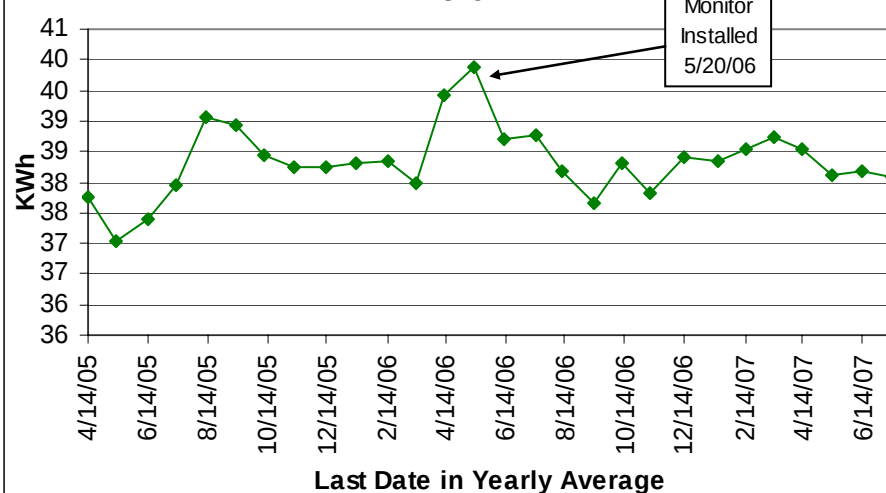
Daily Energy Use - Yearly Average C-3
