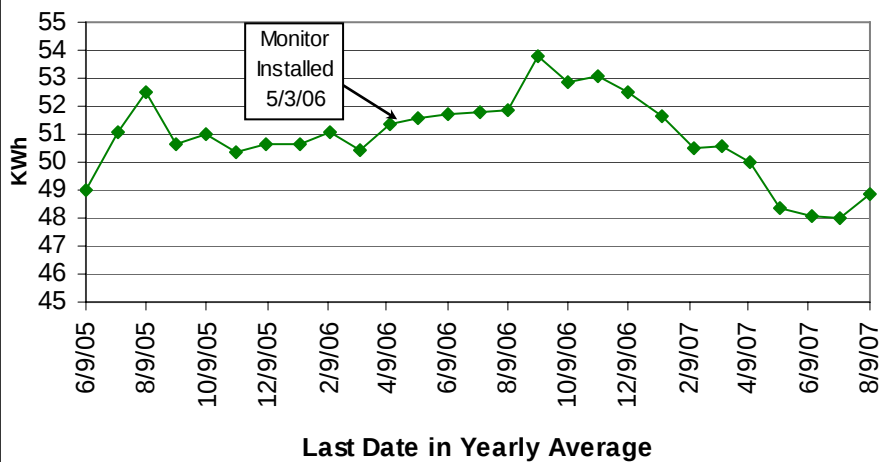
Average kWh used per day- Yearly Average F-1
