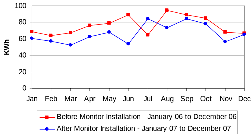
Energy Use Before and After TED Load Monitor Installation - H-4
