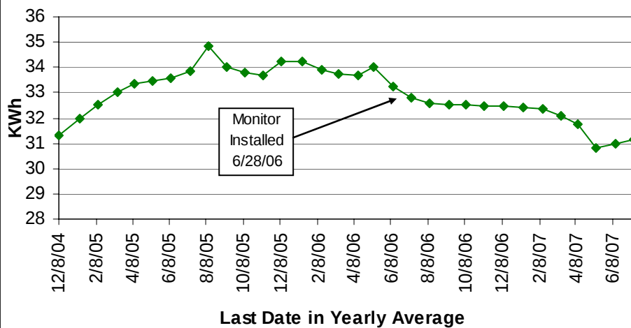
Daily Energy Use - Yearly Average M-2
