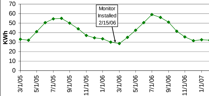
Energy Use Before and After TED Load Monitor Installation - C-2
