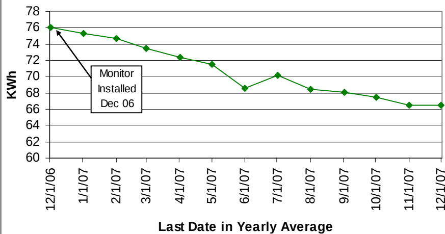
Daily Energy Use - Yearly Average H-4
