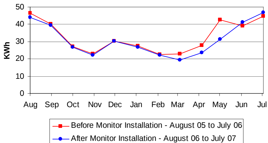
Energy Use Before and After TED Load Monitor Installation - M-2
