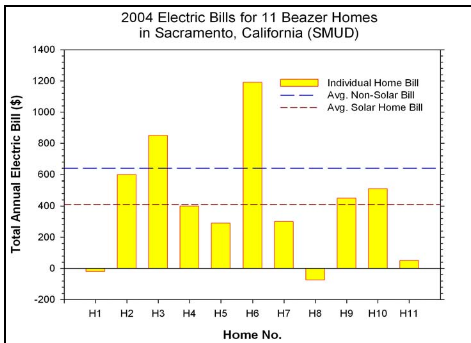
Figure 2. Variation in annyal energy use in eleven similar SMUD solar homes in Sacramento, CA (2004).
