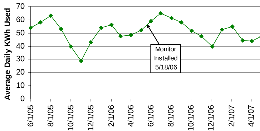
Energy Use Before and After TED Load Monitor Installation - C-1
