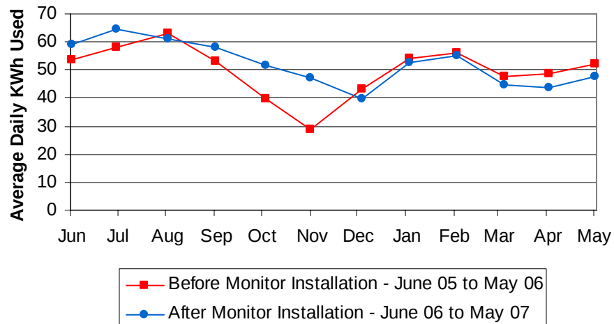
Energy Use Before and After TED Load Monitor Installation - C-1
