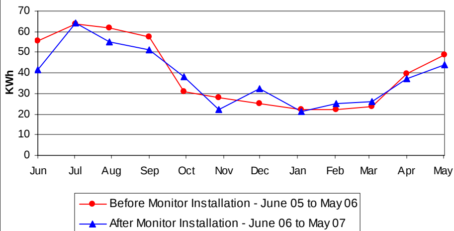
Energy Use Before and After TED Load Monitor Installation - C-3
