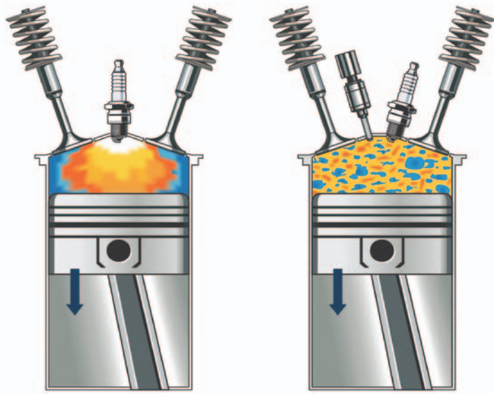
Illustrations of normal combustion (left) and homogeneous charge compression ignition (right)
