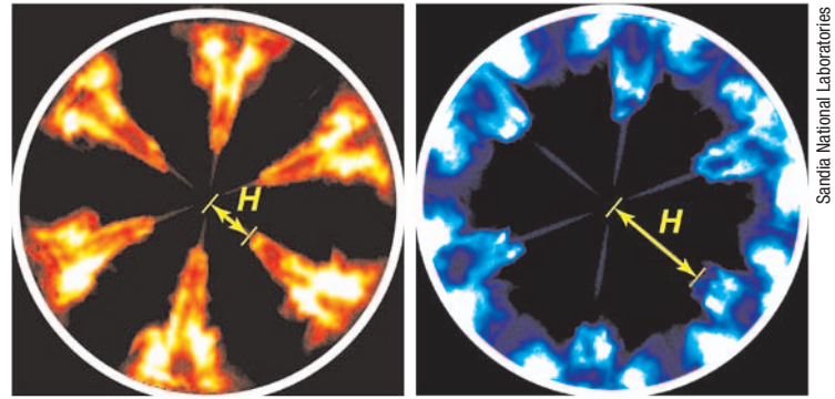
In-cylinder images from normal combustion (left) and non-sooting, low-NO x combustion obtained by lowering intake-gas oxygen content (right)
