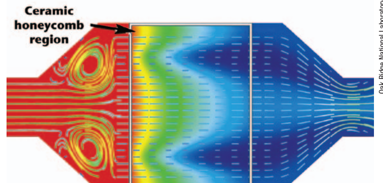
Analysis of a catalytic converter during cold starting
