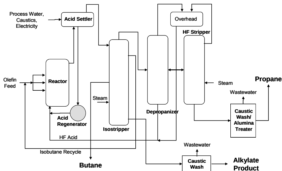
Figure 12. Hydrofluoric Acid-Based Alkylation Flow Diagram [DOE 1998]
