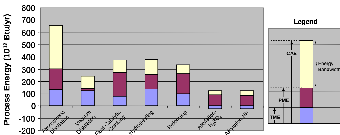
Figure 14. Petroleum Refining Industry Energy Bandwidth, Production per Year Basis
