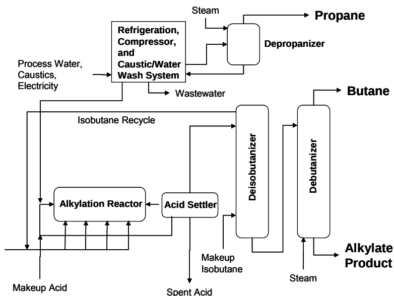
Figure 11. Sulfuric Acid-Based Alkylation Flow Diagram [DOE 1998]
