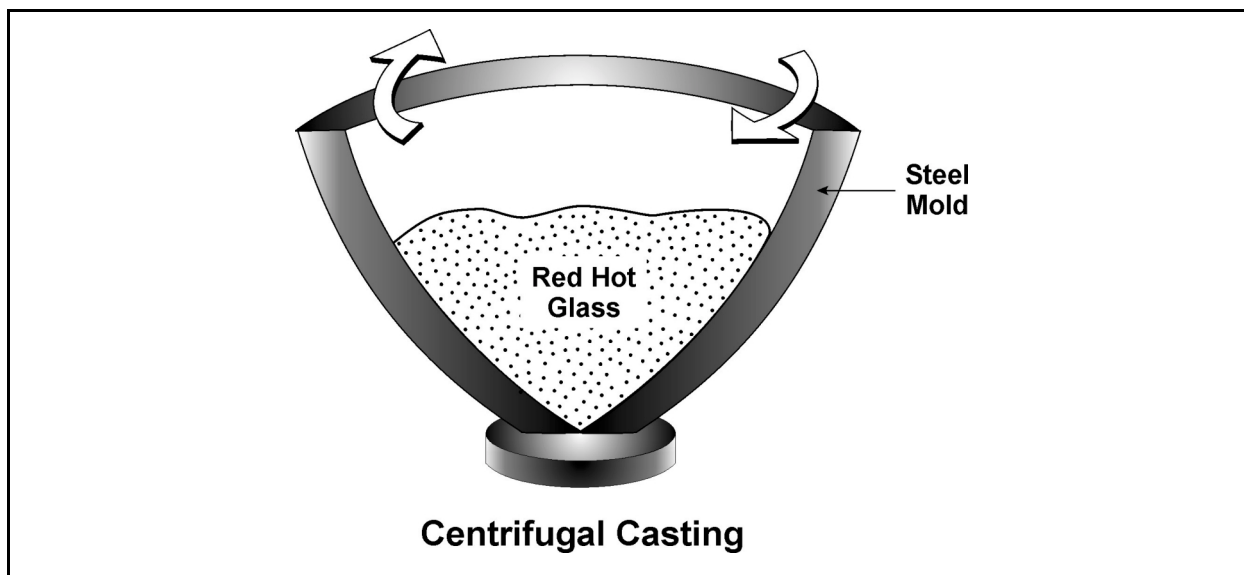
Figure 5-8. Centrifugal Casting of TV Tube Conical Sections [Corning 2000]
