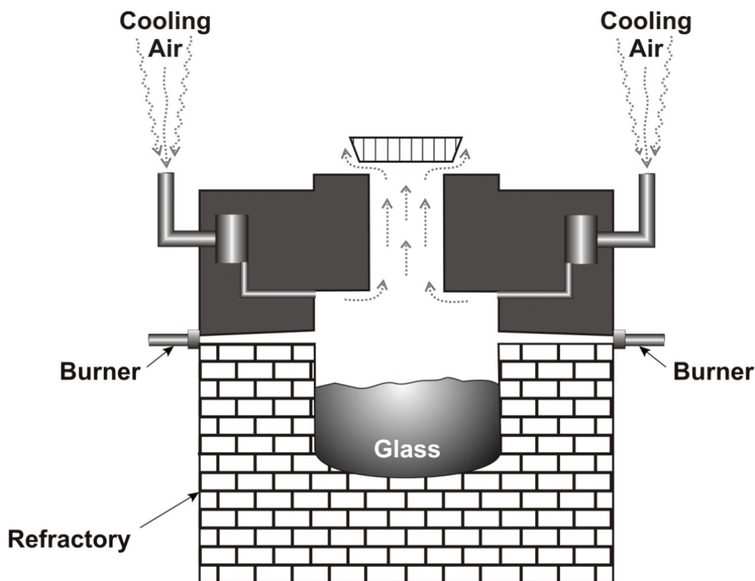
Figure 4-2. Forehearth [EI 1988]
