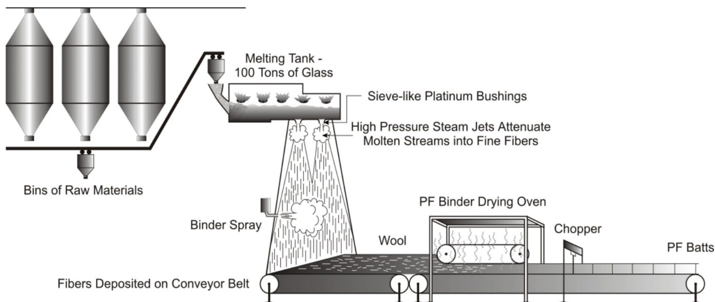
Figure 5-12. Steam or Air Injection Process for Glass Wool Manufacture [El 1988]
