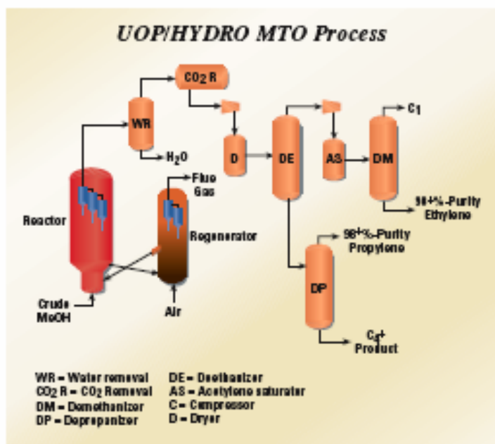
Exhibit 8: UOP Methanol to Olefins Flow Diagram
