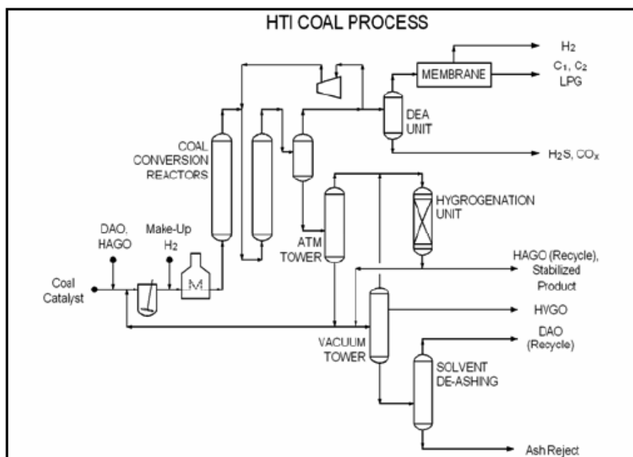
Exhibit 3: Coal Liquefaction Flow Diagram (Source: Shenhua Group Corporation)
