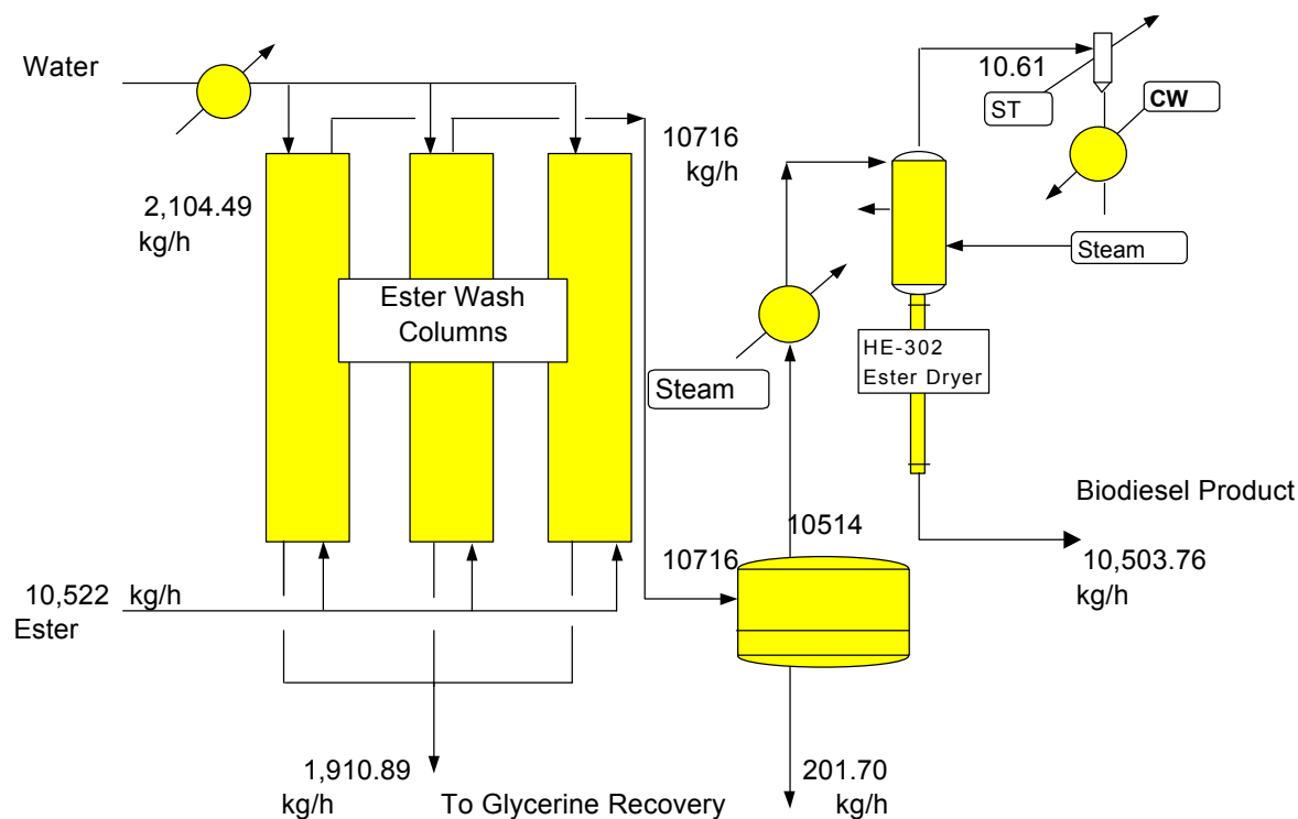
Figure 60: Methyl Ester Purification
