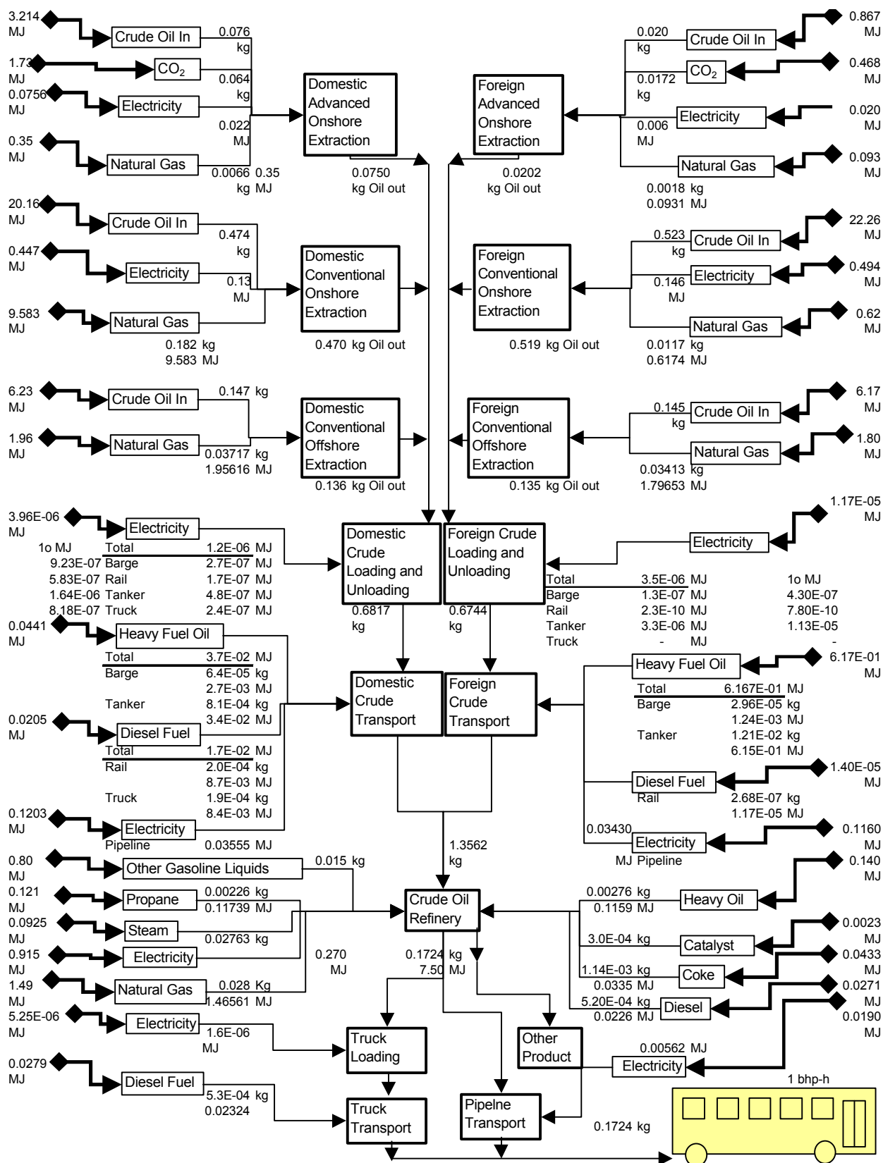
Figure 25: Primary Energy Balance for Petroleum Diesel Fuel Life Cycle (No Mass Allocation)
