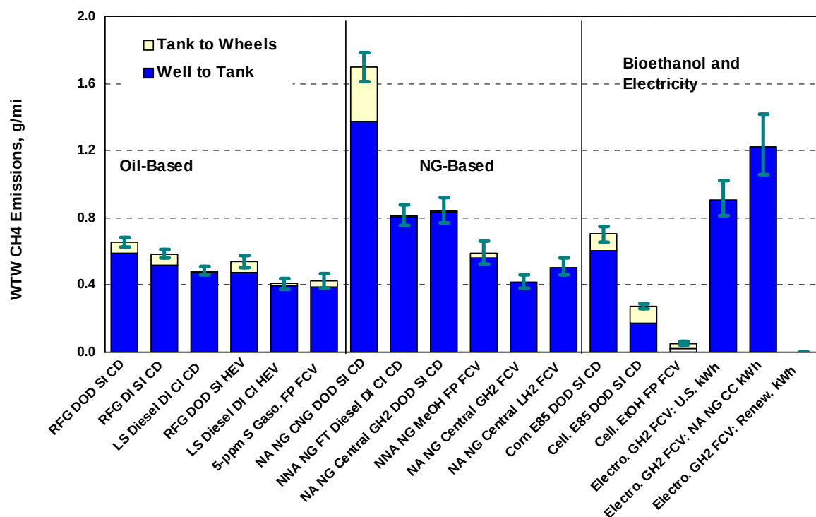
Figure 4-7 WTW CH 4 Emissions of 18 Vehicle/Fuel Systems (g/mi)
