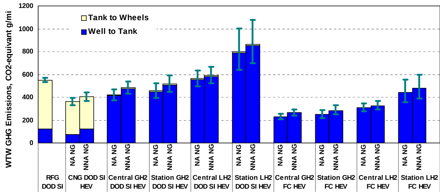
Figure 4-28 WTW Effects of North American NG vs. Non-North American NG: GHG Emissions (CO 2 -equivalent g/mi)
