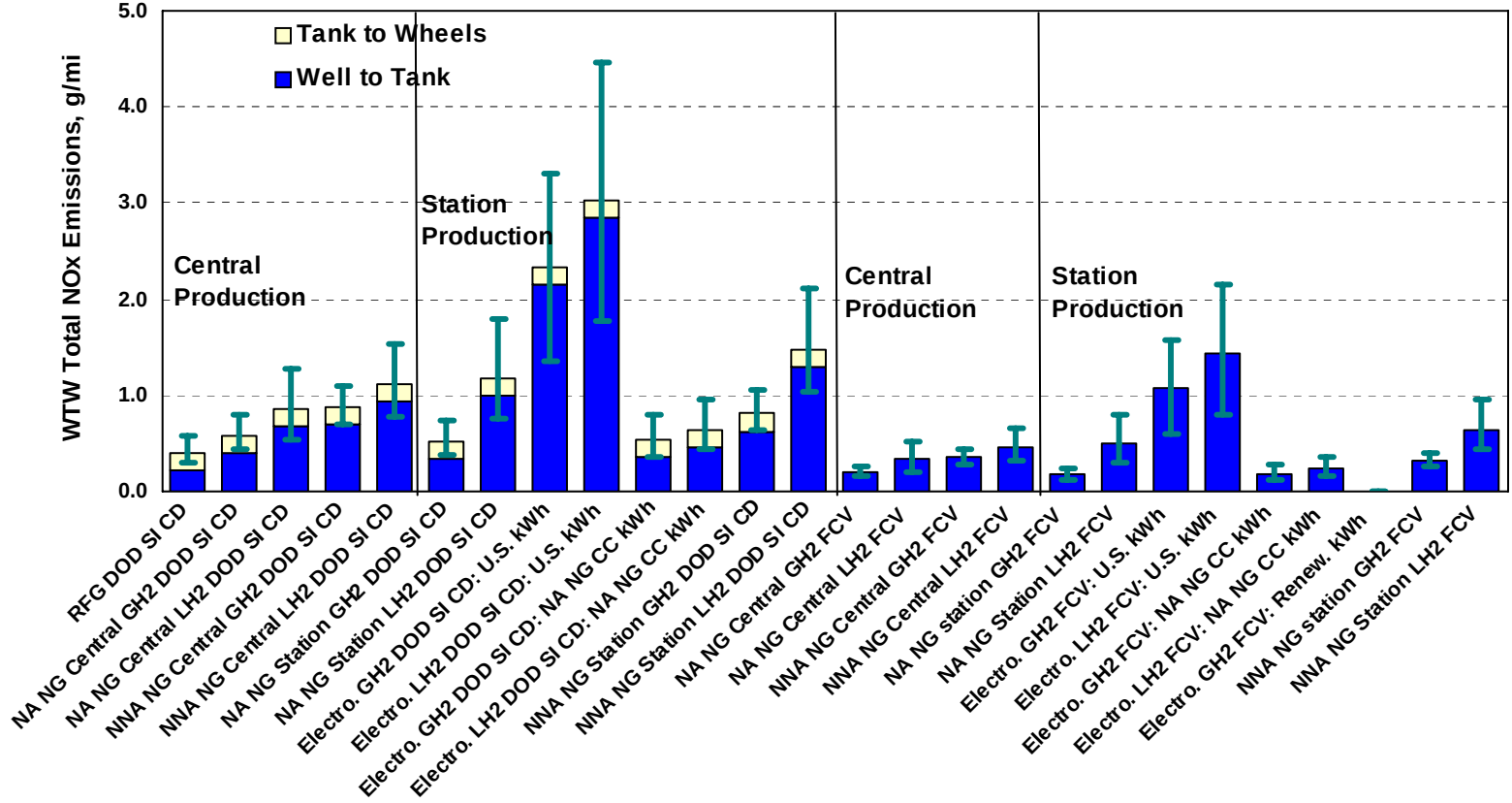
Figure 4-39 WTW Total NO x Emissions of Hy hydrogen Production Options (g/mi)
