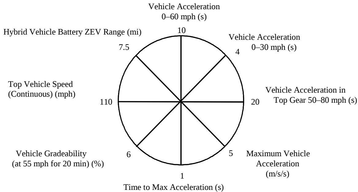
Figure 2-27 Minimum Vehicle Performance Requirements
