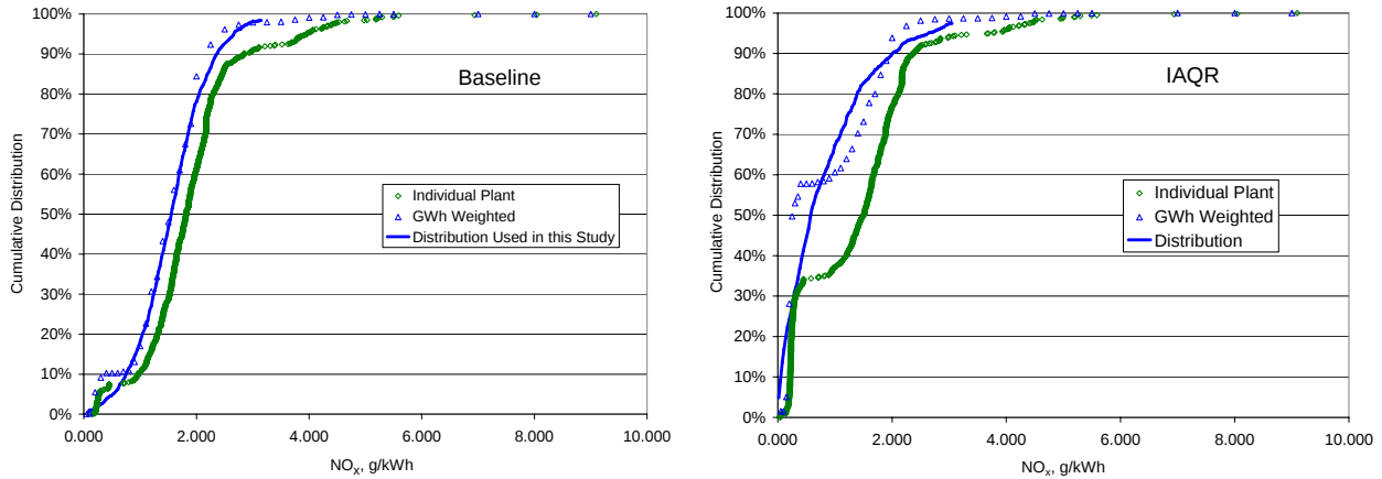
Figure 2-20 NO x Emissions for Utility Coal Boilers
