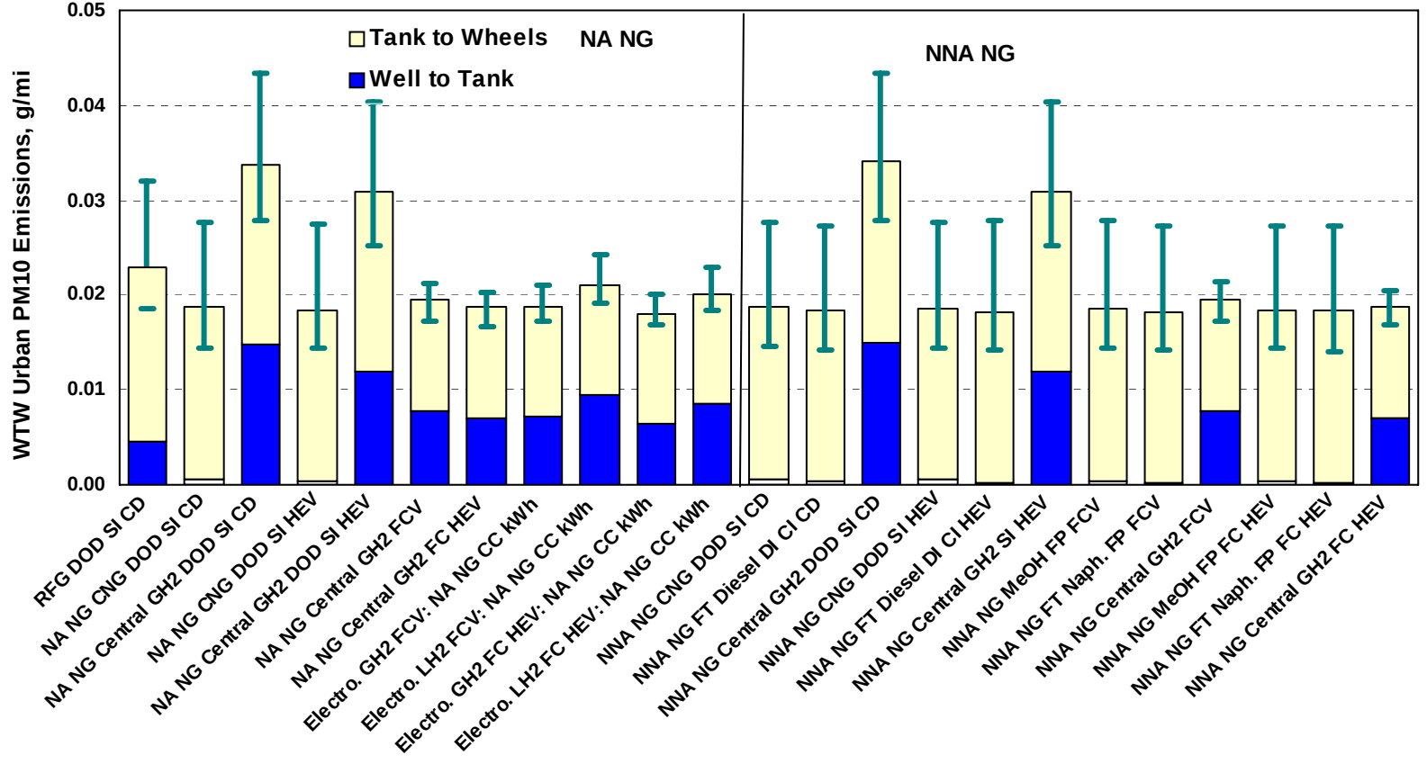
Figure 4-51 Comparison of NG-Based Systems: WTW Urban PM 10 Emissions (g/mi)
