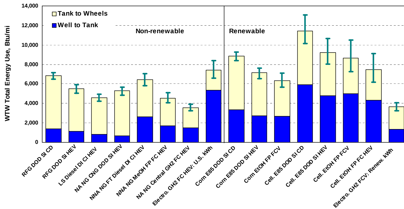
Figure 4-42 Comparison of Non-Renewable and Renewable Fuels: WTW Total Energy Use (Btu/mi)
