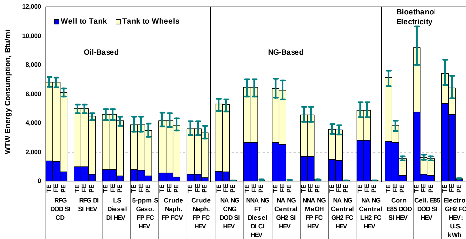
Figure 4-19 WTW Total Energy Use, Fossil Energy Use, and Petroleum Energy Use of Selected Vehicle/Fuel Systems (Btu/mi)
