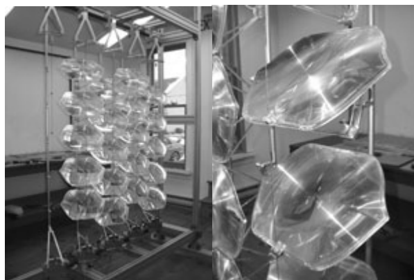
Figure 1. IC Solar Façade – Version 4.1
