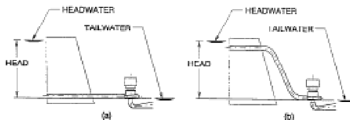
Figure 16. Providing mild pressure changes in short penstocks. (Source: Franke et al. 1997)
