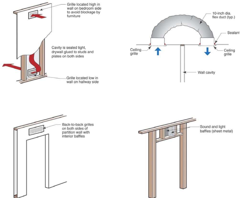
Figure 1-12. Placement of ducts and transfer grilles
