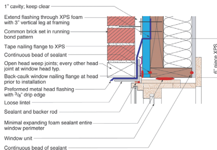
Figure 3-3. Rough opening flashing
