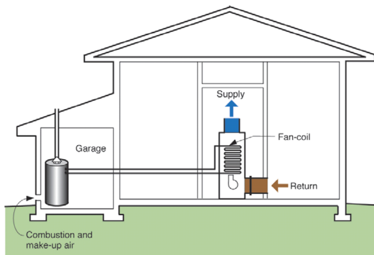
Figure 4-3. Combo heating system
