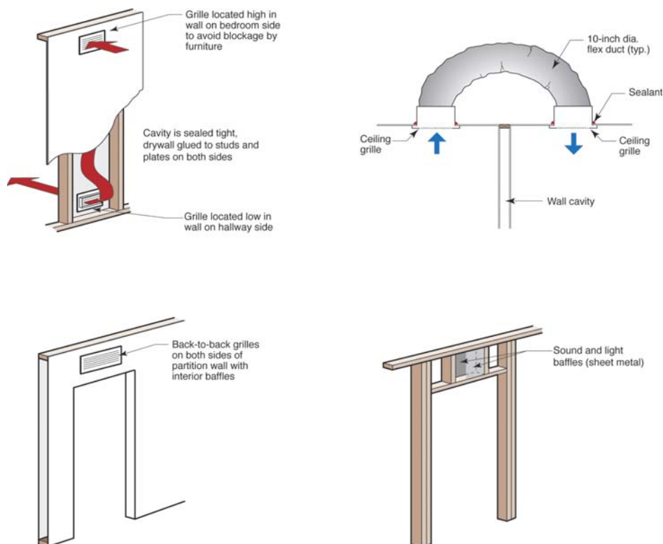
Figure 3-10. Transfer grille and jump ducts approaches
