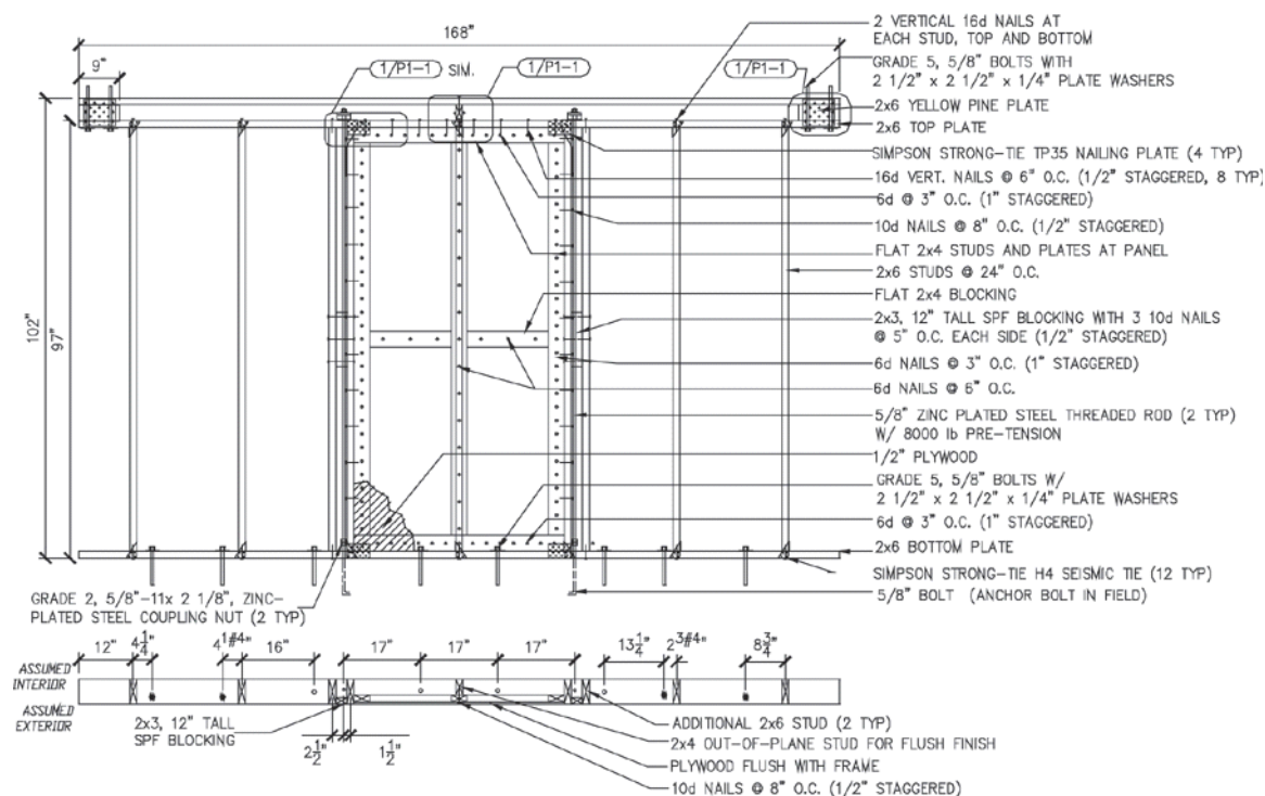
Fig. 66. Advanced framing detail
