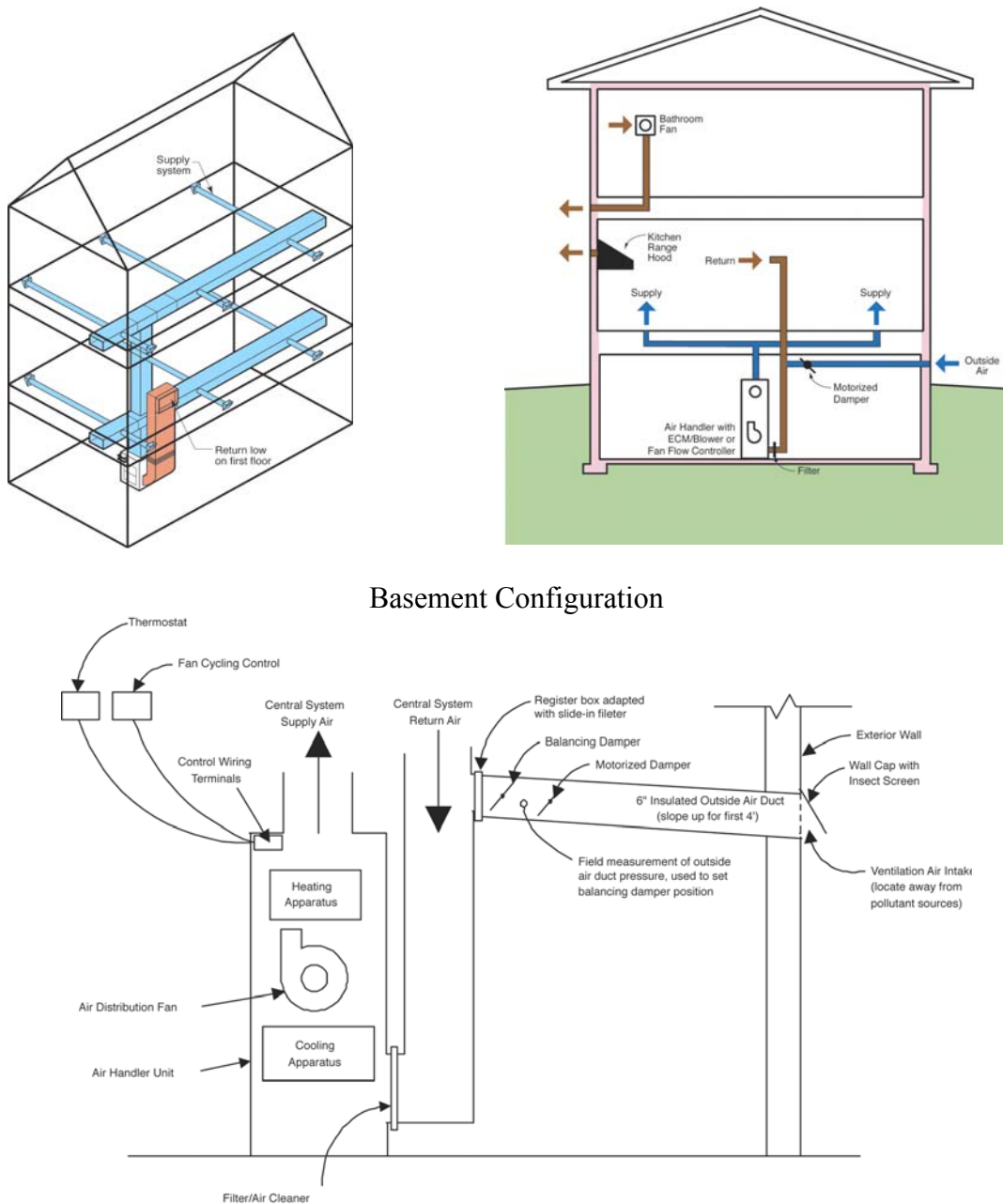
Figure 2-4. Recommended ventilation system in the "Chicago"
