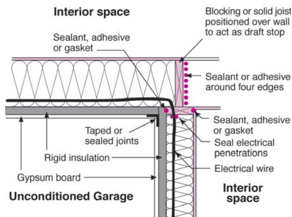
Figure 2-13. Creating a continuous air barrier
