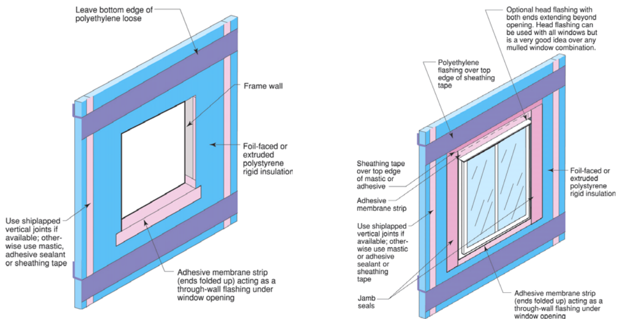
Figure 1-21. Window flashing
