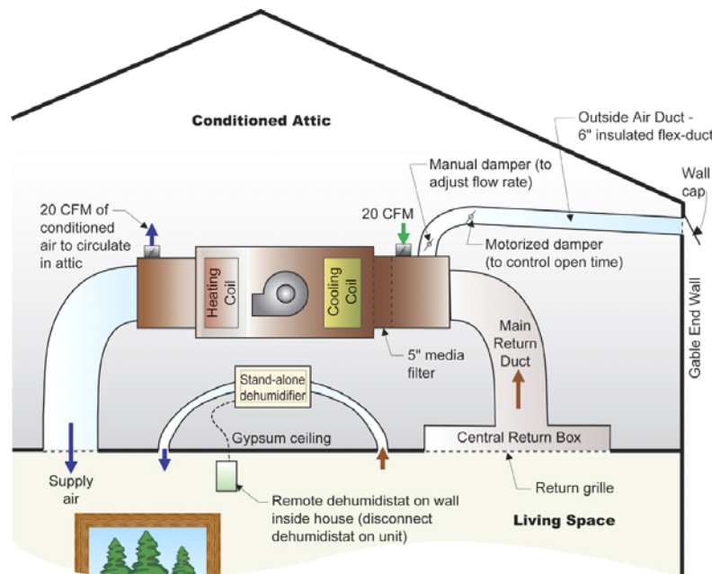
Figure 1-4. A conditioned attic
