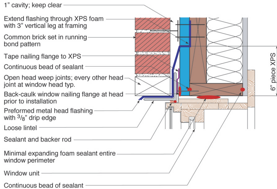
Figure 3-9. Rough opening flashing
