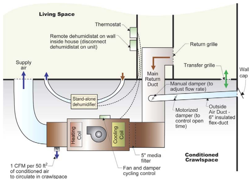
Figure 1-22. Mechanical system and ventilation in conditioned crawlspace
