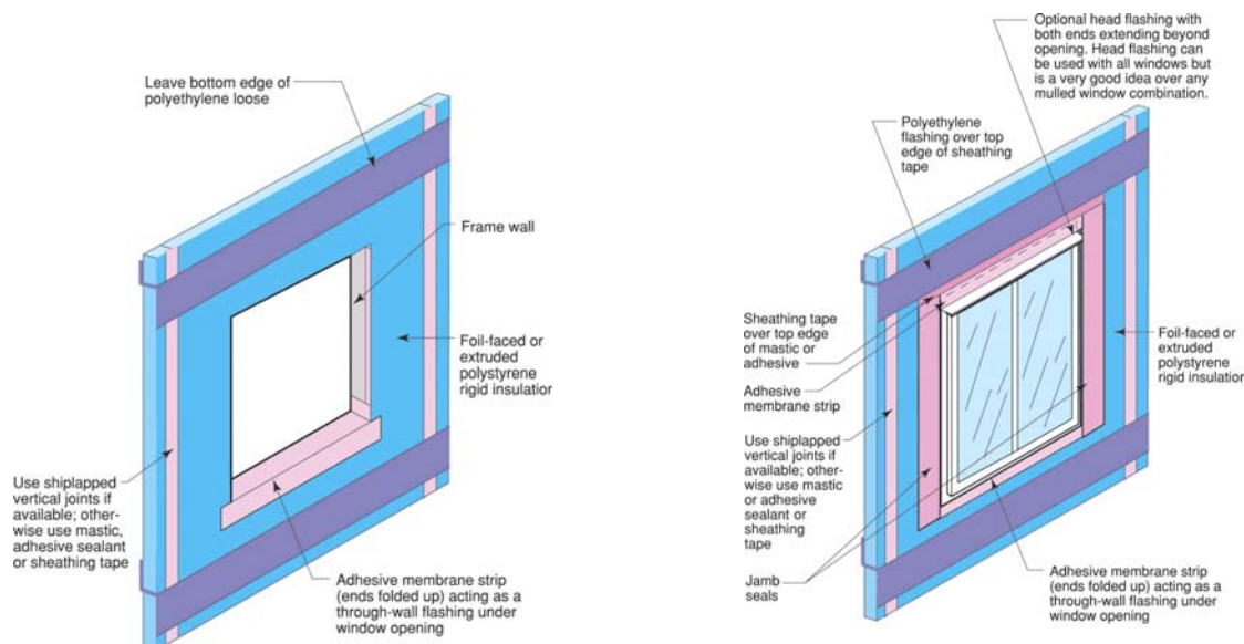
Figure 1-3. Window flashings
