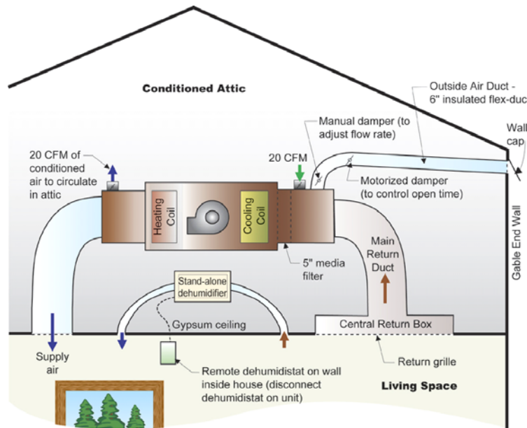
Figure 1-11. Dehumidification
