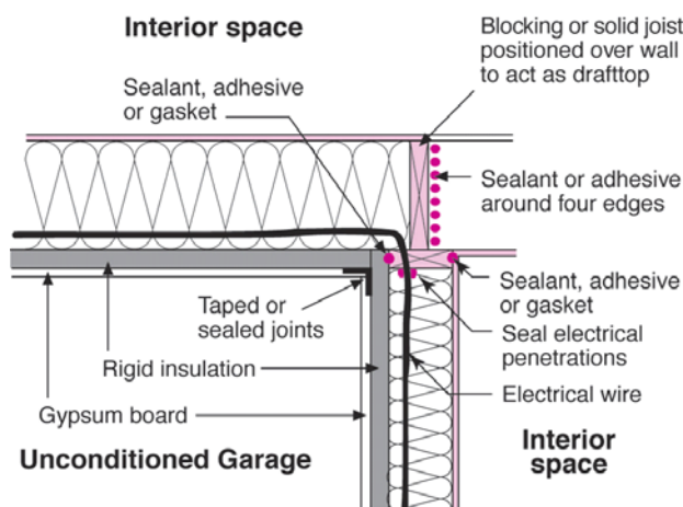
Figure 3-15. Creating a continuous air barrier
