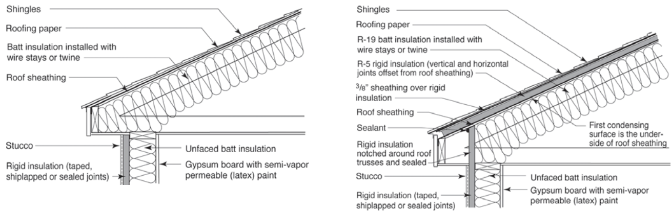
Figure 4-14. Unvented, conditioned attic design
