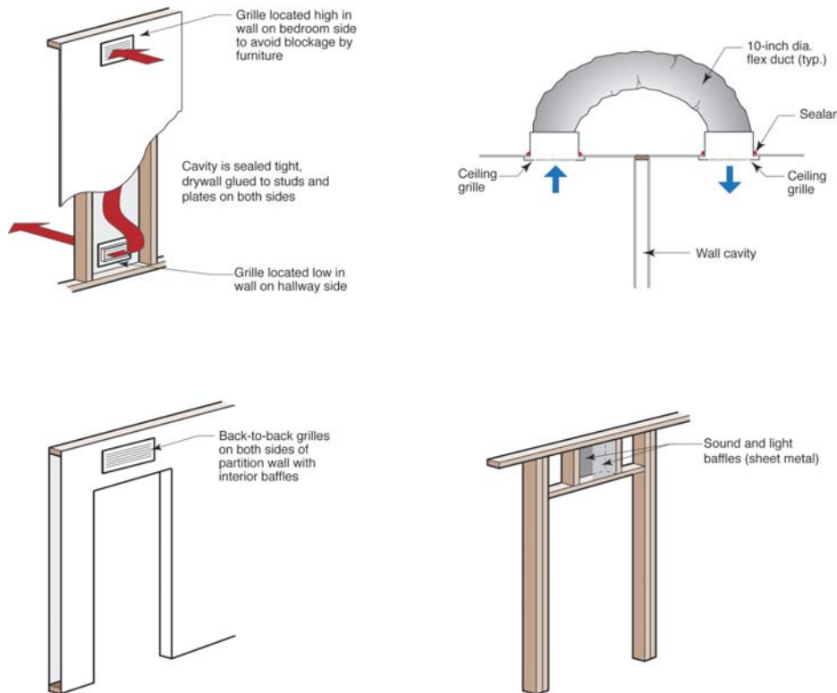
Figure 1-23. Transfer grilles and jump ducts
