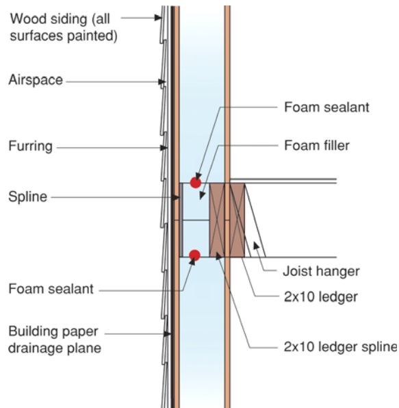
Figure 1-17: Above-grade wall spline
