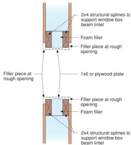
Figure 1-18. Load-bearing window jamb assembly
