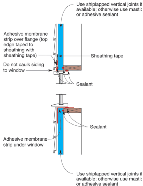
Figure 3-16. Rough opening flashing
