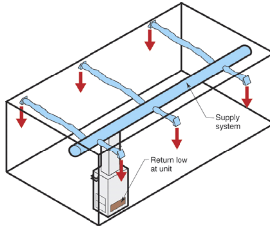
Figure 4-17. Heating and cooling system layout
