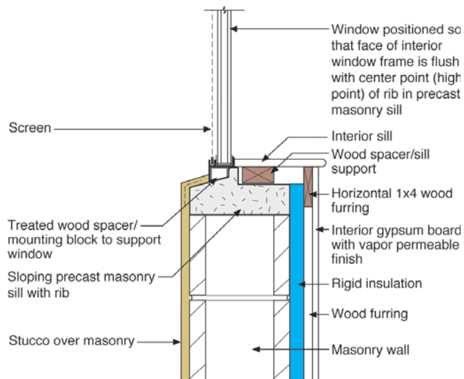
Window sill drainage section
