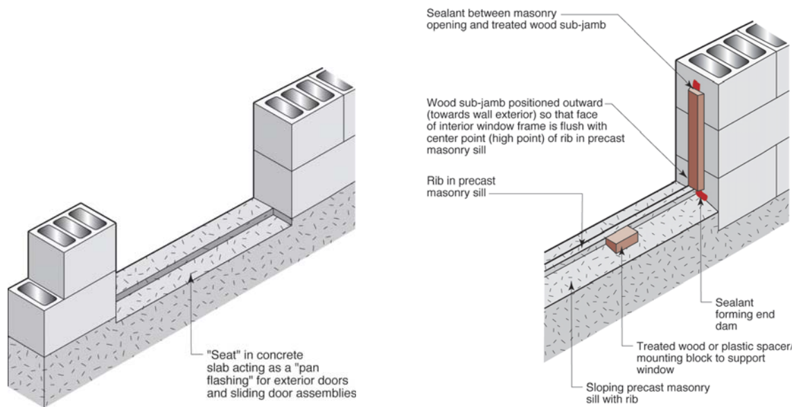
Exterior door pan flashing "seat"
