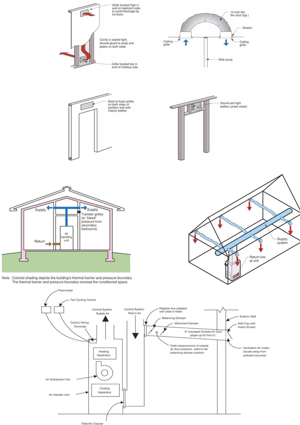
Figure 4-4. Ducting, transfer grilles, and interior closet configuration
