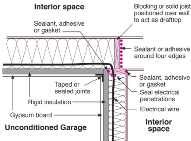
Figure 3-8. Creating a continuous air barrier
