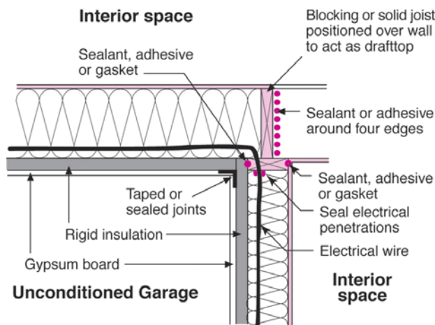
Figure 2-7. Creating a continuous air barrier
