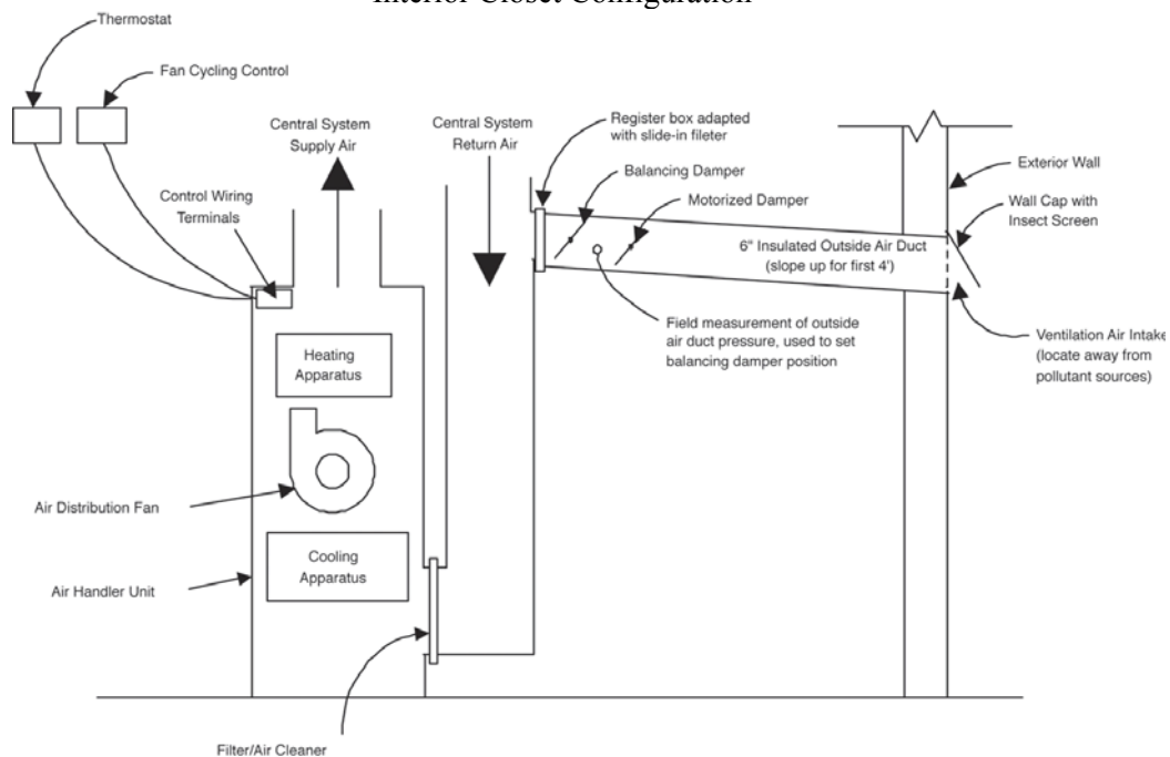
Figure 3-11. Mechanical ventilation for the “Atlanta”
