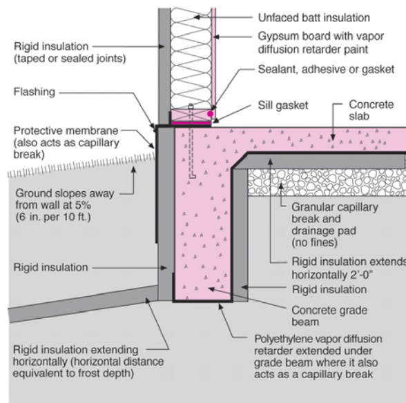
Figure 2-17. Slab foundation details
