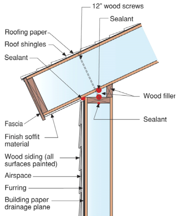
Figure 1-15. Alternative SIPS roof framing
