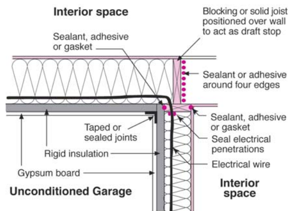
Figure 1-9. Using sealants and rigid insulation to create a continuous air barrier
