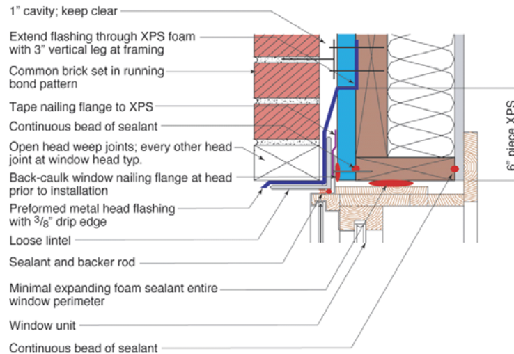
Figure 2-8. Brick veneer flashing
