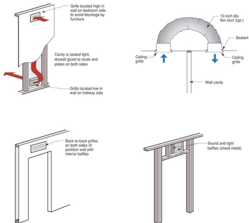
Figure 2-9. Return grilles
