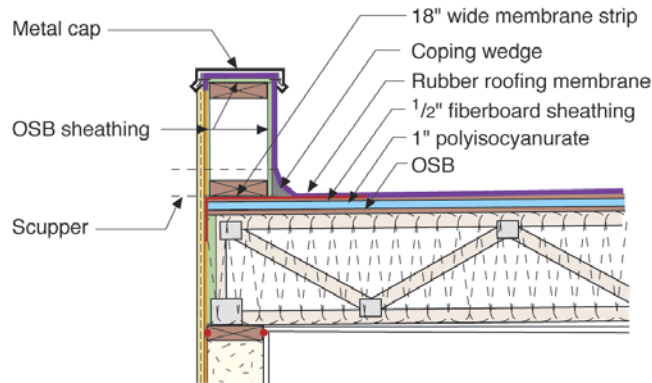
Figure 4-19. Flat-roof assembly
