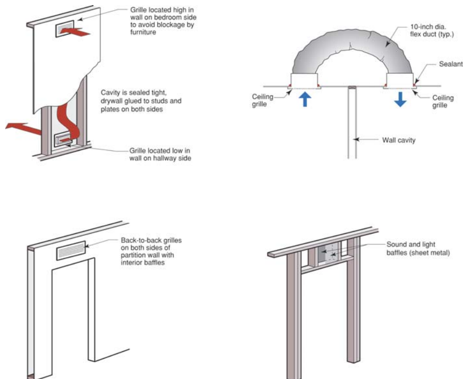
Figure 4-18. Transfer grilles and jump ducts
