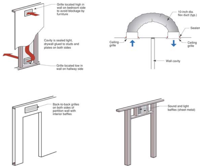
Figure 3-4. Transfer grille and jump duct approaches
