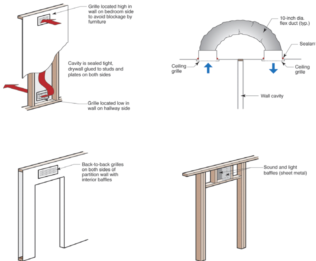
Figure 1-6. Transfer grilles and jump ducts
