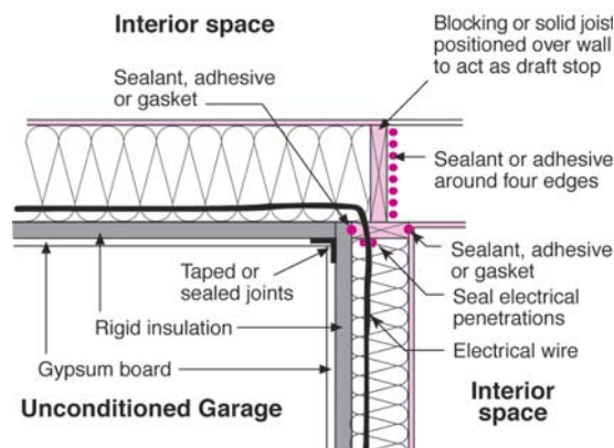
Figure 4-2. Continuous air barrier
