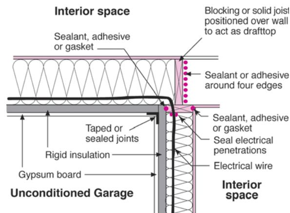
Figure 4-9. Creating a continuous air barrier
