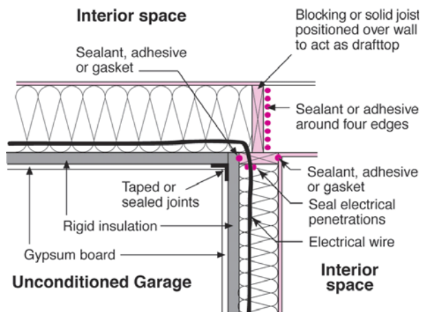
Figure 3-2. Air sealing
