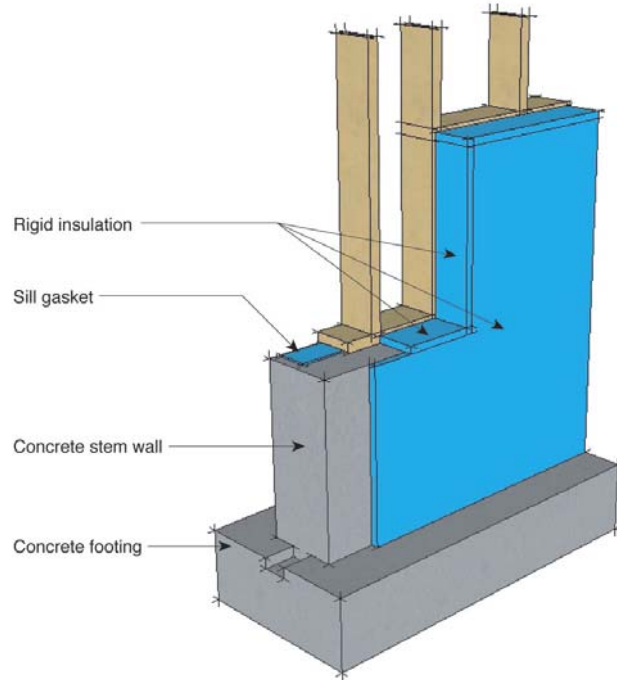
Figure 3-20. Stepped foundation insulation detail
