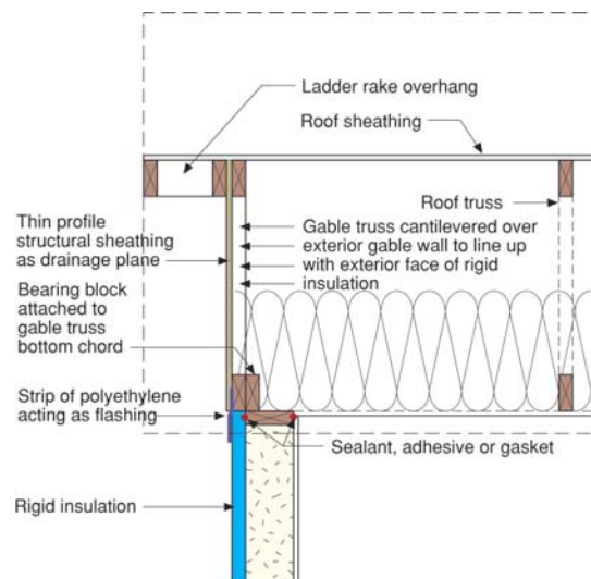
Figure 3-12. Gable end exterior sheathing detail
