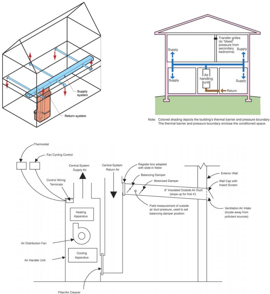
Figure 4-12. HVAC configuration in the “Sacramento”
