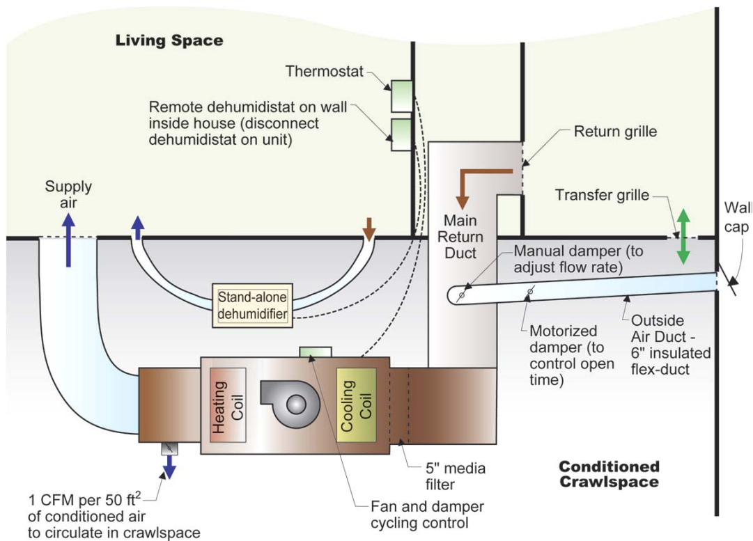
Figure 3-5. Mechanical system and ventilation in conditioned crawlspace
