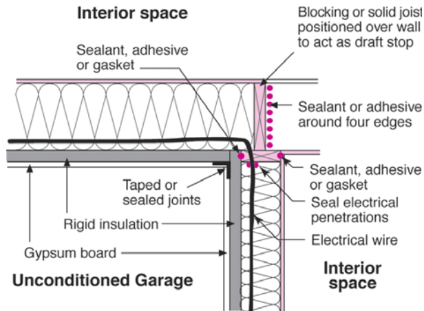
Figure 1-20. Creating a continuous air barrier
