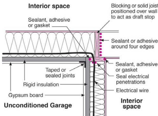
Figure 1-2. Creating a continuous air barrier
