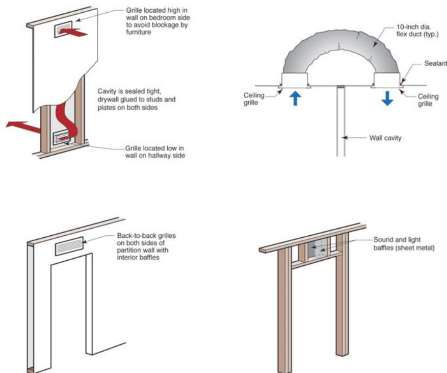
Figure 4-11. Transfer grilles and jump ducts
