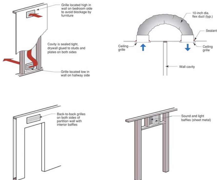
Figure 2-3. Transfer grille and jump duct approaches
