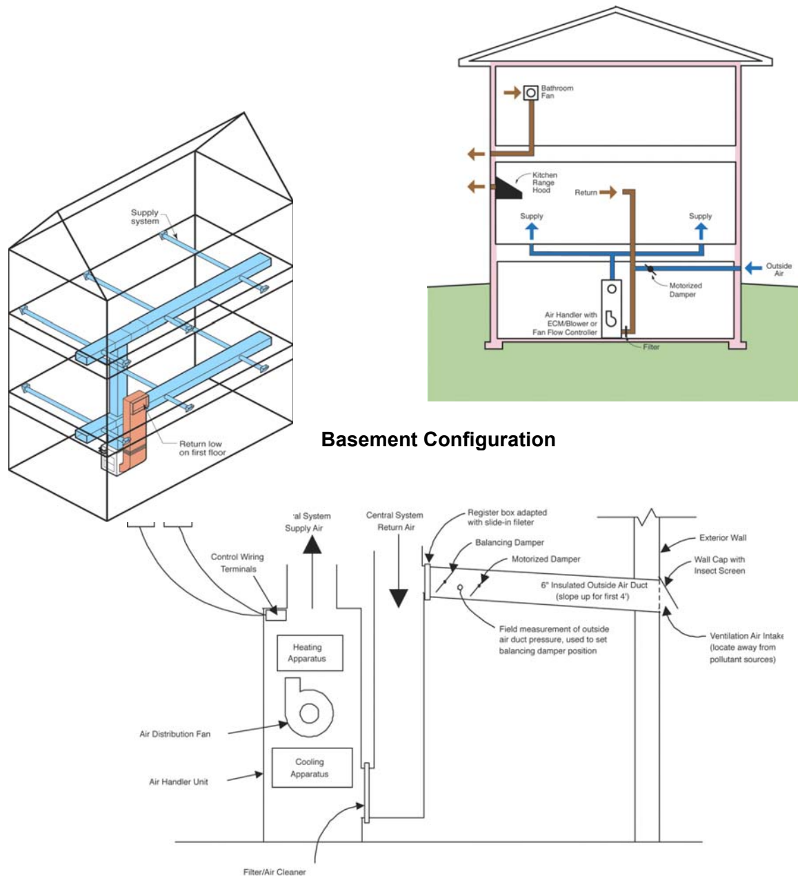
Figure 2-10. Recommended ventilation system
