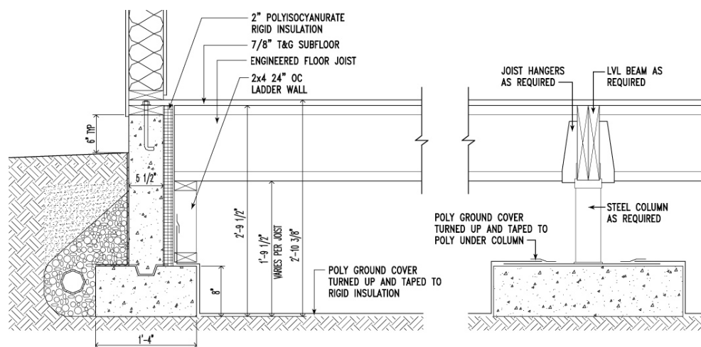
Figure 4-7. Conditioned crawlspace
