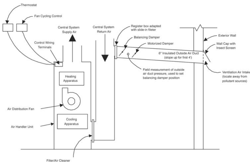
Figure 2-14. HVAC configuration
