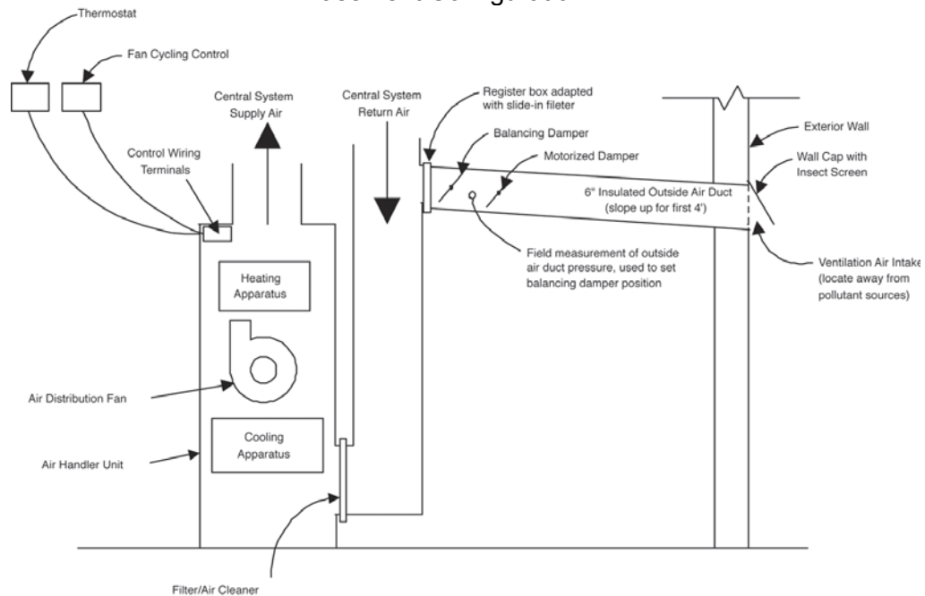
Figure 3-18. Mechanical ventilation in the "Louisville"
