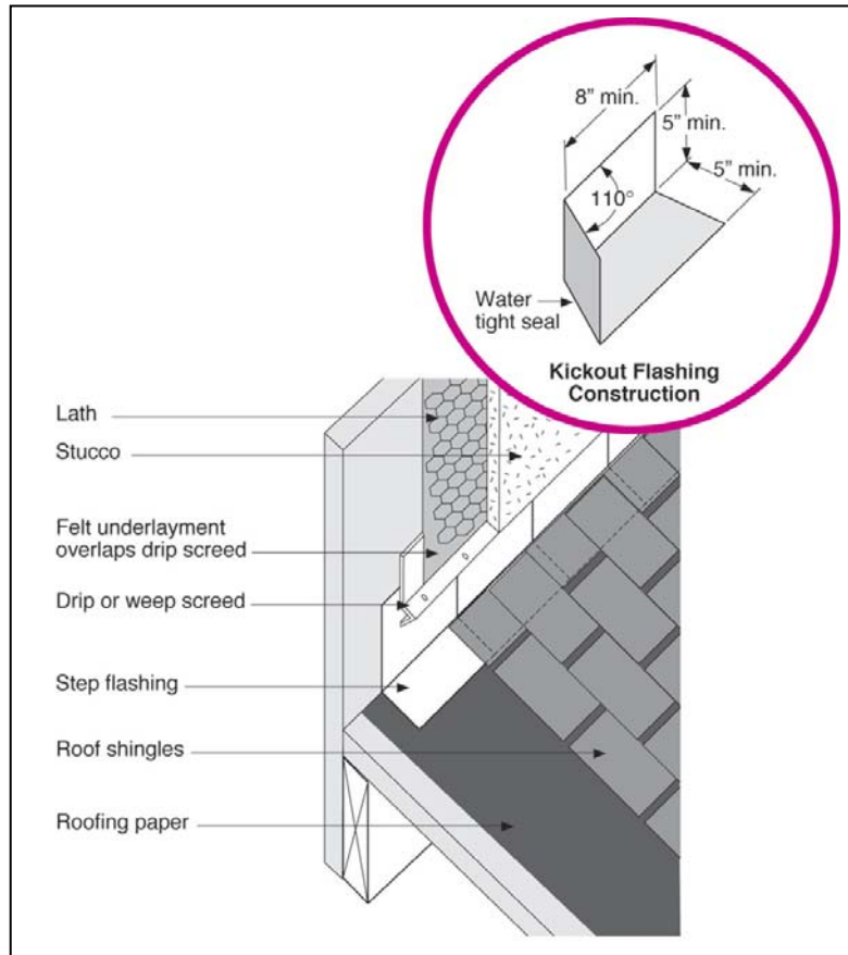
Figure 2-15. Stucco flashing
