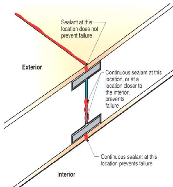
Figure 1-16. Sealant locations between panels
