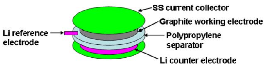
Figure III-1. Three-electrode cell configuration for formation experiments.
