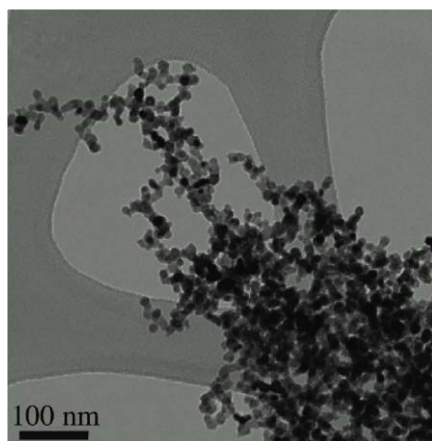
Figure IV-26. TEM image of \text{MoO}_3 HWCVD nanoparticles.
