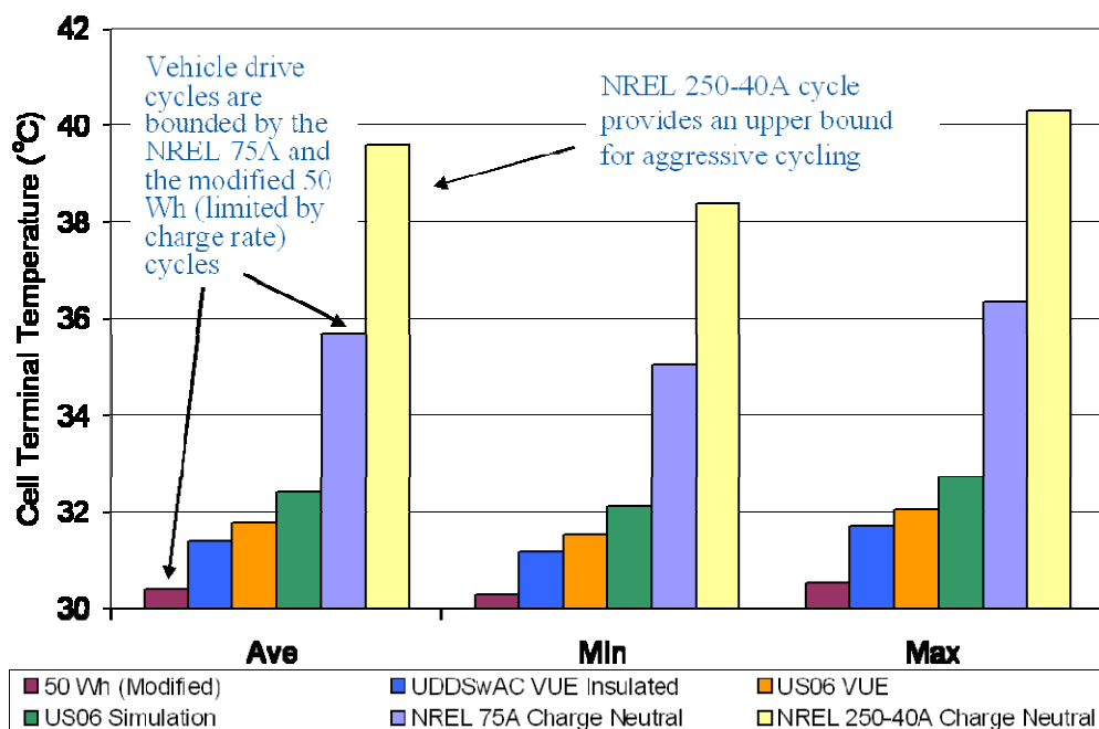
Figure II-4. Comparison of cell terminal temperatures for several drive cycles with ambient and coolant temperatures at 30°C.
