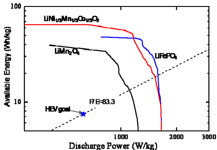
Figure IV-55. Optimal available energy vs. discharge power for baseline chemistries.
