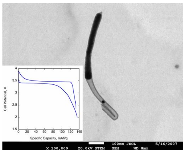
Figure IV-7. Carbon nanotube in \text{LiFePO}_4 sample and first cycle in Li cell.
