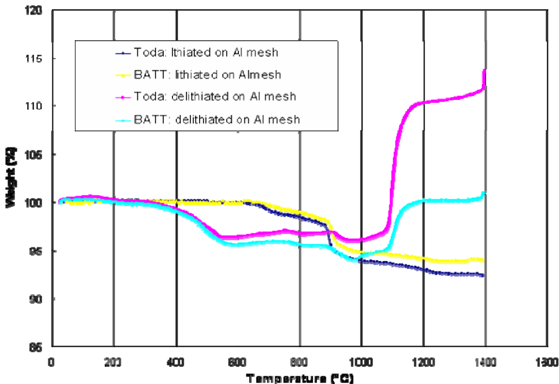
Figure IV-11. TGA of two Mn-spinel cathodes powders with and without lithium.
