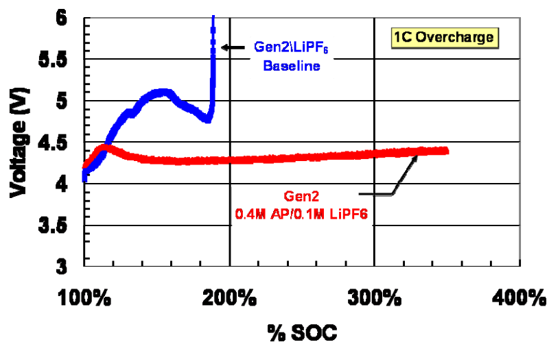
Figure III-43. Overcharge profile showing voltage for cells with and without Air Products overcharge shuttle salt.
