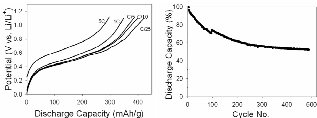
Figure IV-31. Rate (left) and cycling (right) performance of the C/Sn thin film nano-composite anode produced by MPVCVD on a Cu-foil. The electrode was charged at C/10 in the rate experiment, long-term cycling was performed at room temperature at the 1C rate.
