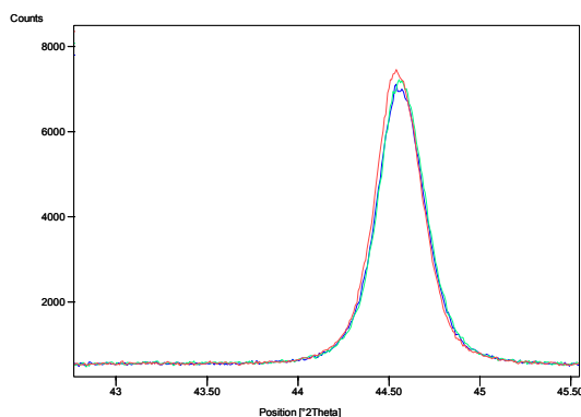
Figure III-10. 003 XRD peak showing no particle isolation in formatted Gen-3 cathodes.
