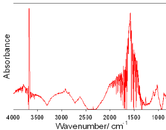
Figure IV-32. A typical FTIR microscopy spectrum of the SEI layer at the cycled thin-film Sn anode.
