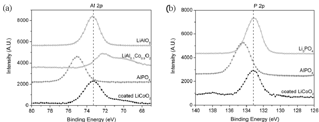
Figure IV-52. XPS spectra of the (a) Al 2p and (b) P 2p photoemission lines for AlPO 4 -coated LiCoO 2 and pure AlPO 4 . The large shifts to lower binding energy for the coated LiCoO 2 relative to the reference AlPO 4 for both spectra indicate that the Al and P are not present as AlPO 4 in the surface coating. The oxidation states of Al and P on the coated LiCoO 2 surface are similar to those of P in Li 3 PO 4 and Al in LiAlO 2 . Dashed lines indicate peak positions in the coated LiCoO 2 sample.
