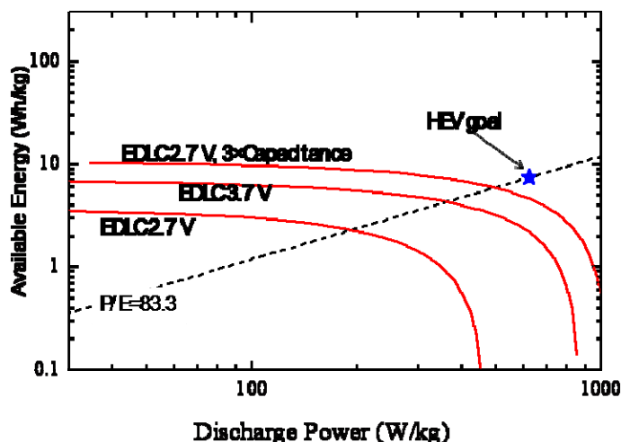
Figure IV-57. Possible UCap improvements vs. HEV goal.
