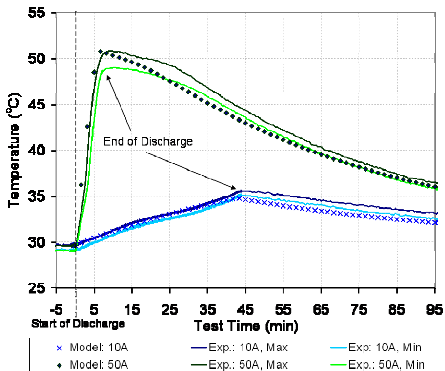
Figure II-6. Validation of thermal model with experiment measurements at different constant discharge rates.
