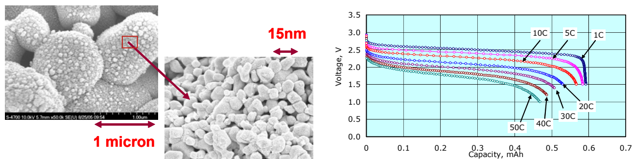
Figure: Cells incorporating Argonne's nano-phase lithium titanate material exhibit extremely high rate capability when coupled with lithium manganese spinel cathode.
