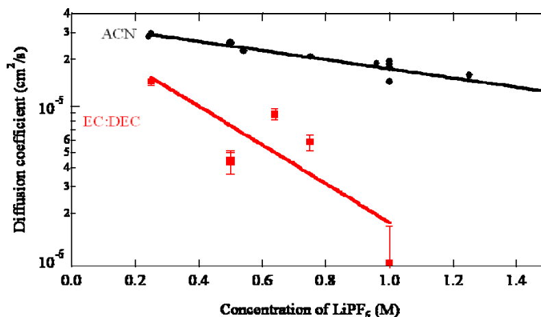
Figure IV-53. Diffusion-coefficient results for LiPF 6 in ACN and in EC:DEC at 296 K. The diffusion coefficients are seen to decrease with increasing salt concentration. Results for LiPF 6 in EC:DEC at higher concentrations have more error because the diffusion coefficient is approaching the limitations of the technique (ca. 10 -6 cm 2 /s).
