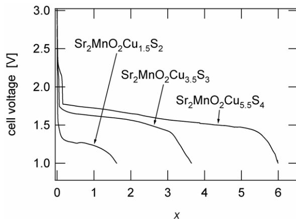
Figure IV-22. The first discharge of \text{Sr}_2\text{MnO}_2\text{Cu}_{2m-0.5}\text{S}_{m+1} for m = 1, 2, 3 , vs. a \text{Li}|\text{Li}^+ negative electrode, with a discharge rate of \text{C}/20 (i.e., all the Cu ions are replaced by Li within 20 hours). x denotes the number of Li ions inserted per formula unit.
