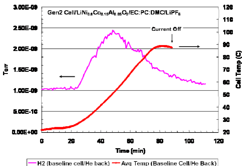
Figure III-42. Overcharge profile showing heat and hydrogen generation starting at 100% SOC.
