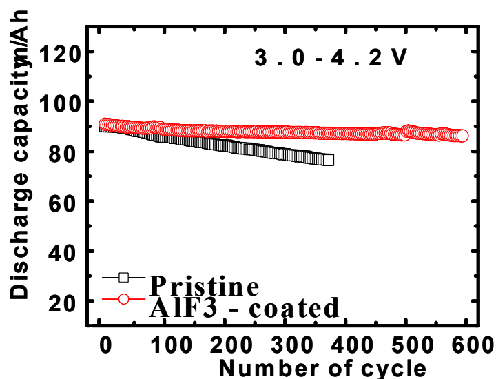
Figure III-47. Continuous charge-discharge curves of C/pristine Gen2 and C/ \text{AlF}_3 -coated Gen2 cell.
