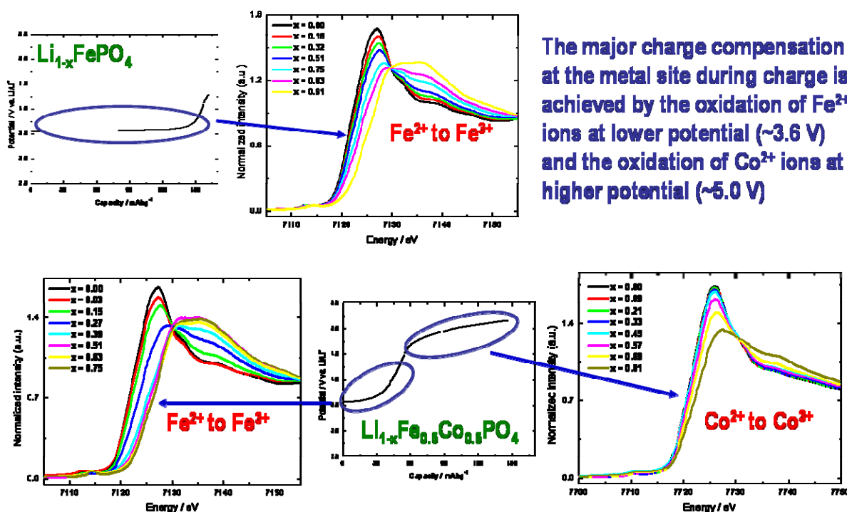
Figure IV-8. In situ Fe K-edge XAS for \text{Li}_{1-x}\text{FePO}_4 and Fe and Co K-edge for \text{Li}_{1-x}\text{Fe}_{0.5}\text{Co}_{0.5}\text{PO}_4 during charge.
