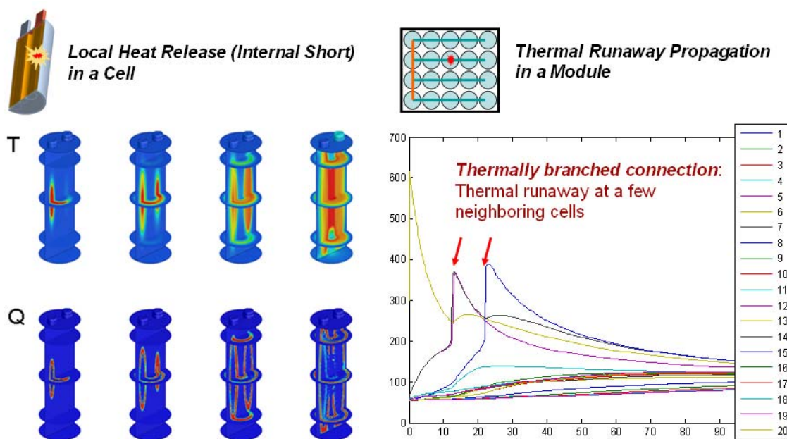
Figure II-12. Results of chemical-thermal modeling of lithium-ion battery thermal runaway: cell-internal abuse reaction propagation during internal short circuit event (left), thermal runaway propagation through a module after the red-marked cell goes into thermal runaway (right).
