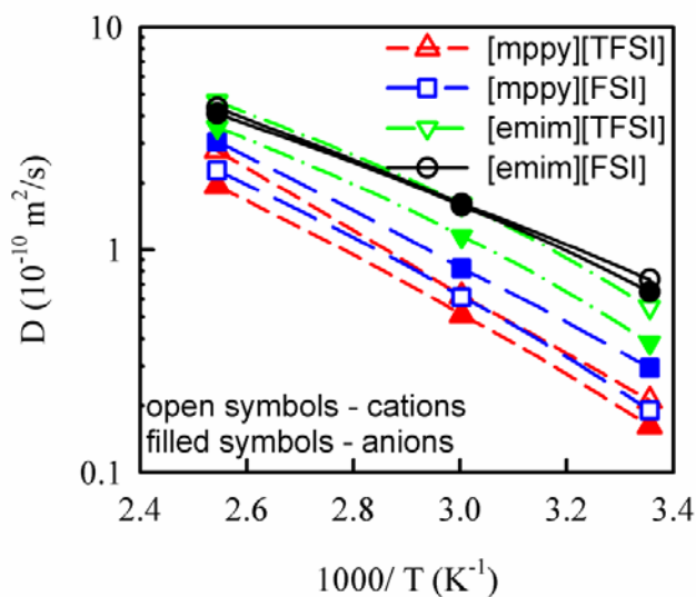
Figure IV-45. Ion self-diffusion coefficients predicted from MD simulations.
