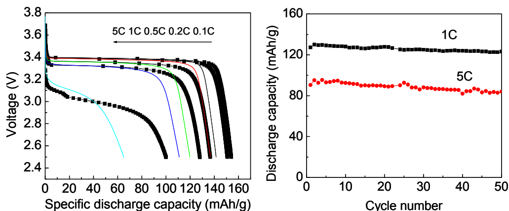
Figure IV-2. Rate capability of C- \text{LiFePO}_4 /PAN. The light curves are for C- \text{LiFePO}_4 without PAN (left). Discharge capacity vs. cycle number for C- \text{LiFePO}_4 /PAN at 1C and 5C (right).
