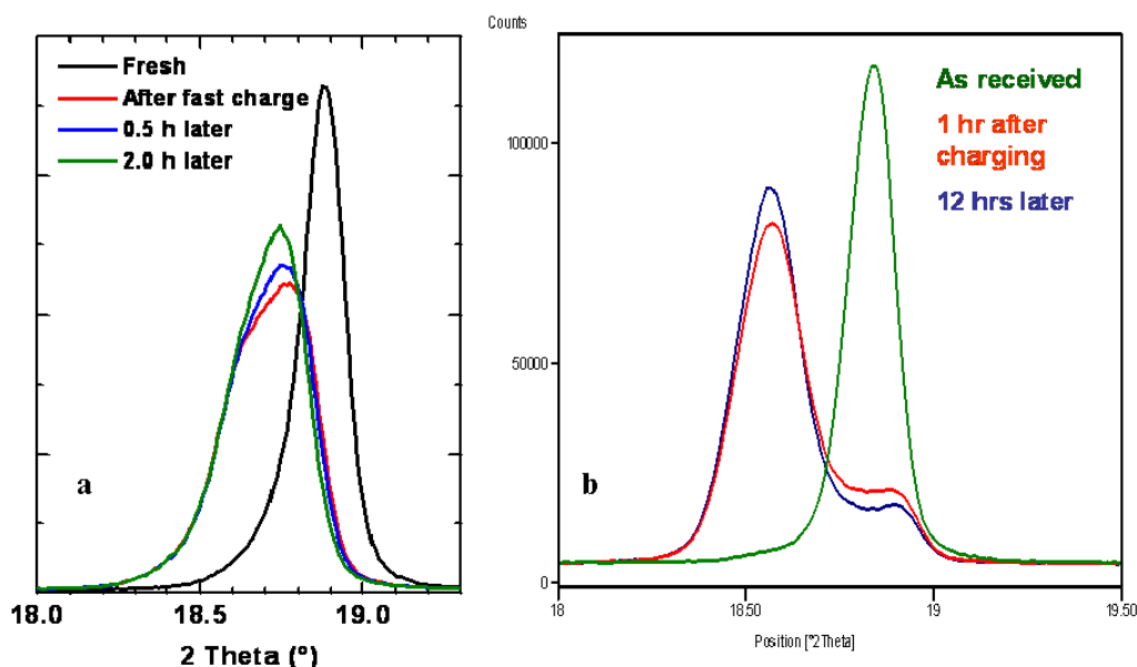
Figure III-9. 003 XRD peak showing particle isolation in a) fresh and b) aged Gen-2 cathodes.
