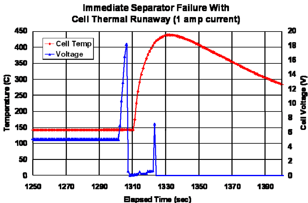
Figure III-33. Immediate 20V Breakdown with Cell Thermal Runaway.
