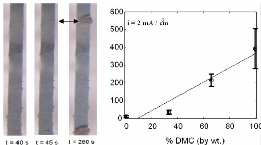
Figure IV-33. Method to detect a dendrite (left) and dendrite detection time vs. PC/DMC ratio (right).
