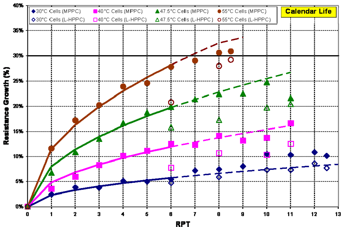
Figure III-13. Average, temperature-compensated, discharge resistance growth of all groups of cells calendar-life tested at SOC MAX and four different temperatures.
