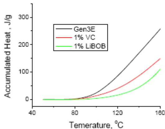
Figure III-28. Effect of electrolyte additives on the heat generated from lithiated graphite.
