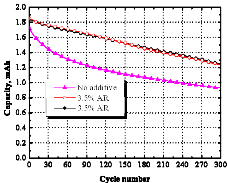
Figure III-40. Capacity retention at 55°C of MCMB/Gen3 cells showing the positive impact of PFPTFBB (shown as AR in the labels).
