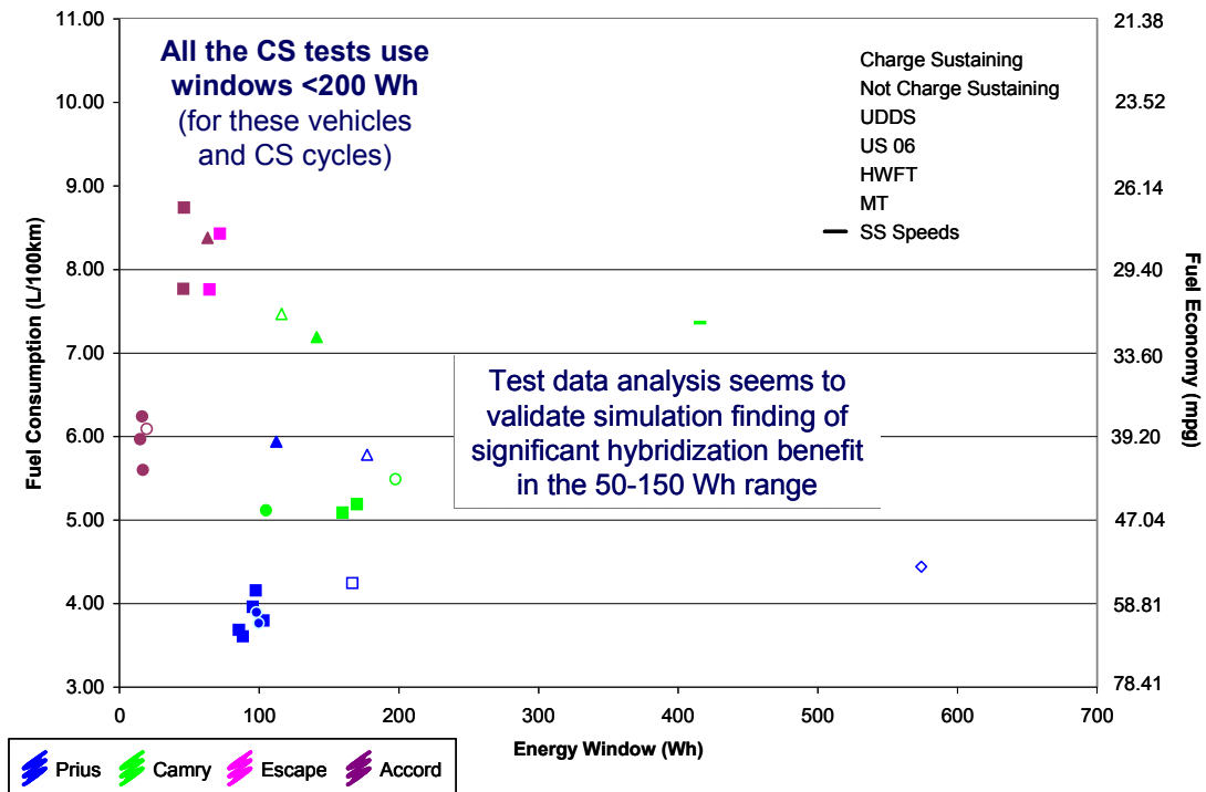
Figure II-11. Test data analysis for four commercial hybrids over several test cycles: the Urban Dynamometer Driving Schedule (UDDS), US06 profile, Highway Fuel Economy Test (HWFT), a mountain trace (MT) and steady- state (SS) speed testing. All charge-sustaining tests for these vehicles use energy windows smaller than 200 Wh.
