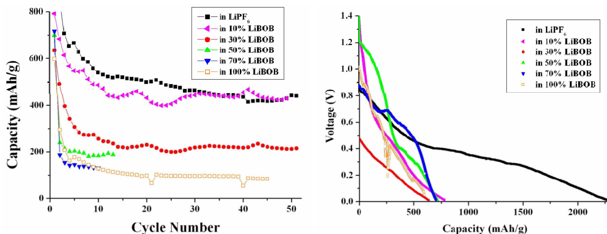
Figure IV-29. Electrochemical behavior of MnO nanofibers: (left) discharge capacities in LiBOB/LiPF 6 mixed electrolytes, and (right) first discharge capacity showing the elimination of the excess capacity by LiBOB.
