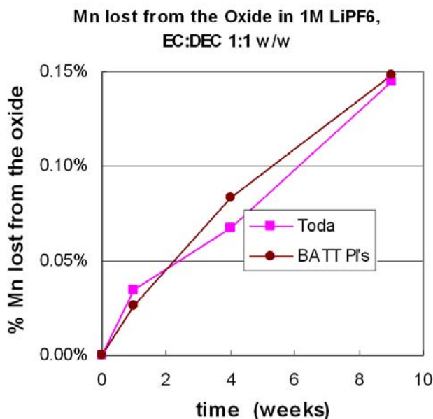
Figure IV-12. Toda and BATT Mn-spinel sample Mn dissolution. The amount of Mn found in solution was measured over time using ICP-OES. The amount of Mn found in the electrolyte was used to calculate the amount of Mn that was lost from the oxide.
