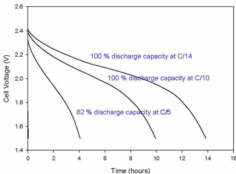
Figure IV-41. Discharge curves for cells of composition Li_4Ti_5O_{12} / IM550 + 50 wt% PEGDME / LiCoO_2 composite cathode.
