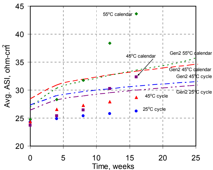
Figure III-6. Average ASI vs. time comparing the values obtained from the Gen3 additive pouch cells with those from Gen2 baseline cells. The curves represent the best-fit to Gen2 data and the points are the Gen3 data under the same conditions.
