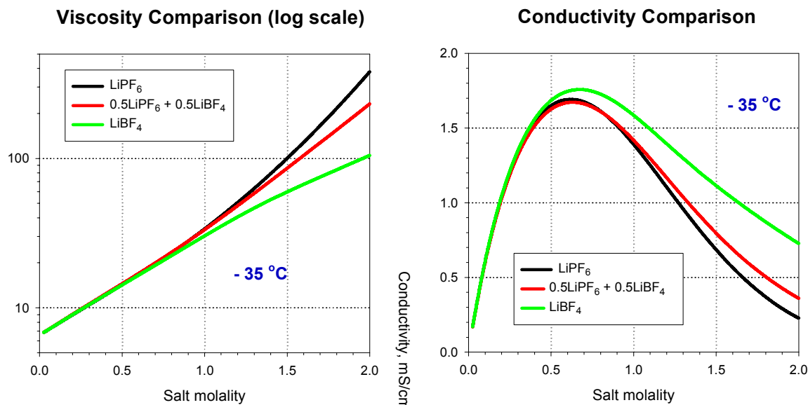
Figure III-24. Comparison of AEM results for viscosity and conductivity of single and mixed-salt electrolytes having gamma-butyrolactone as the solvent.
