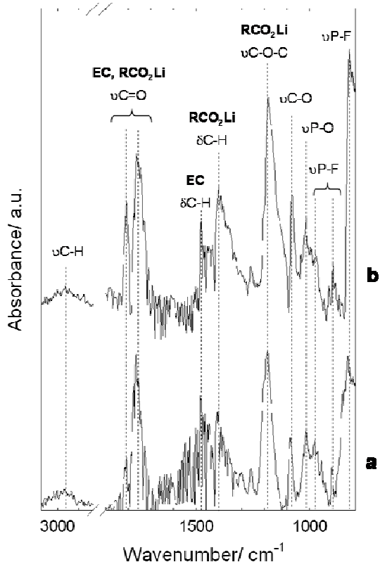
Figure III-4. FTIR spectra of cycled (a) un-sputtered and (b) 120s sputtered Mag-10 electrodes, washed in DMC.
