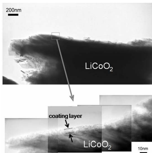
Figure IV-49. Cross-sectional TEM images of the “ \text{AlPO}_4 ”-coated \text{LiCoO}_2 show uniform coverage of the particle surface, with a thickness variation of 10-100 nm. High-resolution TEM images of the coating cross-section show a light-dark variation which may indicate regions of varying composition or thickness in the coating.
