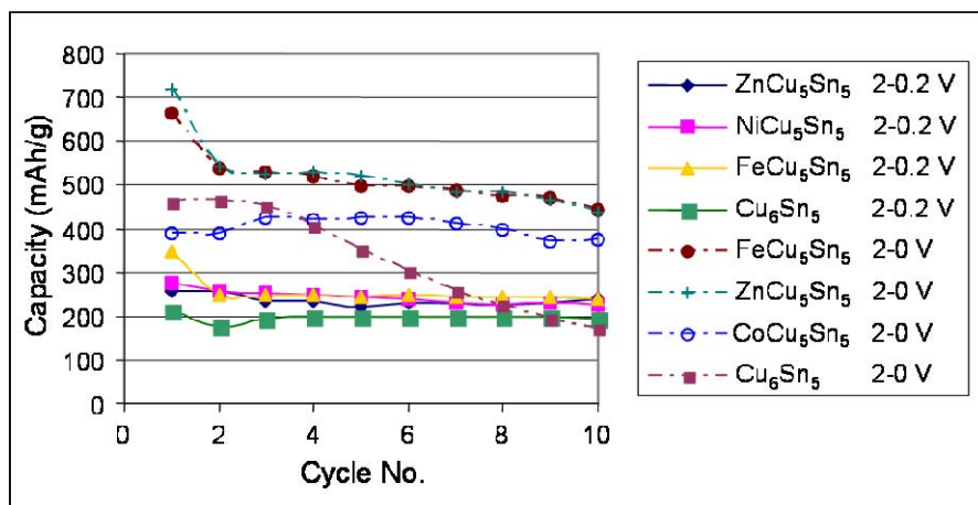
Figure IV-24. Capacity vs. cycle no. plots of various Li/Cu 5 MSn 5 cells (M= Fe, Co, Ni, Zn).
