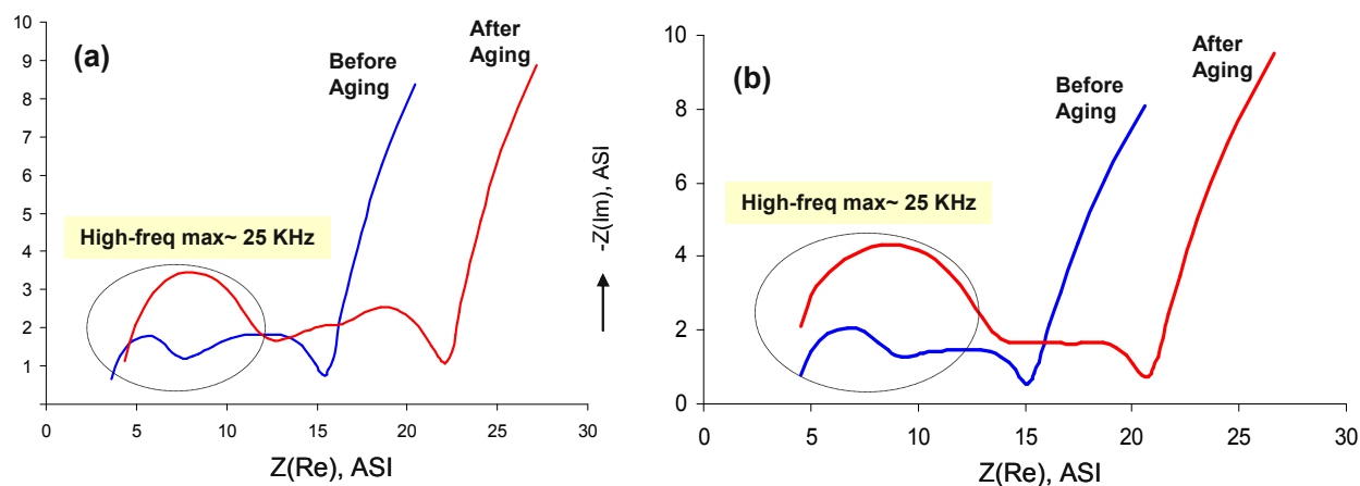
Figure III-7. EIS data from a Gen3 electrode pouch cell that contained the following electrolytes: (a) Gen2 and (b) Gen2 + 3 wt% \text{LiF}_2\text{BC}_2\text{O}_4 . The data were acquired at 3.72V, 30°C, and between 100kHz-10mHz. The cells were aged at 55°C.
