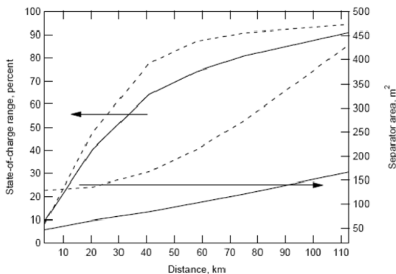
Figure IV-54. Comparison between the graphite – manganese oxide spinel (solid curves) and titanate spinel – iron phosphate (dashed curves) electrode systems for various all-electric driving distances.
