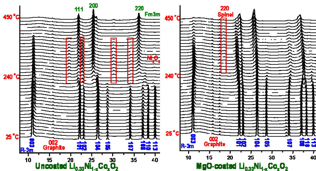
Figure III-19. Time resolved in-situ XRD spectra of uncoated and \text{MgO} coated fully charged \text{Li}_{0.33}\text{Ni}_{1-x}\text{Co}_x\text{O}_2 cathodes during heating.
