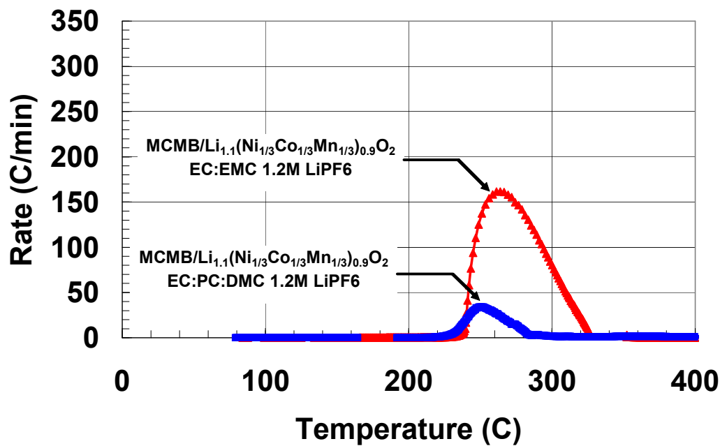
Figure III-35. ARC profile showing significant reduction in heating rate for the less reactive Gen3 cathode material with EC:PC:DMC.
