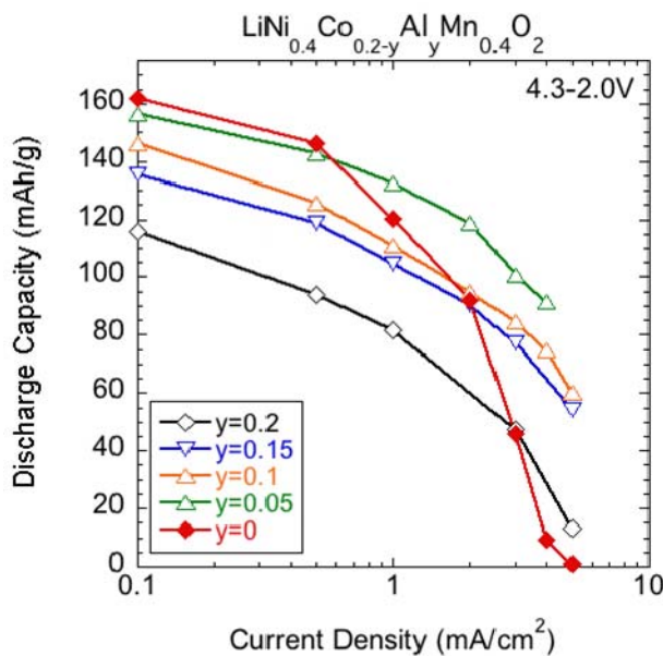
Figure IV-15. Rate behavior of \text{Li}[\text{Ni}_{0.4}\text{Co}_{0.2-y}\text{Al}_{0.1}\text{Mn}_{0.4}]\text{O}_2 electrodes ( y=0.05-0.2 ) in Li cells, 4.3-2.0V.
