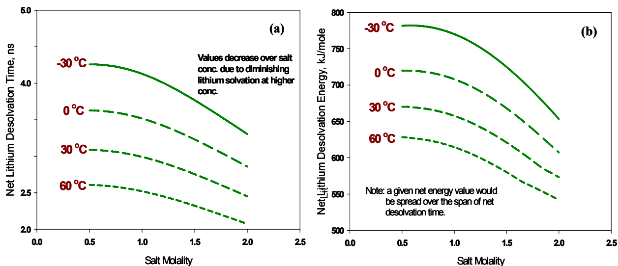
Figure III-23. Net requirements for (a) lithium desolvation time, and (b) lithium desolvation energy, as determined from kinetic and thermodynamic analyses via the AEM.
