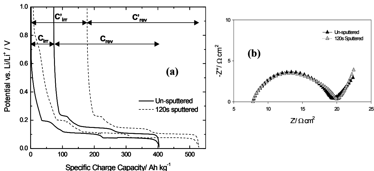
Figure III-3. (a) First galvanostatic charge-discharge curves of un-sputtered (—) and 120s sputtered (--) Mag-10 graphite in 1.0 M LiPF 6 , EC:DMC 1:1 w/w at C/25. (b) Impedance spectra, measured at 0.05 V vs. Li/Li + , of cycled un-sputtered (—) and 120s sputtered (--) Mag-10 anodes.
