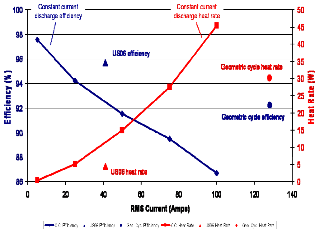
Figure II-2. CPI Gen 4.2 (5 Ah) cell's heat generation rate and efficiency for various profiles at 30°C.
