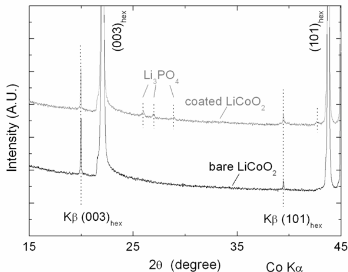
Figure IV-50. XRD patterns of bare \text{LiCoO}_2 and \text{AlPO}_4 -coated \text{LiCoO}_2 show the appearance of peaks corresponding to \text{Li}_3\text{PO}_4 in the coated sample.
