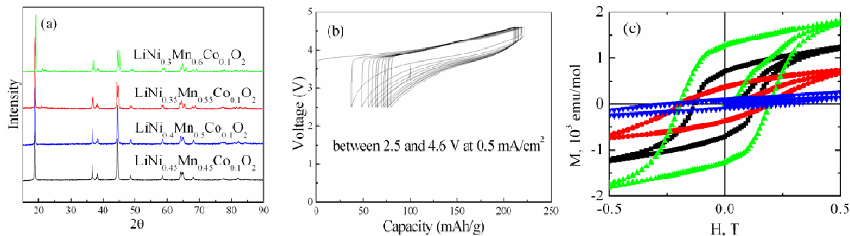
Figure IV-14. (a) XRD patterns of \text{Li}[\text{Ni}_y\text{Mn}_{0.9-y}\text{Co}_{0.1}]\text{O}_2 , 0.3 \leq y \leq 0.45 ; (b) charge-discharge curves for \text{LiNi}_{0.4}\text{Mn}_{0.5}\text{Co}_{0.1}\text{O}_2 cycled between 2.5 and 4.6 V at 0.5 \text{ mA/cm}^2 ; (c) magnetization curves of \text{NaNi}_{0.5}\text{Mn}_{0.5}\text{O}_2 (blue triangles), \text{LiNi}_{0.5}\text{Mn}_{0.5}\text{O}_2 ion-exchanged in: LiBr solution at 160-170°C (red circles); ion-exchanged at 280°C in molten salts (green triangles); and synthesized by high-temperature solid-state reaction (black squares).
