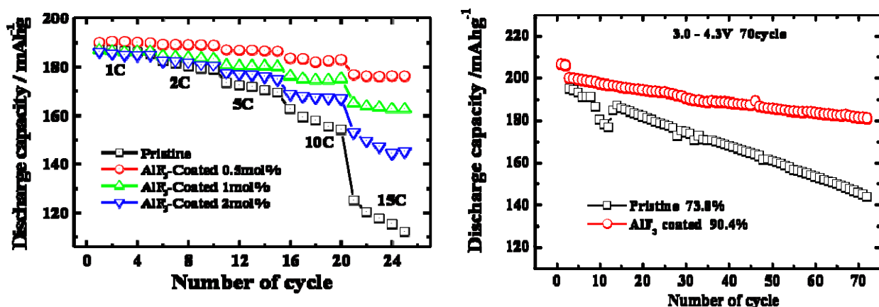
Figure III-46. Comparison of pristine and AlF 3 coated Gen2 material: rate capability (left), cycling stability (right).
