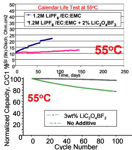
Figure 1. More stable impedance & capacity are achieved with additive.
