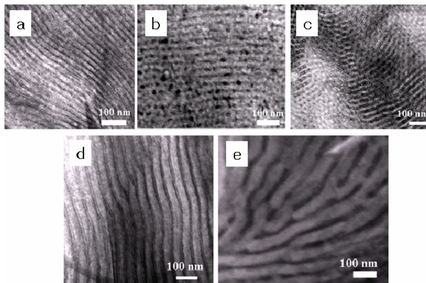
Figure IV-38. TEM of the pure SEO copolymers: a) SEO(16-16); b) SEO(36-25); c) SEO(40-31); d) SEO(40-54); e) SEO(74-98). The PEO phase is darkened by RuO 4 staining.
