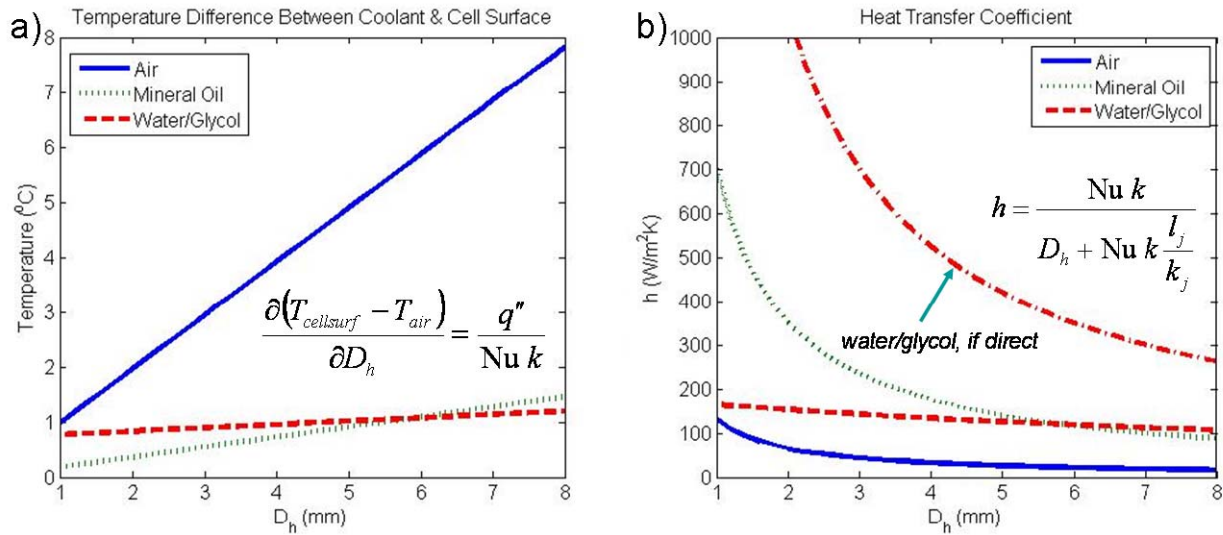
Figure II-8. Steady state laminar channel flow relations; (a) temperature difference between coolant and cooling surface, and (b) heat transfer coefficient at cooling surface to hydraulic diameter of channel.
