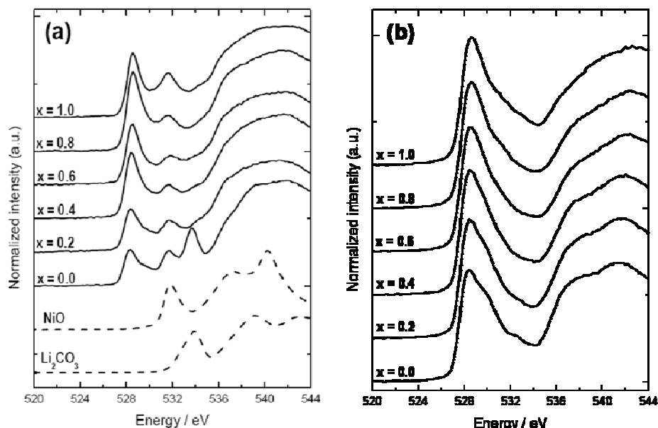
Figure IV-17. Normalized O K-edge XAS spectra of \text{Li}_{1-x}\text{Ni}_{0.8}\text{Co}_{0.15}\text{Al}_{0.05}\text{O}_2 electrode at different x values using (a) PEY method and (b) FY method.
