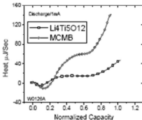
Figure III-29. Comparison of the heat measured by isothermal microcalorimetry during the lithiation process of graphite and \text{Li}_4\text{Ti}_5\text{O}_{12} .
