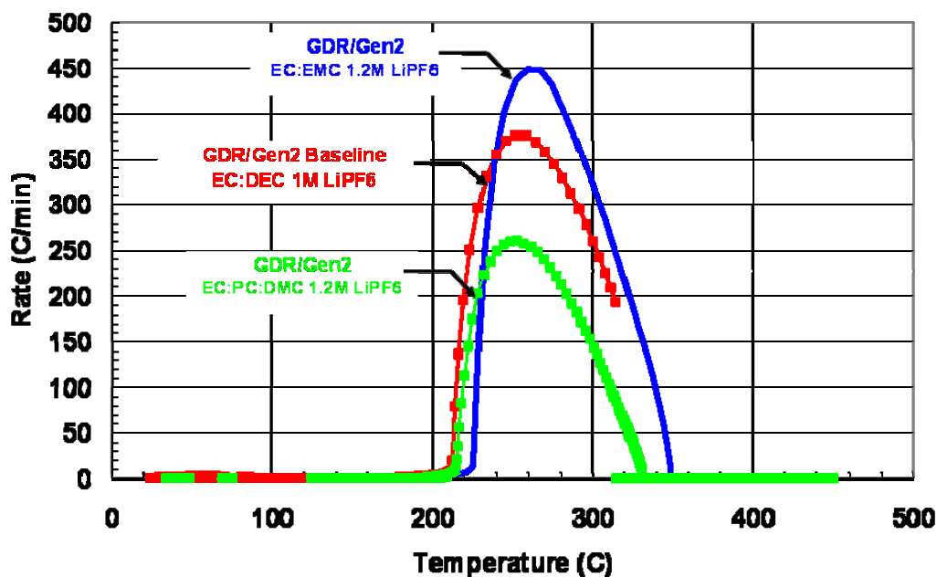
Figure III-34. ARC thermal runaway profiles showing improved thermal response with EC:PC:DMC based electrolytes.
