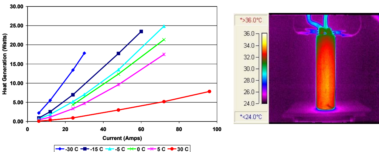
Figure II-1. Heat generation rate of JCS Gen II cells at various temperatures and currents (left), Thermal image of Gen II Cell at the end of 72 A constant current discharge (right).
