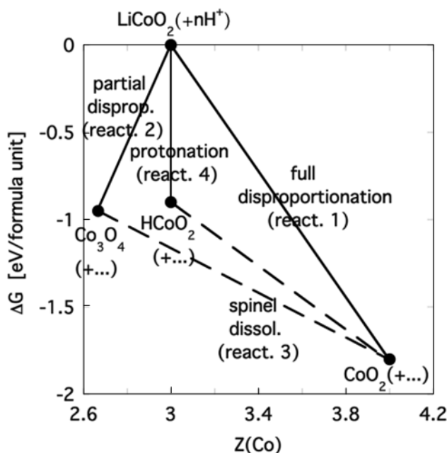
Figure IV-13. Schematic representation of the free energy magnitude ( \Delta G ) for various reactions of \text{LiCoO}_2 with acid.
