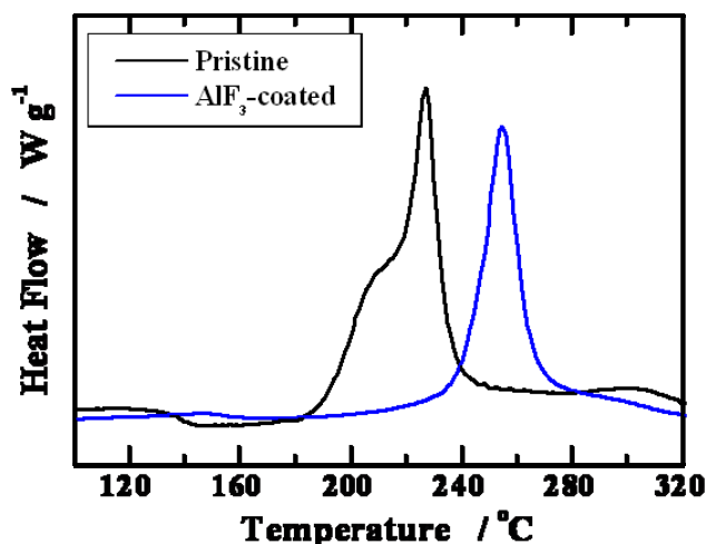
Figure III-48. DSC profiles of pristine Gen2 and \text{AlF}_3 -coated Gen2 cell charged to 4.3 V.
