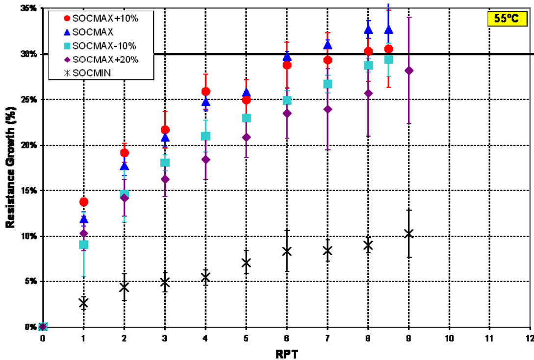
Figure III-14. Average, temperature-compensated discharge resistance growth for groups of cells calendar-life tested at 55°C.
