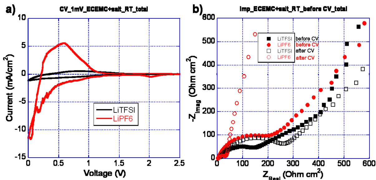
Figure III-2. Cyclic voltammetry (a) and impedance (b) of Gen-2 anodes versus a lithium reference electrode in 3-electrode configuration for EC/EMC-LiX (1.2M), where X=PF 6 or TFSI.
