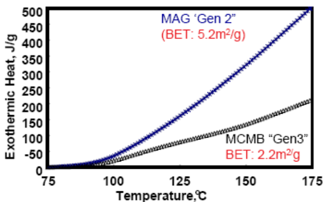
Figure III-27. Accumulated heat curves of two lithiated graphites with different surface areas
