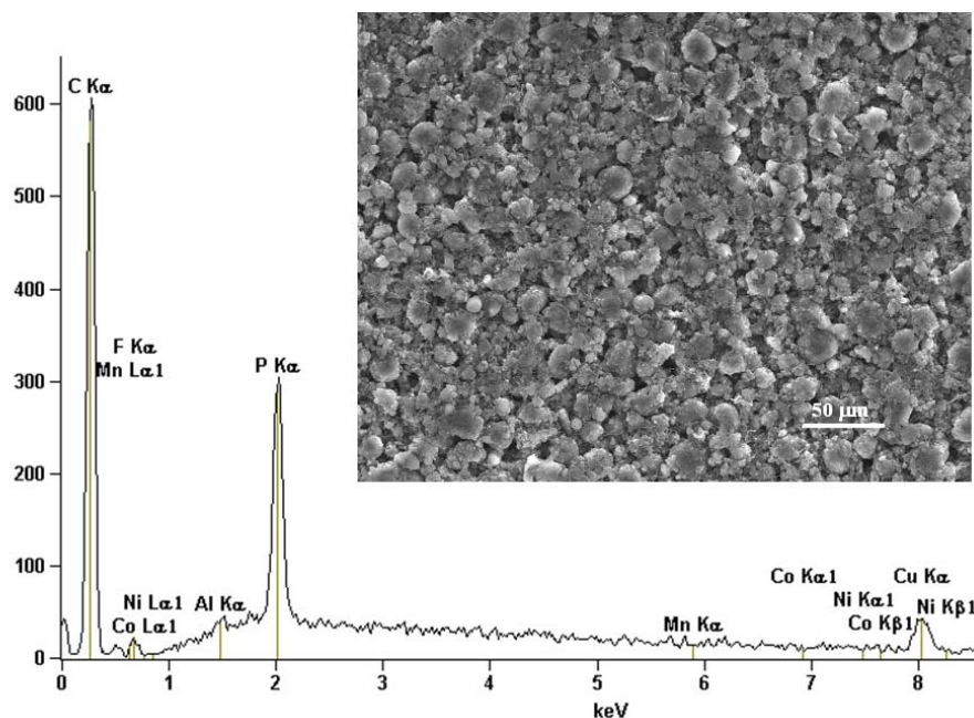
Figure III-11. SEM/EDX of aged Gen-3 anode (DAP10).
