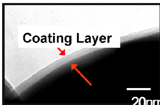
Figure III-45. Bright- field TEM images of AlF 3 -coated Li[Ni 0.8 Co 0.15 Al 0.05 ]O 2 .
