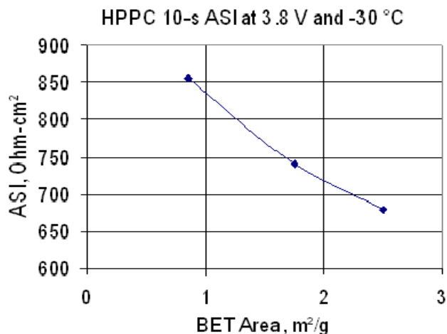
Figure III-21. HPPC ASI of three ConocoPhillips’ graphites with varying surface area at -30°C.
