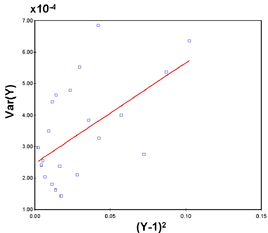
Figure III-16. Error model fit. The variance of the data at a given temperature and time is plotted versus the square of the resistance rise as predicted by the model at the same temperature and time. The line is a linear fit of the data whose slope is \sigma_\delta^2 and whose intercept is 2\sigma_\epsilon^2 .
