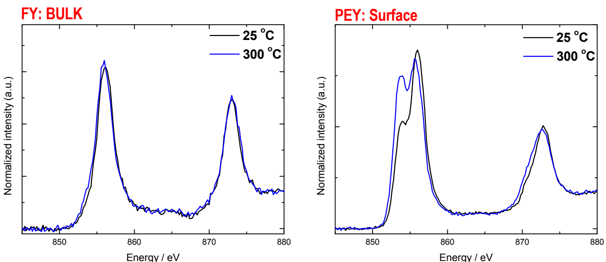
Figure III-18. Ni L-edge XAS for \text{Li}_{1-x}\text{Co}_{1/3}\text{Ni}_{1/3}\text{Mn}_{1/3}\text{O}_2 cathode at 100% SOC in bulk and at surface.
