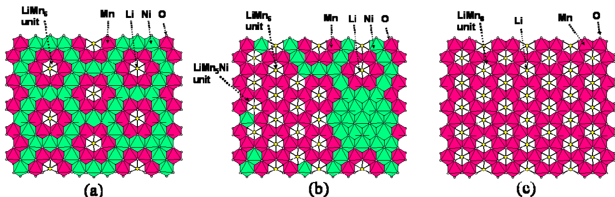
Figure IV-18. Schematic illustrations of the atomic arrangements in the transition metal (TM) layers of (a) \text{LiMn}_{0.5}\text{Ni}_{0.5}\text{O}_2 , (b) \text{Li}_{1+x}(\text{Mn}_{0.5}\text{Ni}_{0.5})_{1-x}\text{O}_2 ( x \approx 0.1 ) and (c) \text{Li}_2\text{MnO}_3 .
