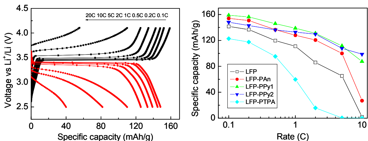
Figure IV-1. Rate capability of C- \text{LiFePO}_4 /PPy prepared with simultaneous chemical polymerization (left). Rate capabilities for C-LFP/polymer composite cathodes (right). LFP-PPy1 was obtained by electrodeposition; LFP-PPy was prepared with chemical polymerization (right).
