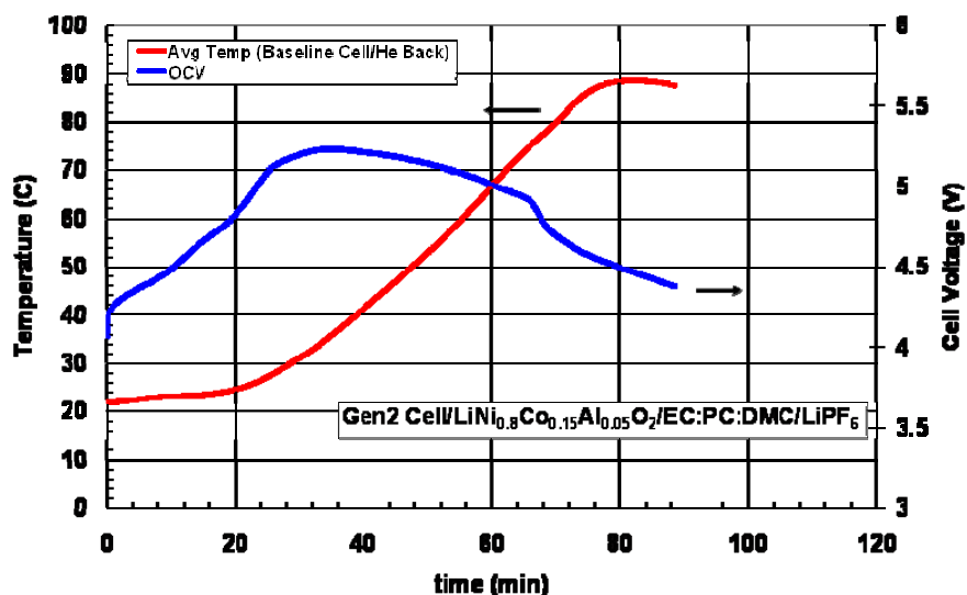
Figure III-41. Overcharge profile showing temperature and voltage correlation starting at 100% SOC.
