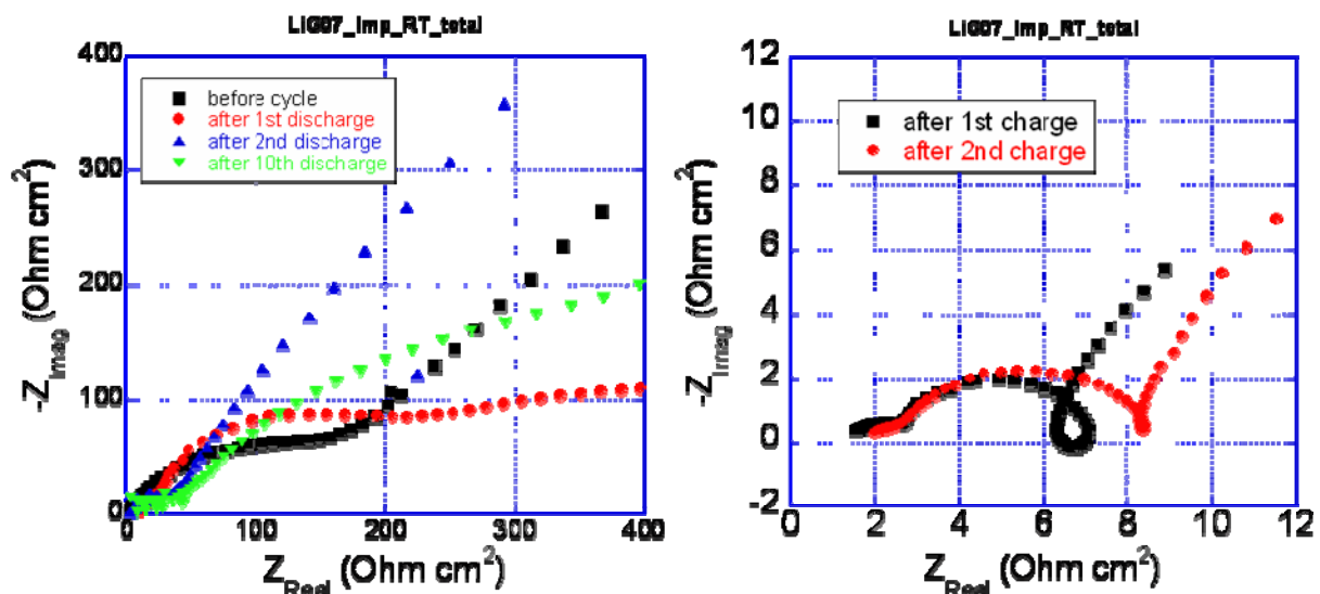
Figure IV-36. Nyquist plot of Li/EC/EMC + 1.2M LiTFSI/GEN2 cathode cell at room temperature. Working electrode: GEN2 cathode. Counter electrode: Li metal. Reference electrode: Li.
