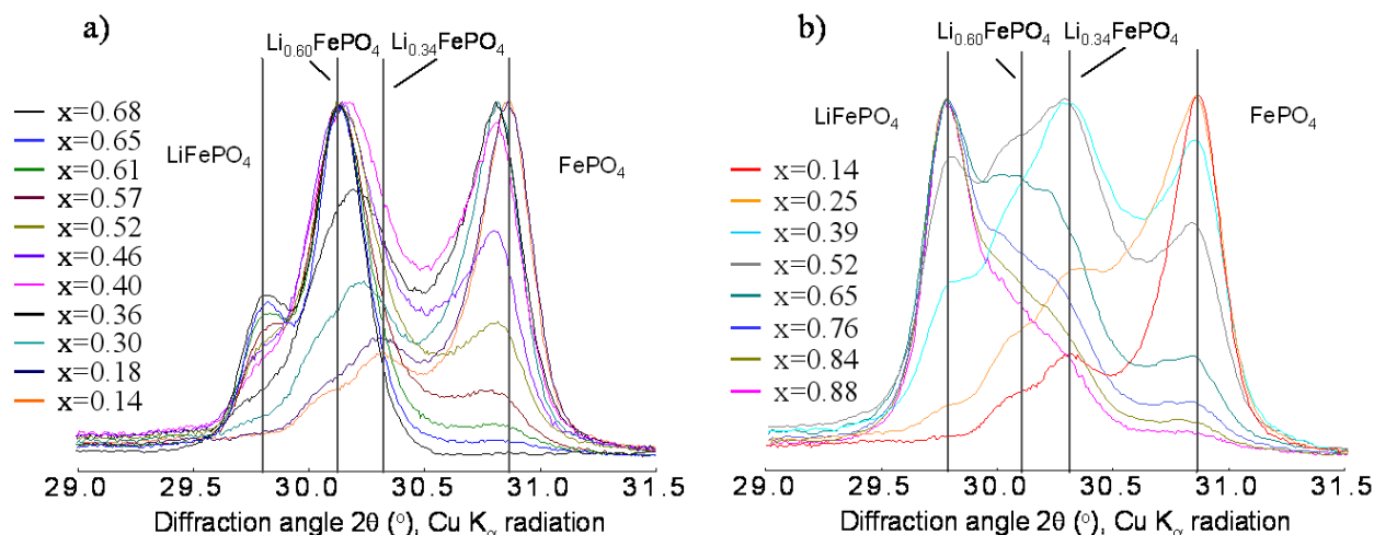
Figure IV-5. Ex situ XRD patterns of a \text{Li}_{0.68}\text{FePO}_4 solid solution electrode at various stages of electrochemical extraction and insertion of lithium. a) charging at 4.2 V; b) discharging at 2.5 V.
