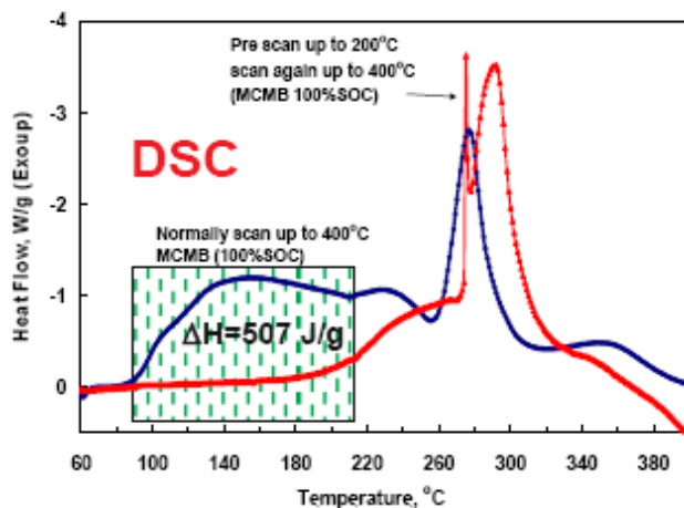
Figure III-26. DSC curves of lithiated graphite before (blue) and after (red) SEI decomposition
