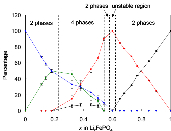
Figure IV-4. Room temperature phase diagram of \text{Li}_x\text{FePO}_4 crystals after cooling from a solid-solution state. (●) \text{LiFePO}_4 (●) \text{Li}_{0.60}\text{FePO}_4 (●) \text{Li}_{0.34}\text{FePO}_4 (●) \text{FePO}_4
