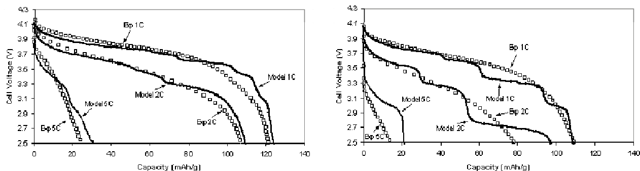
Figure IV-6. Model and experimental discharge comparisons for two porosities, left has a loading of 1.62 \text{ mA/cm}^2 with porosity=0.43, right has a loading of 1.53 \text{ mA/cm}^2 with porosity=0.71.
