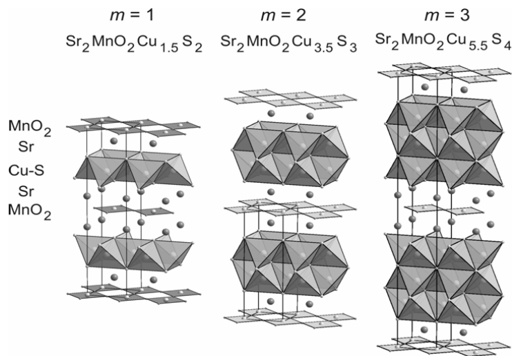
Figure IV-21. Structure of \text{Sr}_2\text{MnO}_2\text{Cu}_{2m-0.5}\text{S}_{m+1} ( m = 1, 2, 3 ).
