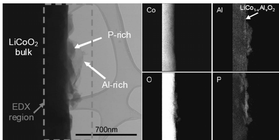
Figure IV-51. EDX mapping of “AlPO 4 ”-coated LiCoO 2 particle edge with STEM. Only the center region of the image has been mapped by EDX.
