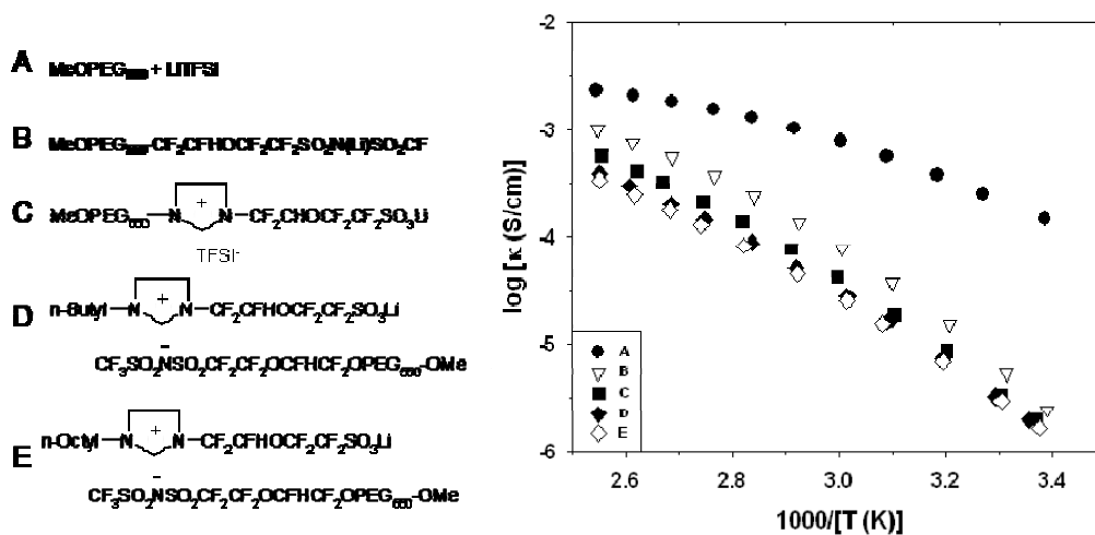
Figure IV-43. Structures and ionic conductivity data for a series of Li imidazolium fluorosulfonate and fluorosulfonimide IMs. Sample A is a binary salt (LiTFSI) dissolved in a polyether solvent; included for comparison.
