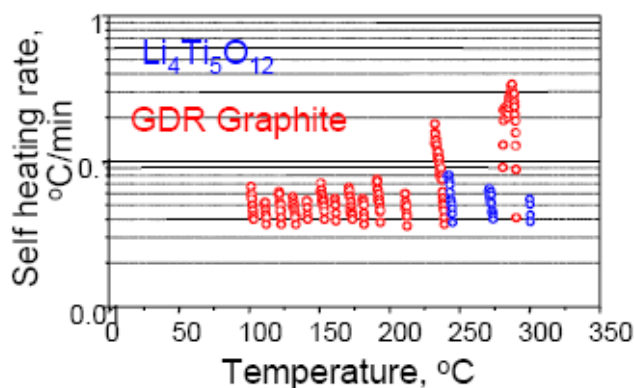
Figure III-30. ARC results of lithiated graphite and lithiated \text{Li}_4\text{Ti}_5\text{O}_{12} .
