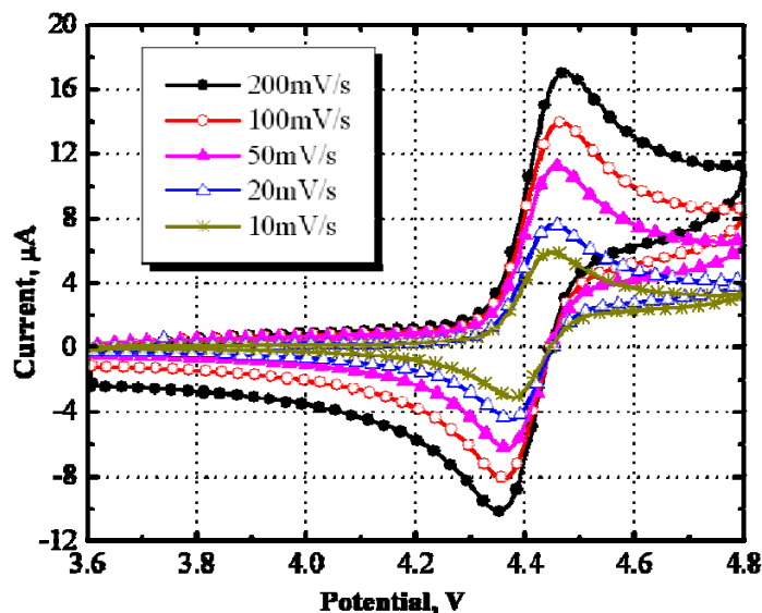
Figure III-38. Cyclic voltammograms of 0.05 M PFPTFBB and 1.2 M \text{LiPF}_6 in EC/EMC (3:7, by weight) using a Pt/Li/Li three-electrode cell.
