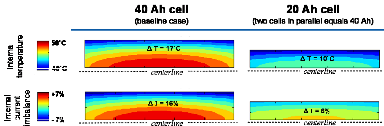
Figure II-9. Steady state internal temperature and current distributions in PHEV cylindrical cells under aggressive cycling. The 40Ah cell, with 17°C internal temperature imbalance and 16% current imbalance, may have a shorter life than the two 20Ah cells in parallel with a 10°C internal temperature imbalance and 6% current imbalance.
