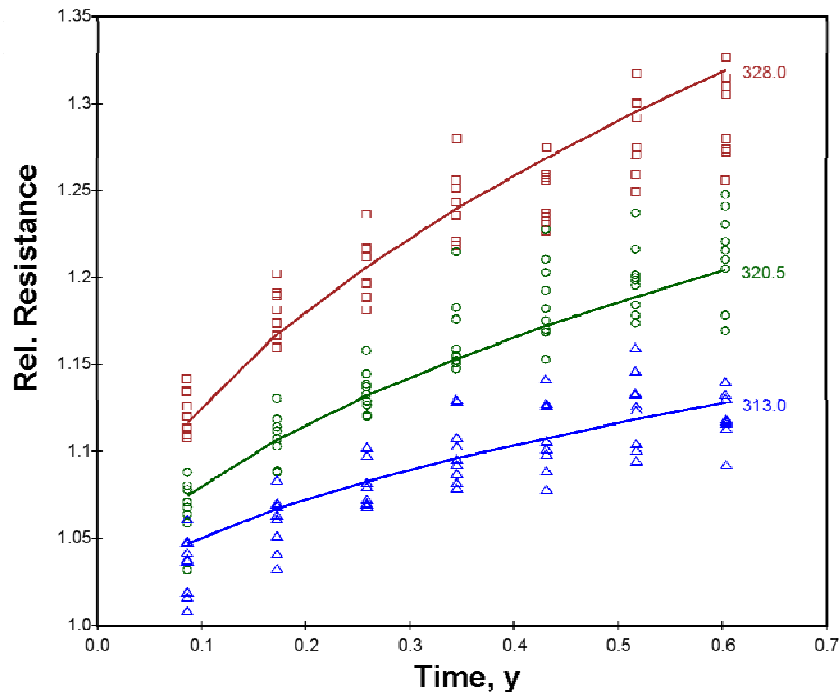
Figure III-15. Degradation model of calendar-life data. Temperature (K) is shown next to the curves.
