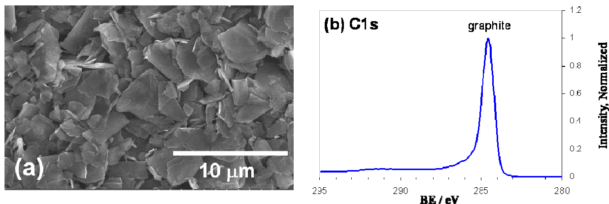
Figure III-5. Representative (a) SEM image and (b) XPS data, from fresh BF-graphite electrode
