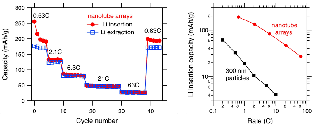
Figure IV-28. Rate capability of TiO 2 NT electrodes (left) and comparison with the rate capability of electrode composed of 300 nm particles (right). Data for 300 nm particle films was adapted from Maier et al, Adv. Mater. 19, 2087 (2007).
