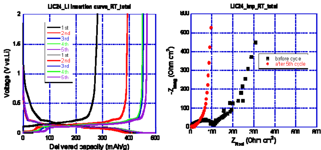
Figure IV-35. Voltage profile vs. Li reference of galvanostatic Li insertion/extraction (left) at 0.1mA at RT and Nyquist plot (right) for Li/EC/EMC(3/7 v/v) + 1.2M LiTFSI/Gen2 cell (Three electrode configuration- Li reference).
