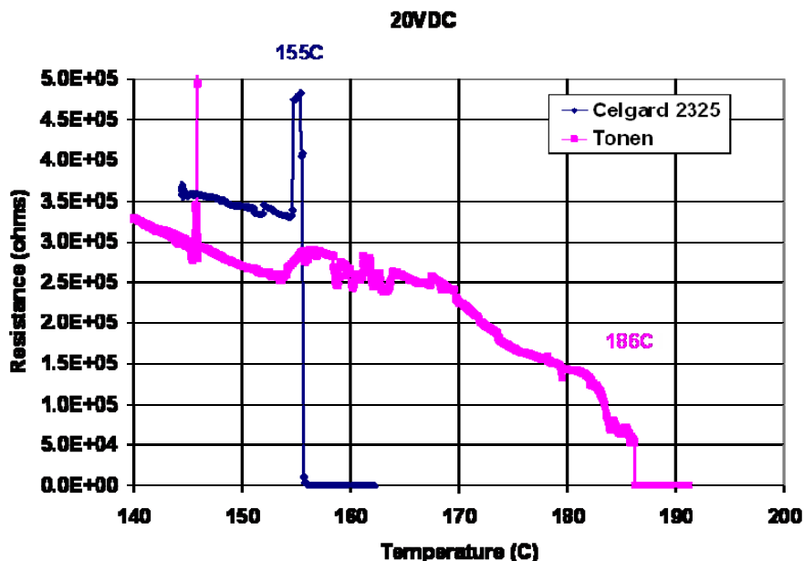
Figure III-32. Separator failure above shutdown with applied 20V.
