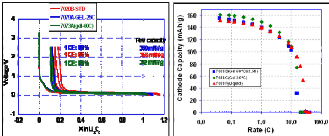
Figure IV-47. Left) Cycling of Li/graphite cells with the new gel polymer electrolytes at C/24. Right) Ragone plot of Li/LiFePO 4 cells with new gel polymer formed at 25°C and at 60°C.
