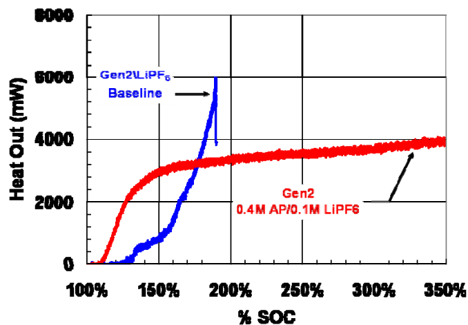
Figure III-44. Overcharge profile showing heat generation for cells with and without Air Products overcharge shuttle salt.
