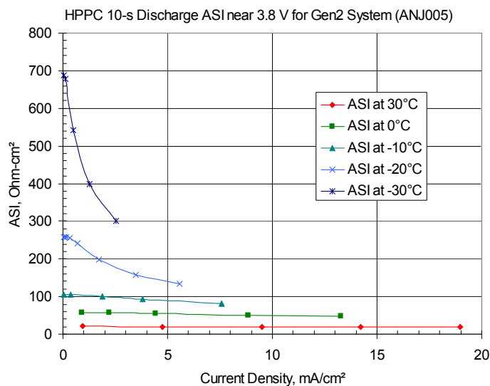
Figure III-22. ASI as a function of pulse current level for the Gen2 system with temperature as a parameter.
