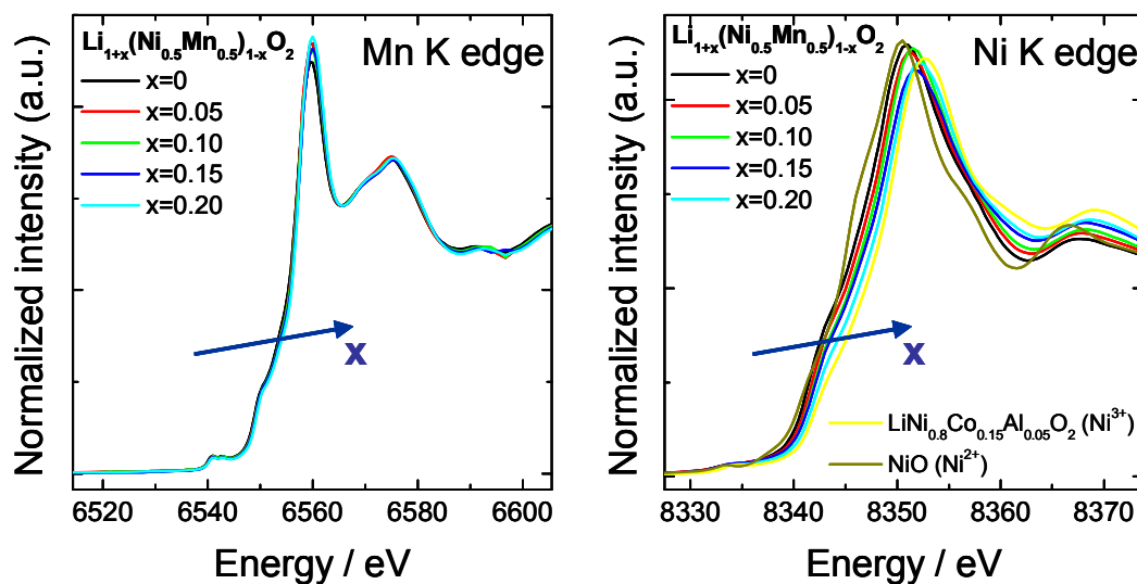
Figure IV-16. Normalized Mn and Ni K-edge XANES spectra of \text{Li}_{1+x}(\text{Ni}_{0.5}\text{Mn}_{0.5})_{1-x}\text{O}_2 powders as a function of x .
