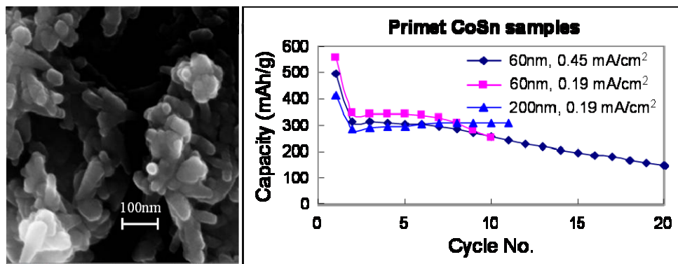
Figure IV-25. SEM image of \text{CoCu}_5\text{Sn}_5 particles (left), Cycling stability of 60nm and 200nm CoSn electrode particles (right).
