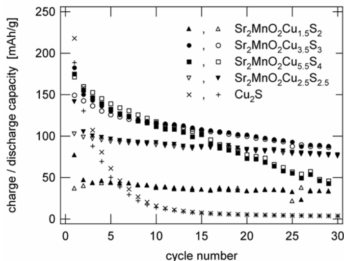
Figure IV-23. The charge and discharge capacities of \text{Sr}_2\text{MnO}_2\text{Cu}_{2m-0.5}\text{S}_{m+1} , m = 1-3 , and \text{Cu}_2\text{S} as a function of cycle number, between 2.7 and 1.1 V. Full symbols: discharge; empty symbols: charge; crosses: \text{Cu}_2\text{S} .
