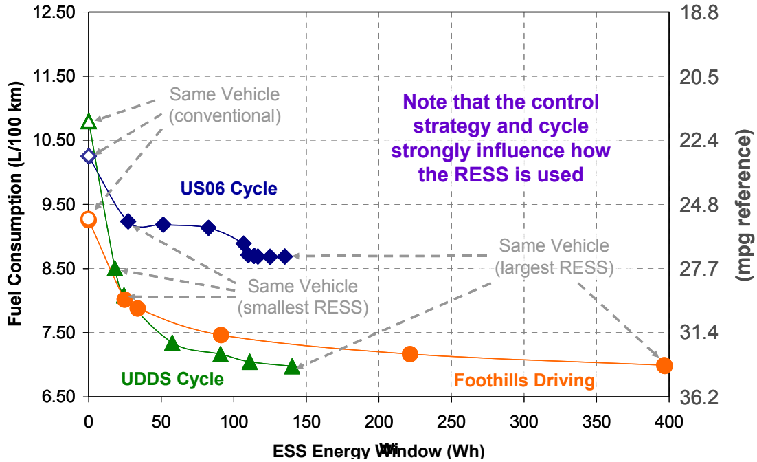
Figure II-10. Simulation results for different rechargeable energy storage system (RESS) vehicle cases over three different drive cycles.
