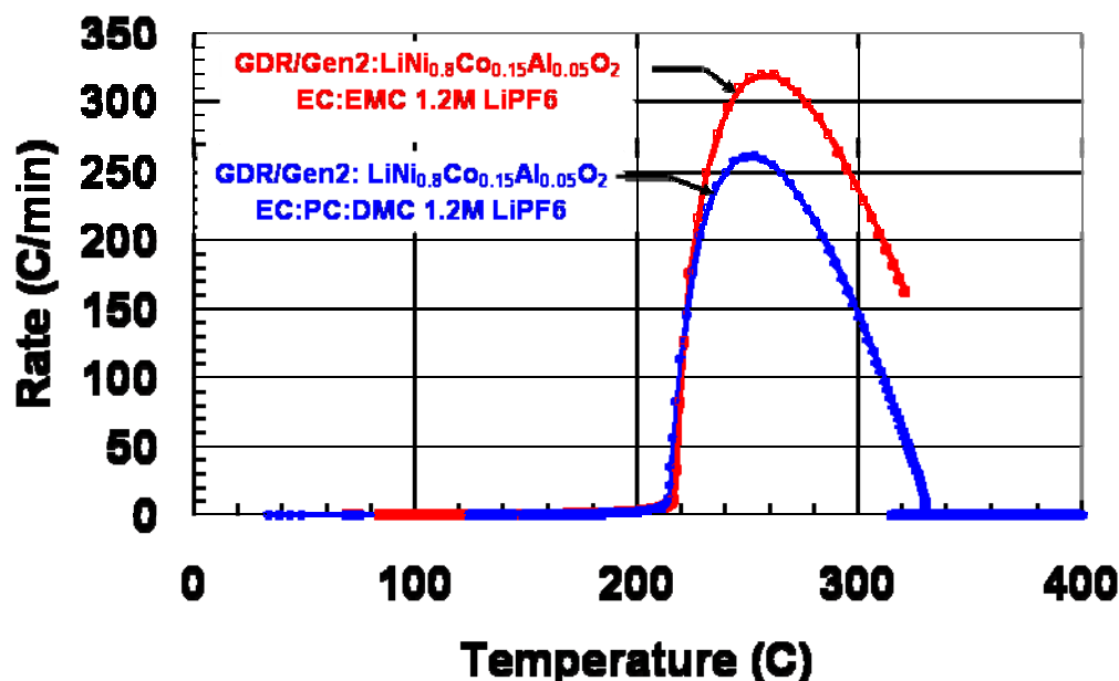
Figure III-36. ARC profile showing less effect of EC:PC:DMC with the more reactive Gen2 oxide cathode.
