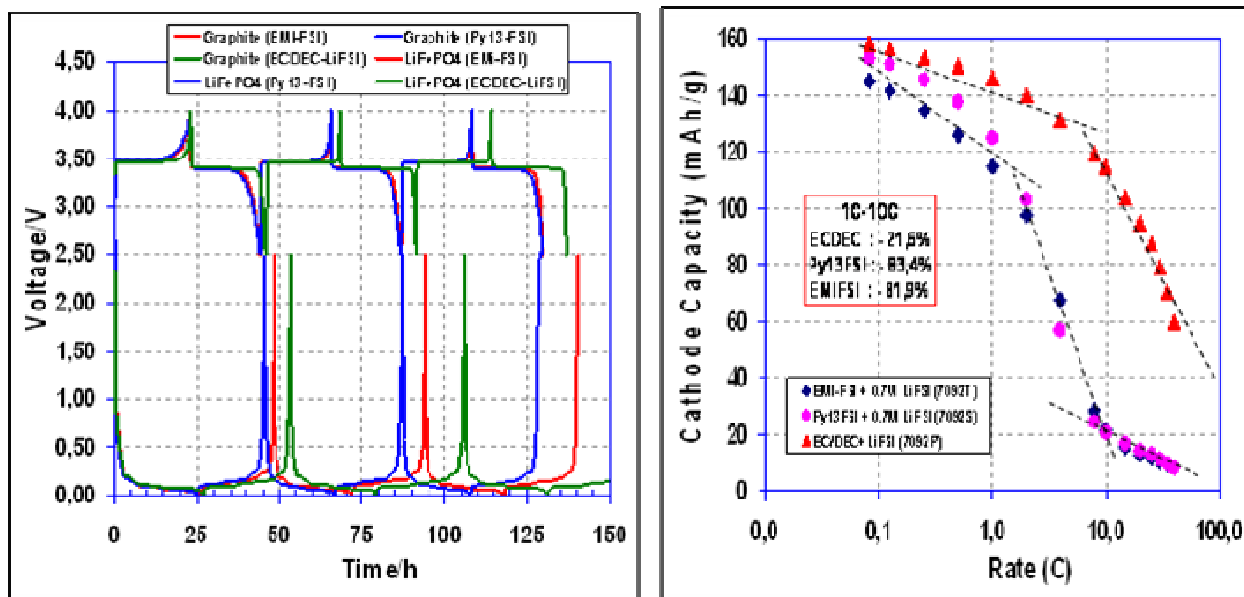
Figure IV-46. Left) Cycling of Li/LiFePO 4 and Li/graphite cells with different electrolytes at C/24, Right) Ragone plot of Li/LiFePO 4 cells with different electrolytes at 25°C.
