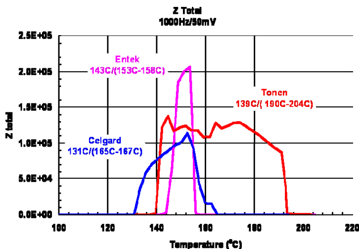
Figure III-31. Separator impedances over temperature range showing shutdown and loss of integrity (Celgard, Entek, and Tonen separators).
