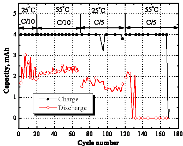
Figure III-39. Charge and discharge capacity of a graphite/Gen2 cell during an overcharge test. The electrolyte used contained 5 wt% PFPTFBB.
