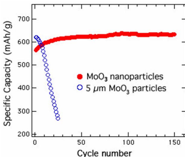
Figure IV-27. The cycling stability of the \alpha -phase \text{MoO}_3 nanoparticle negative electrode compared to commercially available \mu\text{m} -sized \text{MoO}_3 particles cycled at C/2 rate.
