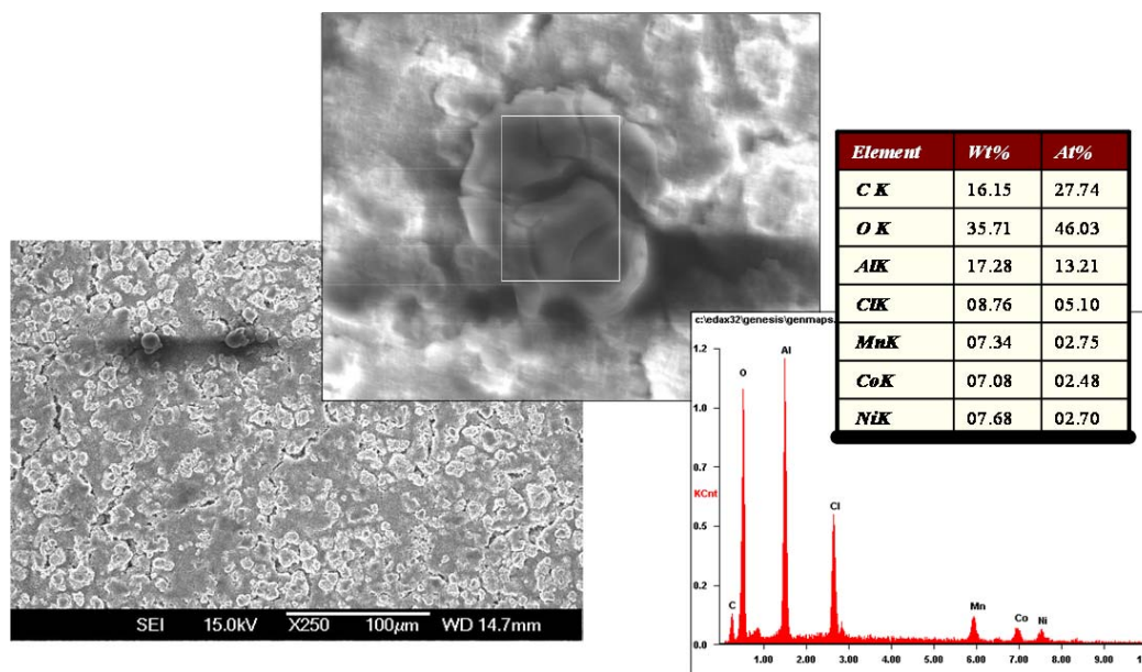
Figure III-12. SEM/EDX of Gen-3 cathode after 20 cycles.
