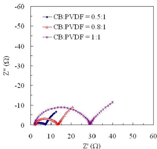
Figure IV-48. Nyquist plot of the ac impedance of films of different ratios of carbon black to polyvinylidene difluoride binder (CB:PVdF).
