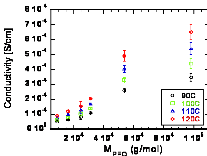
Figure IV-39. Ionic conductivity of SEO/LiTFSI mixtures with r = 0.02 versus MPEO, at selected temperatures.
