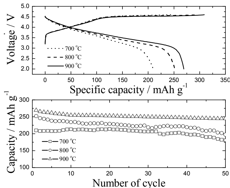
Figure – Stable high capacities achieved by optimizing processing conditions.
