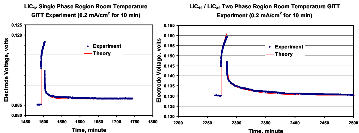
Figure III-25. Comparison of typical Gen3 negative electrode GITT experimental results for lithium diffusion in the graphitic active material single and two phase regions to electrochemical model simulations.
