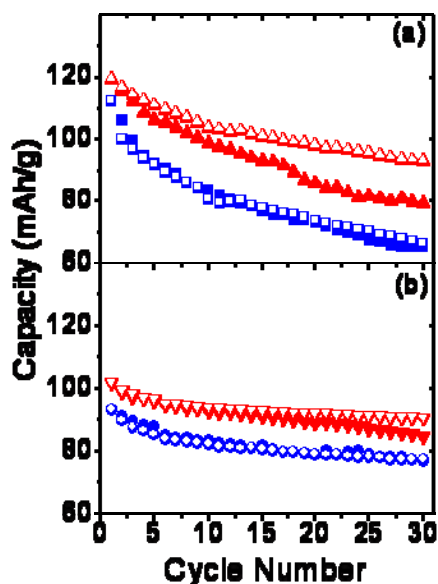
Figure IV-9. Cycling performance of Li-ion cells fabricated with graphite anode. (a) (■) \text{LiMn}_2\text{O}_4 between 3.5 and 4.3 V, (□) \text{LiMn}_2\text{O}_4 between 3.5 and 4.3 V after charging up to 4.7 V during first charge, (▲) 70 wt% \text{LiMn}_2\text{O}_4 + 30 wt% \text{LiCoO}_2 between 3.5 and 4.3 V, and (△) 70 wt% \text{LiMn}_2\text{O}_4 + 30 wt% \text{LiCoO}_2 between 3.5 and 4.3 V after charging up to 4.7 V during first charge, (b) (●) \text{LiMn}_{1.8}\text{Li}_{0.1}\text{Ni}_{0.1}\text{O}_{3.8}\text{F}_{0.2} between 3.5 and 4.3 V, (○) \text{LiMn}_{1.8}\text{Li}_{0.1}\text{Ni}_{0.1}\text{O}_{3.8}\text{F}_{0.2} between 3.5 and 4.3 V after charging up to 4.7 V during first charge, (▼) 70 wt% \text{LiMn}_{1.8}\text{Li}_{0.1}\text{Ni}_{0.1}\text{O}_{3.8}\text{F}_{0.2} + 30 wt% \text{LiCoO}_2 between 3.5 and 4.3 V, and (▽) 70 wt% \text{LiMn}_{1.8}\text{Li}_{0.1}\text{Ni}_{0.1}\text{O}_{3.8}\text{F}_{0.2} + 30 wt% \text{LiCoO}_2 between 3.5 and 4.3 V after charging up to 4.7 V during first charge. The first cycle discharge capacities are not included as they vary with first cycle charge voltage of 4.3 or 4.7 V.
