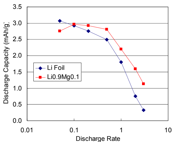
Figure IV-30. Discharge capacity vs. rate for \text{Li}_{1.1}\text{Mn}_{0.3}\text{Ni}_{0.3}\text{Co}_{0.3}\text{O}_2 cells with Li and \text{Li}_{0.9}\text{Mg}_{0.1} anodes.
