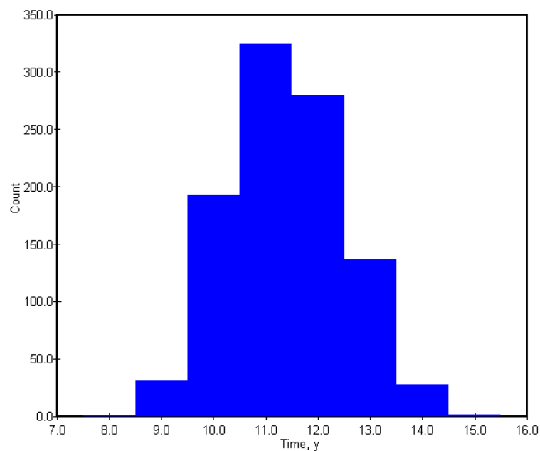
Figure III-17. Distribution of estimated average cell life obtained via the Monte Carlo simulations contained in the software package.
