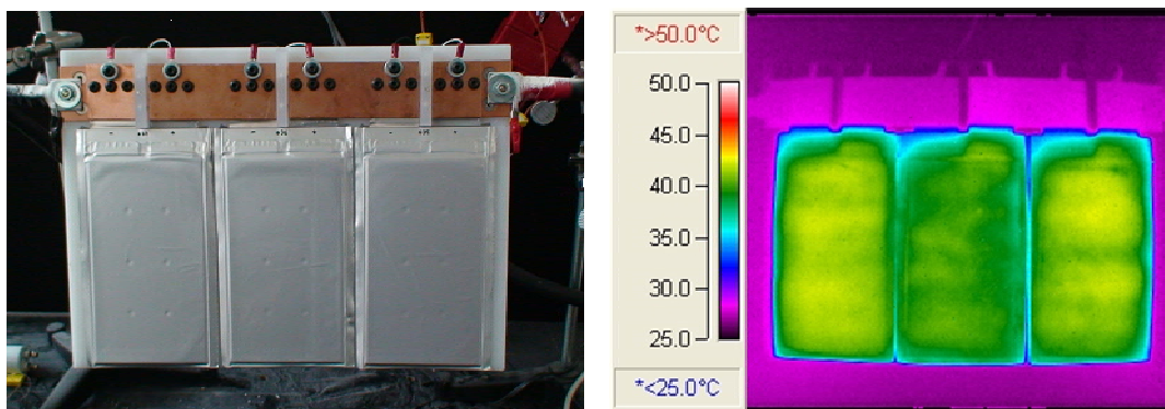
Figure II-3. Images of three CPI cells connected in series (left); Infrared thermal image of the cells at the end of 20C discharge, the thermal performance of the center cell is representative of most of cells in a module.
