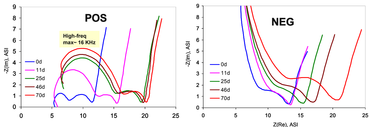
Figure III-8. Positive and negative electrode impedance data from a Gen3 cell that contained Gen2 + 3 wt% \text{LiF}_2\text{BC}_2\text{O}_4 electrolyte. The cell was aged at 4V and 55°C. The data were acquired at 3.72V, 30°C, and in the 100 kHz-10mHz frequency range. Note the increase in high-frequency arc width on aging for the positive electrode.
