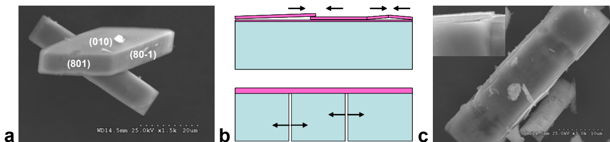
Figure IV-3. a) Fresh hydrothermal crystals measuring 15 \mu\text{m} x 10 \mu\text{m} x 40 \mu\text{m} ; b) brittle fracture modes for an expanding surface layer strongly bonded to a rigid substrate; c) brittle fracture in partially delithiated crystal.
