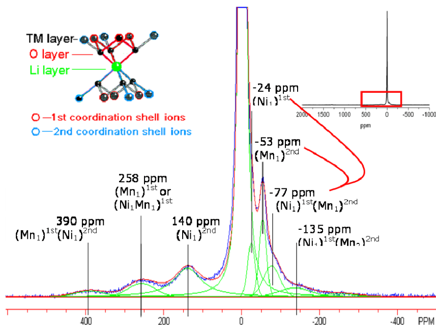
Figure IV-20. Enlargement of the ^6Li MAS NMR spectrum of Li[Ni_{0.02}Mn_{0.02}Co_{0.96}]O_2 (full spectrum shown in inset). Assignments of the resonances to different Li local environments, differing in the number of Ni and Mn ions in the 1st and 2nd cation coordination shell, are shown.
