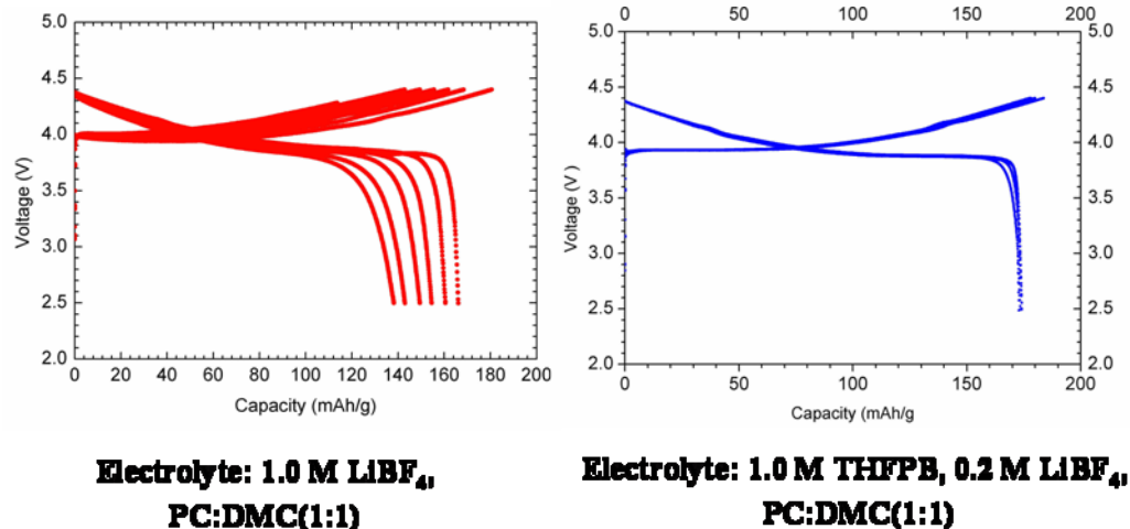
Figure IV-37. The cyclability of a Li/LiCoO 2 half cell using LiBF 4 based electrolytes without or with boron-based additive. The boron based additive used here is [(CF 3 ) 2 CHO] 3 B:THFPB.
