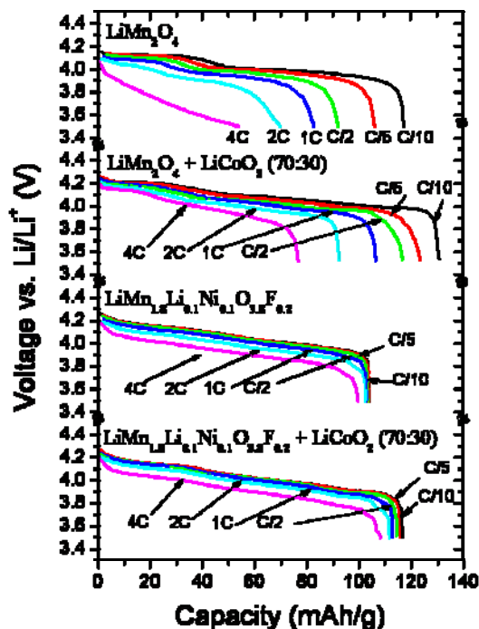
Figure IV-10. Comparison of the discharge profiles at various C rates of coin cells with metallic Li anode, illustrating the rate capabilities of \text{LiMn}_2\text{O}_4 , 70 wt% \text{LiMn}_2\text{O}_4 + 30 wt% \text{LiCoO}_2 , \text{LiMn}_{1.8}\text{Li}_{0.1}\text{Ni}_{0.1}\text{O}_{3.8}\text{F}_{0.2} , and 70 wt% \text{LiMn}_{1.8}\text{Li}_{0.1}\text{Ni}_{0.1}\text{O}_{3.8}\text{F}_{0.2} + 30 wt% \text{LiCoO}_2 .
