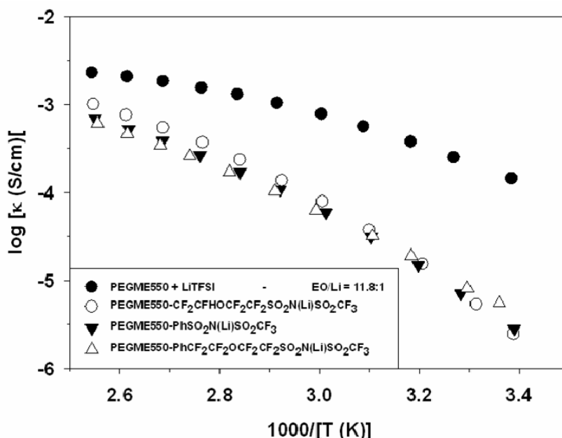
Figure IV-42. Arrhenius plots for 3 different PEGME550-based fluorosulfonimide ionic melts: a PFVE-based IL 550 (open circles), a phenyl-based (filled triangles) and an extended-phenyl-based (open triangles). Data for salt LiTFSI in PEGME550 solvent are included for comparison.
