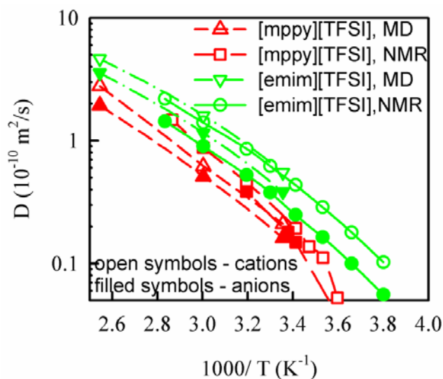
Figure IV-44. Comparison of the ion self-diffusion coefficients from MD simulations and previously published pgf-NMR experiments (J Phys Chem B 2005, 109, 22814; J Phys Chem B 2001, 105, 4603).
