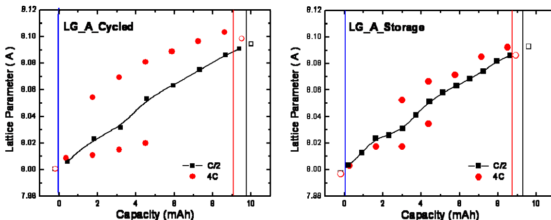
Figure III-20. Lattice parameters calculated from the Time resolved XRD data.
