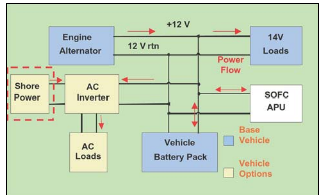
Figure 1. Vehicle Electrical System Diagram
