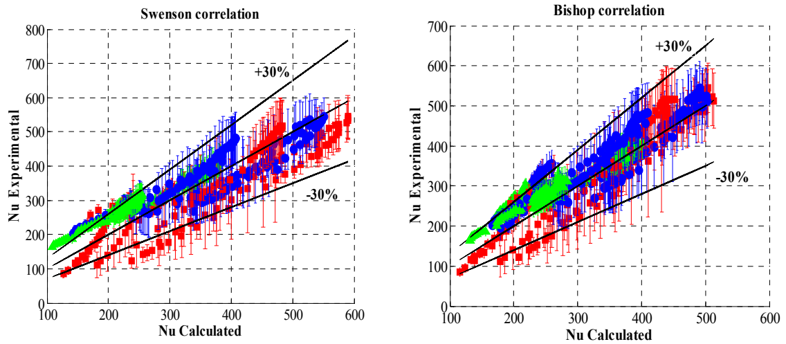
Figure 116. Calculated Nusselt number for downward flow
