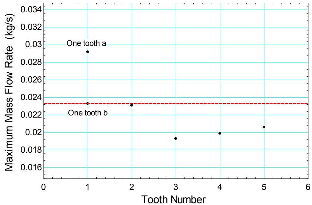
Figure 35. Variation in tooth number for the same total length. One Tooth a: short length, depicts maximum flow rate. One Tooth b: Tooth occupies entire length and depicts the flow rate approached as tooth number is further increased [7].
