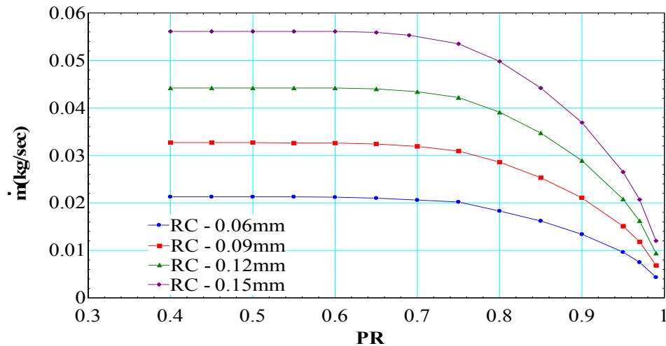
Figure 58. Variation of Leakage rate with Radial clearance
