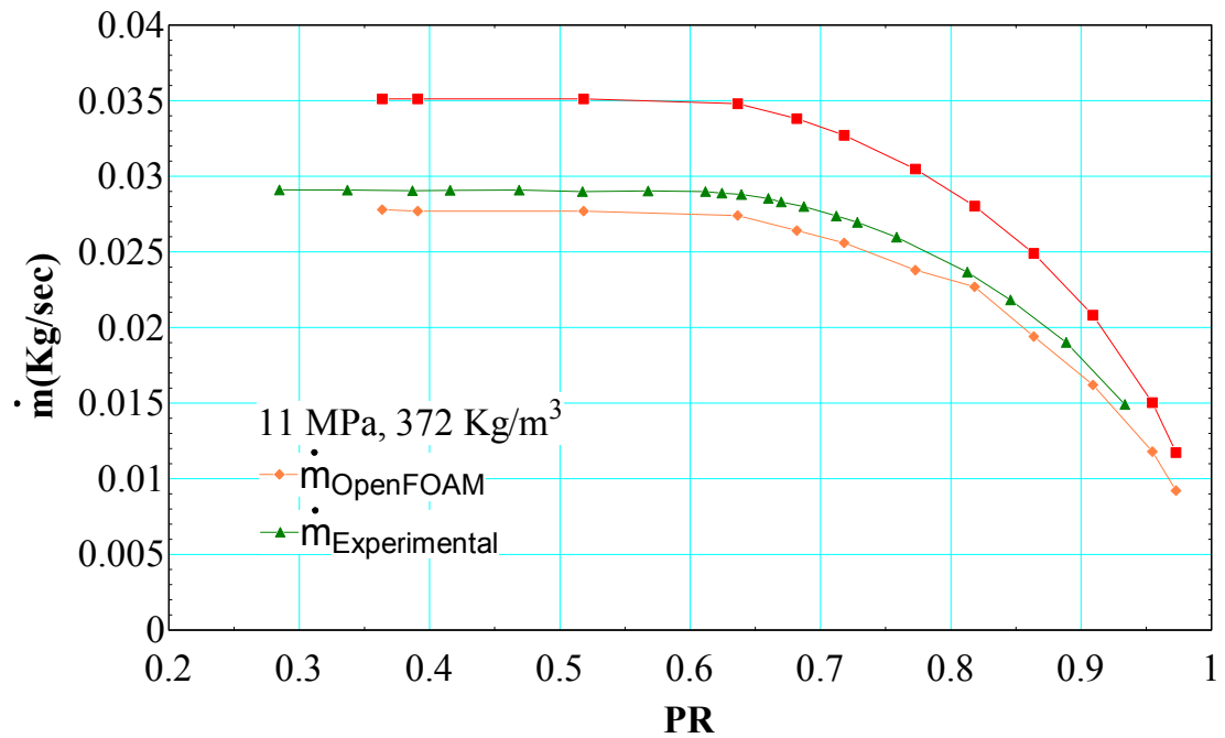
Figure 55. Leakage rate for inlet condition of 11 MPa, 372 Kg/m 3 (case 5 in Table D.3)
