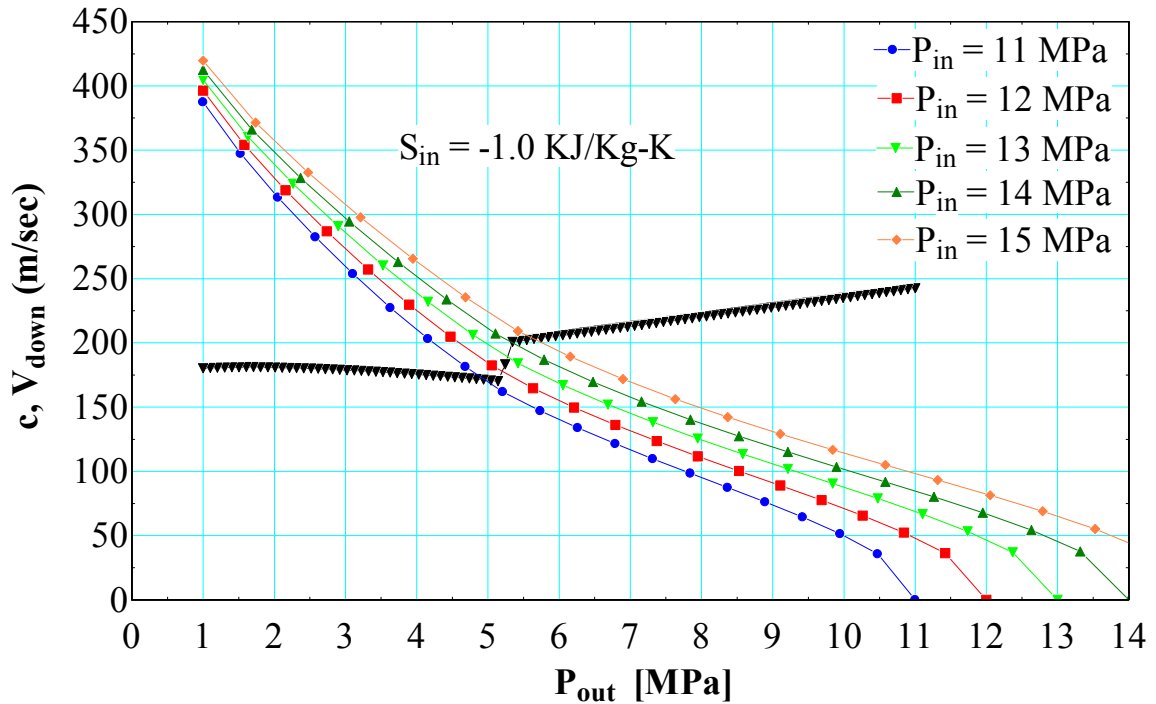
Figure 106. Downstream velocity of labyrinth seal and local sound speed as a function of outlet pressure
