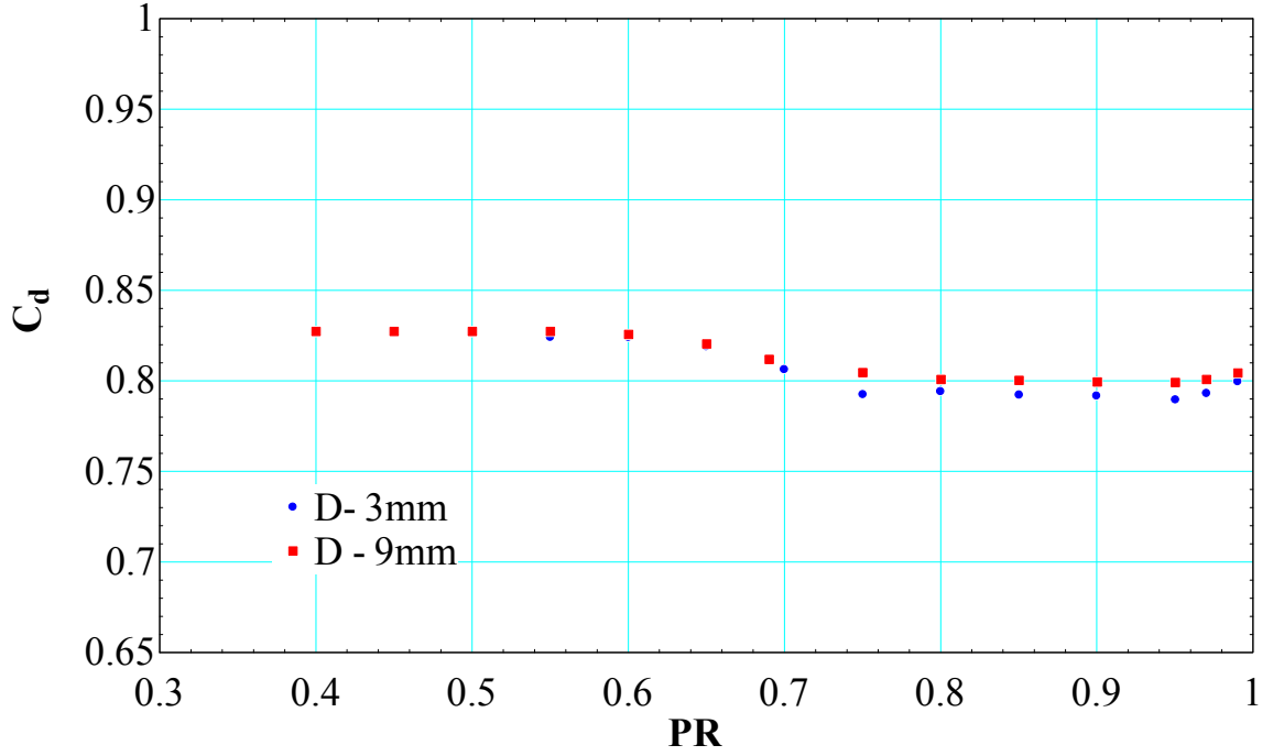
Figure 65. Variation of C_d with shaft diameter
