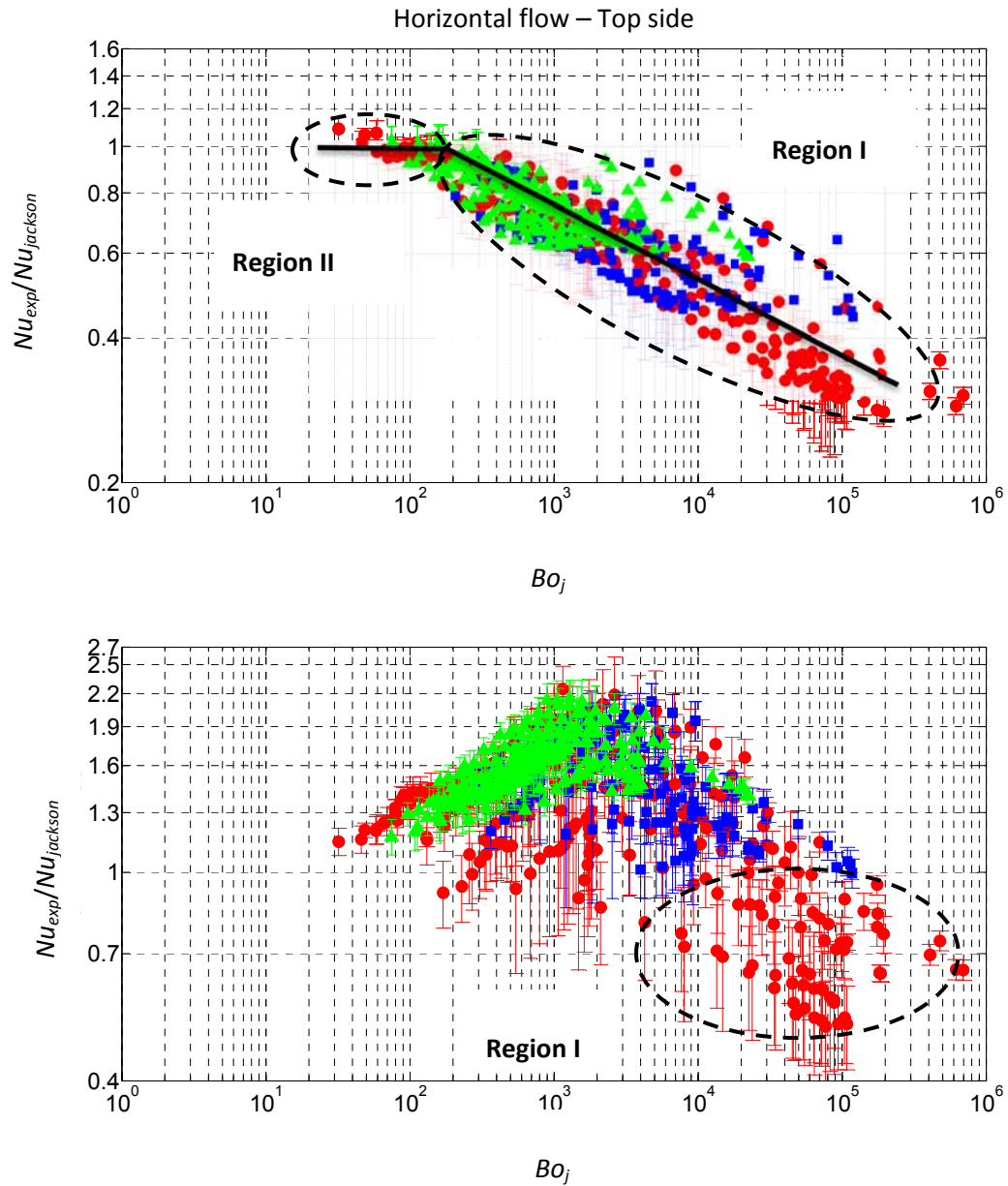
Figure 114. Normalized Nusselt number versus Jackson's buoyancy parameter, Bo_j
