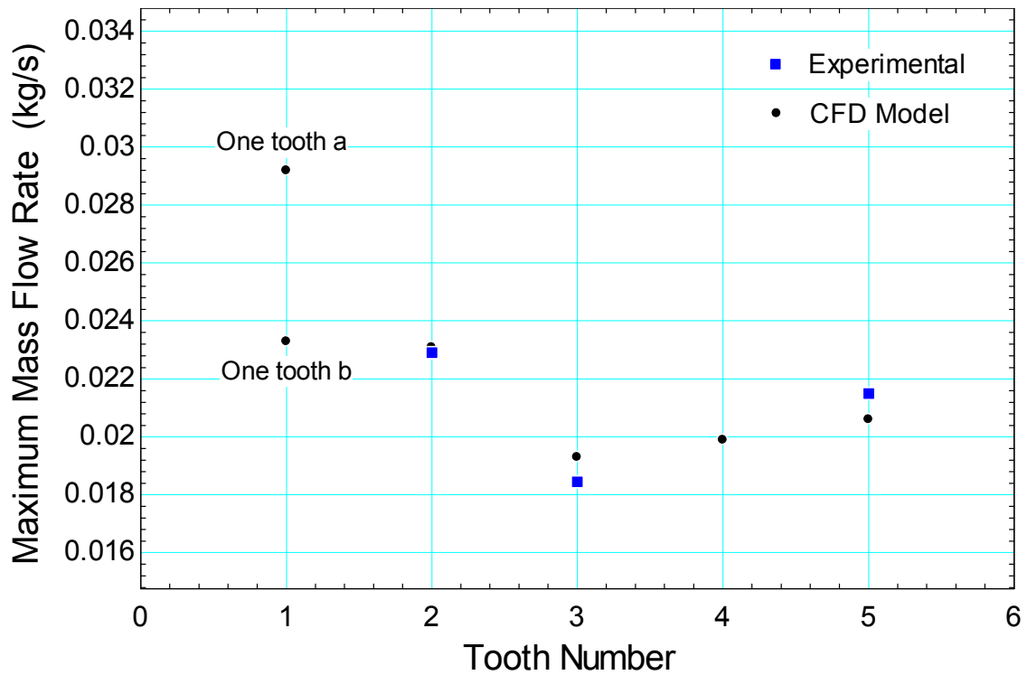
Figure 38. Comparison of measured flow rate to CFD calculated flow rate for varying tooth number with same total length.
