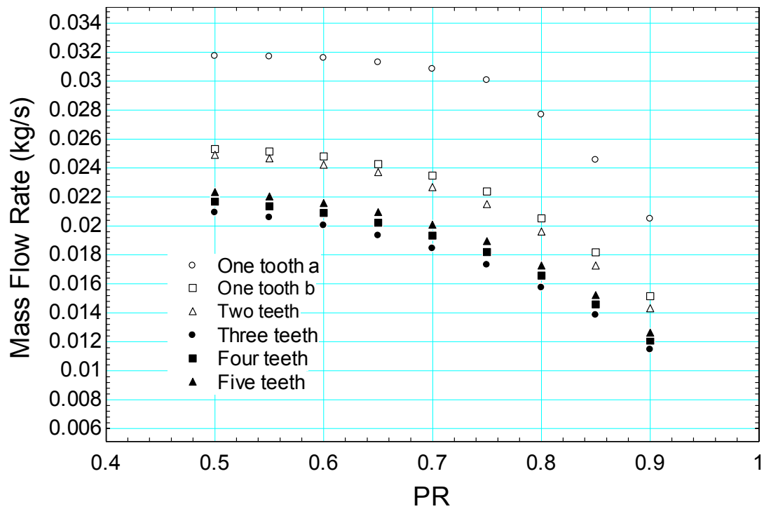
Figure 36. Variation in tooth number for the same total length. Variation in pressure ratio shows an optimal tooth number of three [7].
