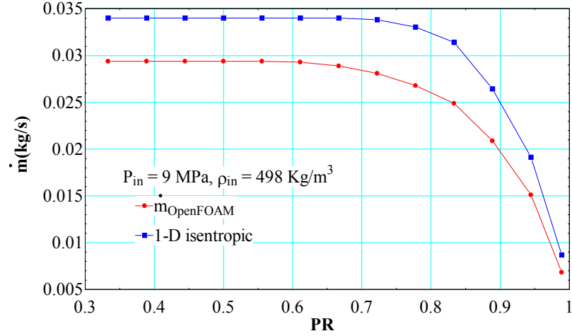
Figure 86. Leakage rate for inlet condition of 9 MPa and 498 Kg/m 3
