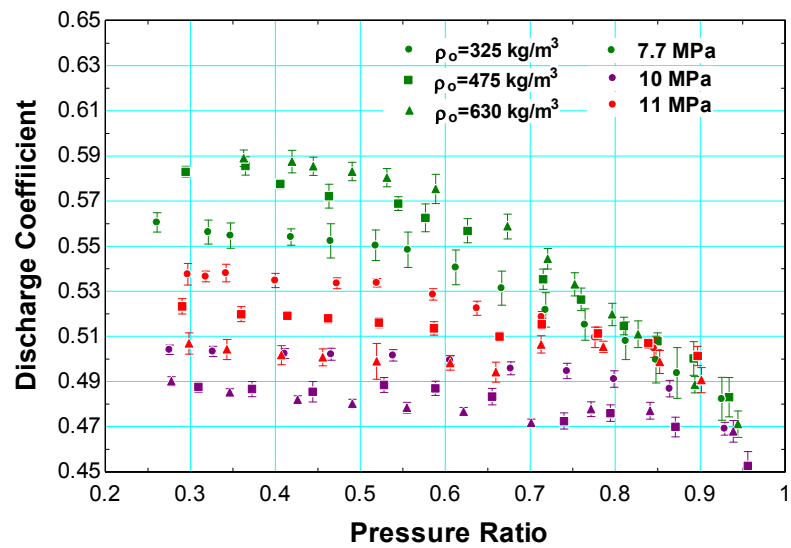
Figure 33. Discharge coefficient results for three-tooth straight through labyrinth seal at varying inlet conditions.
