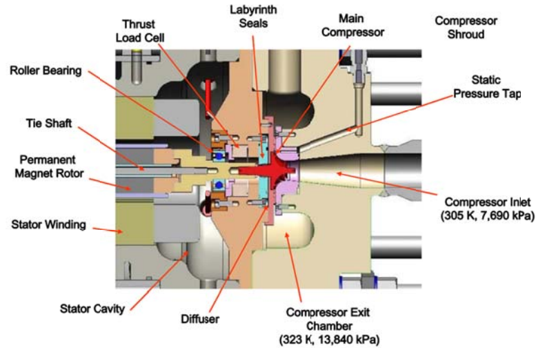
Figure 5. Detail of SNL main compressor, labyrinth seals, ball bearings, and location of other major components [2].
