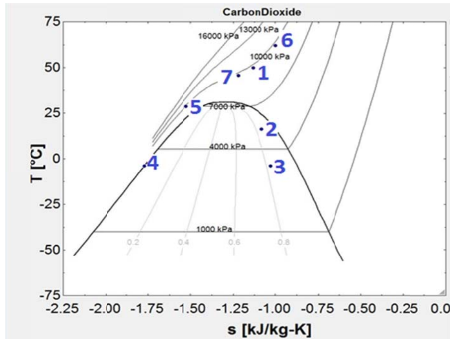
Figure 13. Conditions for various locations on the loop (Figure 8), shown on a temperature-specific entropy diagram during typical experiment conditions.
