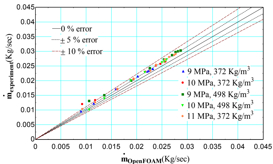
Figure 56. Error analysis for plain orifice data
