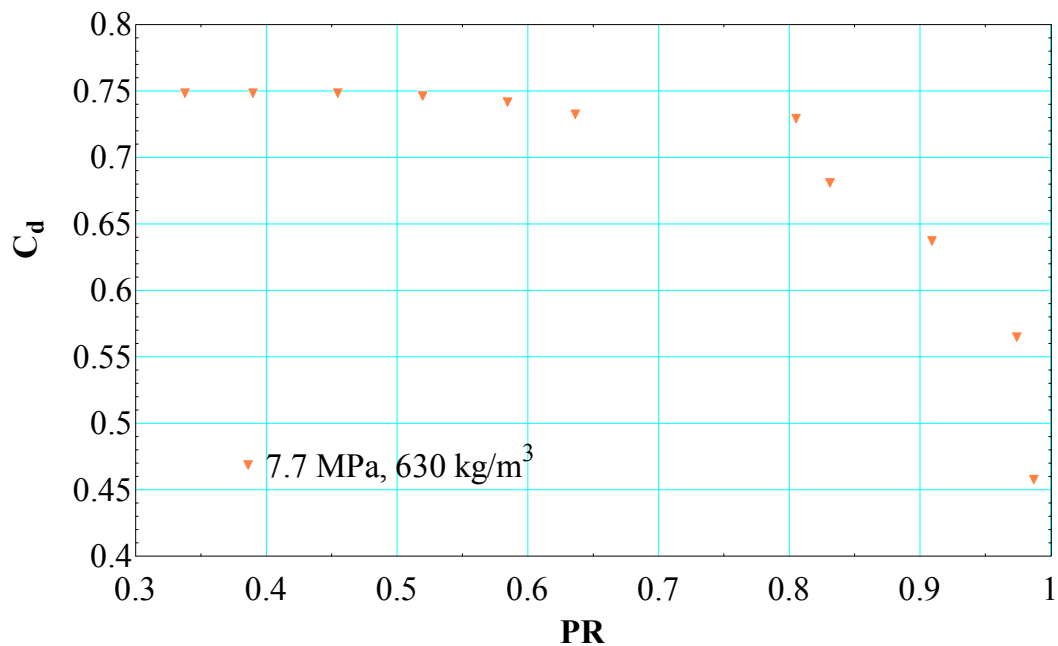
Figure 104. C_d for an inlet pressure of 7.7 MPa
