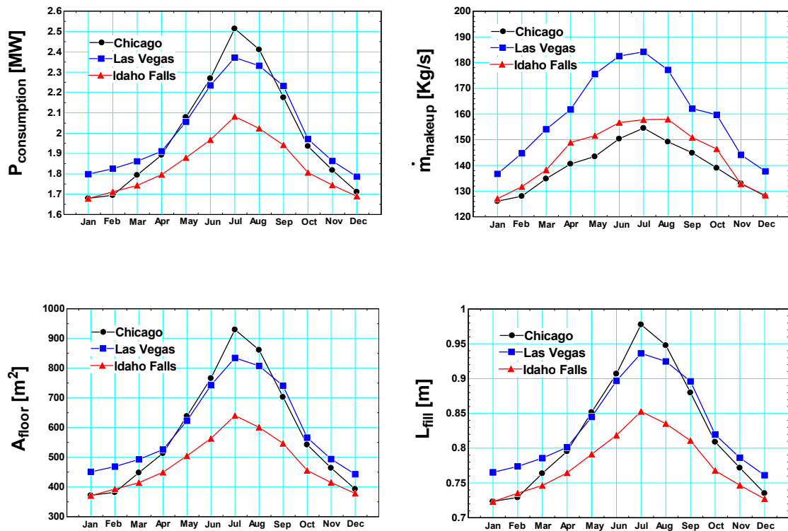
Figure 127. Variation of requirements for AFR-100 at optimum \dot{m}_w/\dot{m}_a conditions
