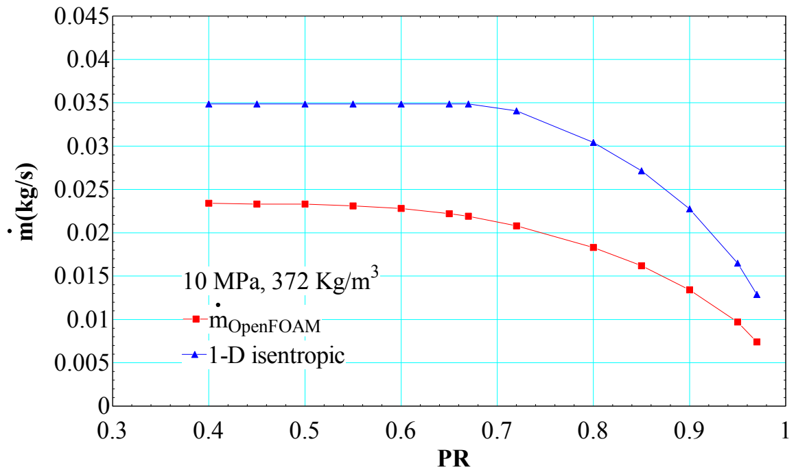
Figure 100. Leakage rate for inlet condition of 10 MPa and 372 Kg/m 3
