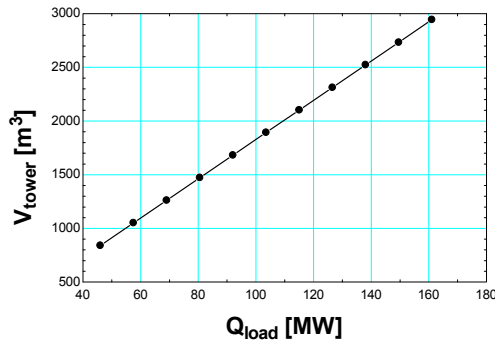
Figure 123. Effect of heat load
