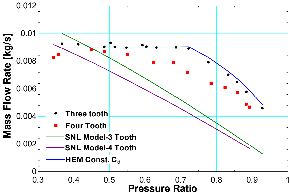
Figure 46. Mass flow rate experimental measurements and calculations for three and four tooth stepped labyrinth seal including the SNL Martin leakage equation and the HEM model with constant discharge coefficient.
