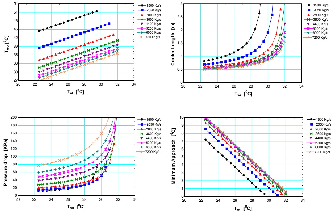
Figure 129. Effect of water conditions on the cooler variables
