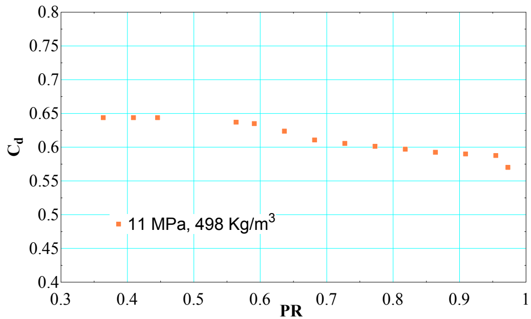
Figure 103. C_d for an inlet pressure of 11 MPa
