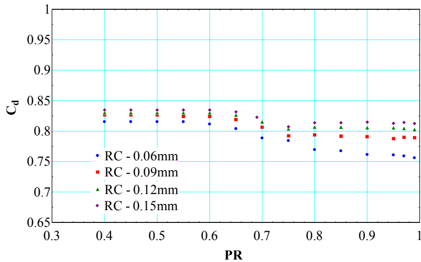
Figure 59. Variation of discharge coefficient with radial clearance
