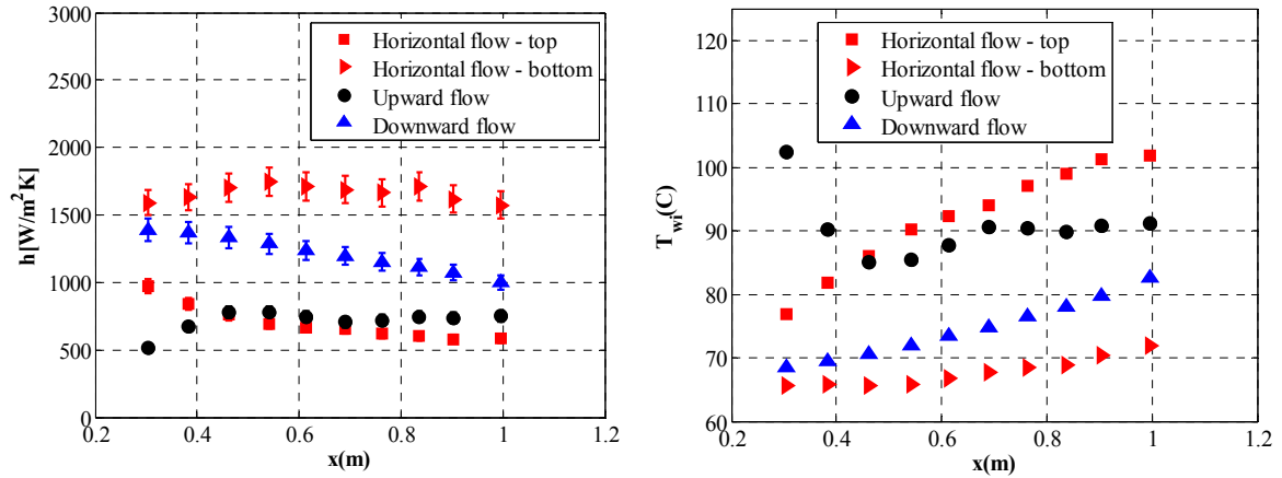
Figure 110. Effect of flow configuration on heat transfer for p = 8.1 MPa, G = 195 kg/m 2 s, Q''_{PS} = 24 kW/m 2 , T_{in} = 46^\circ\text{C}
