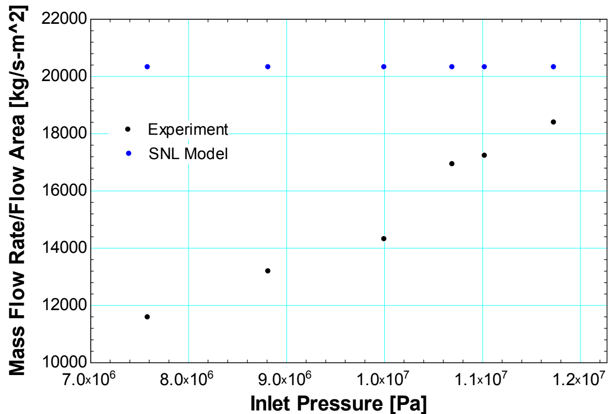
Figure 44. Area normalized leakage for four-tooth stepped labyrinth seal compared to calculated flow rate from SNL compressor facility.
