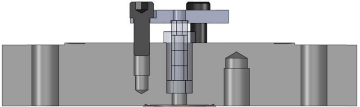
Figure 15. Cross Section of test section flange showing seal configuration.
