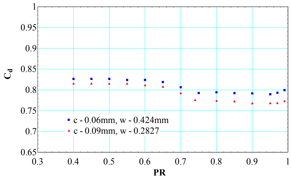
Figure 62. C_d of annular orifices having same w/c
