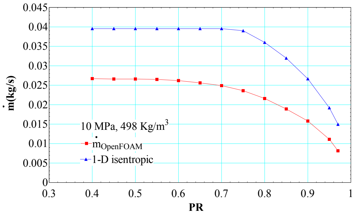
Figure 101. Leakage rate for inlet condition of 10 MPa and 498 Kg/m 3
