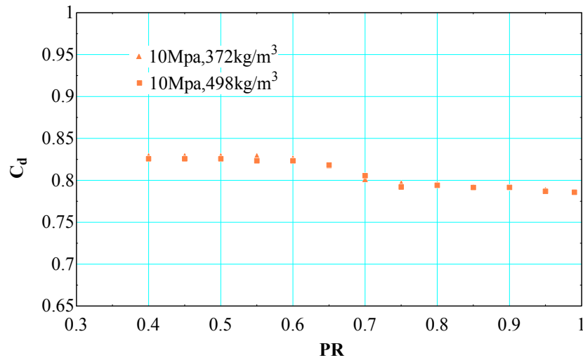
Figure 90. C_d for case 3 in Table D.1 and case 2 in Appendix B
