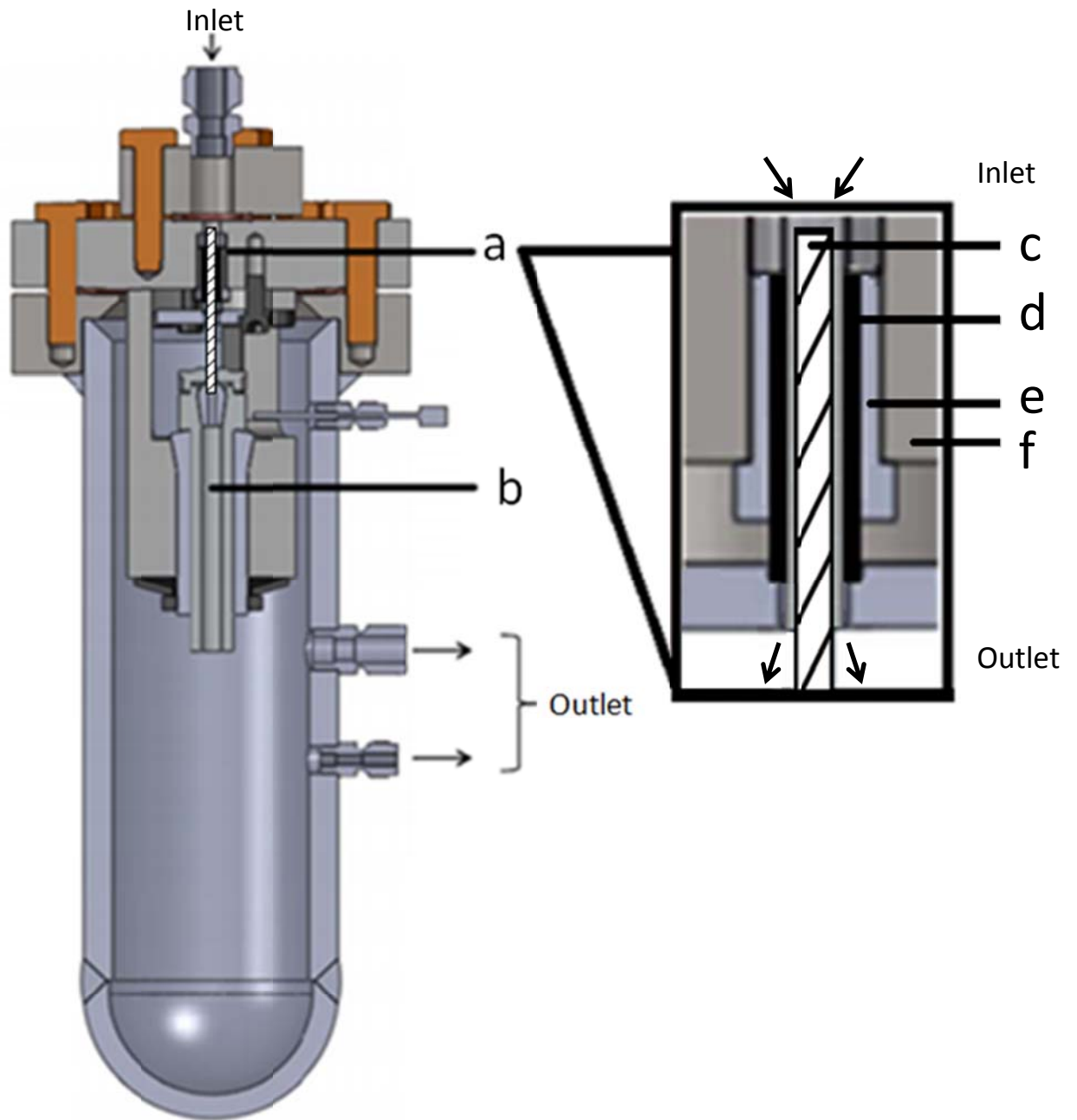
Figure 14. Cross Section of pressure vessel showing a) seal location/configuration, b) collet sub-assembly, c) shaft, d) seal, e) spacer drill bushing, f) test section flange.
