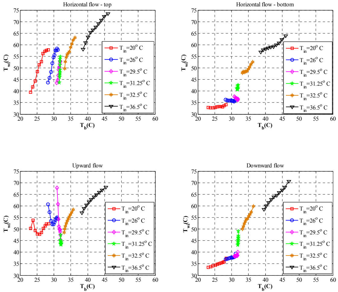
Figure 111. Effect of inlet temperature on the wall temperatures for p = 7.5 \text{ MPa} , G = 320 \text{ kg/m}^2\text{s} , Q''_{ps} = 24 \text{ kW/m}^2
