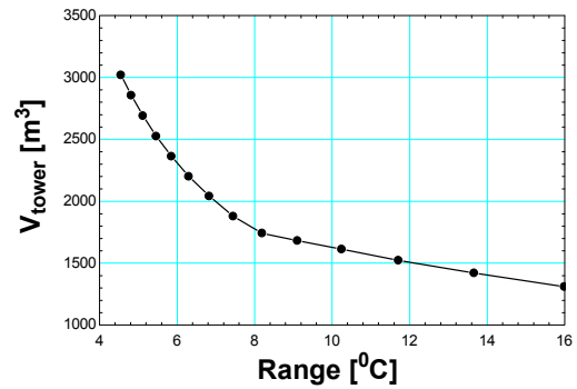
Figure 124. Effect of range
