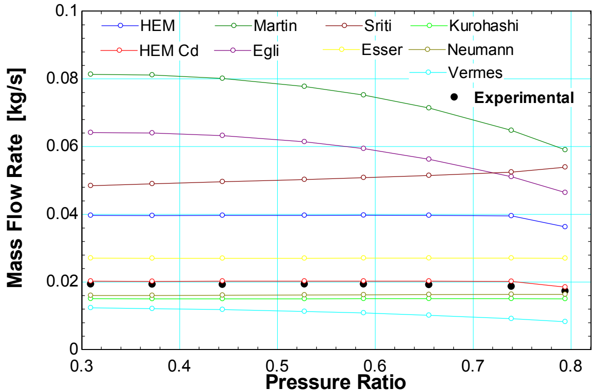
Figure 39. Measure flow rates through straight through 3-tooth labyrinth seal for inlet pressure of 10 MPa and inlet density of 325 \text{ kg/m}^3 compared to various labyrinth seal leakage models.
