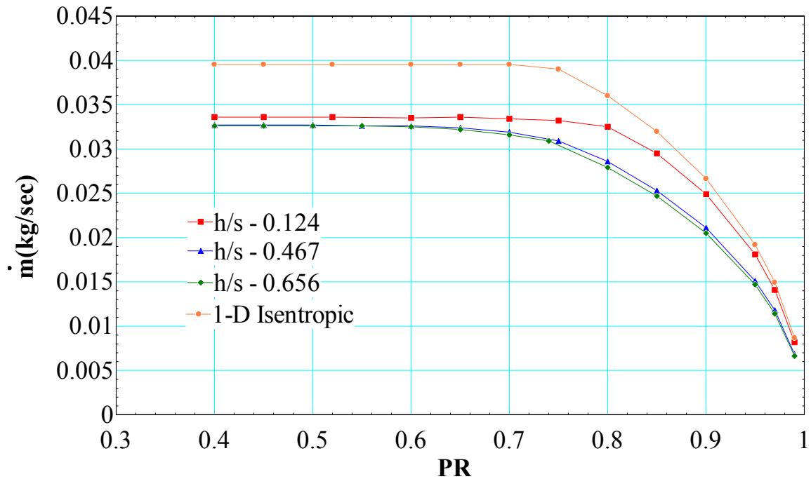
Figure 63. Variation of leakage rate with tooth height
