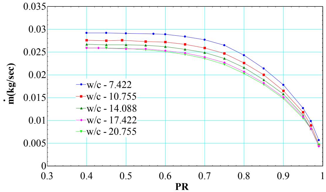
Figure 70. Effect of cavity width on leakage rate
