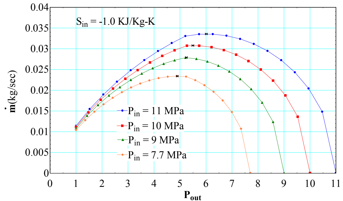
Figure 80. Isentropic flow behavior for S_{in} = -1.0 KJ/Kg-K
