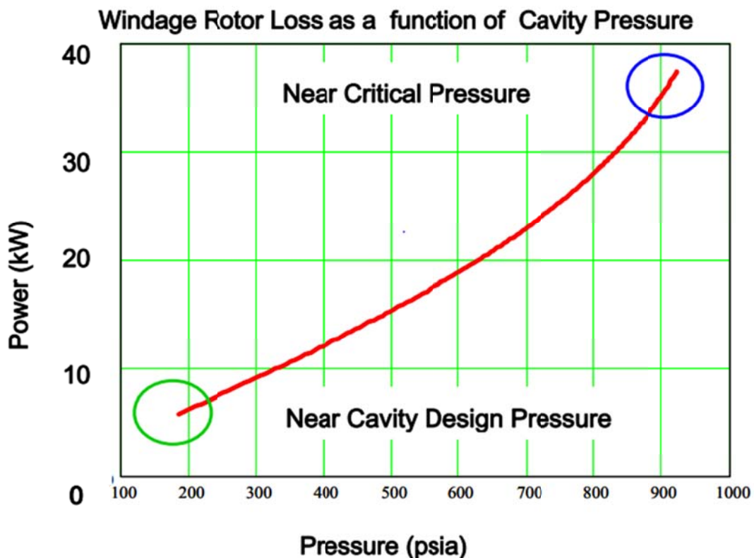
Figure 2. Calculated windage loss for the S-CO 2 SNL turbo-alternator-compressor as a function of rotor cavity pressure [2].
