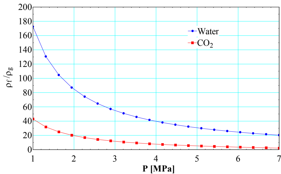
Figure 27. Density ratios for two phase CO 2 and water
