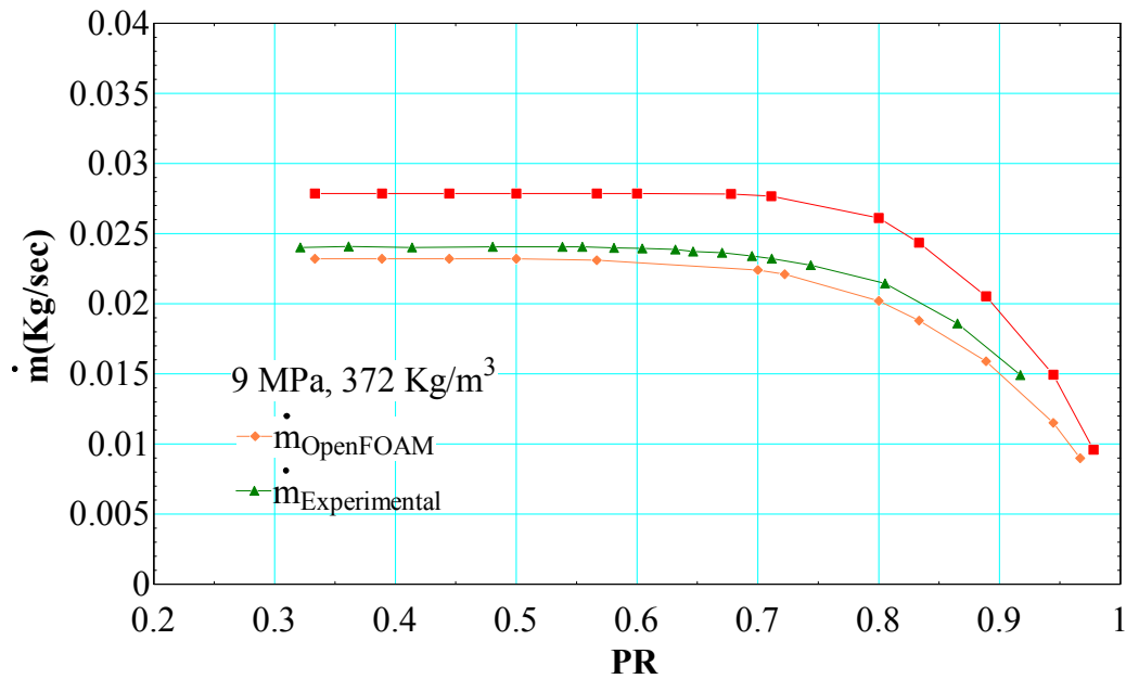
Figure 51. Leakage rate for inlet condition of 9 MPa, 372 Kg/m 3 (case 1 in Table D.3)
