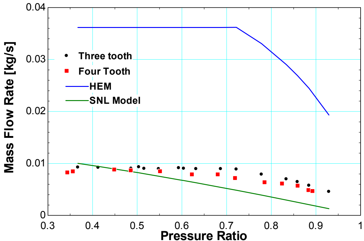
Figure 45. Three-tooth and four-tooth stepped labyrinth seal flow rate measurement for inlet pressure of 10 MPa and inlet density of 640 \text{ kg/m}^3 .
