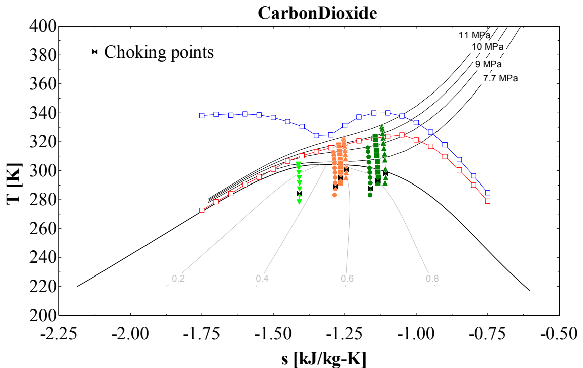
Figure 95. Choking point calculations for annular orifice (Flow curve).
