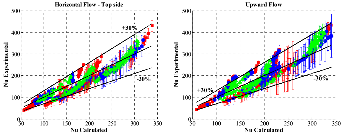
Figure 115. Calculated Nusselt number using Mokry et al. correlation
