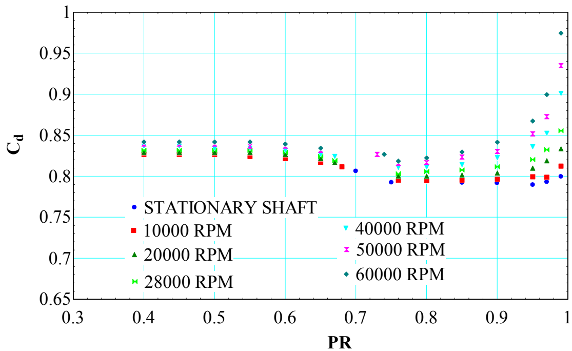
Figure 73. Influence of shaft rotation on C_d of annular orifices
