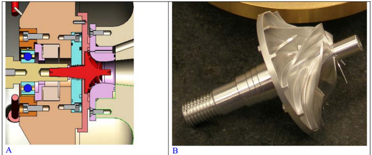
Figure 6. Sandia National Laboratory engineering diagram of labyrinth seal (A). The seal is made of brass and has four teeth that approach the steps on the rotating shaft. The compressor wheel (B) shows the four steps on the shaft [2].
