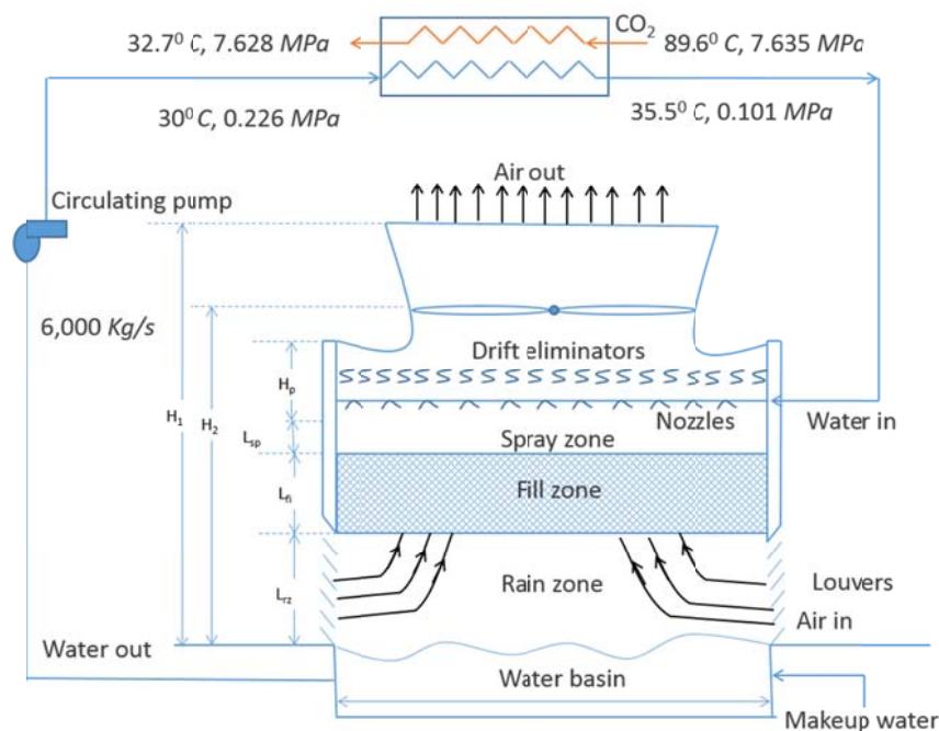
Figure 117. Proposed schematic of the cooler and induced draft cooling tower
