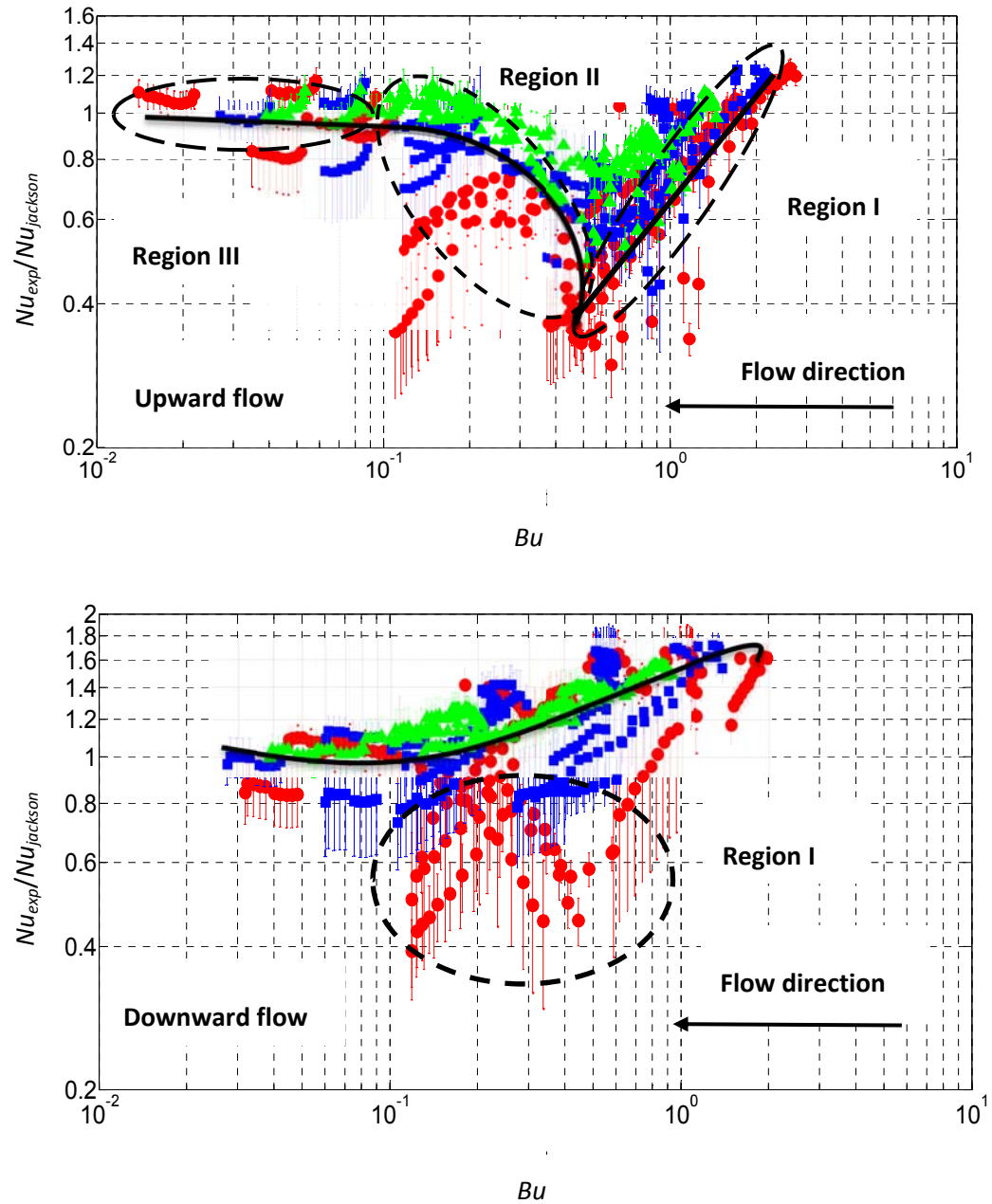
Figure 113. Normalized Nusselt number versus Jackson's buoyancy parameter, Bu
