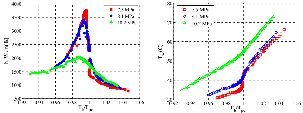
Figure 109. Effect of operating pressure on heat transfer for downward flow, G = 195 \text{ kg/m}^2\text{s} , Q''_{PS} = 13.5 \text{ kW/m}^2
