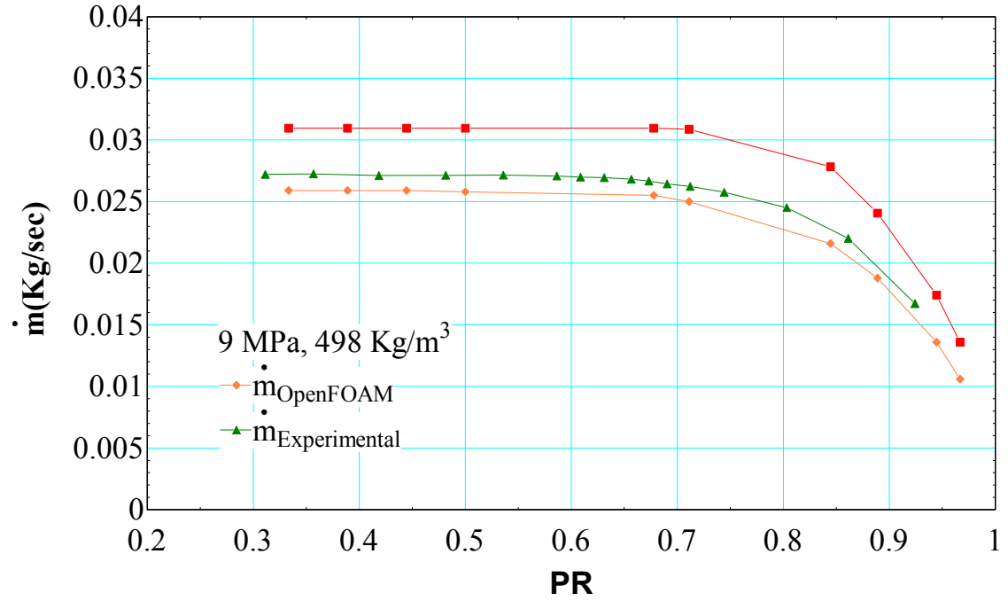
Figure 52. Leakage rate for inlet condition of 9 MPa, 498 Kg/m 3 (case 2 in Table D.3)
