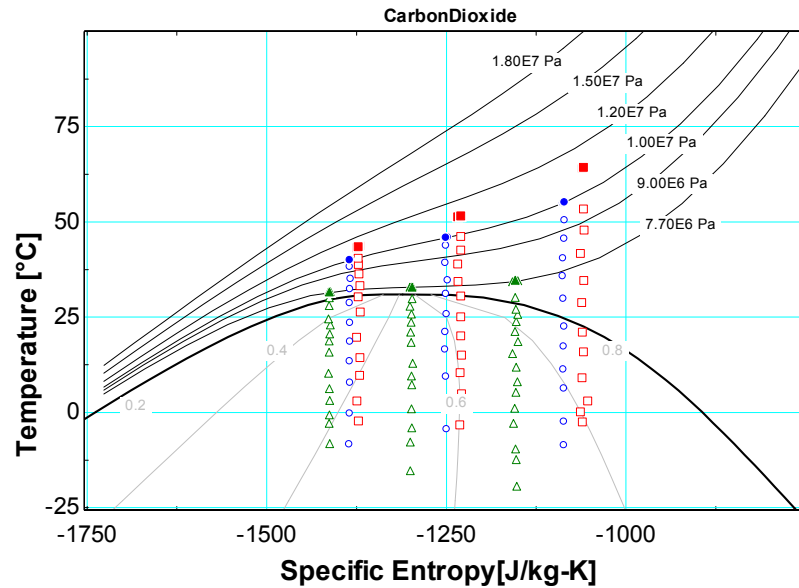
Figure 32. Temperature-specific entropy diagram for a 3 tooth straight-through labyrinth showing inlet conditions (filled markers) and outlet conditions (hollow markers) assuming isentropic expansion.
