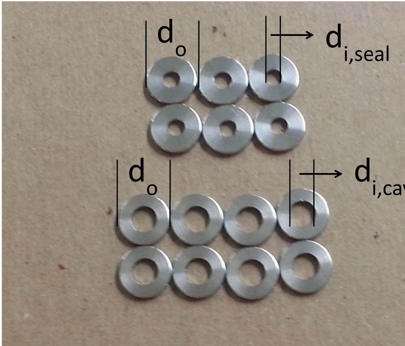
Figure 16. Seals and cavities used in the straight-through labyrinth tests, d_o=9.525 mm, d_{i,seal}=3.175 mm, d_{i,cavity}=4.763 mm and length = 1.27 mm.
