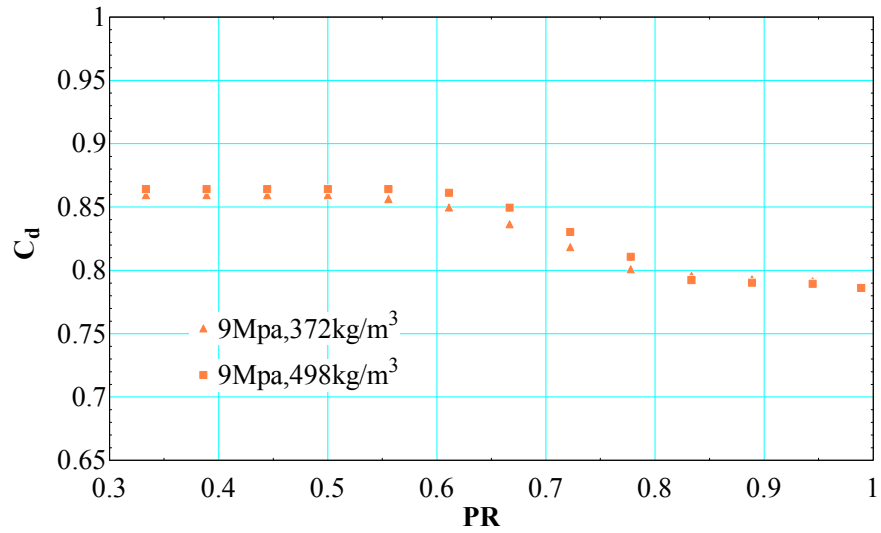
Figure 87. C_d for cases 4 and 5 in Table D.1 of Appendix D
