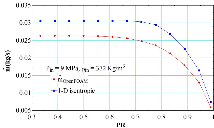
Figure 85. Leakage rate for inlet condition of 9 MPa and 372 \text{ Kg/m}^3
