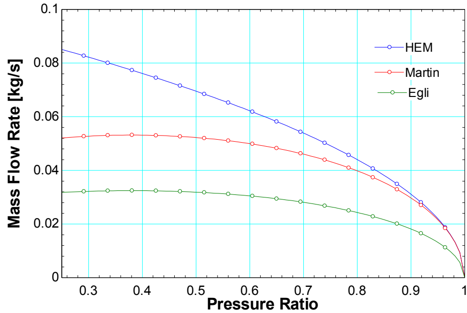
Figure 40. Incompressible and ideal gas condition check for Martin and Egli model over prediction. Inlet pressure of 6.8 MPa with corresponding inlet temperature of 200°C.
