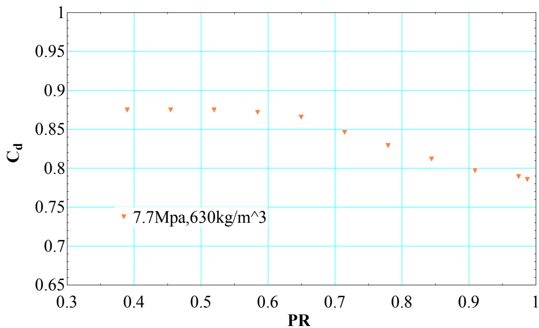
Figure 93. C_d for cases 1 and 2 in Table D.1 of Appendix D
