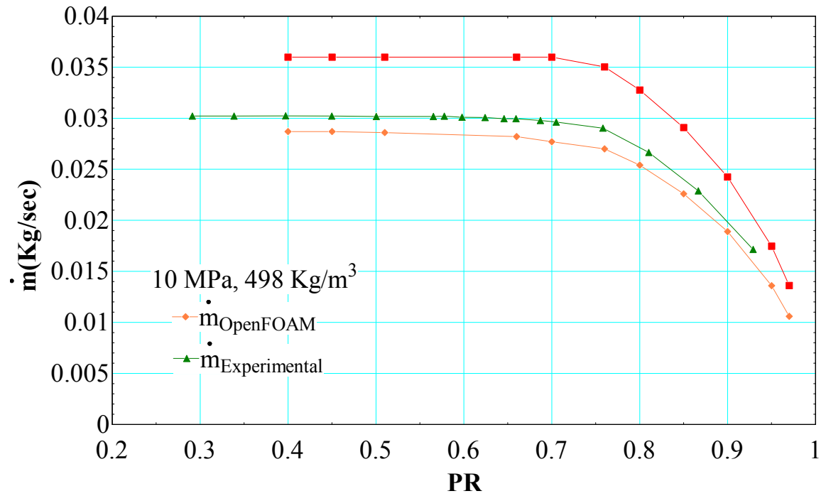
Figure 54. Leakage rate for inlet condition of 10 MPa, 498 Kg/m 3 (case 4 in Table D.3)
