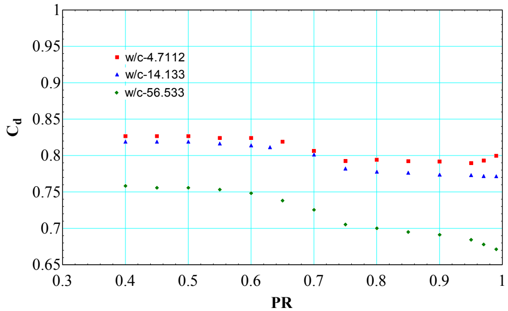
Figure 61. Variation of C_d with tooth width
