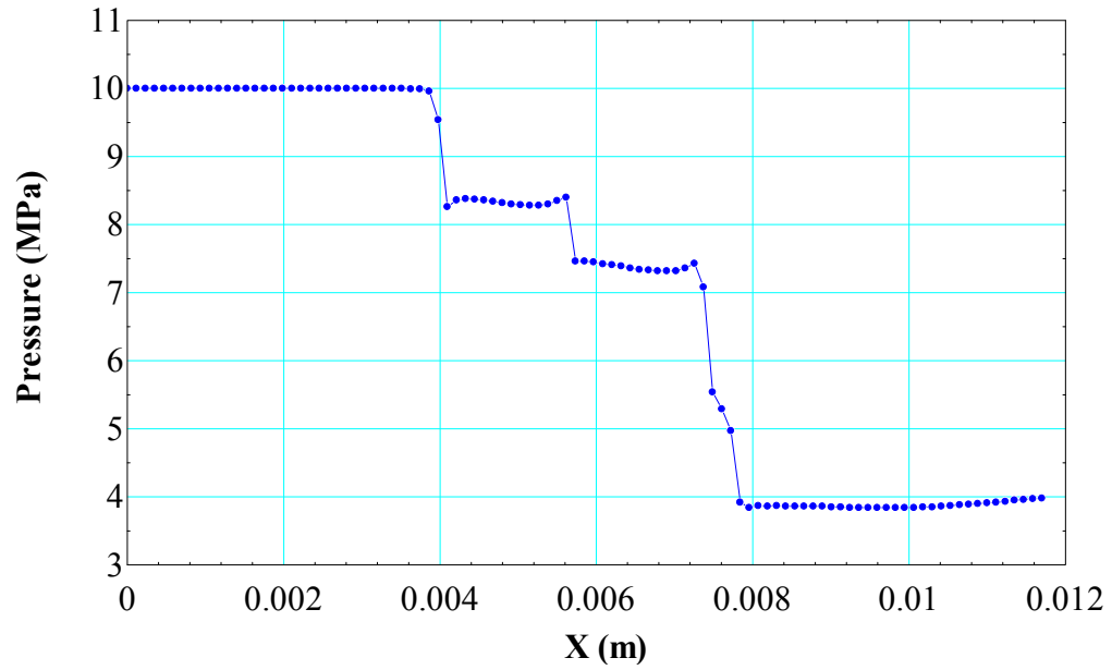
Figure 76. Pressure variation along centerline in the radial clearance region
