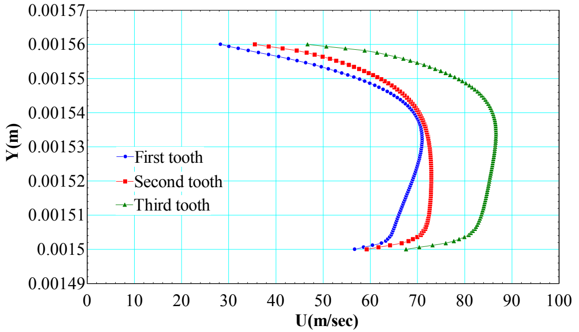
Figure 72. Velocity profile at the entrance of each tooth
