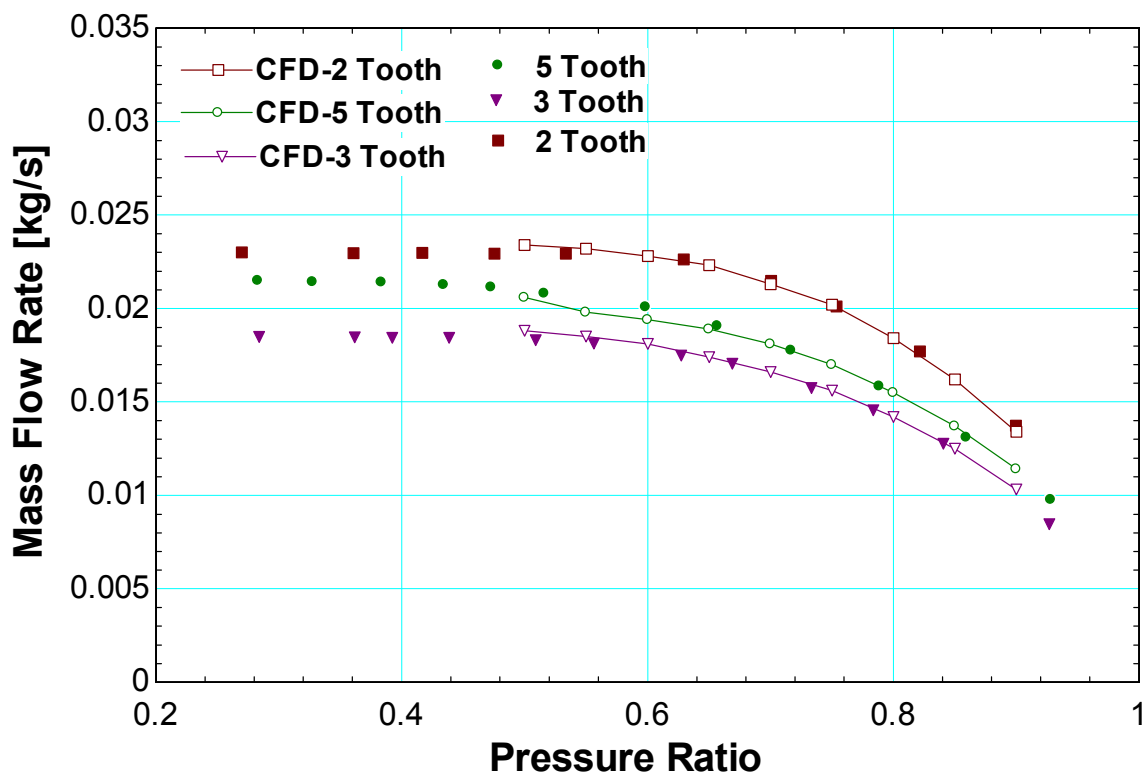
Figure 37. Measured flow rate for variation in tooth number for the same total length compared to calculated flow rate using Open Foam simulation [7]. Minimum leakage is found at a tooth number of three. Inlet Pressure is 10 MPa with corresponding inlet density of 325 \text{ kg/m}^3 .
