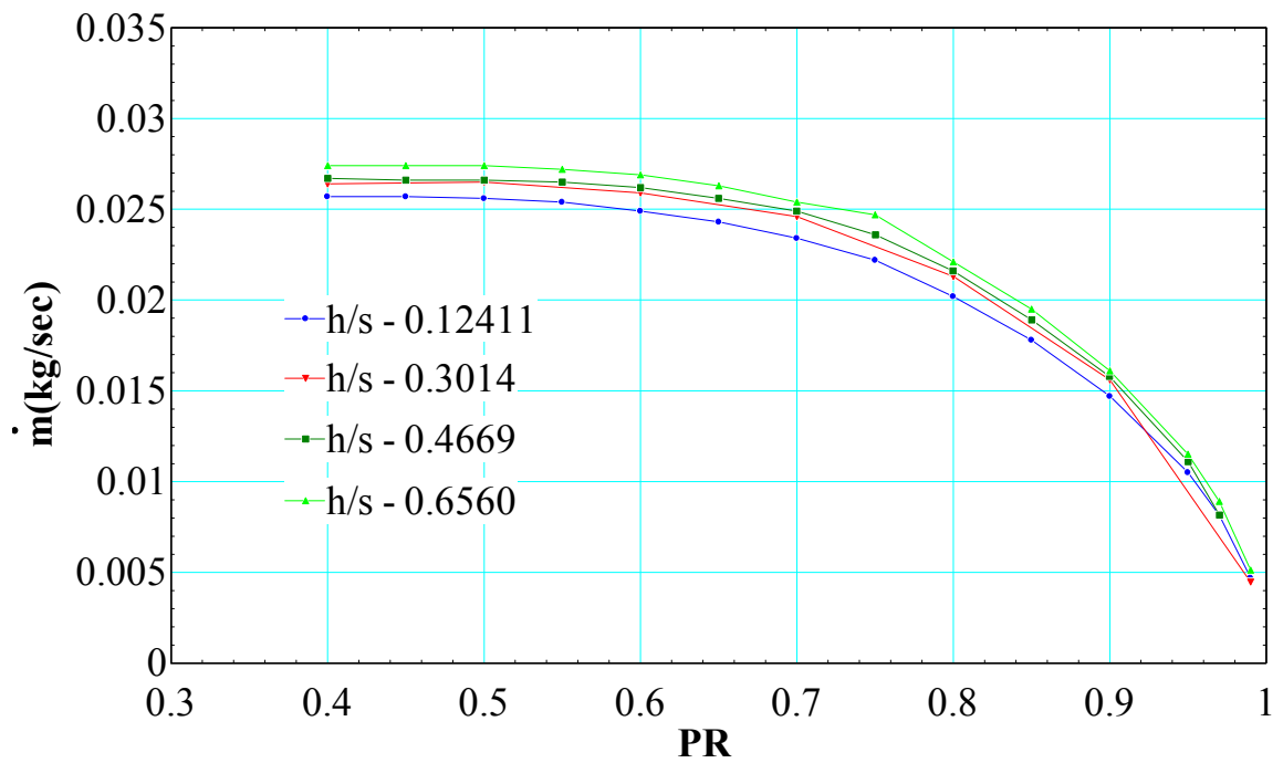
Figure 69. Effect of cavity height on leakage rate
