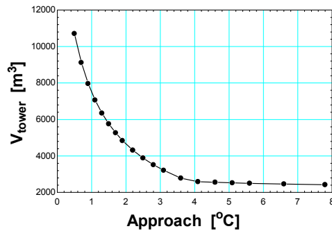
Figure 125. Effect of approach
