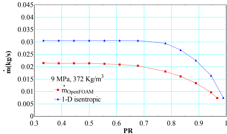
Figure 96. Leakage rate for inlet condition of 9 MPa and 372 Kg/m 3
