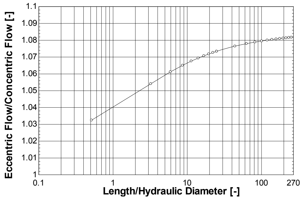
Figure 30. Duct flow approximation results for D_H=0.1956 mm.
