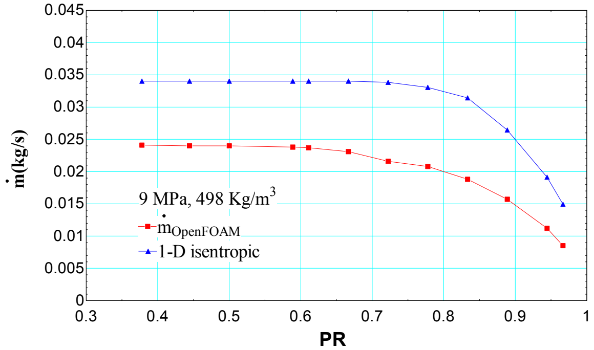
Figure 97. Leakage rate for inlet condition of 9 MPa and 498 Kg/m 3
