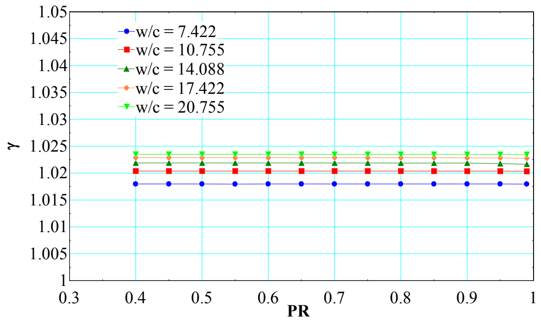
Figure 71. Variation of \gamma with cavity width
