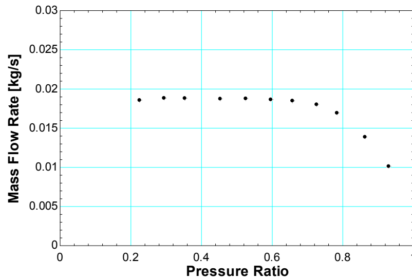
Figure 25. Measured mass flow rate of CO 2 through three tooth labyrinth seal as a function of pressure ratio for an upstream stagnation pressure of 10 MPa and an upstream stagnation density of 475 kg/m 3 .
