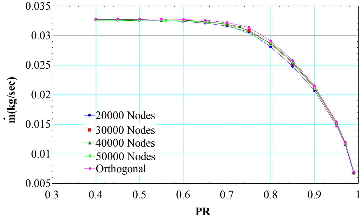
Figure 59. Variation of leakage rate prediction with number of nodes
