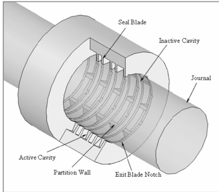
Figure 3. Conventional pocket damper seal [10].
