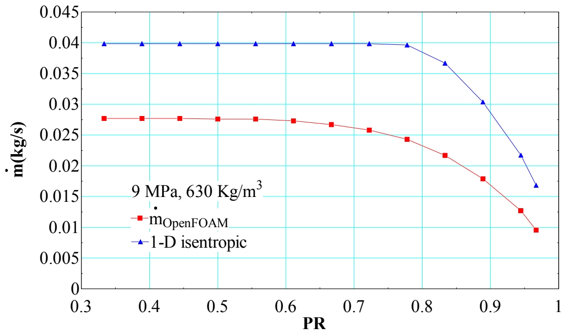
Figure 98. Leakage rate for inlet condition of 9 MPa and 630 Kg/m 3
