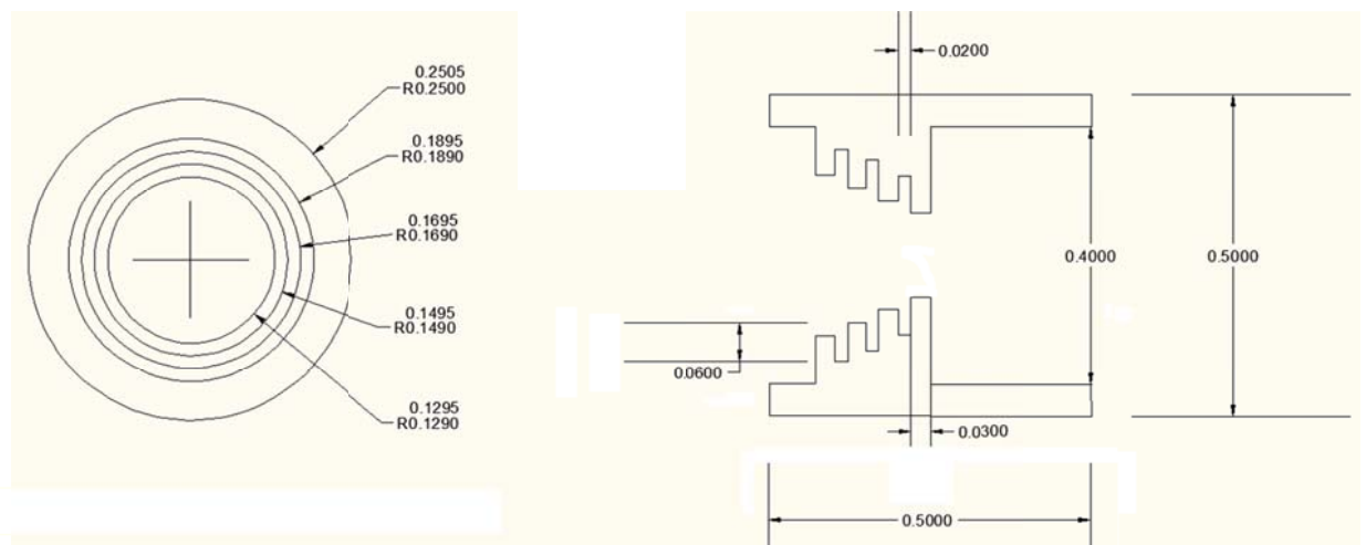
Figure 18. Stepped labyrinth design showing pertinent dimensions.
