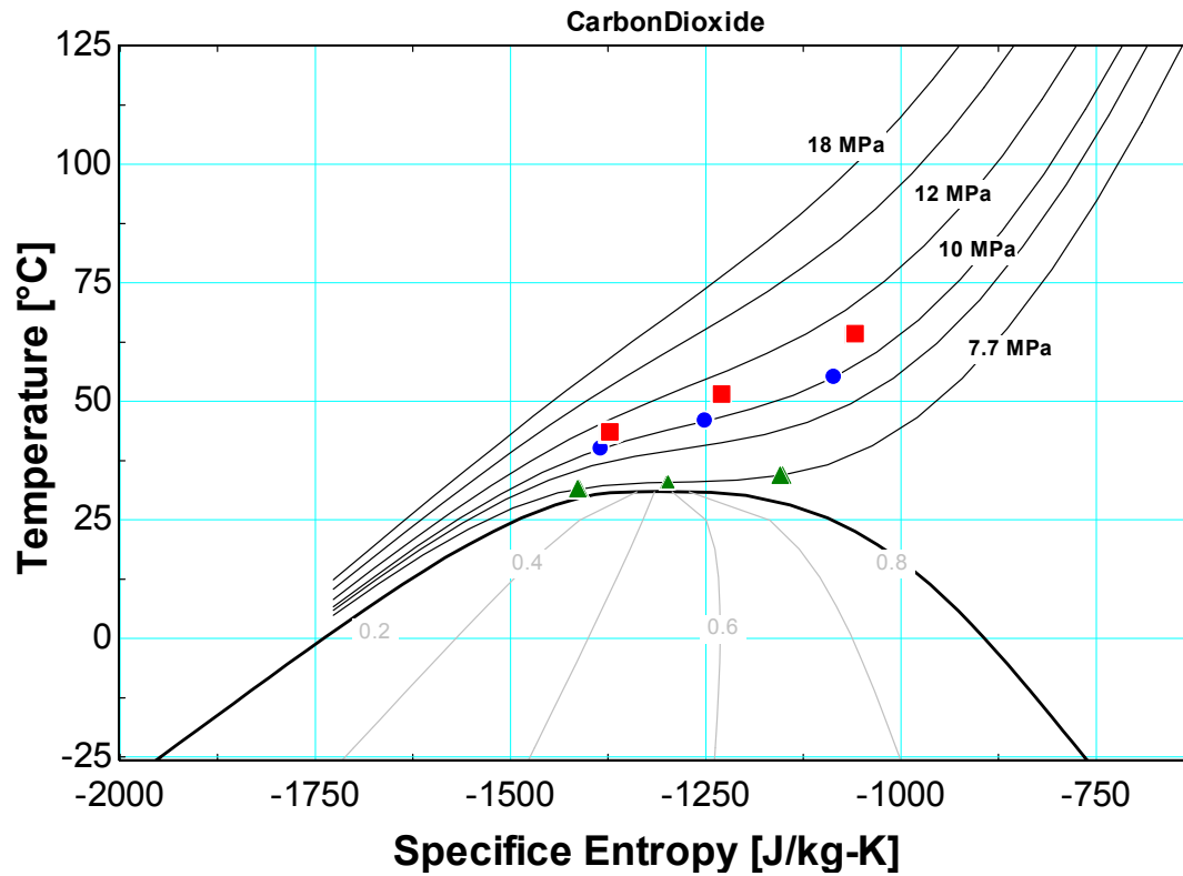
Figure 22. Temperature-specific entropy plot for CO 2 with the test section inlet conditions shown for inlet pressures of 7.7 MPa (green), 10 MPa (blue), and 11 MPa (red) at corresponding inlet densities of 325, 475, and 630 kg/m 3 in three-tooth labyrinth seal tests.
