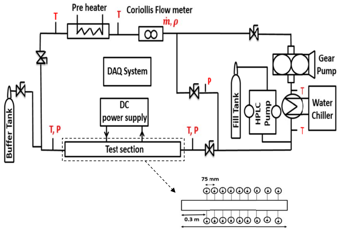
Figure 107. Schematic of the experimental facility and the test section
