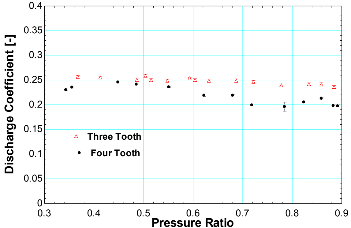
Figure 47. Experimentally determined discharge coefficient for three and four tooth stepped labyrinth seal at an inlet condition of 10 MPa with corresponding inlet density of 640 kg/m 3 .
