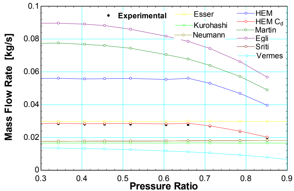
Figure 40. Incompressible and ideal gas condition check for Martin and Egli model over prediction. Inlet pressure of 6.8 MPa with corresponding inlet temperature of 200°C.
