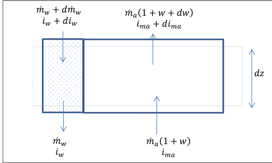
Figure 119. Control volume of counterflow fill configuration
