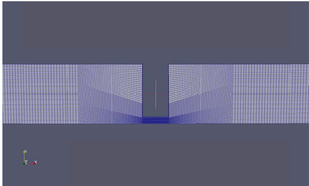
Figure 48. A sample computational mesh used for simulations
