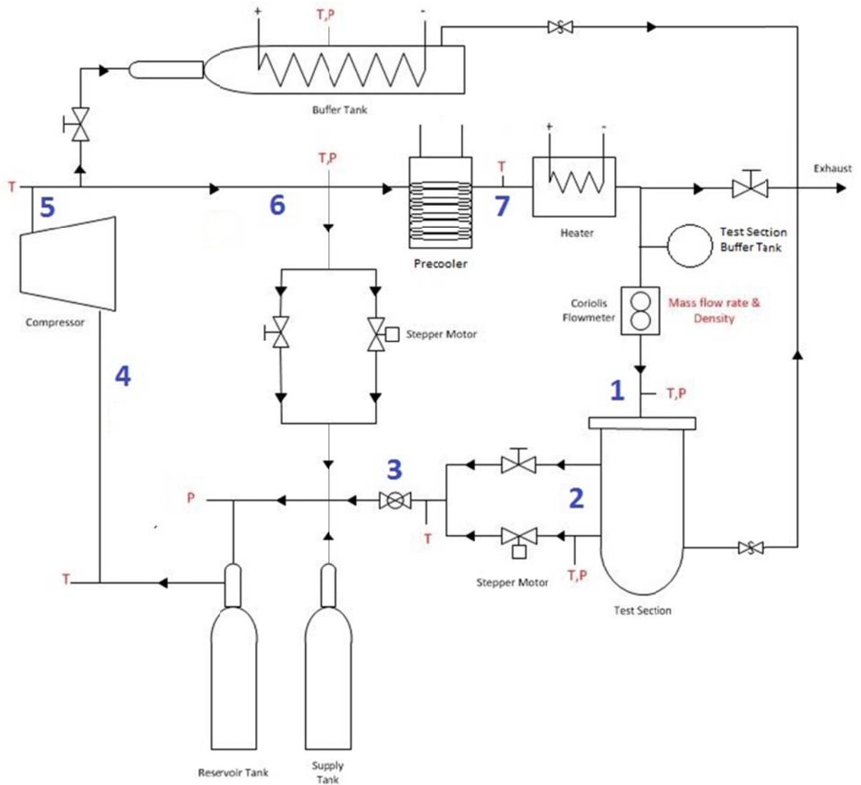
Figure 8. Conceptual layout of the UW-Madison test facility.
