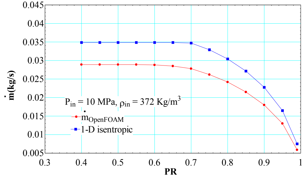
Figure 88. Leakage rate for inlet condition of 10 MPa and 372 Kg/m 3
