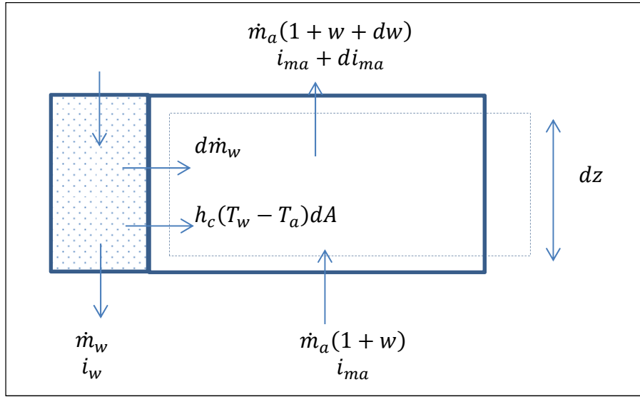
Figure 120. Air side control volume
