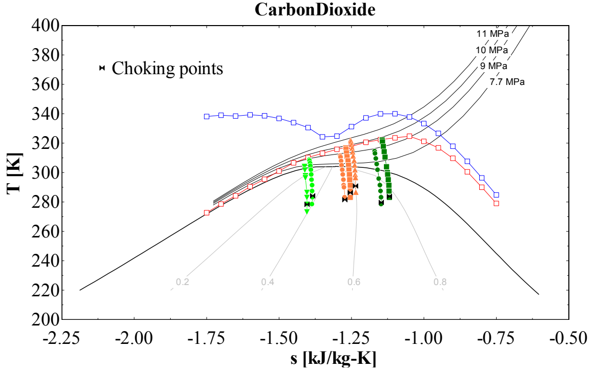
Figure 105. Choking point calculations for labyrinth seal (Flow curve).
