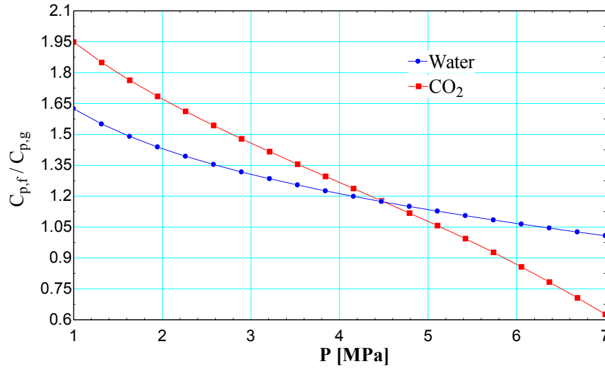
Figure 28. Specific heat ratios for two phase CO 2 and water
