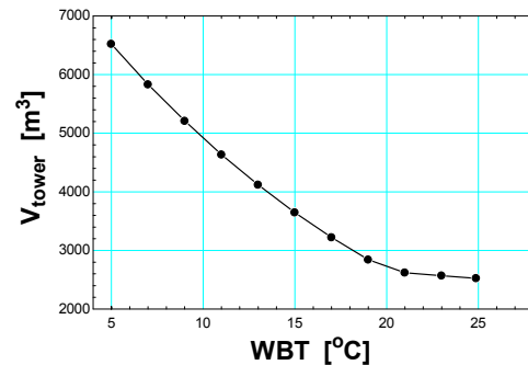
Figure 126. Effect of wet-bulb temperature
