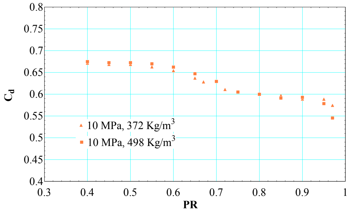
Figure 102. C_d for an inlet pressure of 10 MPa.
