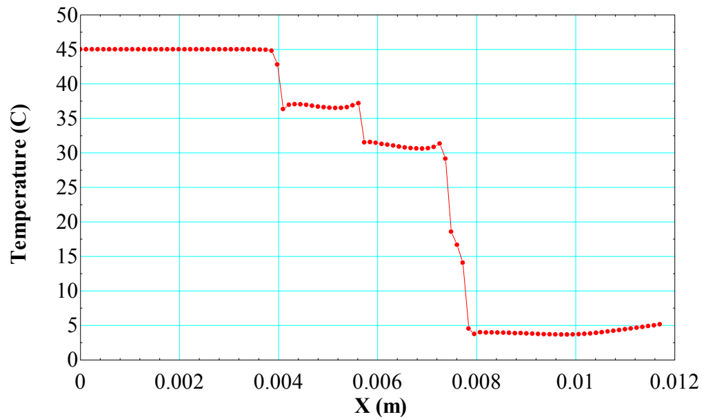
Figure 77. Temperature variation along centerline in the radial clearance region
