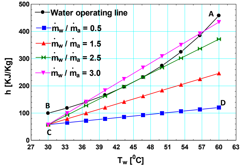
Figure 121. Counterflow cooling diagram
