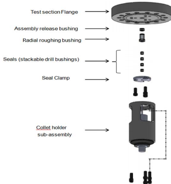
Figure 23. Assembly procedure of shaft-seal sub-assembly.
