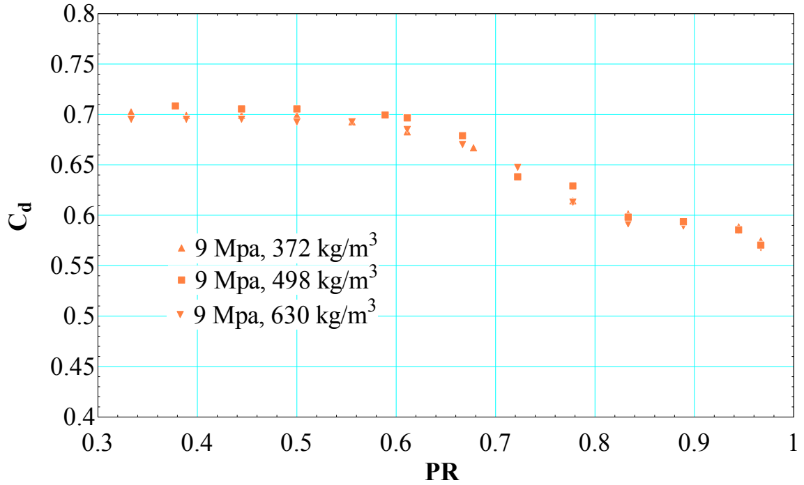
Figure 99. C_d for an inlet pressure of 9 MPa (cases 3, 4 and 5 in Table D.1)
