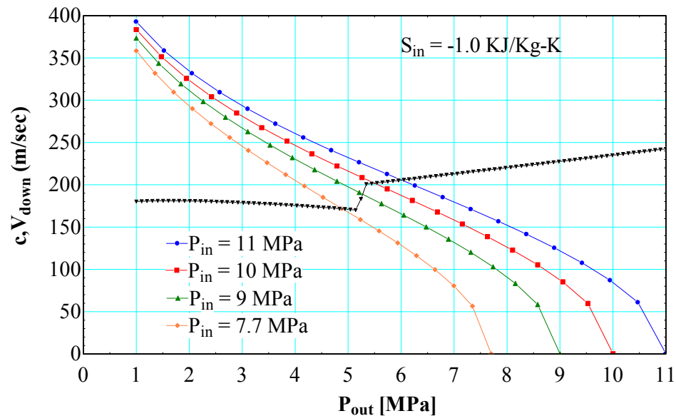
Figure 83. Downstream velocity and local sound speed of an annular orifice as a function of outlet pressure
