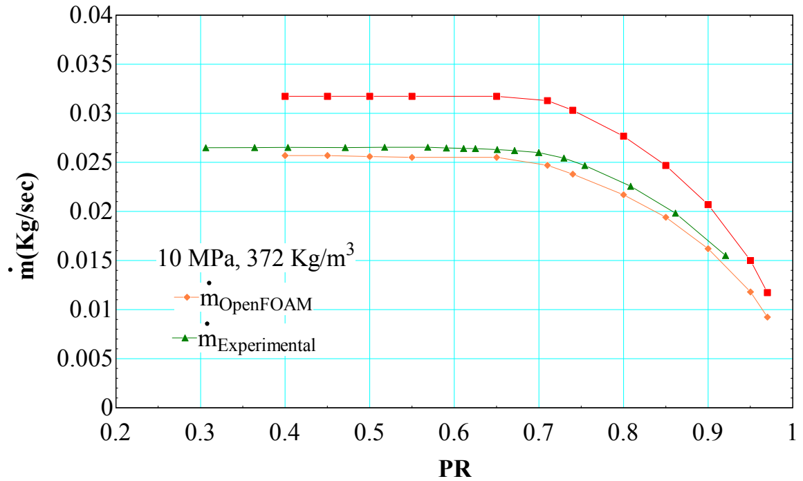
Figure 53. Leakage rate for inlet condition of 10 MPa, 372 Kg/m 3 (case 3 in Table D.3)
