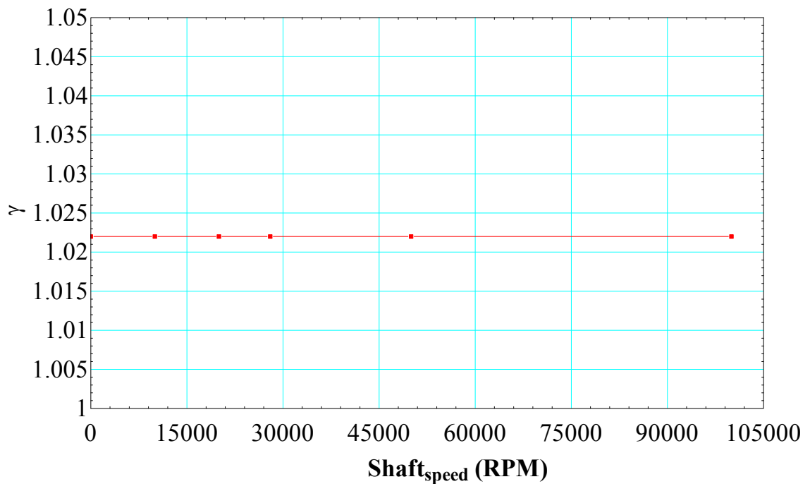
Figure 74. Variation of \gamma with shaft speed
