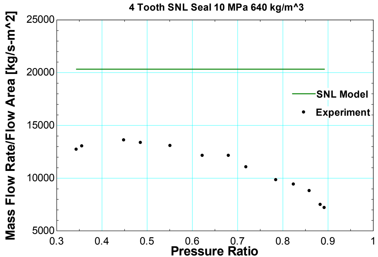
Figure 43. Area normalized mass flow rate comparison of four-tooth stepped labyrinth seal to SNL leakage calculation for inlet condition of 10 MPa and 640 kg/m 3 .
