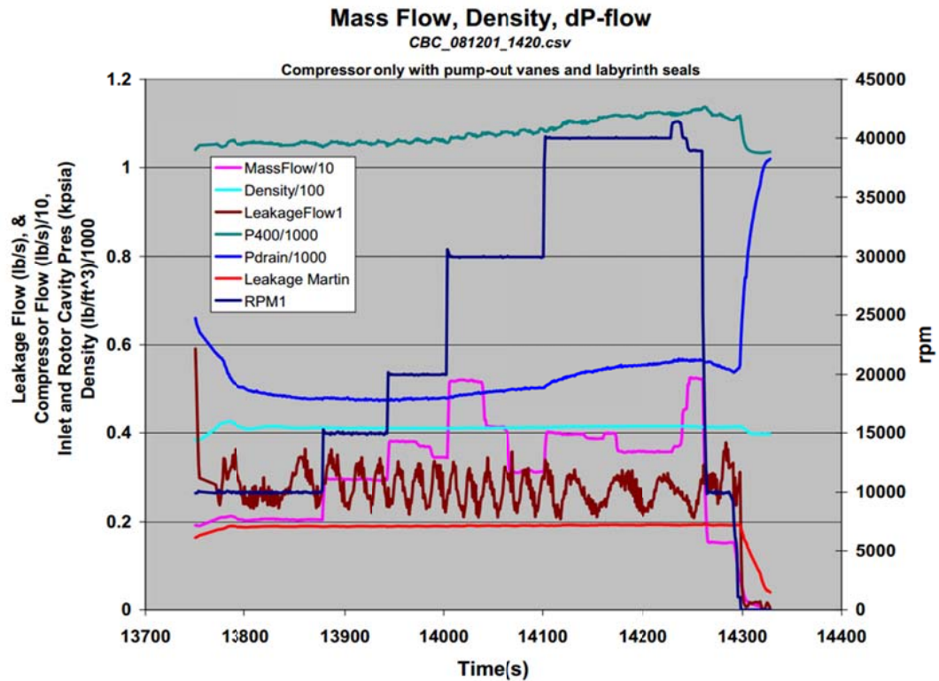
Figure 7. Measured (brown) and predicted (red) leakage flow rate through the SNL four tooth stepped labyrinth seal [2].
