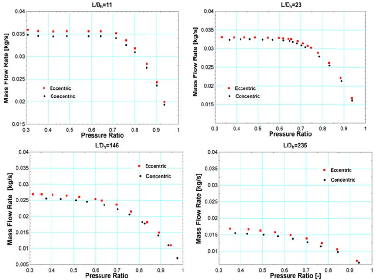
Figure 31. Experimental mass flow rate for annuli of varying L/D_h with a D_H=0.195 mm and inlet conditions of P_{in} = 10 MPa and \rho_{in}=325 kg/m 3 .
