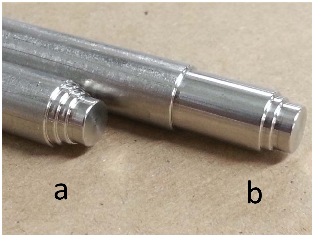
Figure 21. Shafts used in stepped labyrinth geometry, a) 4-land shaft b) 3-land shaft.
