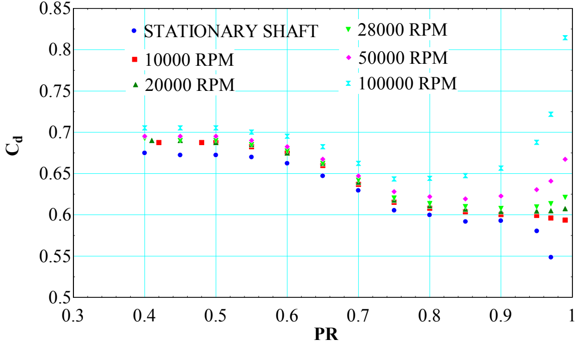
Figure 75. Variation of the C_d with shaft speed for labyrinth seals
