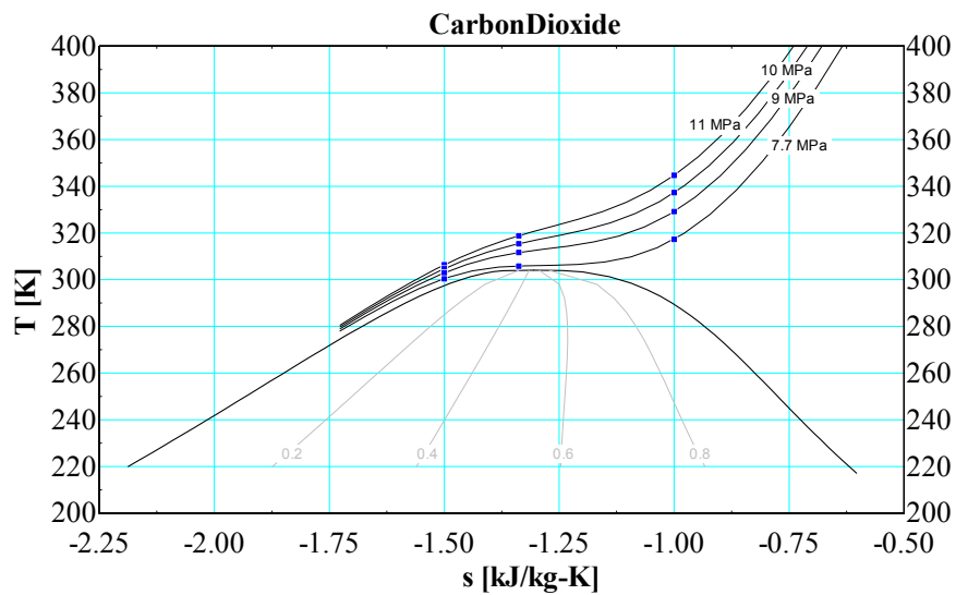
Figure 79. Inlet conditions used for testing 1-D isentropic model
