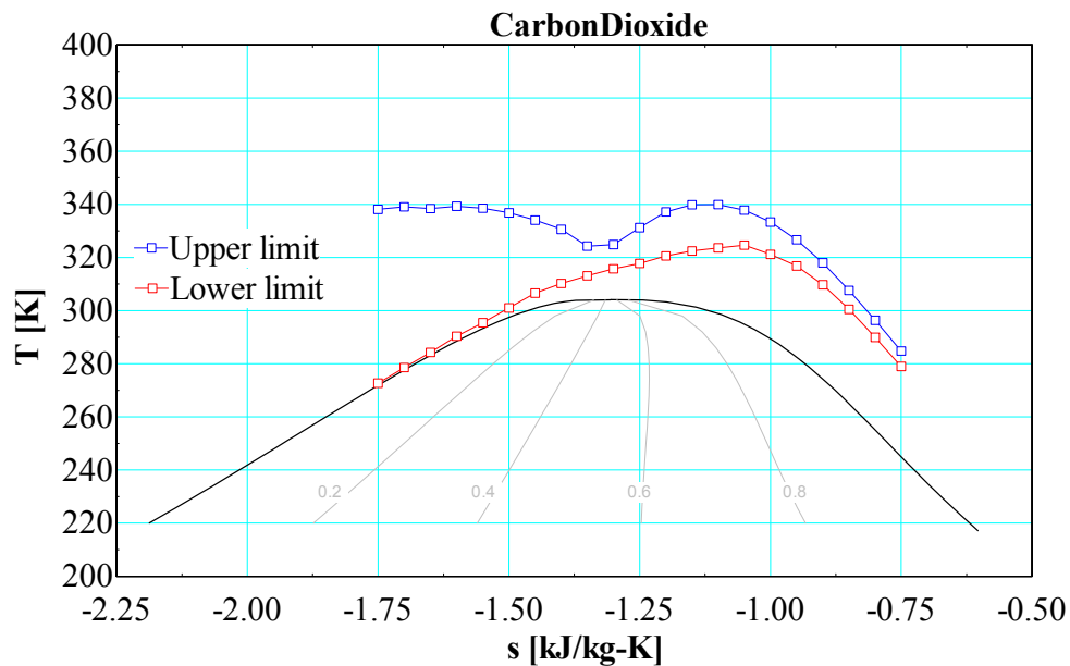
Figure 84. Choking theory for isentropic flow.
