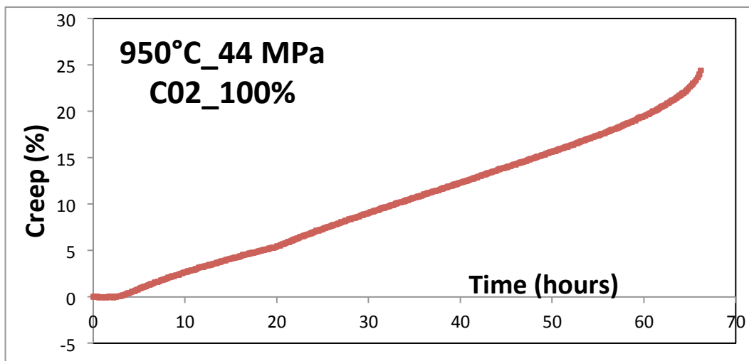
Figure 2.1.2.7. Engineering creep strain as a function of time for specimen C02 at 950°C under 44 MPa. The test ended in rupture at 24.4% strain.
