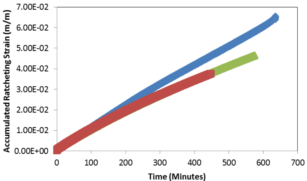
Figure 2.2.2.9. Accumulated axial ratcheting strain as a function of time for specimen 4-5-1 (Blue) and following tests interrupted at 71% and 58% of the accumulated (ratcheted) axial strain to failure.
