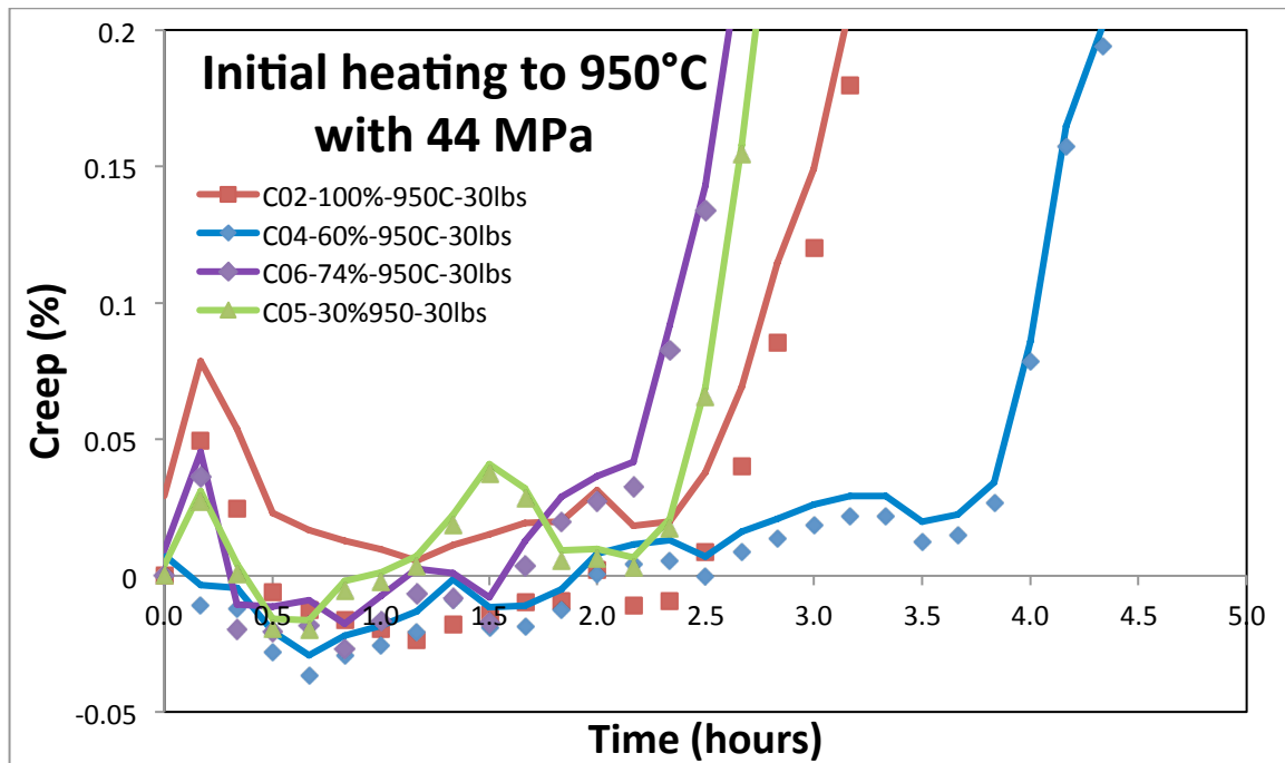
Figure 2.1.2.9. Initial strain during the heating from room temperature to about 950°C.
