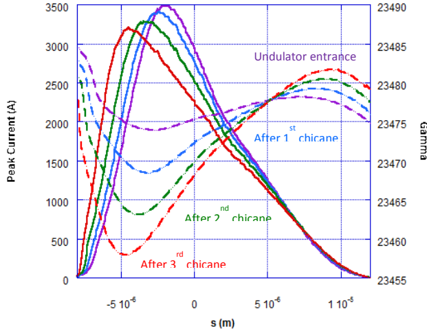
FIG. 4. The CSR-induced reduction in peak current (solid lines) and slice beam gamma (dashed lines) as functions of the electron bunch position at three different undulator locations: purple = undulator entrance, blue = after the first chicane, green = after the second chicane, and red = after the third chicane.
