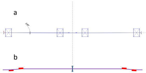
FIG. 2. a) The four-dipole bypass chicane with the 4BCM in between the two middle dipoles; b) expanded view of the 4BCM showing the four Si(111) crystals in red and the slit in blue. The total length of the bypass chicane (2a) is 8.63 m whereas the length of the 4BCM (2b) is 0.4 m.
