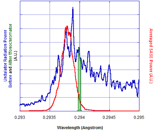
FIG. 3. The undulator radiation spectrum before (blue) and after (green) the 4BCM, and the average SASE signal in the exponential gain regime (red).
