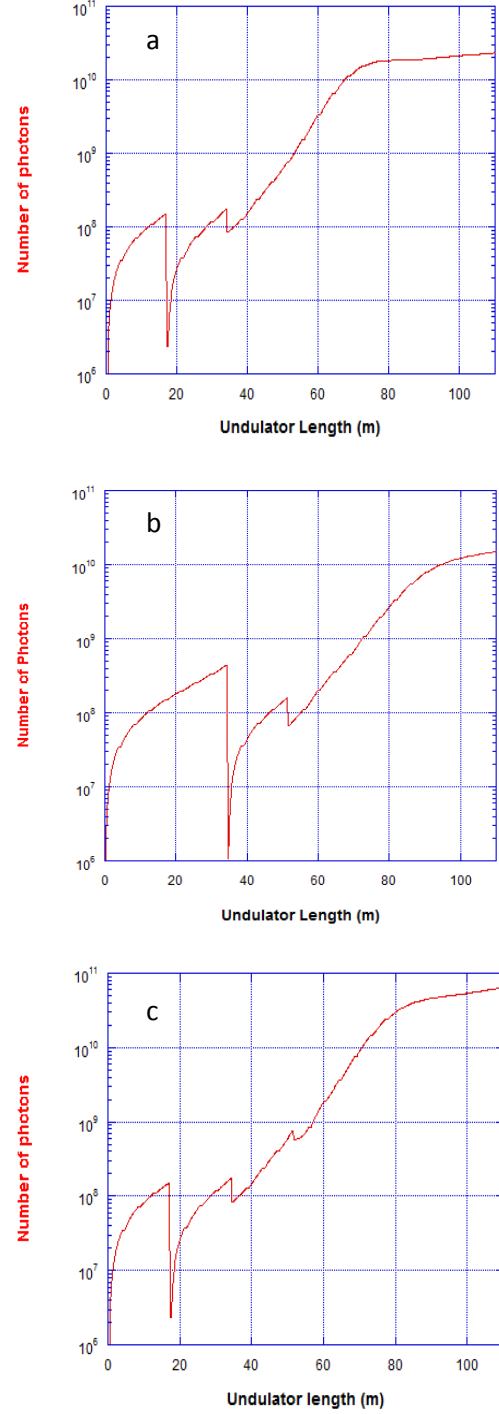
FIG. 5. a) Plots of the number of photons versus undulator length for the DS configurations a) two-filter AB; b) two-filter BC; and c) three-filter ABC.
