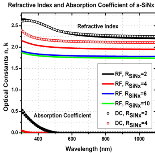
Figure 3.3b) Optical constants of a-SiN x each grown with different process gas flow ratios and deposited by RF or DC plasma.
