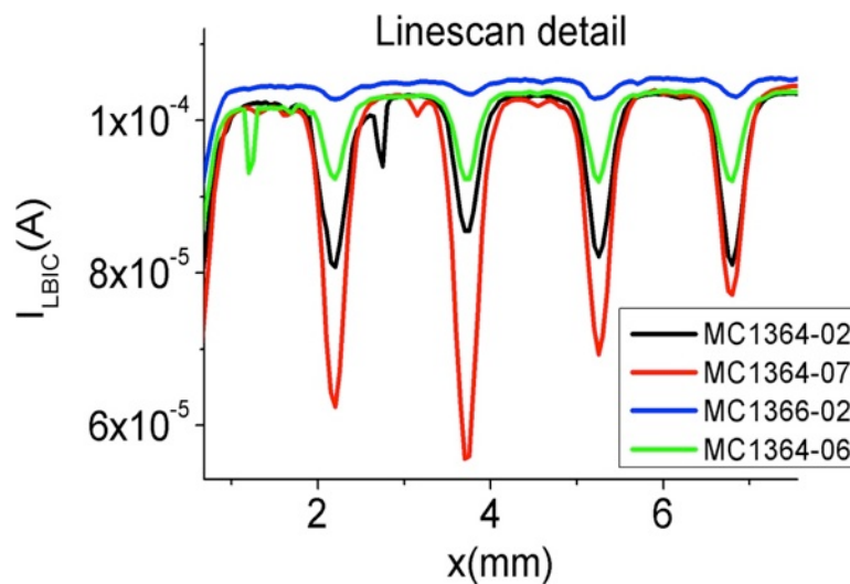
Figure 5.3 LBIC line scans of 4 IBC cells described in Table 5.2. Complete LBIC image for MC1364-02 is shown above in Figure 5.2. The narrow valleys are over the n-strip and wider peaks are over the p-strip.
