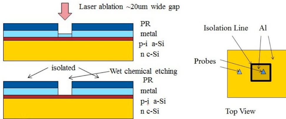
Figure 4.13. (Left) Diagram showing vertical structure during laser-guided chemical isolation. (Right) Horizontal layout for electrical test.
