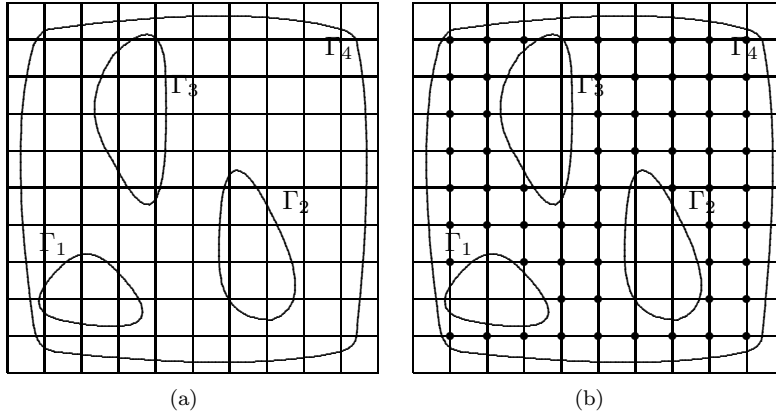
FIG. 2.2. Discretization of the geometry without the mask shown (a) and with the mask shown (b), dots indicate m_{ij} = 1 .
