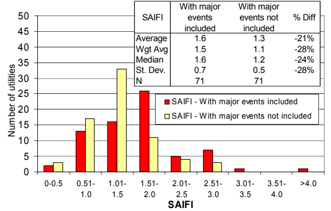
Fig. 3. Distribution of and Summary Statistics for SAIFI Reported With Major Events Included and Not Included
