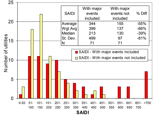
Fig. 2. Distribution of and Summary Statistics for SAIDI Reported With Major Events Included and Not Included
