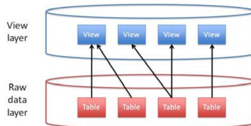
Figure 3: Structure of the MySQL database
