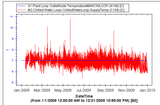
Figure 7: Example time series plot comparing measured and simulated data Chilled water loop supply temperature (measured and simulated) over a 12-month period
