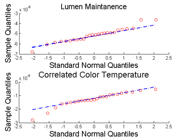
Figure 4: QQ plot for normalized luminous flux output and normalized correlated color temperature for LUXEON LEDs
