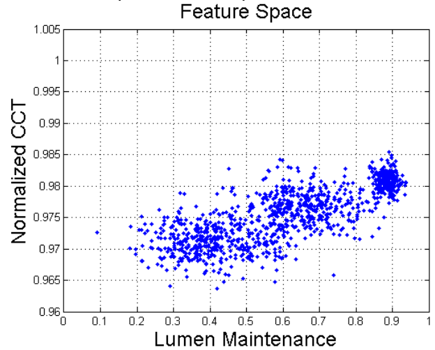
Figure 6: Feature space containing data of lamp's current state, lamp's failure threshold, and pristine healthy distribution of lamps prior to classification.
