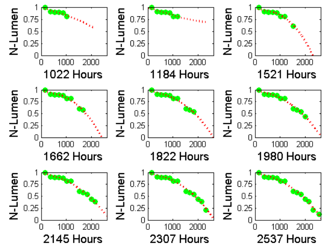
Figure 12: Bayesian Regression Learning Process
