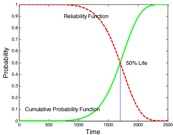
Figure 15 System Reliability Function and Cumulative Probability Function
