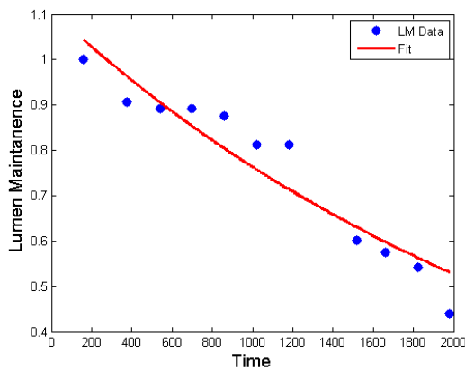
Figure 2: Lumen Maintenance Evolution for the LED Lamp in 85°C/85RH
