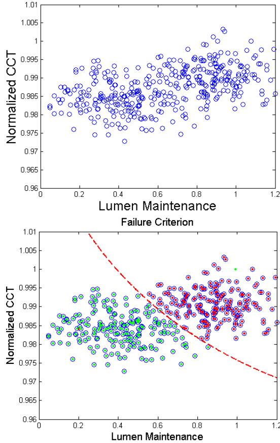
Figure 7: End of Life distribution and pristine for LED Lamp. Red data points are the healthy samples and the green data points are the samples with accrued damage
