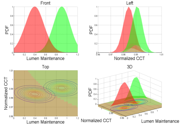
Figure 8: Classification of the lamps with accrued damage and pristine lamp PDFs. Red data points are the healthy samples and the green data points are the samples with accrued damage
