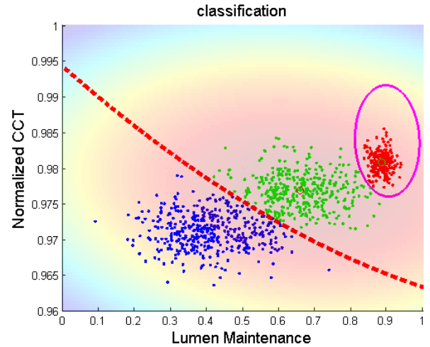
Figure 9: L70 Time Decision Boundary. Pristine lamp group has been shown in RED. Damaged LED Lamp group is shown in GREEN. Lamps beyond the failure threshold are shown in BLUE.
