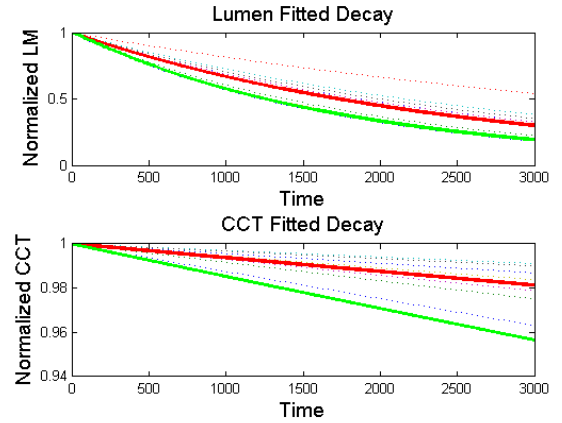
Figure 5: Characterized Decay Rate Curve for the LED Lamp
