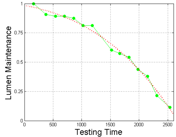
Figure 11: Lumen Maintenance Regression for LED Lamp
