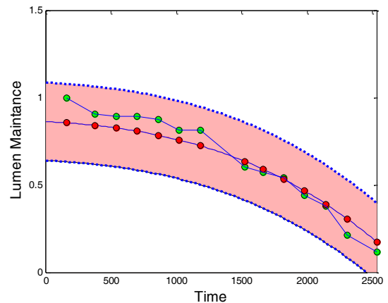
Figure 13: Bayesian Regression with Confidence Interval
