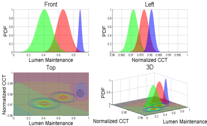
Figure 10: Critical Failure, LED Lamp Failure and Pristine Lamp PDF Distribution
