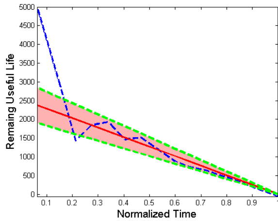
Figure 14: \alpha - \lambda Plot of RUL Prediction
