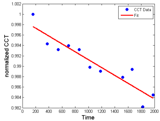
Figure 3: Correlated Color Temperature Evolution for the LED Lamp in 85°C/85RH
