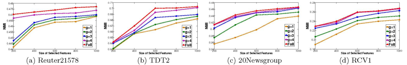
Figure 7: Performance comparison of FSDS with different values of g .
