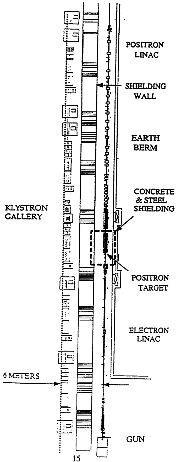
Figure 4. Layout of the linac showing 6 m line in the klystron gallery.
