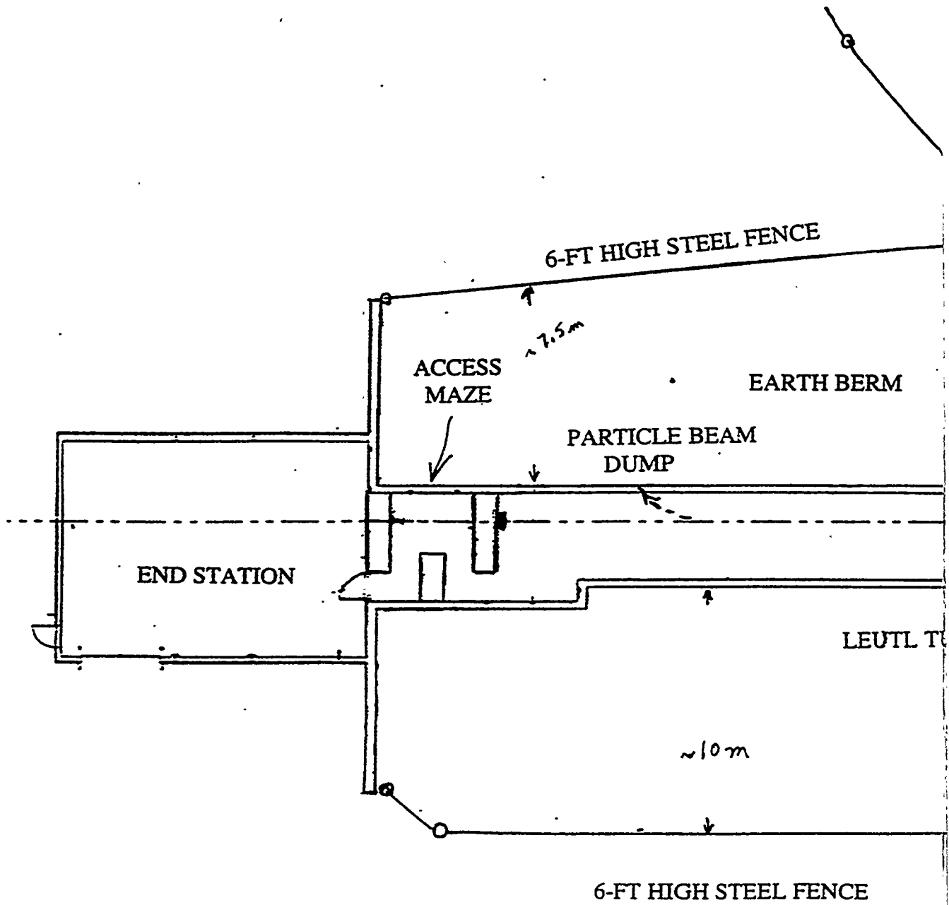
Figure 1. LEUTL building with the end station.
