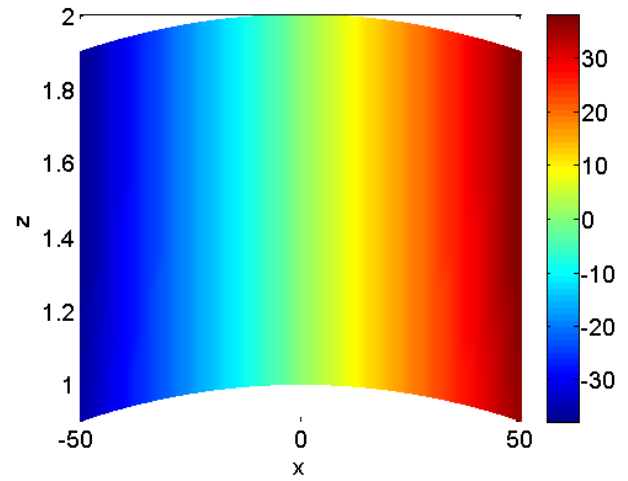
Figure 4. Contour plot of the exact solution to the x - z MMS test case.
