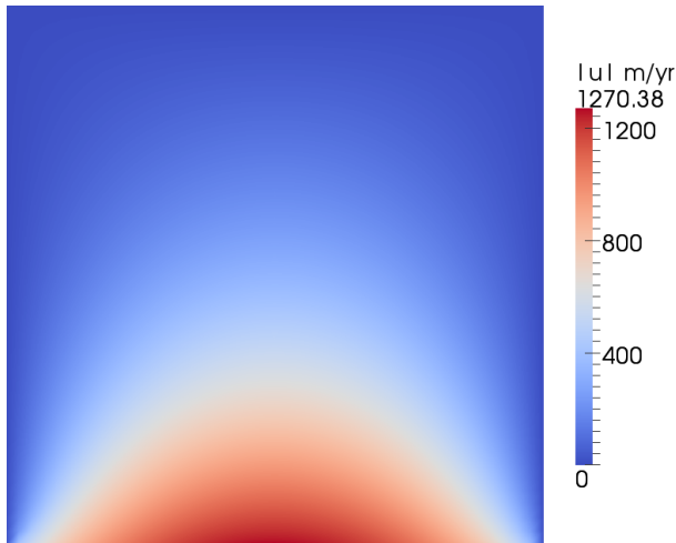
Figure 8. Albany/FELIX solution to the confined-shelf test case (indistinguishable from the solution obtained by the solver of Perego et al. (2012)).
