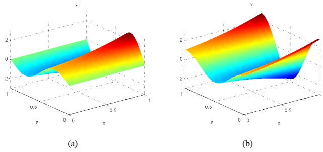
Figure 2. Plots of exact solutions to the x - y MMS test case: (a) u , (b) v .
