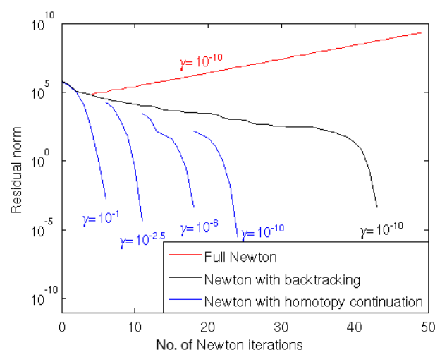
Figure 12. The robustness of Newton's method nonlinear solves with homotopy continuation.
