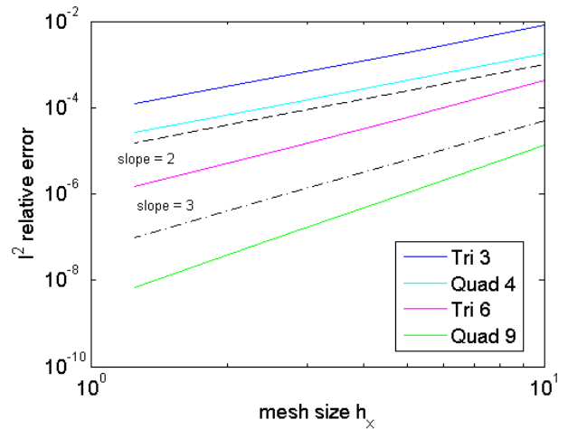
Figure 5. Convergence rates for the x - z MMS test case in the discrete l^2 norm Eq. (23).
