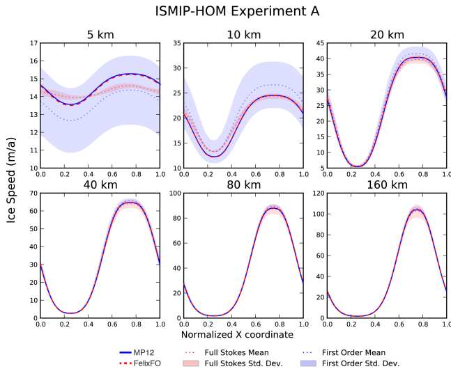
Figure 6. ISMIP-HOM test A: surface velocity component u as a function of x at y = L/4 for each L considered. The blue solid line (MP12) represents results from Perego et al. (2012) and the red dashed line (labeled FelixFO) represents results from the current solver.
