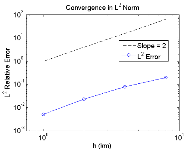
Figure 11. Convergence in the continuous L^2 norm Eq. (46) for the realistic GIS problem with full 3-D refinement.
