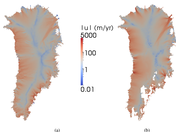
Figure 15. Solution magnitude |u| in meters per year: (a) Albany/FELIX solution (surface speed) on the variable resolution (1–7 km) tetrahedral mesh, and (b) observed surface speeds (from Joughin et al. (2010)).
