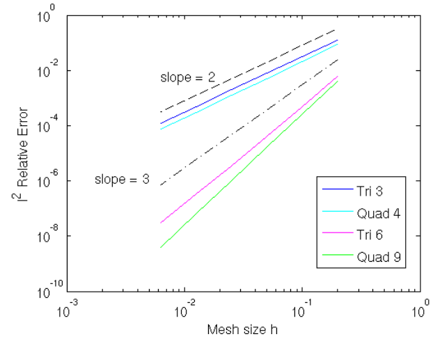
Figure 3. Convergence rates for the x - y MMS test case in the discrete l^2 norm Eq. (23).
