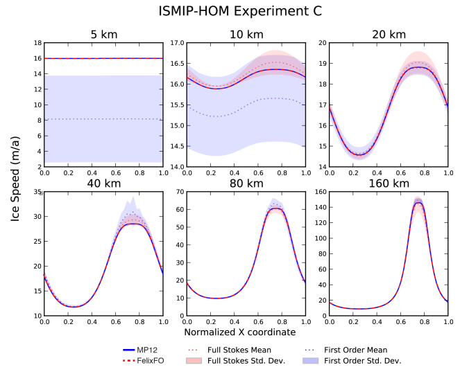
Figure 7. ISMIP-HOM test C: surface velocity component u as a function of x at y = L/4 for each L considered. The blue solid line (MP12) represents results from Perego et al. (2012) and the red dashed line (labeled FelixFO) represents results from the current solver. Note that, for the 5 km test, the MP12 and FelixFO results directly overlie the results for the full Stokes models participating in the original intercomparison.
