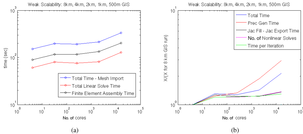
Figure 13. Controlled, weak scalability study on Hopper : (a) total linear solve, finite element assembly, and total run times in seconds, and (b) additional timing information ( X = time or number of iterations).
