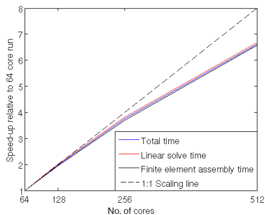
Figure 16. Strong scalability for the 1–7 km resolution GIS problem: speed-up relative to the 64-core run.
