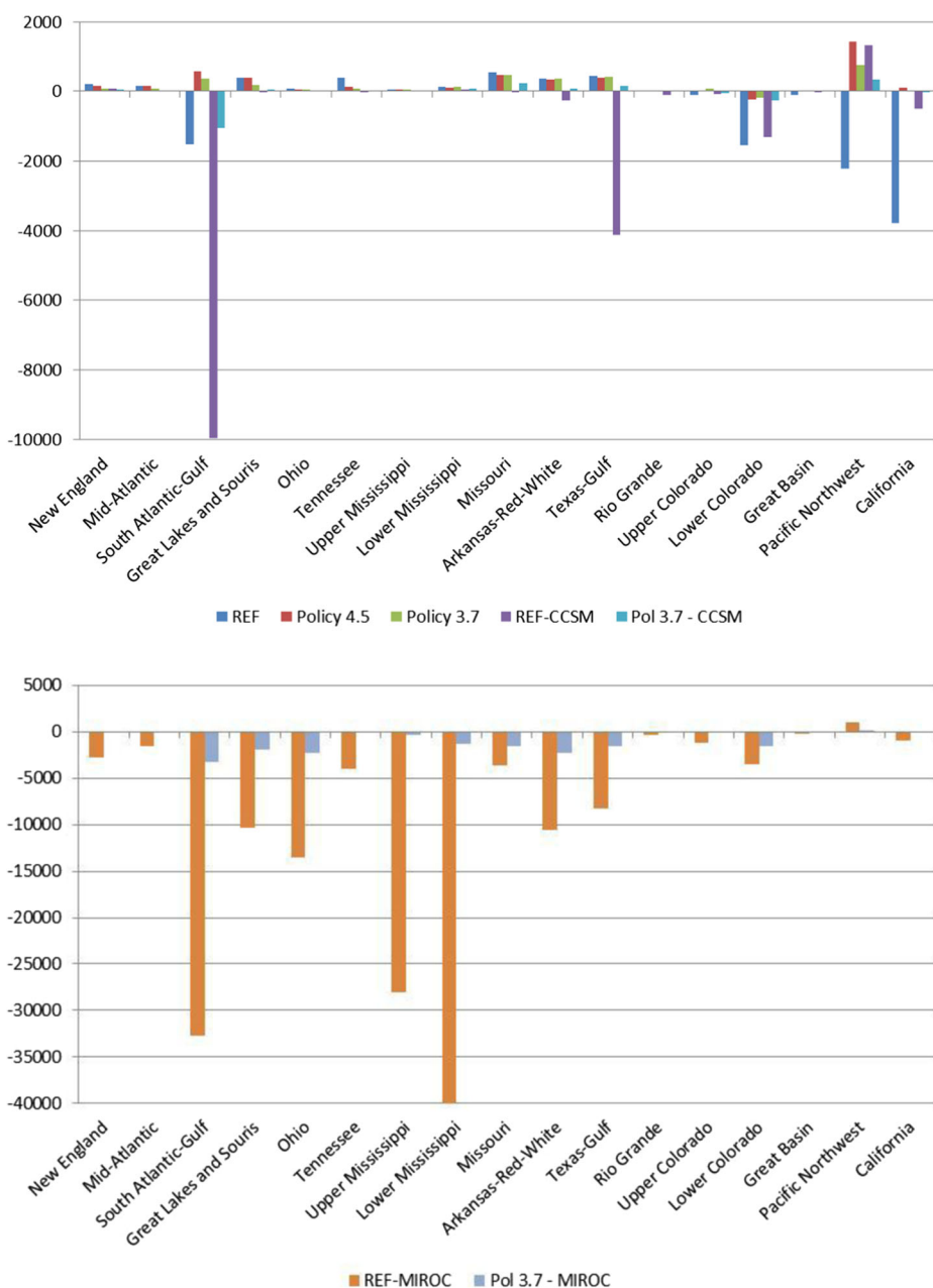
Fig. 6 Supply/demand balance annual economic welfare estimates in 2100 by WRR for REF and GHG mitigation scenarios (million 2005$). The IGSM-CAM and CCSM results in the upper panel , MIROC results in the lower panel ; note the significant difference in the vertical scale of the lower versus upper panels
