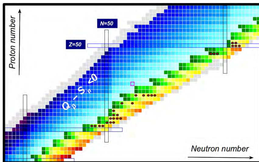
Figure 2. Chart of the nuclei where the colors are a measure of the difference between the energy released in beta decay ( Q_{\beta} ) and the neutron separation energy ( S_n ). For most nuclei (shades of blue) the Q_{\beta} energy is less than the neutron separation energy and therefore no beta-delayed neutrons would be emitted. The red points indicate radioactive ^{238}\text{U} fission products where the beta-delayed neutrons were measured in Winter 2012 with VANDLE at HRIBF.
