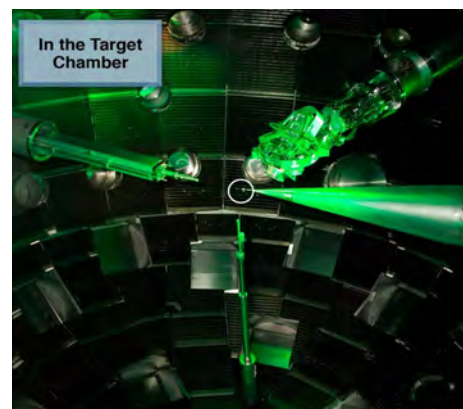
Figure 1. Target assembly for a shock-timing target held in place by the cryogenic cooling target positioner system (left image). View inside the NIF chamber of a target inserted on the positioner system as well as several diagnostic arms (right image).
