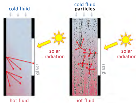
Figure 1. Heating of a mixture via a conventional receiver (left) and a particle-based receiver (right).
