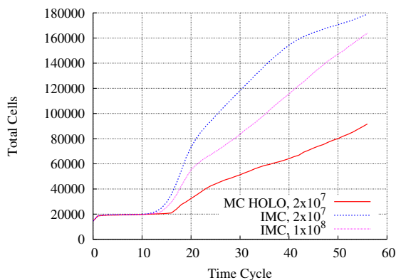
Comparison of total number of spatial cells vs. the time cycle in the Al shell problem; note the two-fold reduction in HO-LO MC vs. IMC.
