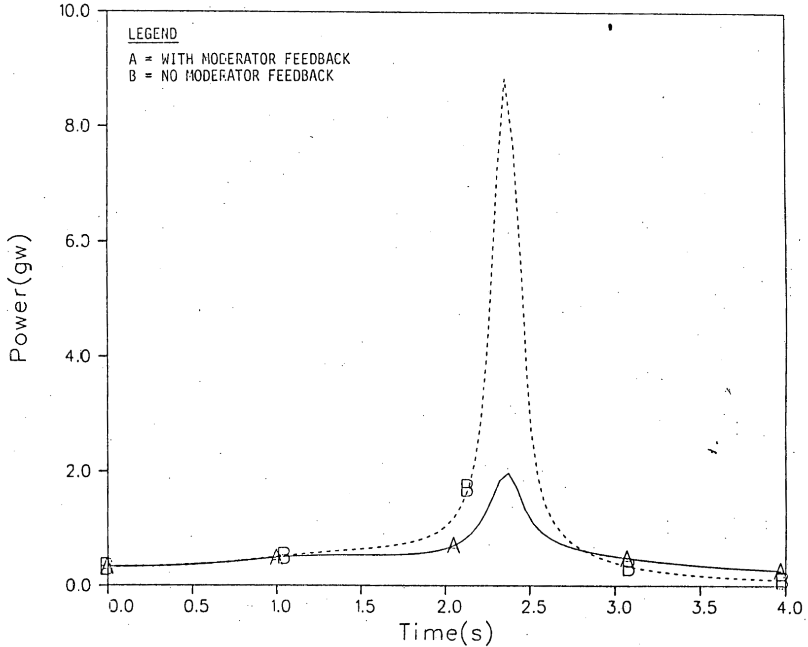
Figure 1 Transient behavior of reactor power
