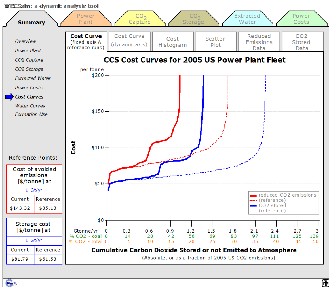
Figure 23. WECSsim Cost Curves.
