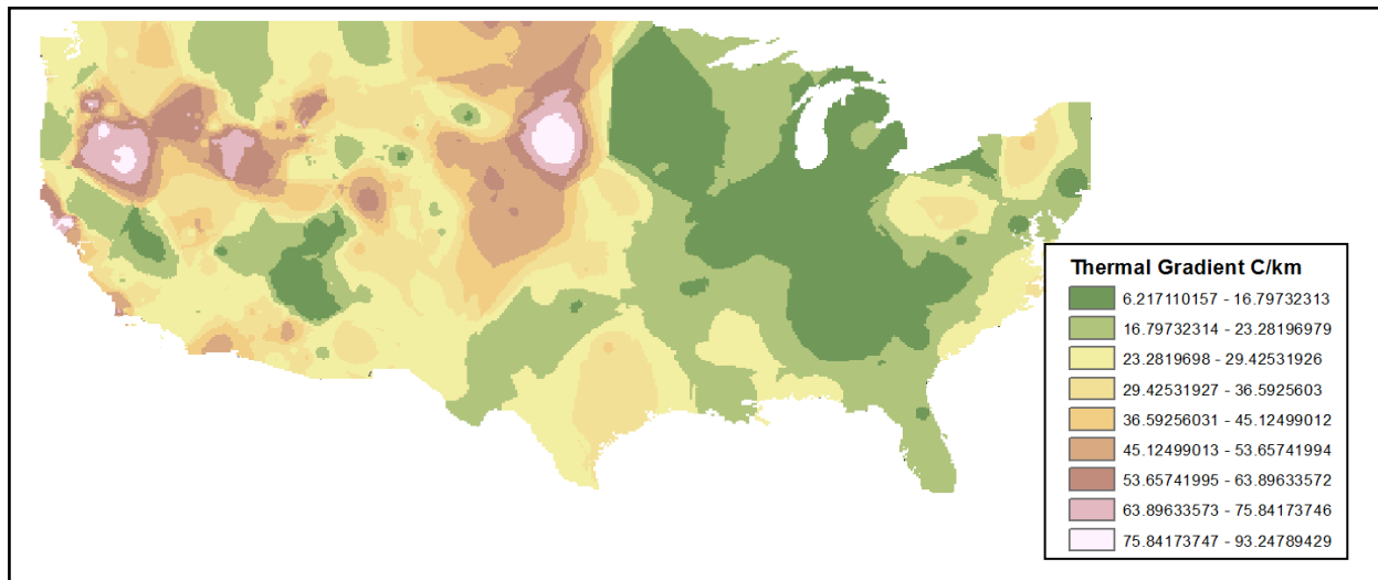
Figure F-12. Initial thermal gradient surface developed using inverse distance weighting of well based point estimates of thermal gradient from the wells shown in Figure F-11.
