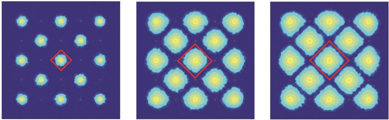
Figure F-3. CO 2 plume (shown in light blue to yellow) growth through time from TOUGH2.
