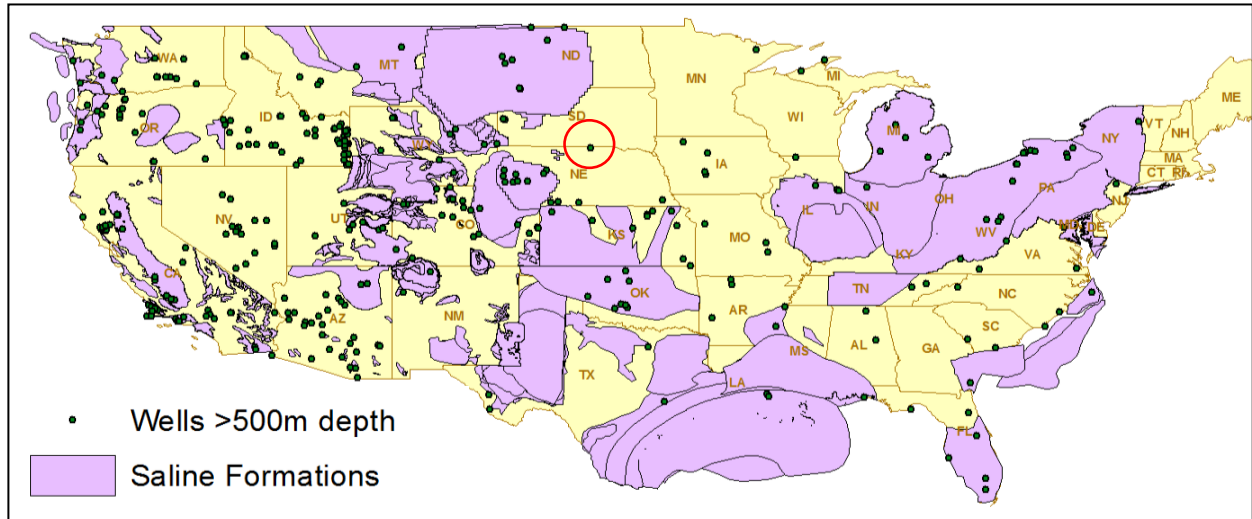
Figure F-11. Wells deeper than 500 meters with thermal gradients less than 100 degrees C per kilometer used to develop the spatially distributed estimate of thermal gradients.
