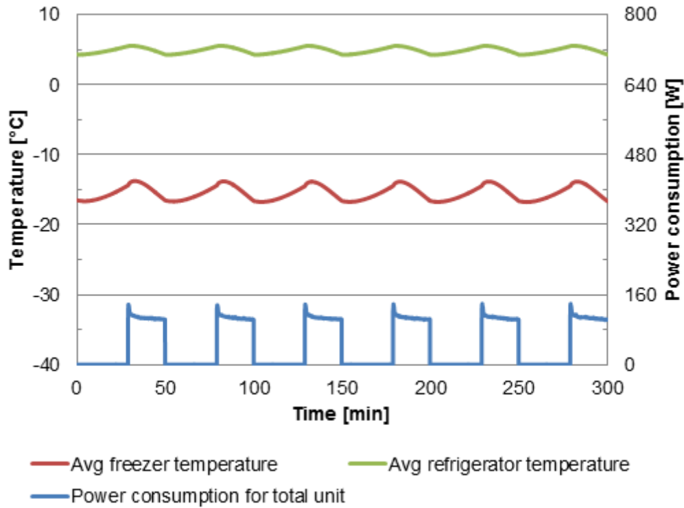
Fig. 4.1: Variation of temperatures and power consumption (“stabilization” at T_{\text{amb}}=32.2^{\circ}\text{C} and medium temperature setting)
