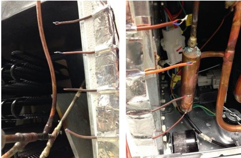
Fig. 2.7: Surface thermocouples for air side temperature measurement
