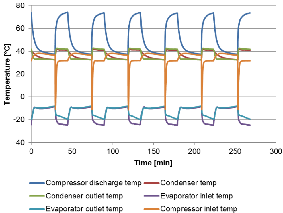
Fig. 4.5: Variation of temperatures and power consumption (“stabilization” at T_{\text{amb}}=32.2^{\circ}\text{C} and warmest temperature setting)
