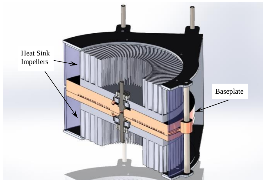
Fig. 3.24: Cross-section of the SCC assembly
