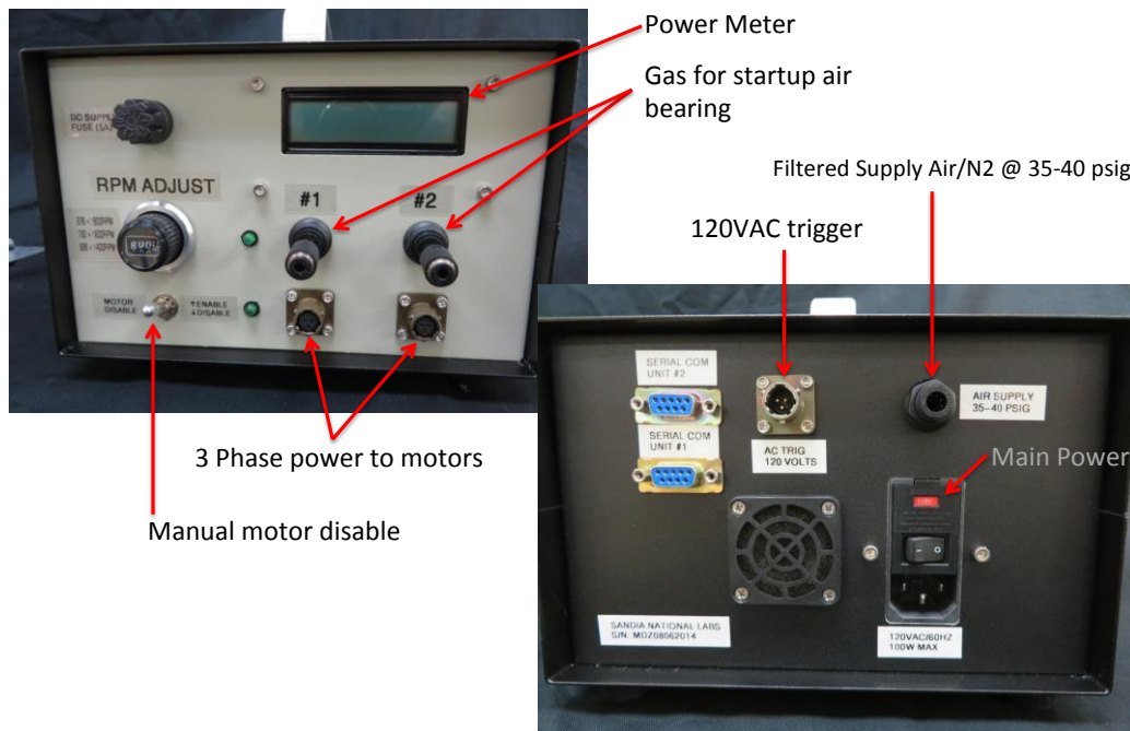
Fig. 3.20: Front/Rear panel
