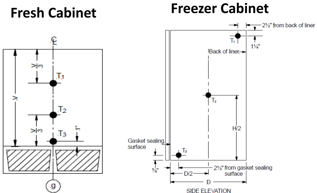
Fig. 2.10: Locations of thermocouples measuring compartment temperature
