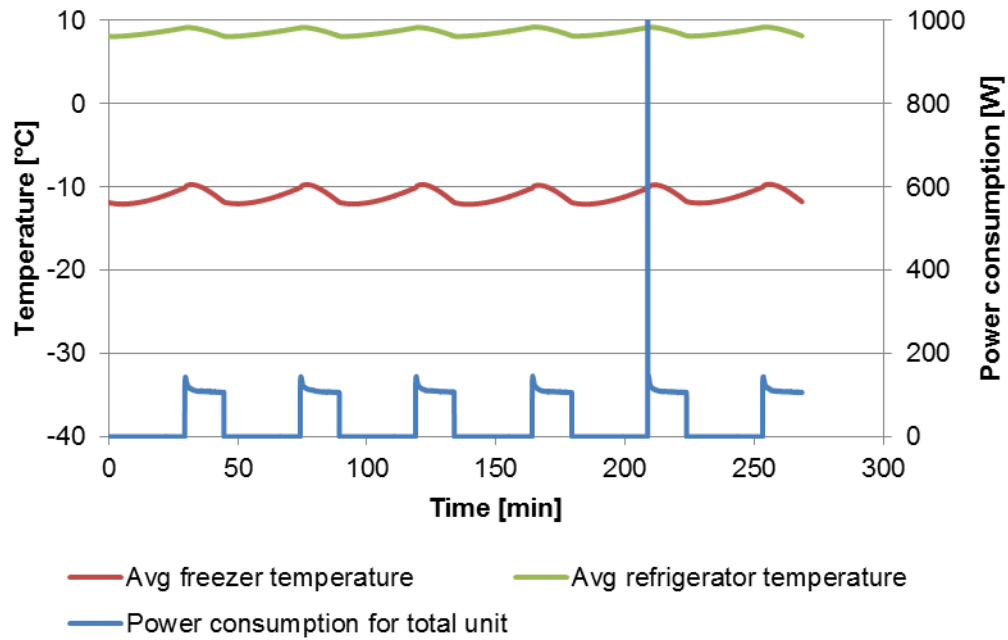
Fig. 4.5: Variation of temperatures and power consumption (“stabilization” at T_{\text{amb}}=32.2^{\circ}\text{C} and warmest temperature setting)
