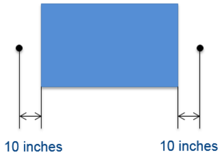
Fig. 2.12: Locations of thermocouples measuring ambient temperature (top-view (left); side-view (right))
