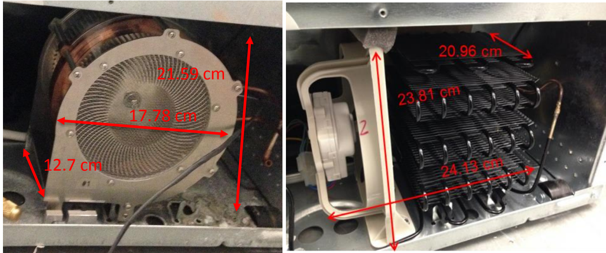
Fig. 4.23: Dimensions for the SCC (left) and conventional tube-fin heat exchanger and fan (right)
