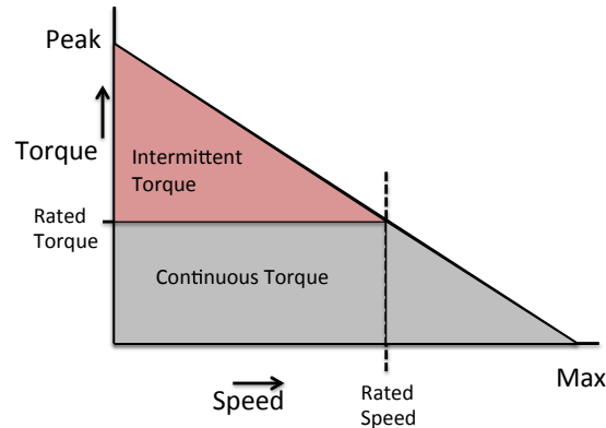
Fig. 3.16: Torque-speed curve
