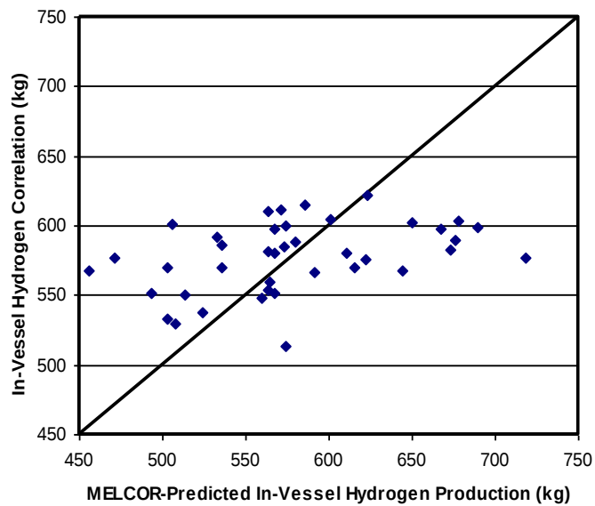
Figure 79: Comparison between MELCOR-predicted and correlated final, in-vessel, hydrogen production
