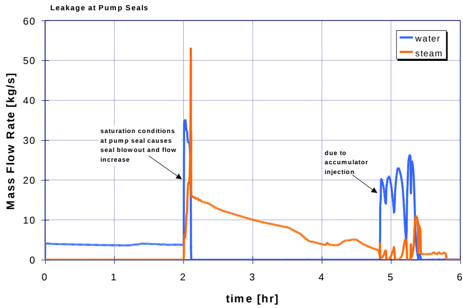
Figure 36: Case 26: Pump seal leakage of water and steam from four RCS pumps
