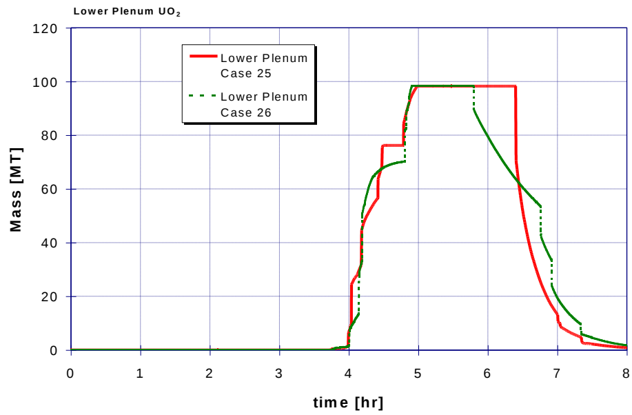
Figure 55: Relocation of fuel to lower plenum - comparison of Case 25 and Case 26
