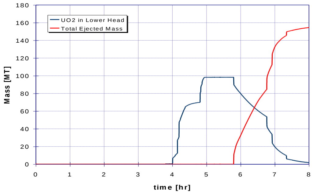
Figure 43: Case 26: Materials in lower head and in cavity
