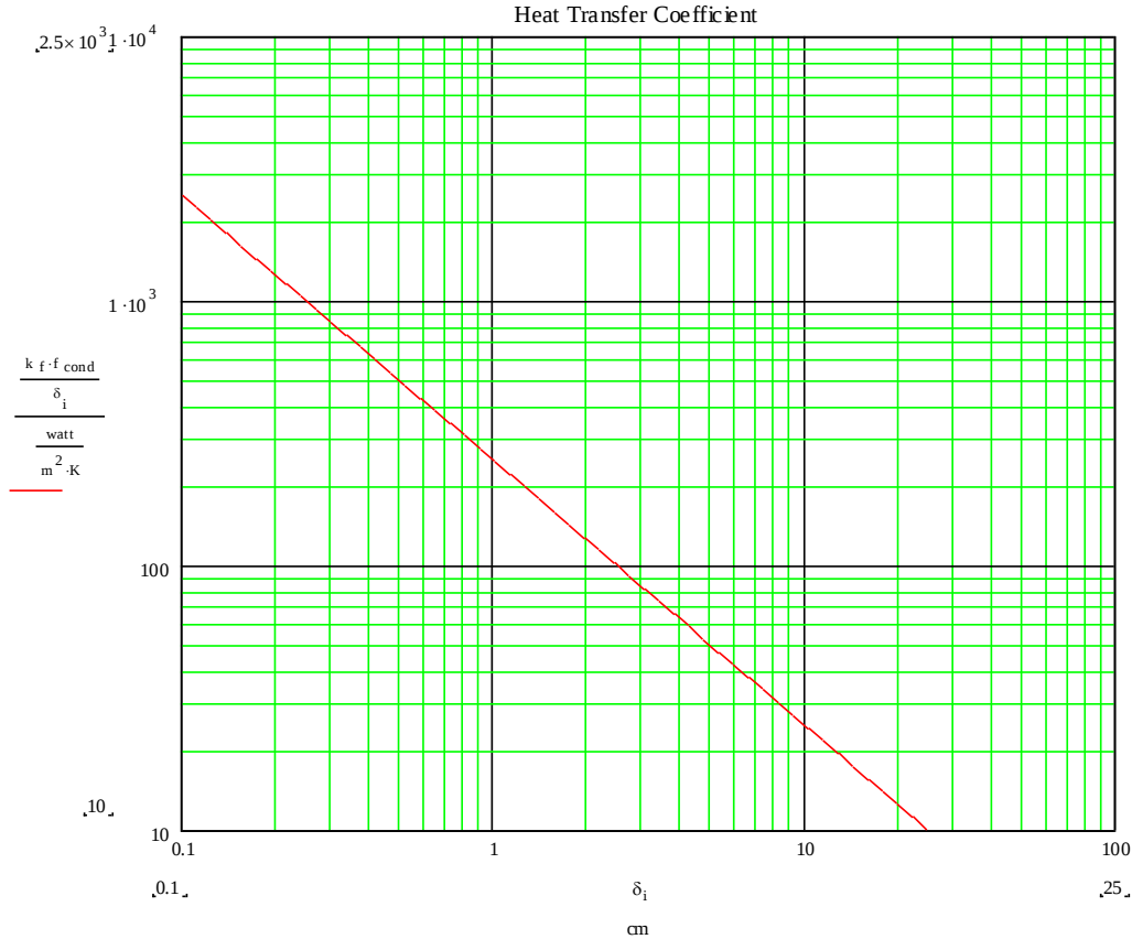
Figure 8: Estimation of heat transfer coefficient for lower heat heating by fuel debris
