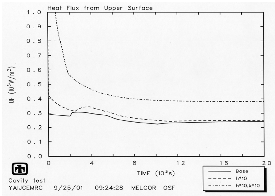
Figure 26: Predicted heat flux to the pool for default and modified CORCON analysis of MCCI in a Sequoyah cavity
