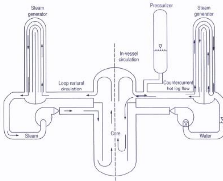
Figure 11: Illustration of the full-loop and hot leg counter-current natural circulation patterns in the Westinghouse PWR reactor coolant system
