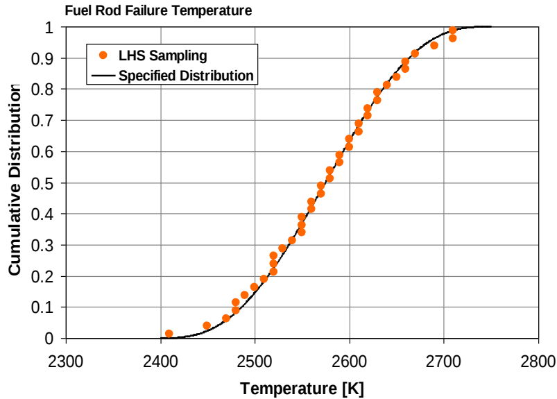
Figure 16: Cumulative probability distributions estimated for fuel rod collapse temperature
