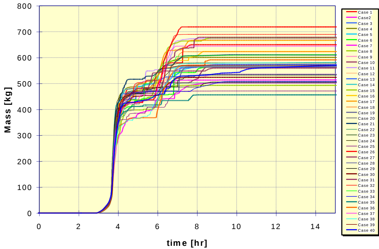
Figure 34: Summary of in-vessel hydrogen production for all cases in study
