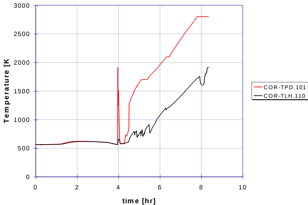
Figure 10: MELCOR-predicted temperatures of lower head debris and head wall for the Sequoyah model using the control function heat transfer coefficient
