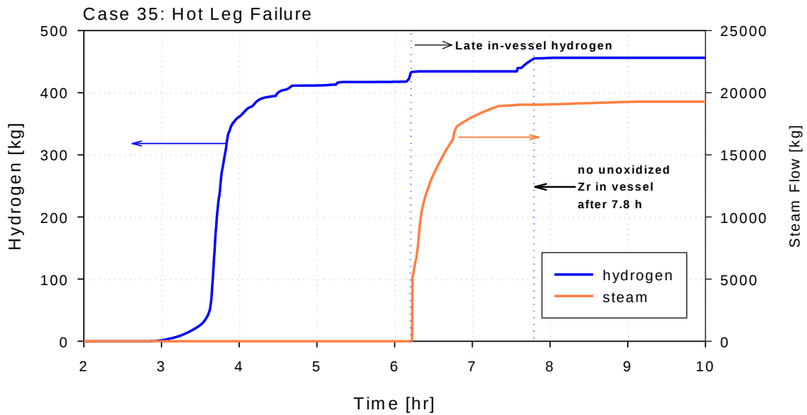
Figure 77: In-vessel hydrogen produced and break steam flow for case with low late-time in-vessel hydrogen for case with hot leg failure and low hydrogen
