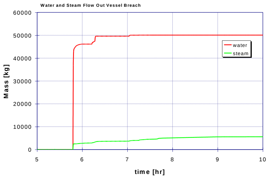
Figure 47: Water and steam escaping through breach in lower head
