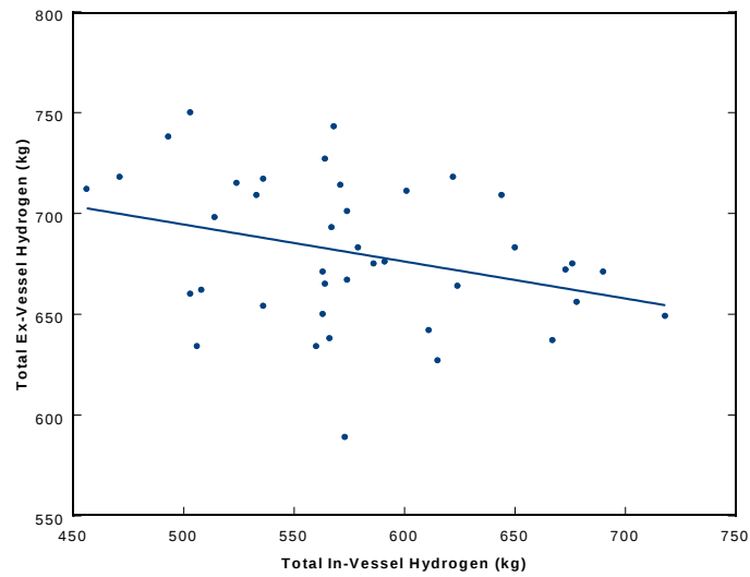
Figure 90: Correlation between in-vessel and ex-vessel hydrogen production
