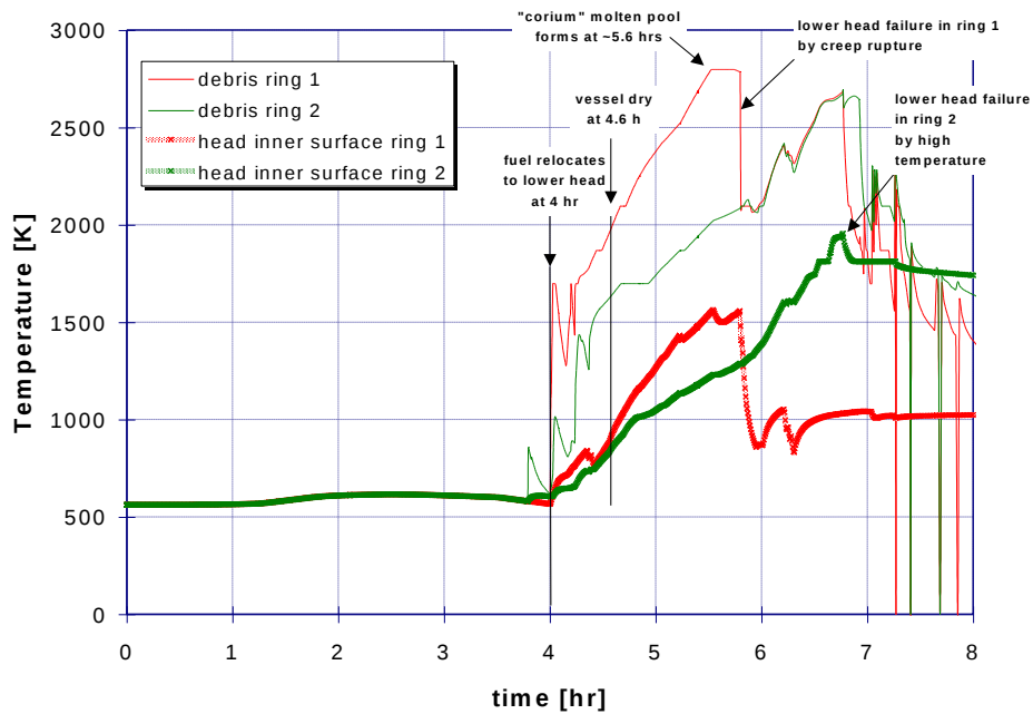
Figure 45: Case 26: Lower head fuel debris and head wall temperatures
