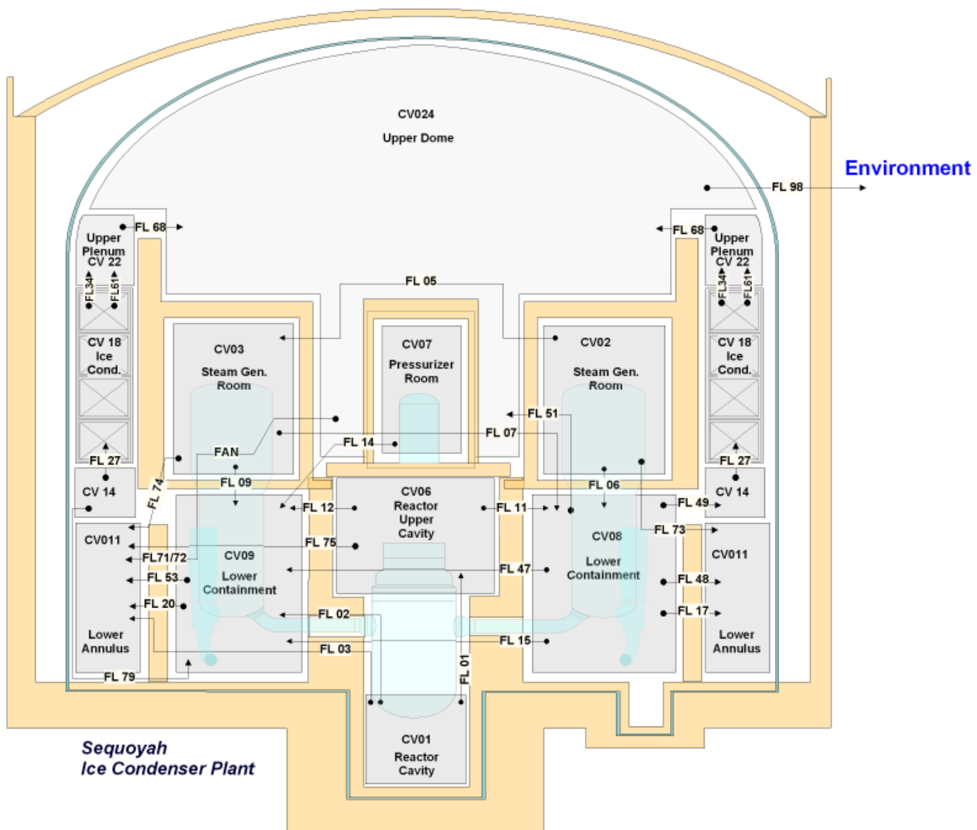
Figure 13: MELCOR 1.8.5 nodalization of the Sequoyah Ice Condenser containment
