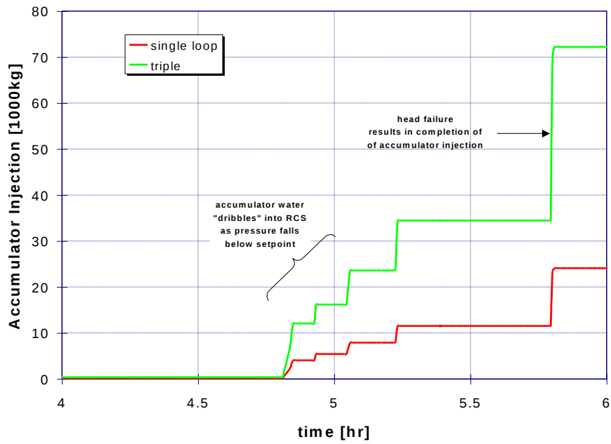
Figure 46: Case 26: Accumulator injection flow
