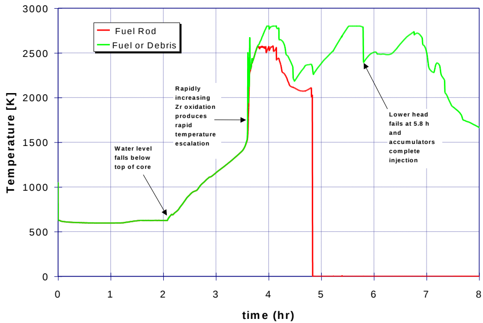
Figure 41: Case 26: Peak core region temperatures - intact fuel rods and fuel debris
