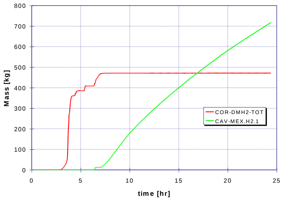
Figure 57: Case 25: Hydrogen produced for case with lower head failure and low hydrogen
