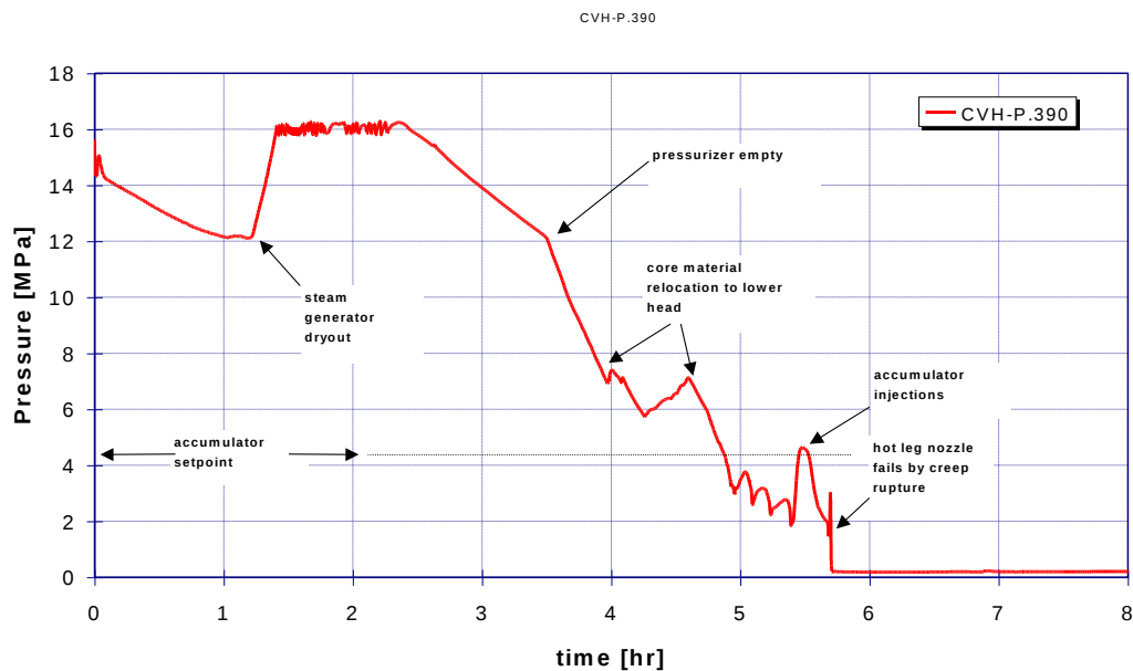
Figure 60: Case 17: Primary system pressure for case with hot leg failure and high hydrogen
