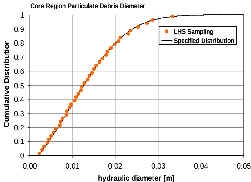
Figure 19: Cumulative probability distribution for core region particulate debris diameter
