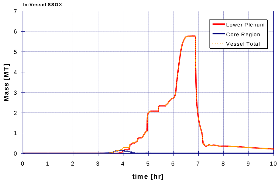
Figure 65: Case 17: Stainless steel oxide inventory in the reactor vessel
