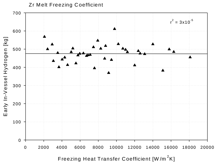
Figure 89: Sensitivity of early-time in-vessel hydrogen production to candling heat transfer coefficient
