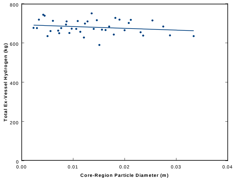
Figure 94: Sensitivity of ex-vessel hydrogen production to core-region particle diameter
