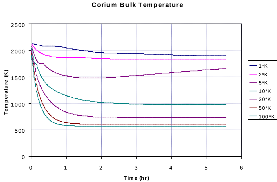
Figure 28: Corium cooling resulting from different values of the conductivity multiplier. The concrete ablation temperature is 1650K
