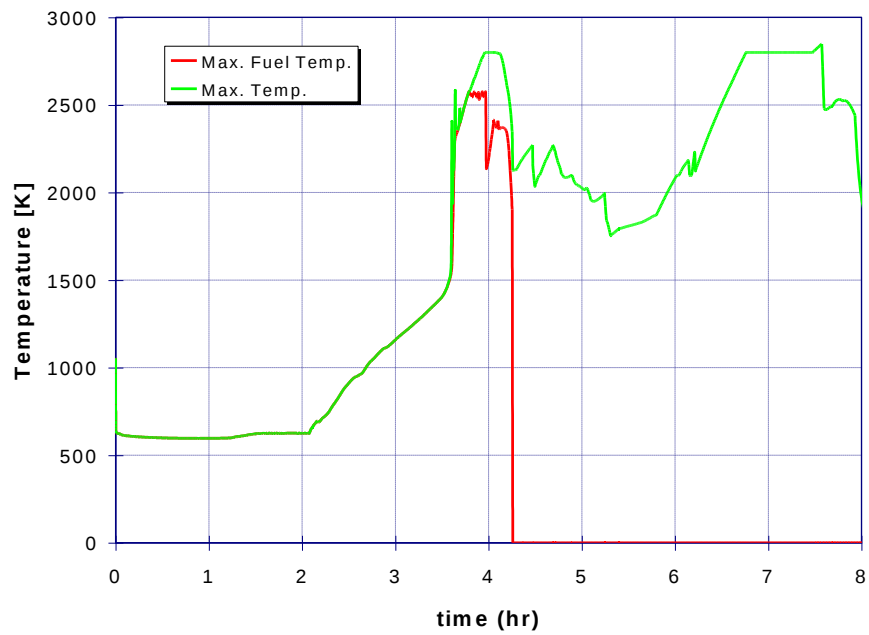
Figure 71: Case 35: Maximum fuel and debris temperature for case with hot leg failure and low hydrogen
