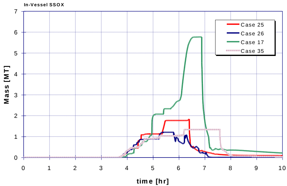
Figure 74: Case 35: Stainless steel oxide for case with hot leg failure and low hydrogen compared with other cases
