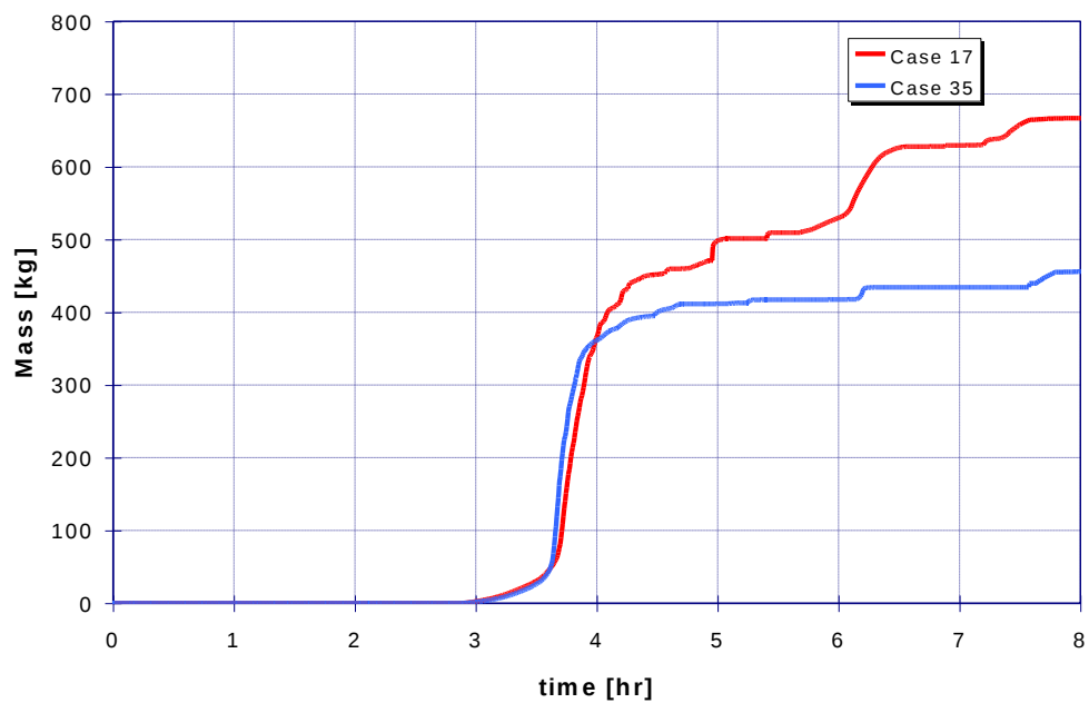
Figure 72: Case 35: In-vessel hydrogen for case with hot leg failure and low hydrogen, compared to Case 17
