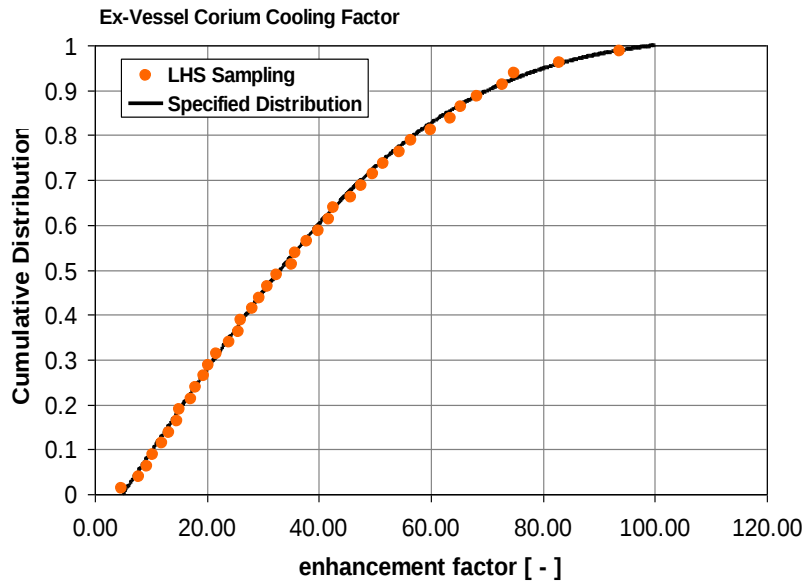
Figure 29: Proposed cumulative distribution for ex-vessel debris cooling
