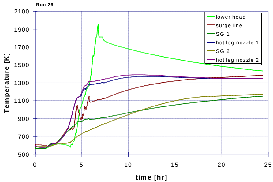
Figure 44: Case 26: Temperatures of potential RCS failure locations
