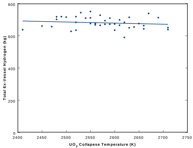
Figure 95: Sensitivity of ex-vessel hydrogen production to UO 2 collapse temperature
