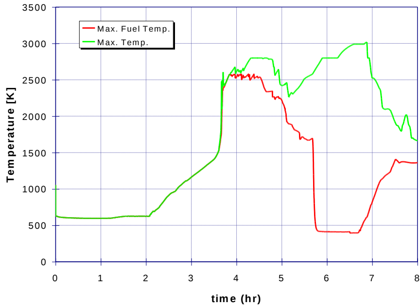
Figure 62: Case 17: Maximum fuel rod and fuel debris temperatures for case with hot leg failure and high hydrogen
