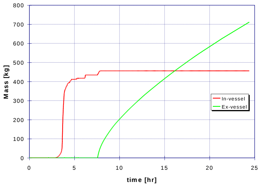
Figure 75: Case 35: Total in-vessel and ex-vessel hydrogen for case with hot leg failure and low hydrogen
