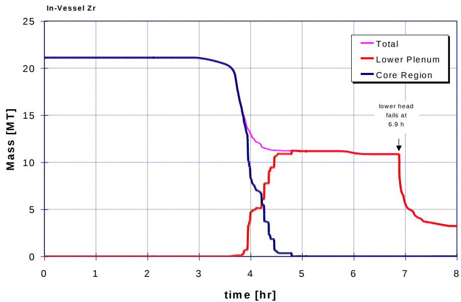
Figure 64: Case 17: Unoxidized in-vessel Zr for case with hot leg failure and high hydrogen
