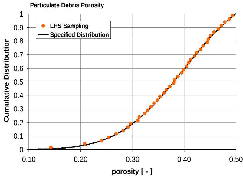
Figure 21: Cumulative distribution for debris porosity
