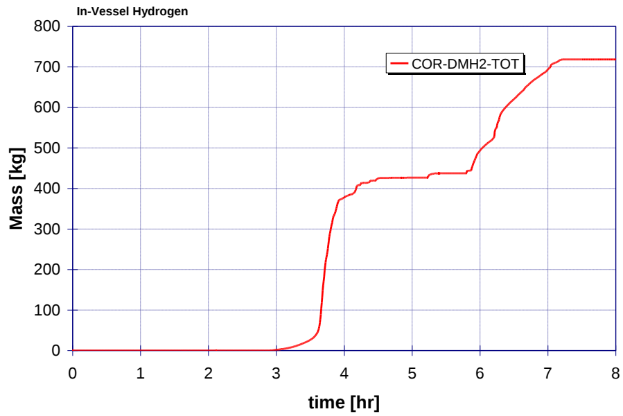
Figure 42: Case 26: In-vessel hydrogen production
