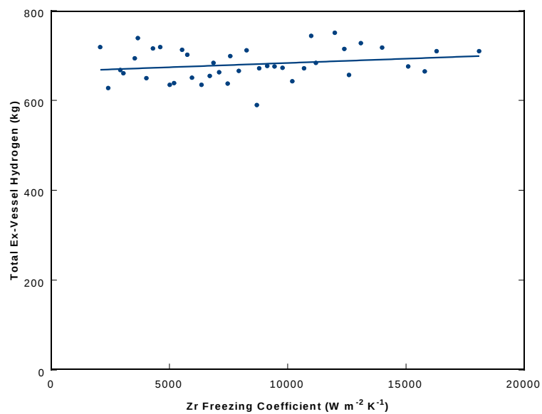
Figure 93: Sensitivity of ex-vessel hydrogen production to candling heat transfer coefficient
