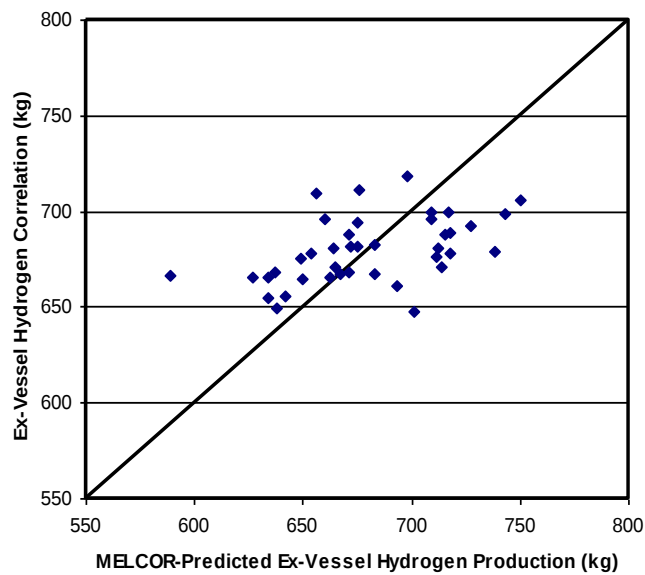
Figure 80: Comparison between MELCOR-predicted and correlated ex-vessel hydrogen production
