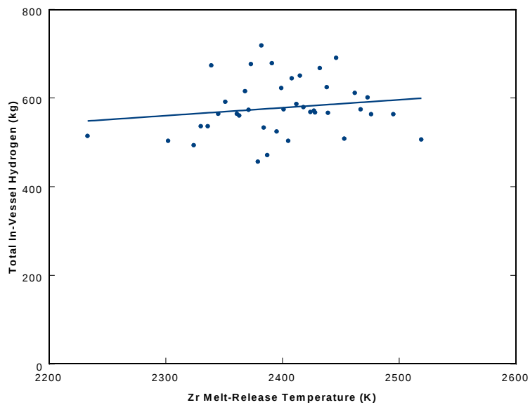
Figure 83: Sensitivity of total in-vessel hydrogen production to zirconium melt-release temperature
