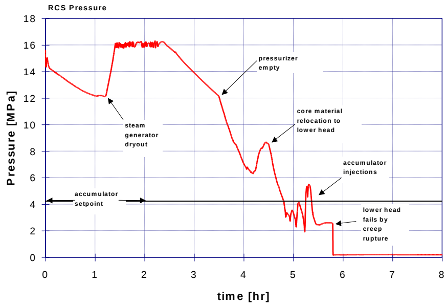
Figure 38: Case 26: Primary system pressure
