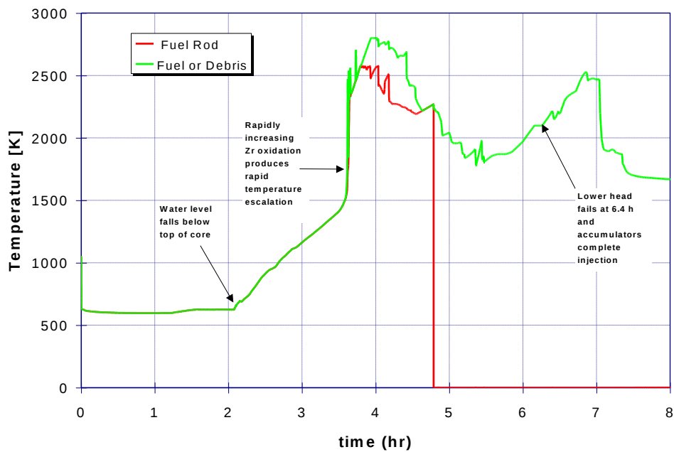
Figure 54: Case 25: Peak fuel rod and debris temperatures for case with lower head failure and low hydrogen
