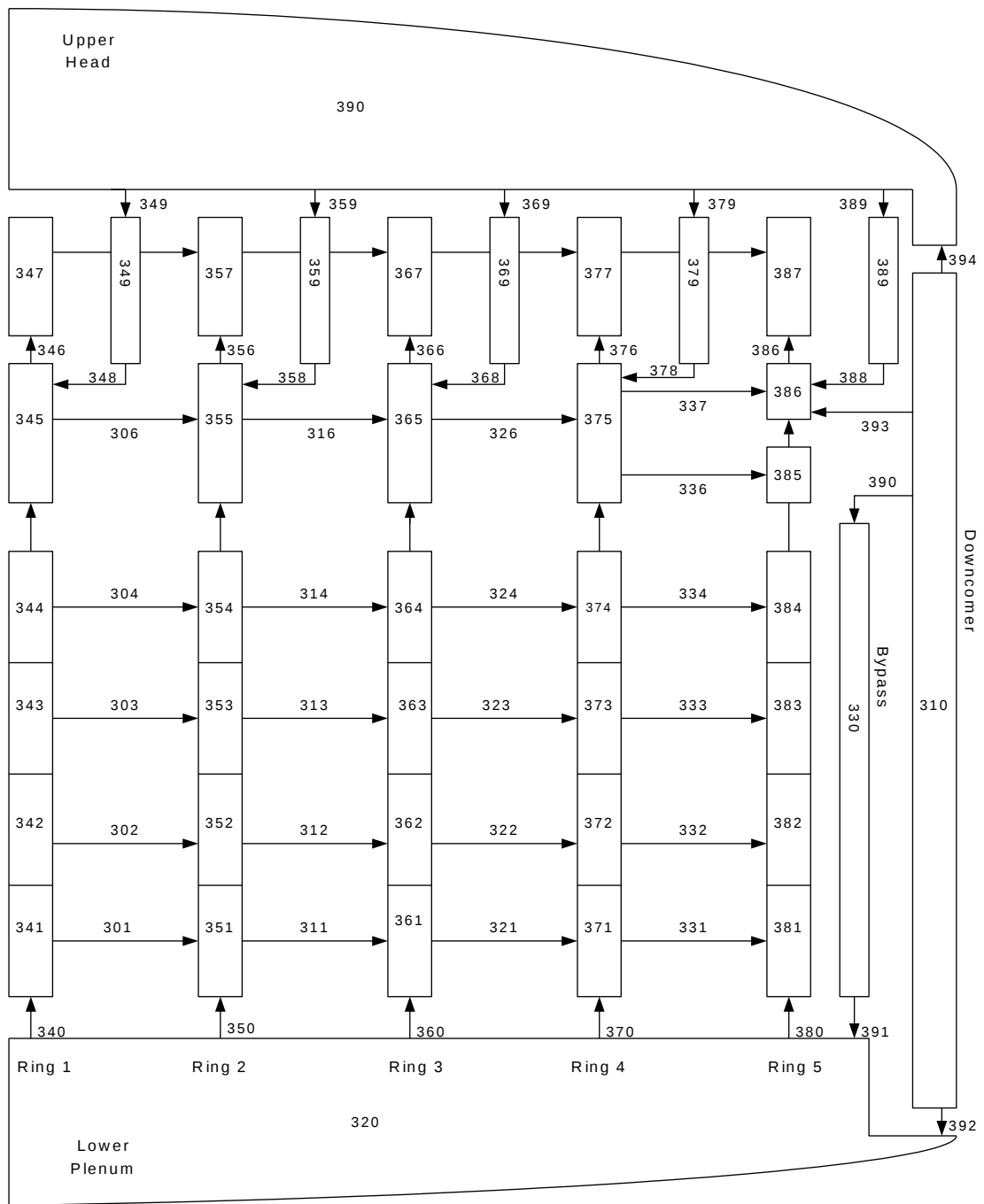
Figure 3: Reactor vessel CVH nodalization used in the Westinghouse Sequoyah model
