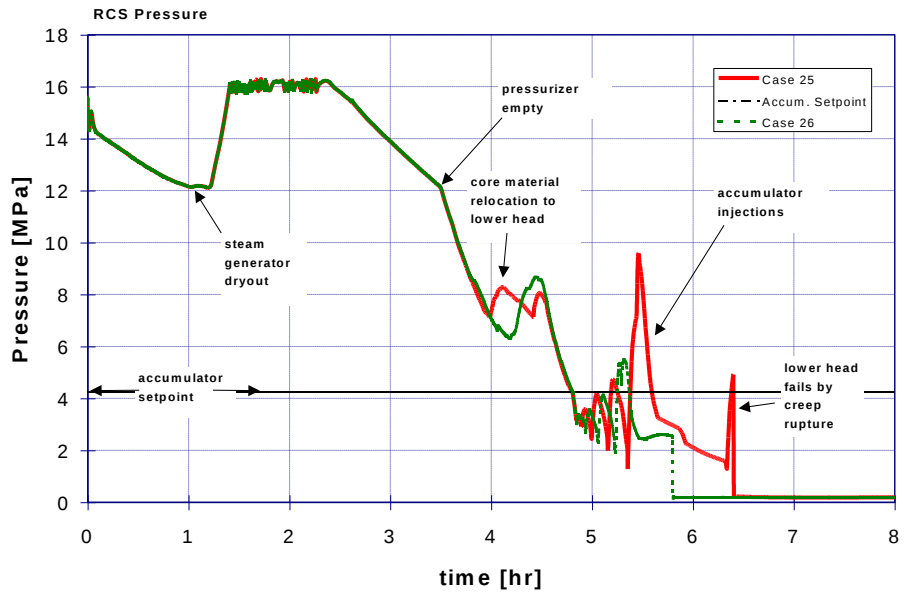
Figure 52: Case 25: RCS pressure for case with lower head failure and low hydrogen
