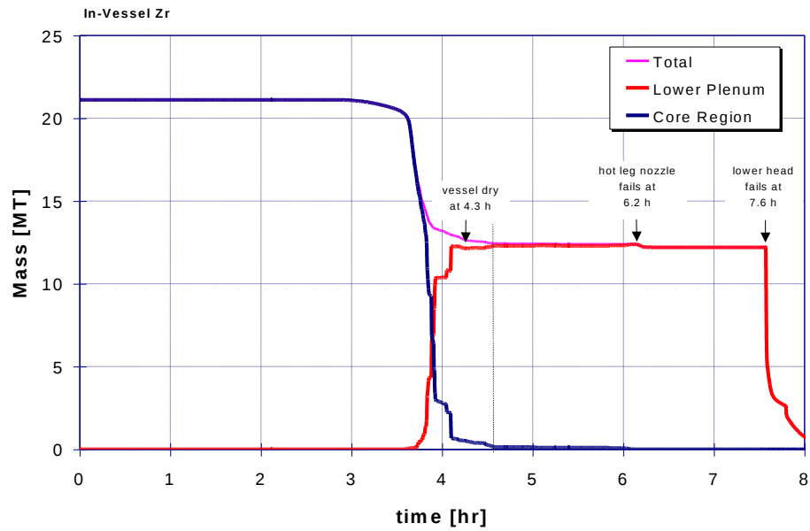
Figure 73: Case 35: Unoxidized in-vessel Zr for case with hot leg failure and low hydrogen
