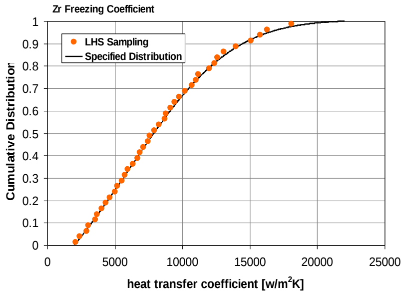
Figure 18: Cumulative distribution proposed for the candling heat transfer coefficient
