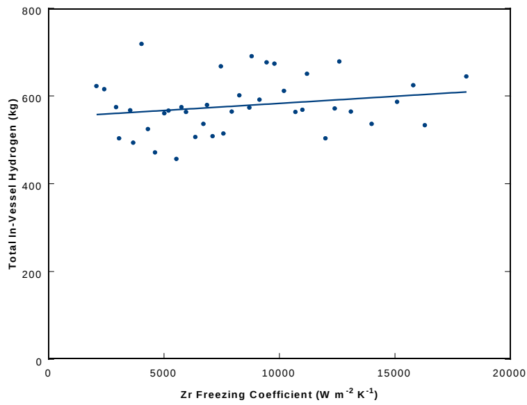
Figure 88: Sensitivity of total in-vessel hydrogen production to candling heat transfer coefficient
