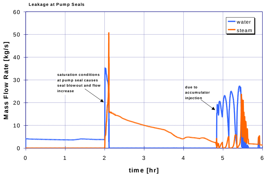
Figure 51: Case 25: Pump seal leakage for case with lower head failure and low hydrogen
