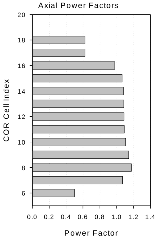
Figure 2: Axial power distribution for the Sequoyah core
