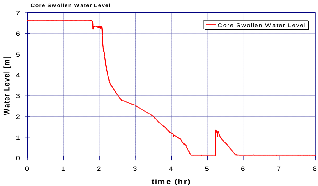
Figure 39: Case 26: Reactor core water level
