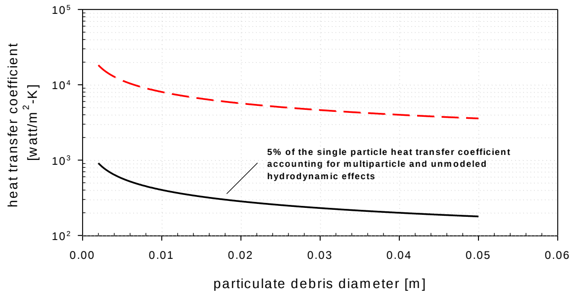
Figure 22 Heat transfer coefficient recommended to be associated with particulate debris diameter
