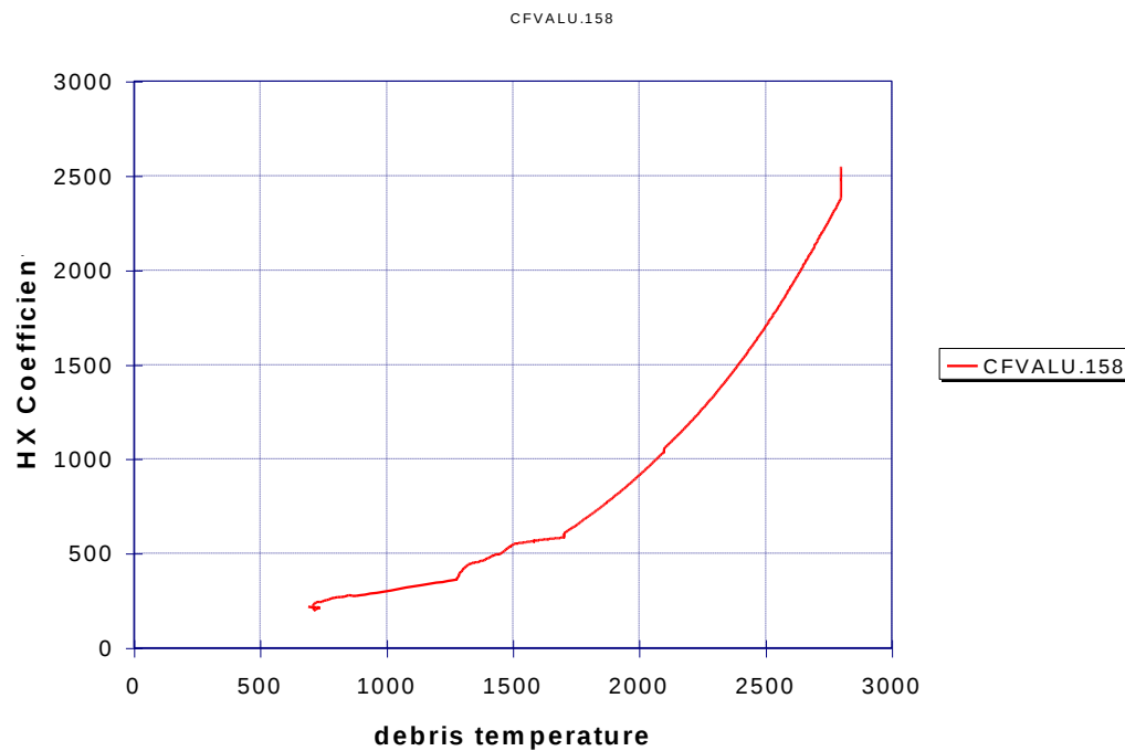
Figure 9: Debris to lower head heat transfer coefficient predicted by MELCOR control function
