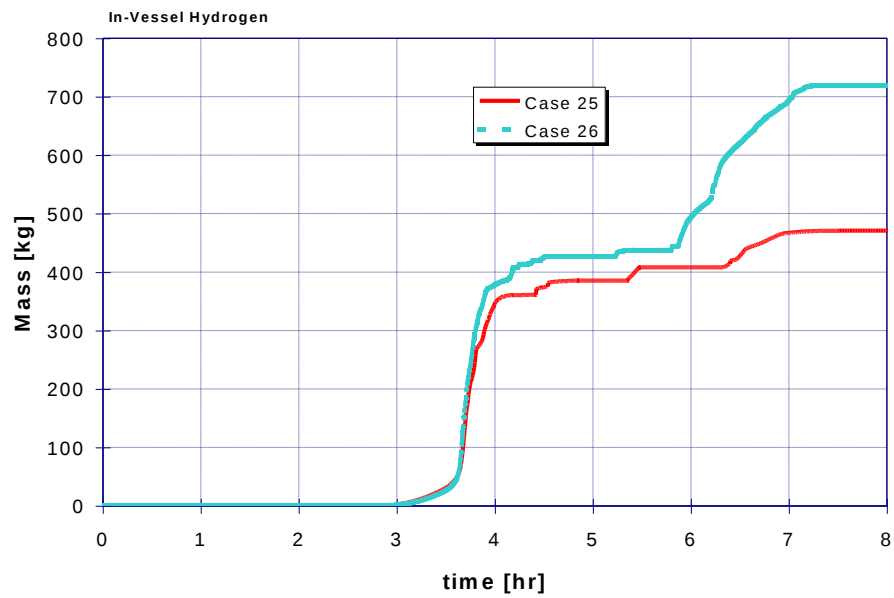
Figure 56: In-vessel hydrogen produced for Case 25 and Case 26
