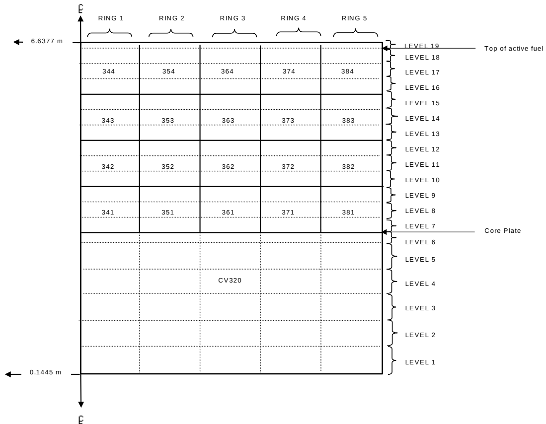
Figure 1: Core nodalization used in the Westinghouse Sequoyah MELCOR model
