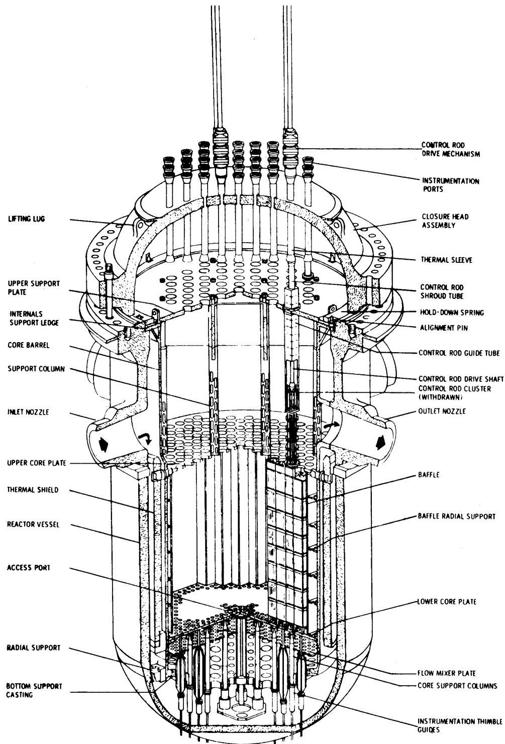
Figure 4: Westinghouse PWR Reactor Vessel Internals
