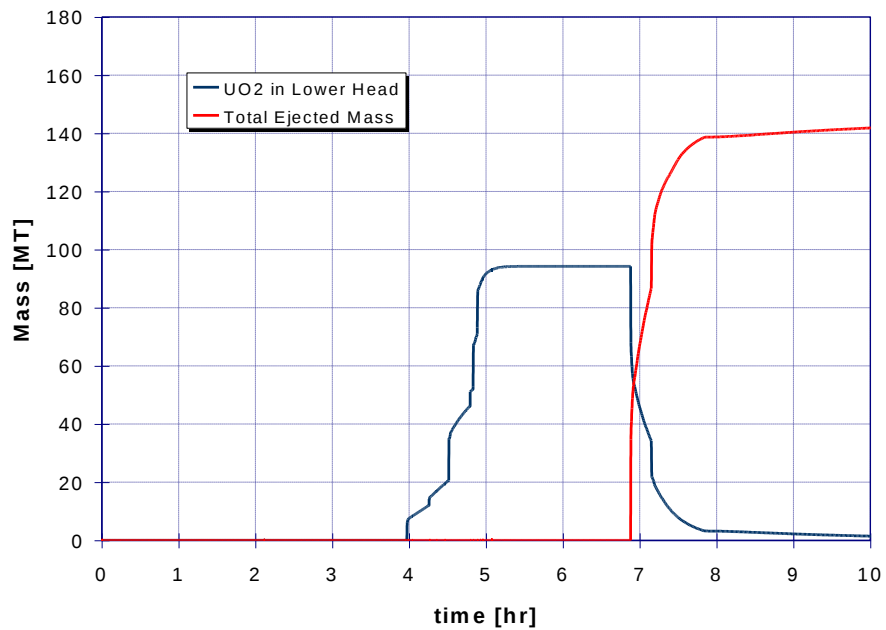
Figure 66: Case 17: Lower head debris and cavity debris for case with hot leg failure and high hydrogen
