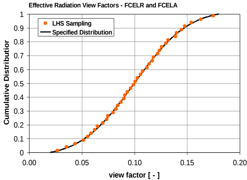
Figure 24: Proposed cumulative distribution of COR radiative view factors FCELA and FCELR
