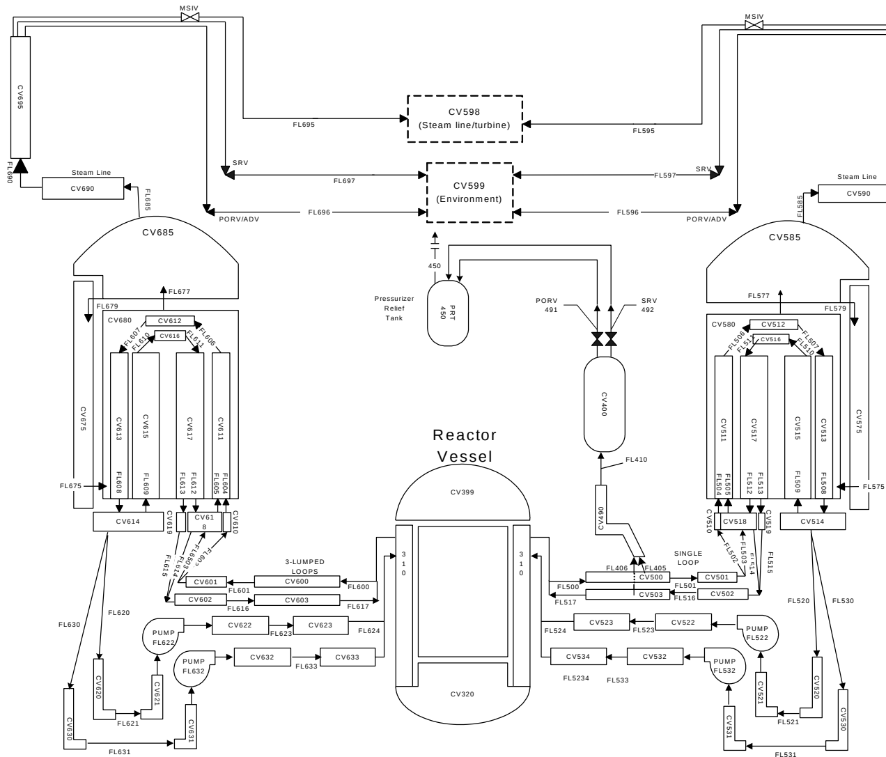
Figure 12: Nodalization of Westinghouse 4-loop PWR reactor coolant system used in the Sequoyah MELCOR model
