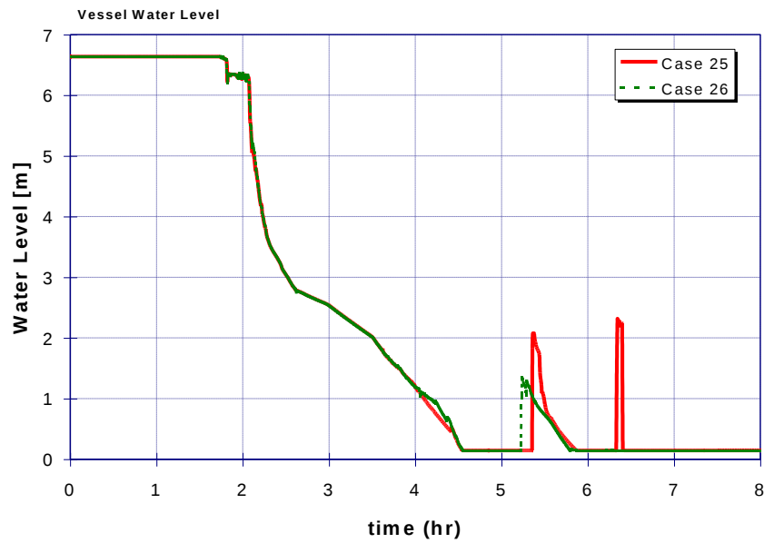
Figure 53: Case 25: Vessel water level for case with lower head failure and low hydrogen
