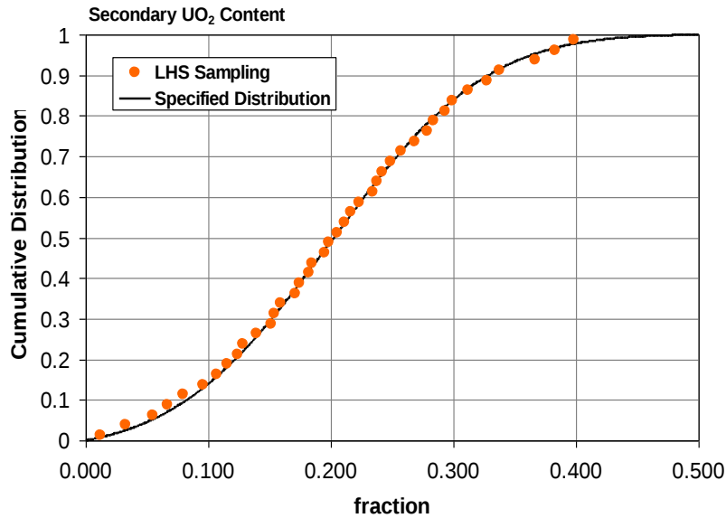
Figure 17: Cumulative probability distribution describing dissolved UO 2
