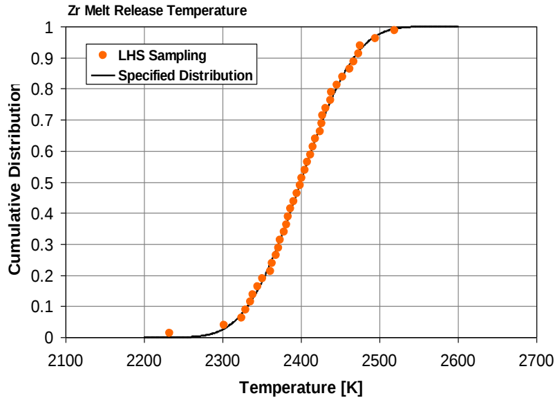
Figure 15: Cumulative probability distribution for molten zircaloy breakout temperature
