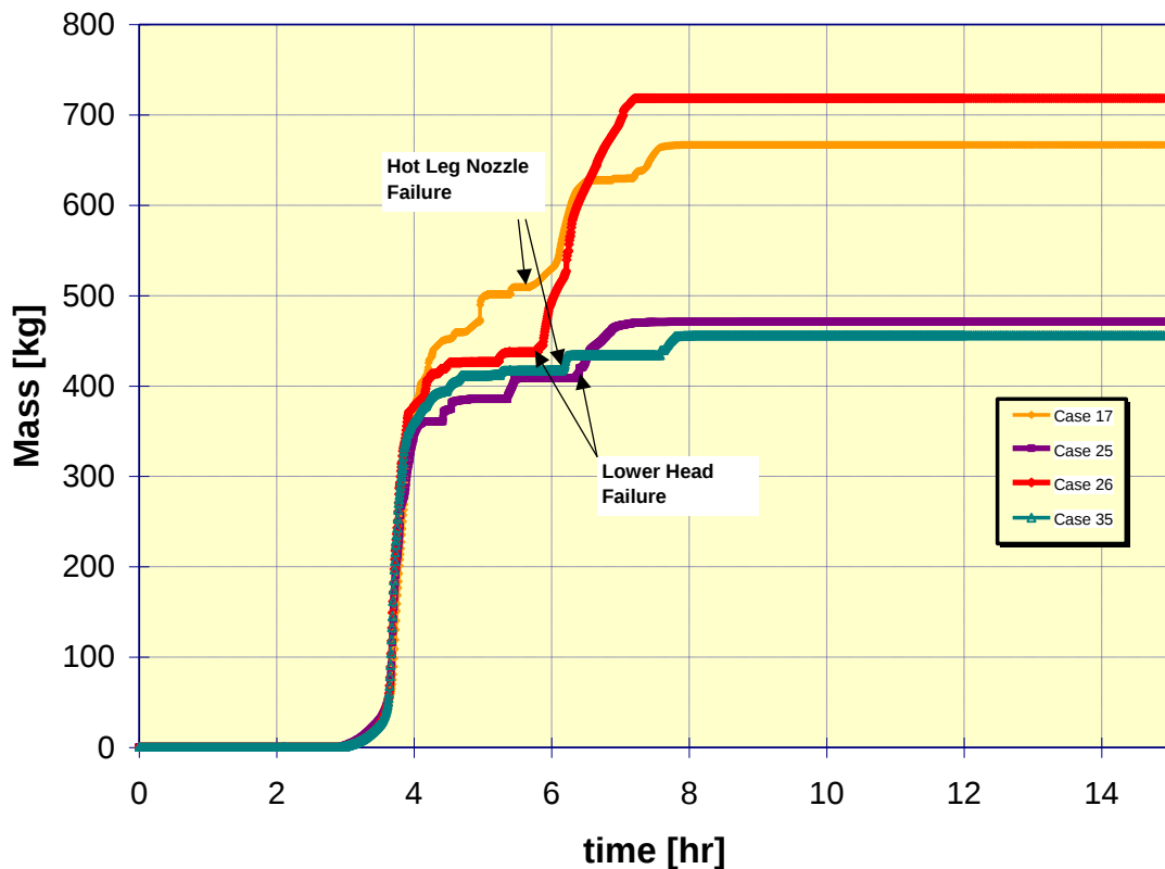
Figure 35: In-vessel hydrogen produced in high and low bounding calculations for both hot leg nozzle and lower head failures
