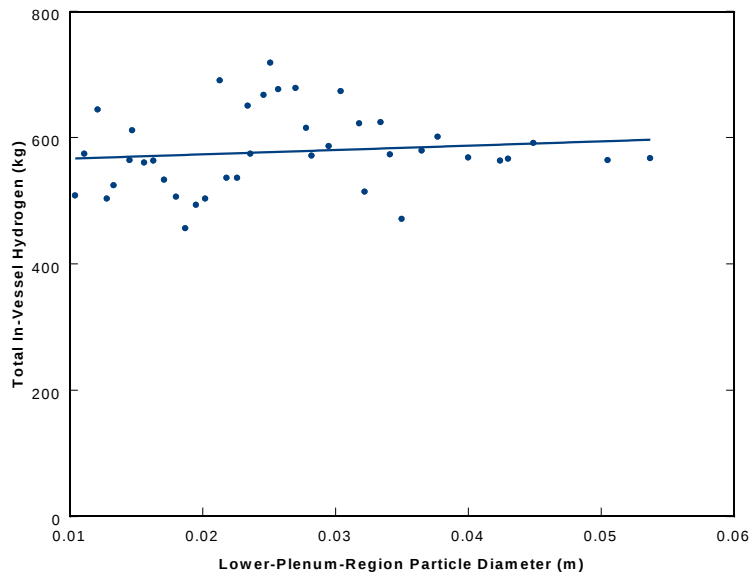
Figure 85: Sensitivity of total in-vessel hydrogen production to debris particle size in the lower plenum
