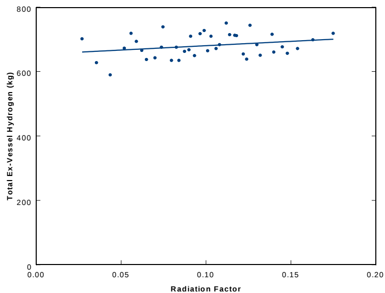
Figure 92: Sensitivity of ex-vessel hydrogen production to radiation factor between adjacent fuel rings
