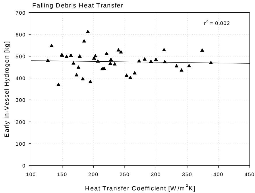
Figure 82: Sensitivity of early-time in-vessel hydrogen production to falling-debris heat-transfer coefficient in the lower plenum
