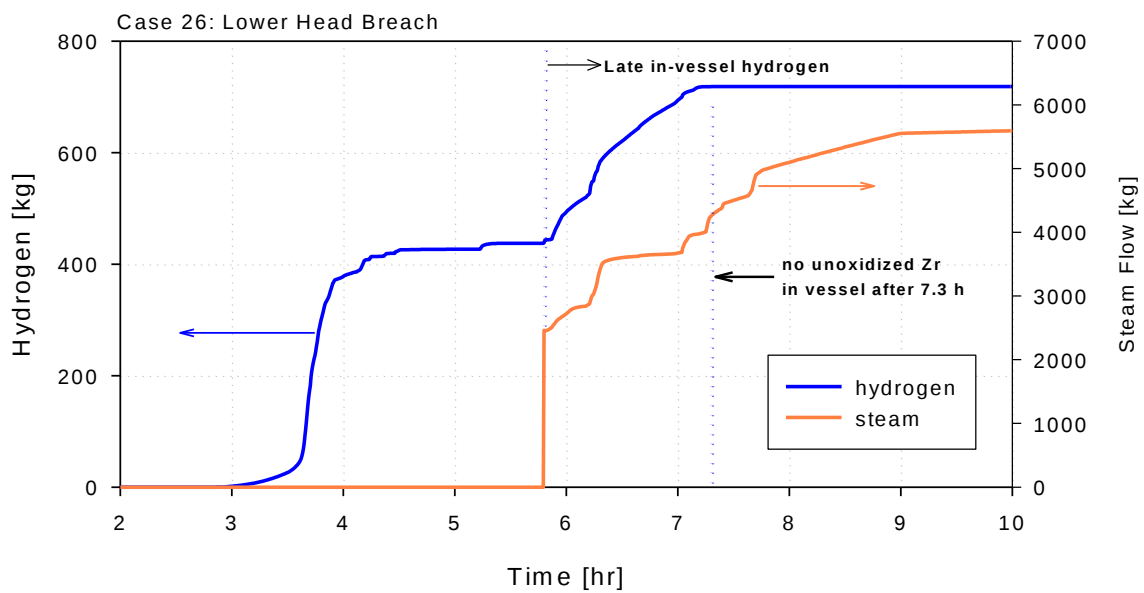
Figure 58: In-vessel hydrogen produced and break steam flow for Case 26 with high late-time in-vessel hydrogen
