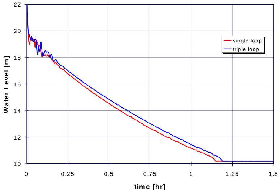
Figure 37: Case 26: Steam generator water level
