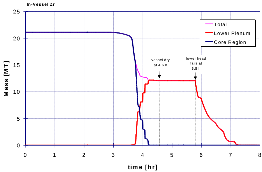
Figure 48: Case 26: Zr inventory in-vessel
