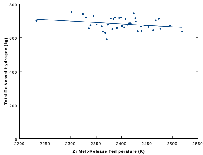
Figure 91: Sensitivity of ex-vessel hydrogen production to zirconium melt-release temperature
