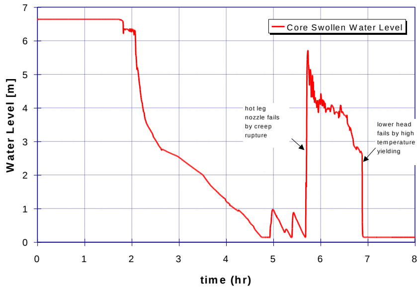
Figure 61: Case 17: Vessel water level for case with hot leg failure and high hydrogen
