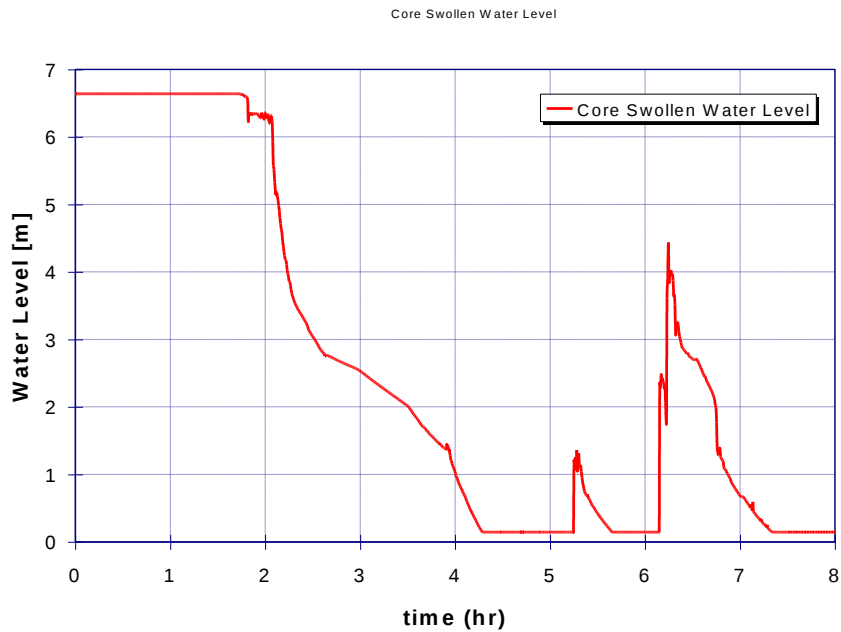
Figure 70: Case 35: Vessel water level for case with hot leg failure and low hydrogen
