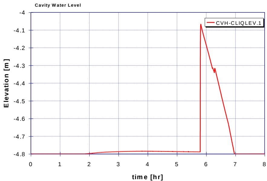
Figure 49: Case 26: Water level in the reactor cavity
