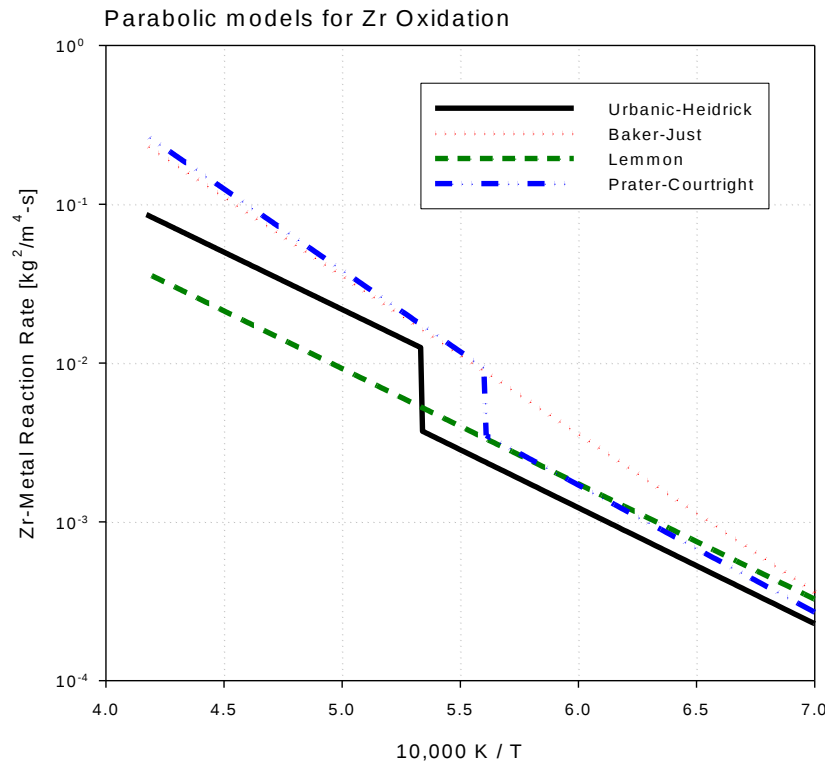
Figure 14: Comparison of different parabolic rate models representing zircaloy oxidation in steam
