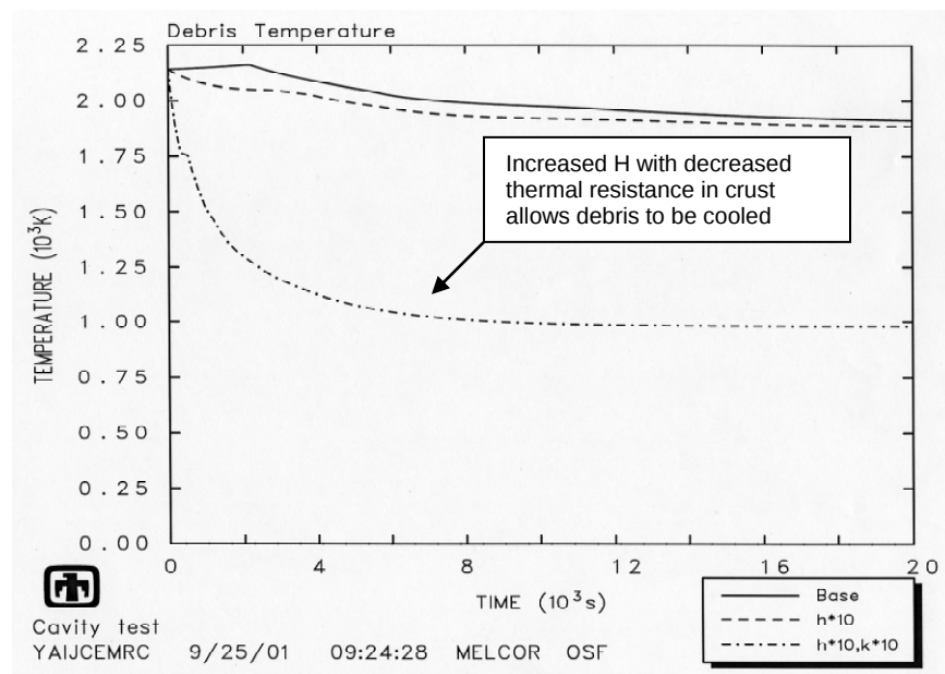
Figure 25: Predicted cavity debris temperature for default and modified CORCON analysis of MCCI in a Sequoyah cavity
