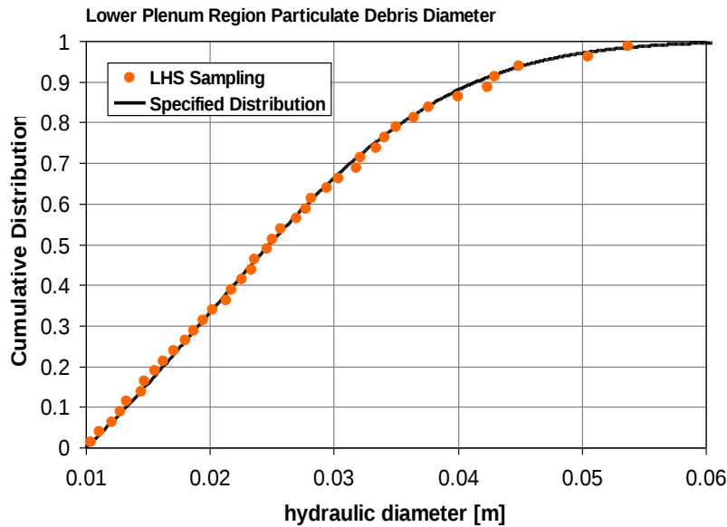
Figure 20: Cumulative probability distribution for lower plenum region particulate debris diameter
