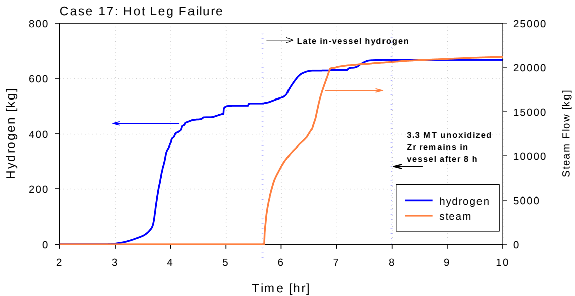
Figure 76: In-vessel hydrogen produced and break steam flow for case with high late-time in-vessel hydrogen for case with hot leg failure and high hydrogen
