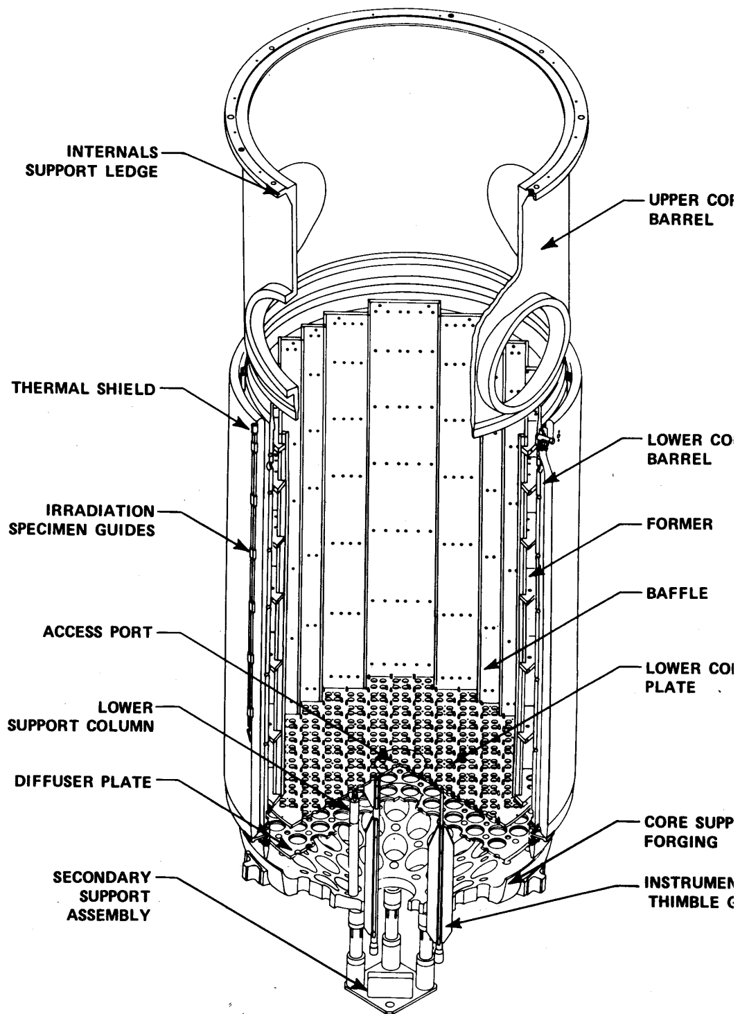
Figure 5: Westinghouse PWR Lower Support Structure
