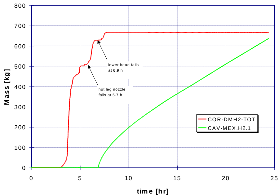
Figure 68: Case 17: In-vessel and ex-vessel hydrogen generation for case with hot leg failure and high hydrogen
