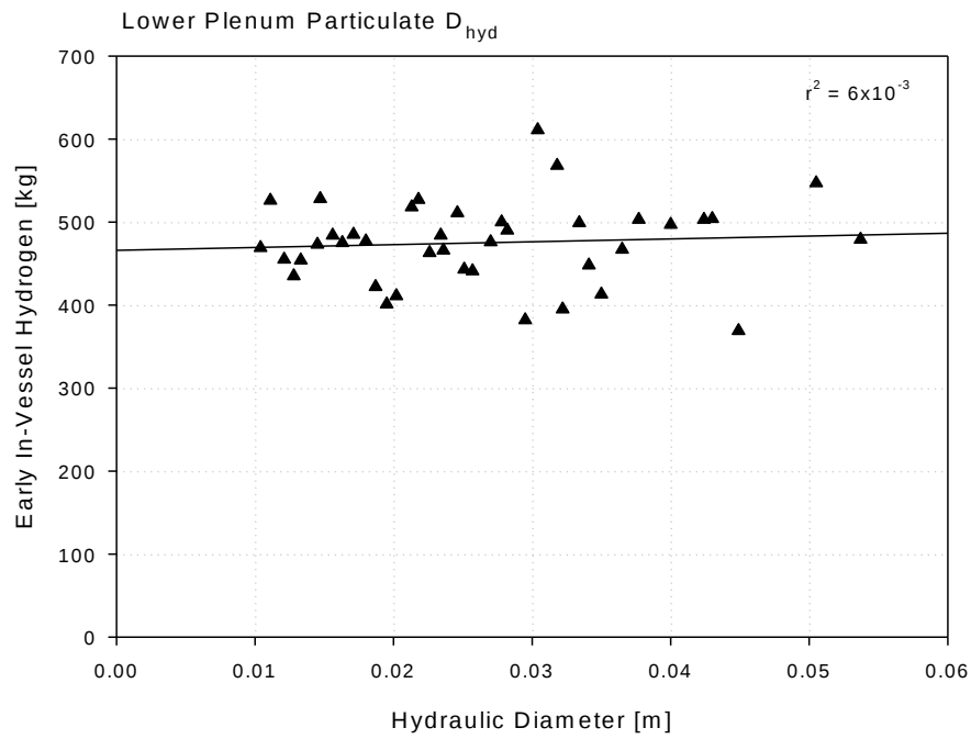
Figure 86: Sensitivity of early-time in-vessel hydrogen production to debris particle size in the lower plenum
