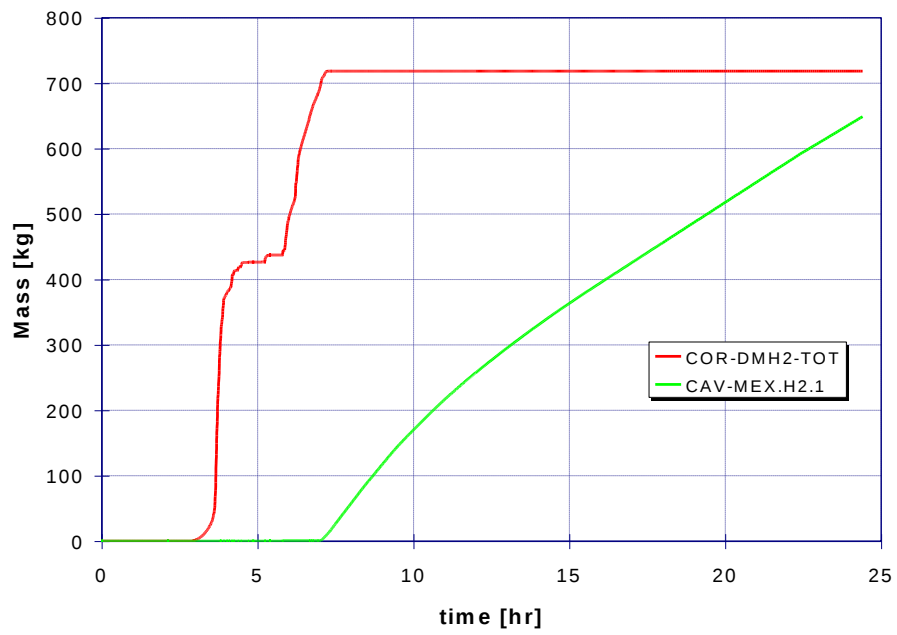
Figure 50: Case 26: In-vessel and ex-vessel hydrogen production
