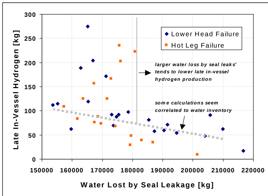
Figure 78: Correlation between late in-vessel hydrogen and RCS water loss via pump seals
