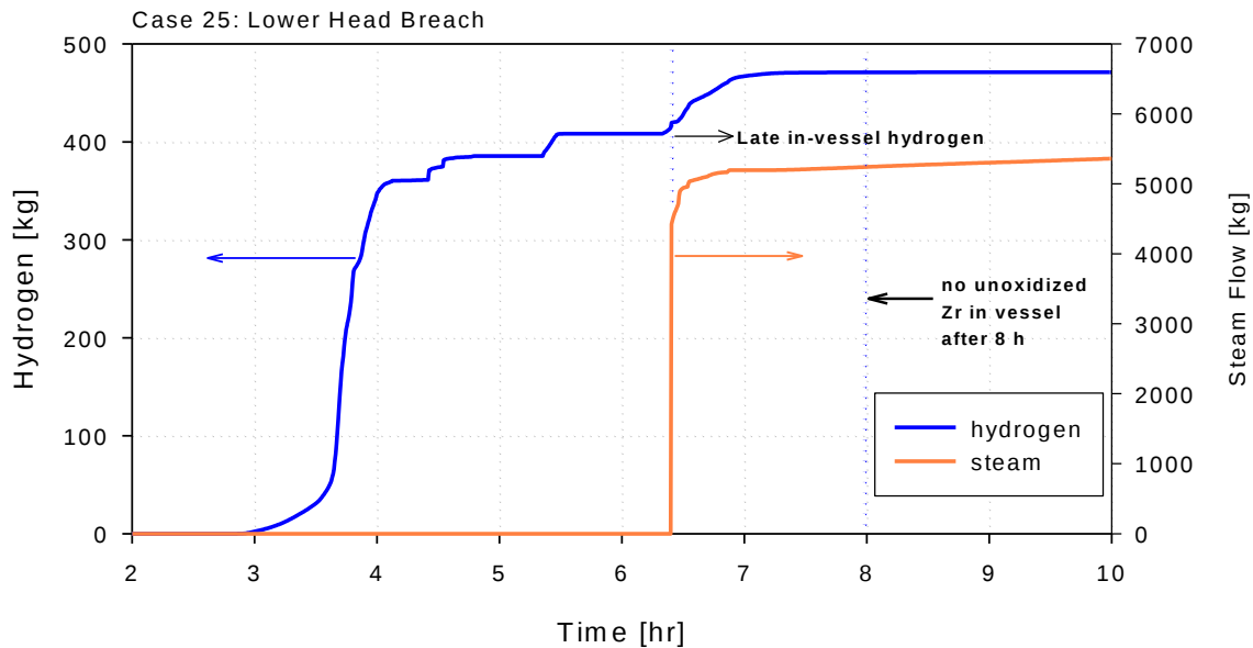
Figure 59: In-vessel hydrogen produced and break steam flow for Case 25 with low late-time in-vessel hydrogen
