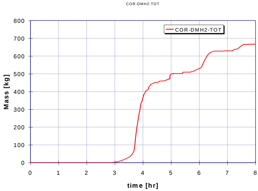
Figure 63: Case 17: In-vessel hydrogen for case with hot leg failure and high hydrogen
