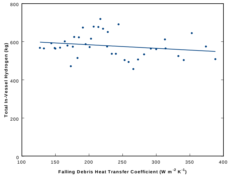
Figure 81: Sensitivity of total in-vessel hydrogen production to falling-debris heat-transfer coefficient in the lower plenum
