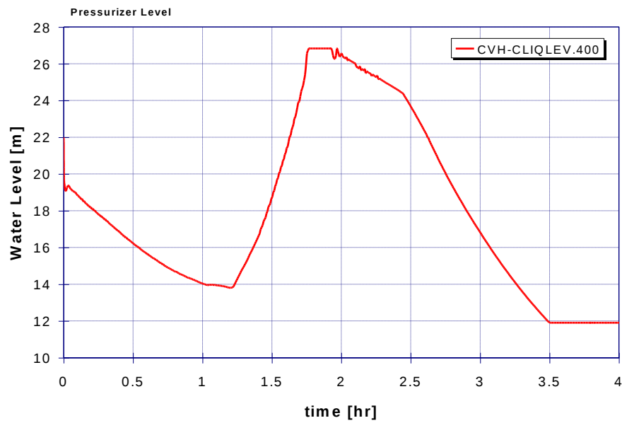
Figure 40: Case 26: Pressurizer water level
