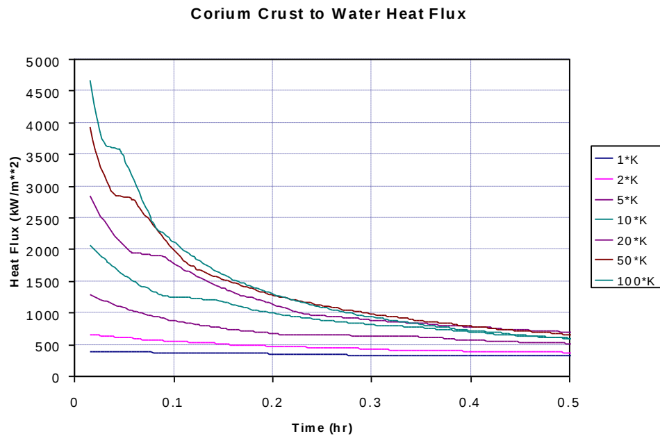
Figure 27: Heat rejection for different values of the conductivity multiplier
