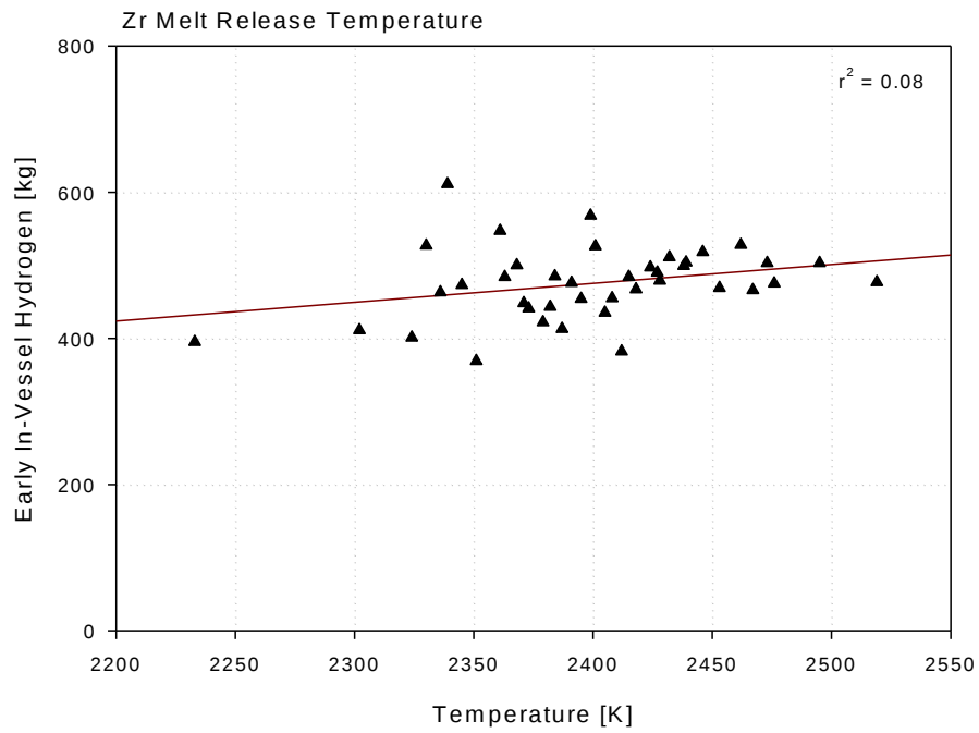
Figure 84: Sensitivity of early-time in-vessel hydrogen production to zirconium melt-release temperature
