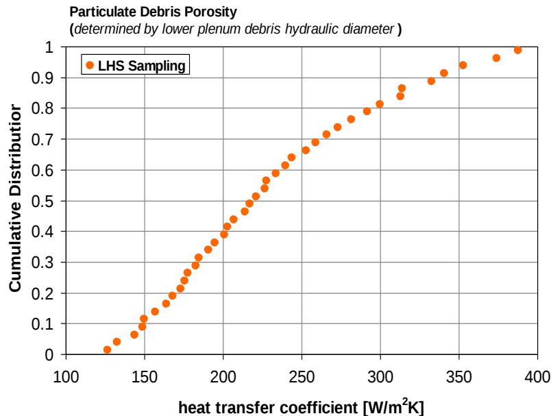
Figure 23: Cumulative distribution proposed for falling debris heat transfer coefficient
