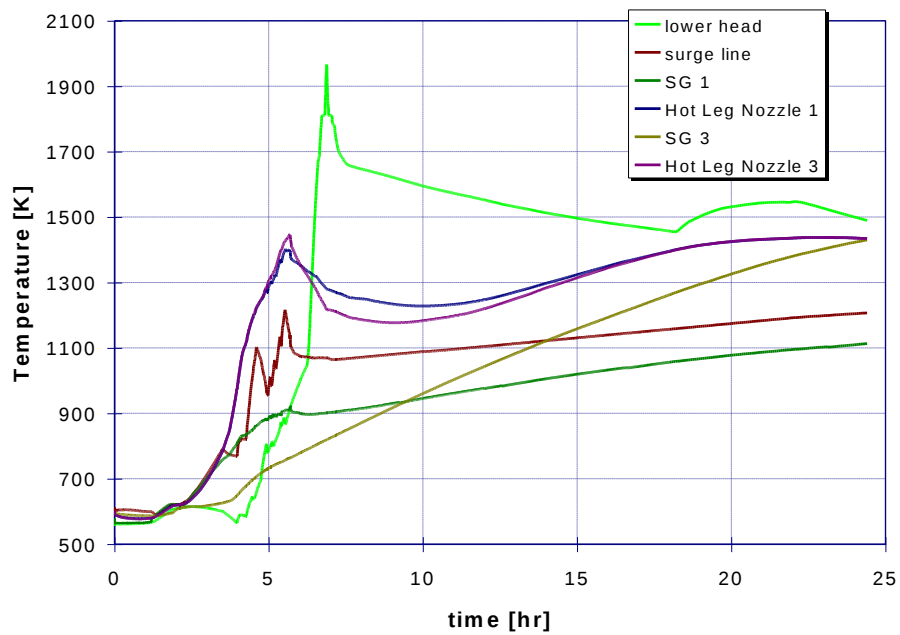
Figure 67: Case 17: Temperatures of potential RCS failure locations for case with hot leg failure and high hydrogen
