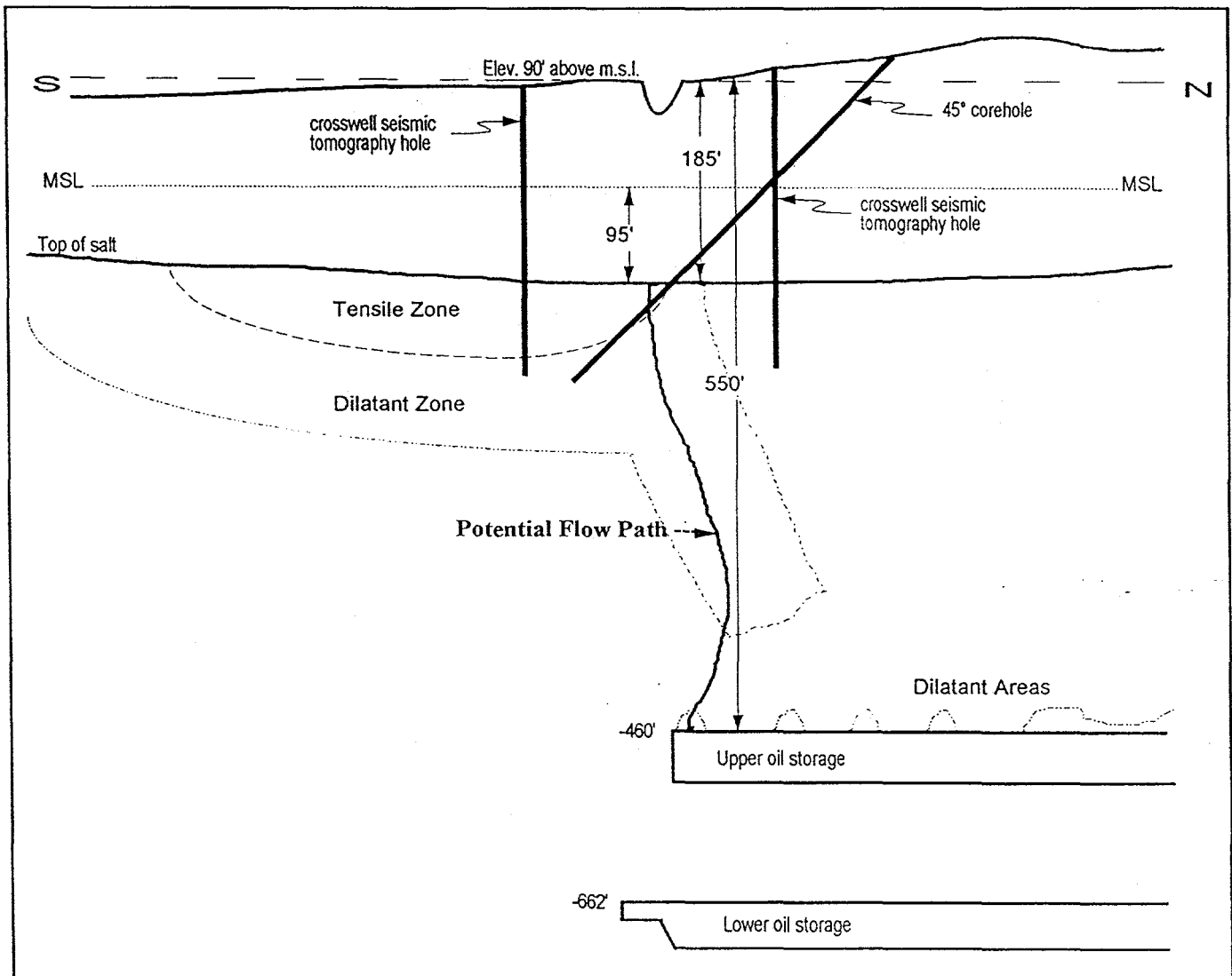
Figure 4 Geomechanical modeling by Ehgartner (1993) showed mechanism for crack development in tension zone that would develop over mined openings after a number of years, and progressing through weakened dilatant zone. Based largely on these modeling results, crosswell tomography was conducted and angled boreholes were planned to intersect such features.
