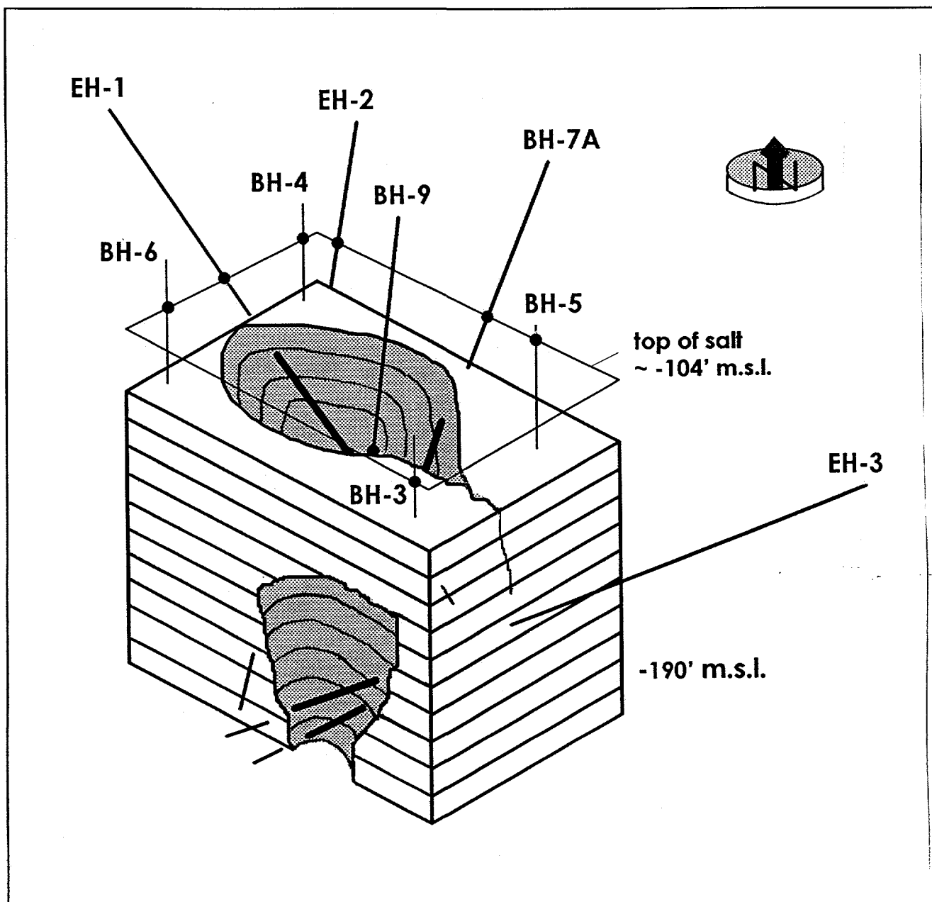
Figure 2 Diagrammatic representation of exploratory drilling and geometry of Sinkhole #1 throat. Boreholes BH-3, 4, 5, and 6 were drilled for crosswell seismic tomography; slantbores BH-7A and 9 were drilled for throat definition. EH-1, 2, and 3 further defined the throat and provided decisive information regarding grouting potential. Accentuated portions of boreholes define throat penetrations.
