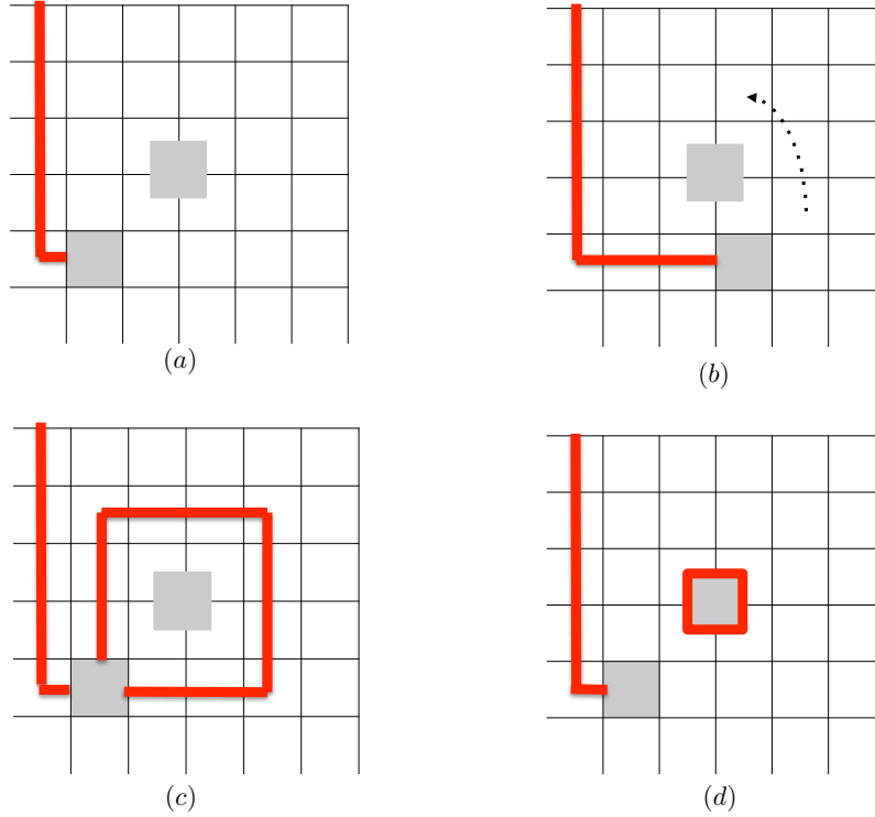
Figure 3: A Hamiltonian in which some terms are inactive (gray) in (a) is adiabatically evolved through a sequence of Hamiltonians in which other terms are turned off (b-d). The net effect is an encoded logical operation on the groundspace of the system.
