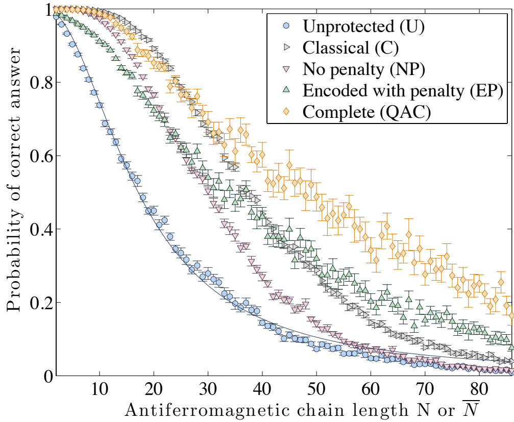
Figure 2: The impact of various error-correction strategies on a D-Wave processor computing the ground state of an antiferromagnetic spin chain. Taken from Pudenz et al. , Nature Comm. 5, 3243 (2014).
