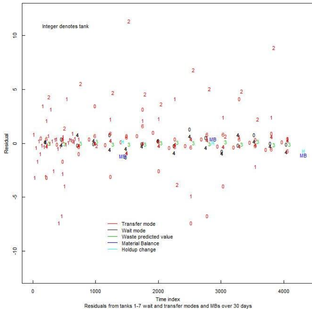
Figure 8. Residuals from PM and NMA for the 7-tank MBA in an aqueous facility. The PM residuals occur at the end of each wait event and after each transfer event. The NMA residuals are the usual MBs every 10 days.
