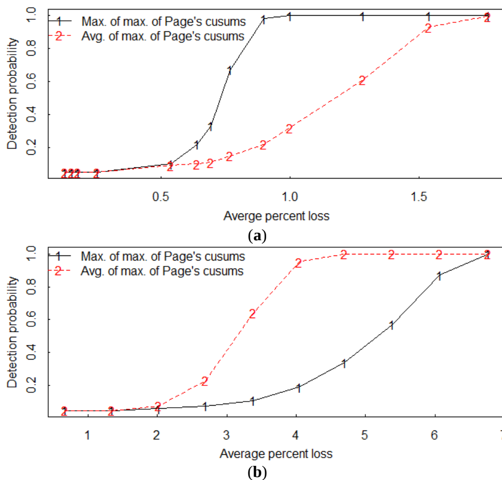
Figure 11. Example estimated detection probabilities versus the average percent loss in a (a) local loss from the input and in a (b) non-local (widespread) loss from all 13 residual streams. The average is over all 13 residual streams during the one-time-step duration of the loss.
