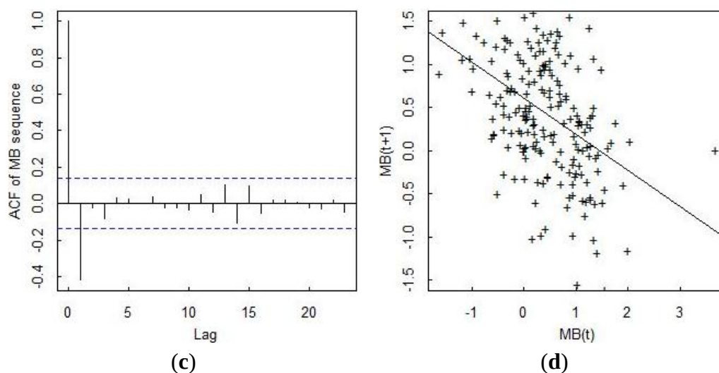
Figure 5. Daily material balances (“batches”) in (a); the estimated probability density of the MB value in (b); the autocorrelation function of the MB sequence in (c); and a lagged plot of the present MB versus the previous MB in (d).
