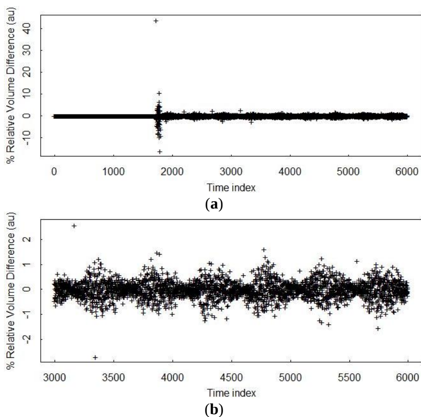
Figure 2. Illustration of synchronization error in an aqueous tank modeled in the System Performance Model (SPM). In (a), the synchronization error is present but a large volume residual occurred at the beginning of material flow near minute 1700 so synchronization errors are almost not visible. In (b), a relatively short section of time is plotted, and synchronization error is approximately a -1 to 2 percent effect (in arbitrary units, au, because this is percent relative change).
