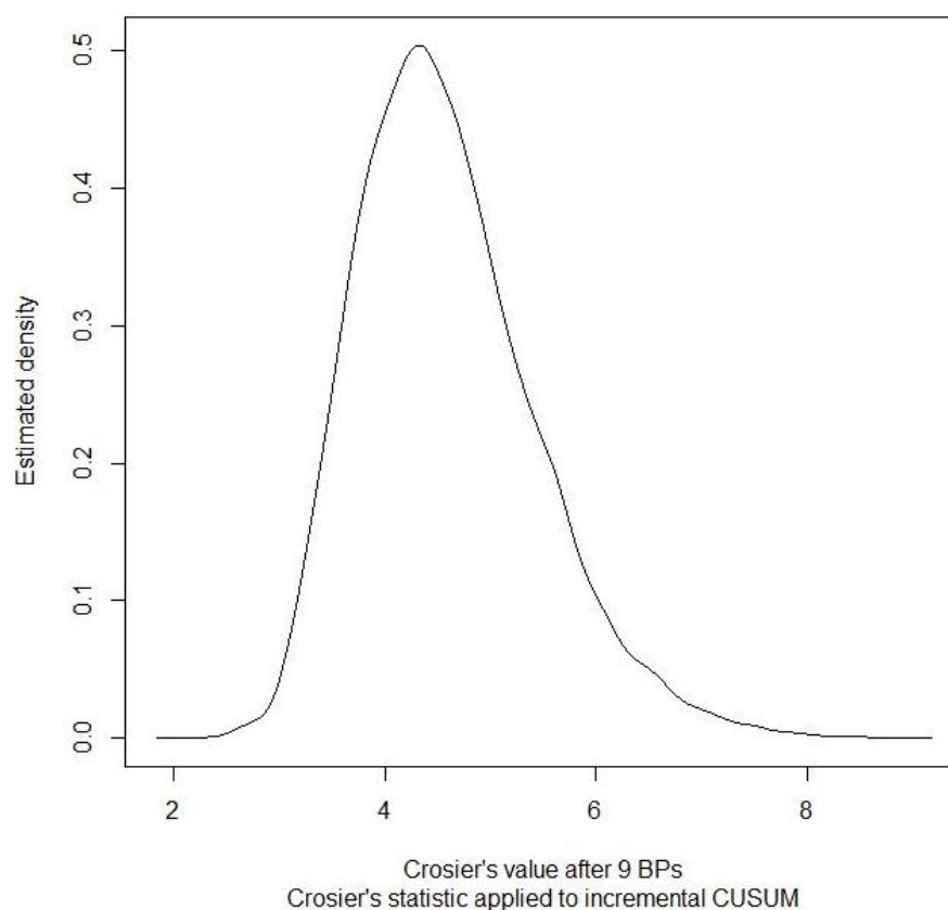
Figure 10. Example of the estimated probability density of Crosier's statistic applied to incremental CUSUMs in the 2-part hybrid at BP 9. The data is simulated from the SPM of an electrochemical facility.
