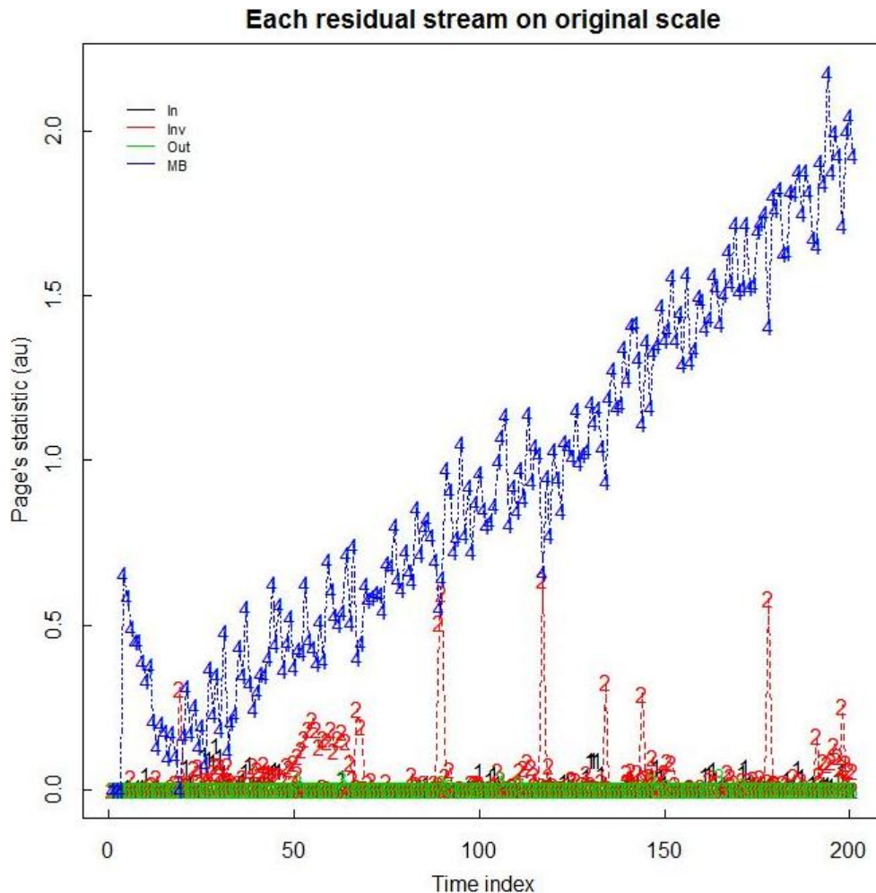
Figure 9. Page's cusum test applied to each of the 14 (13 PM, one NMA) residual streams. To avoid cluttering the figure, only some residual streams are shown, as indicated.
