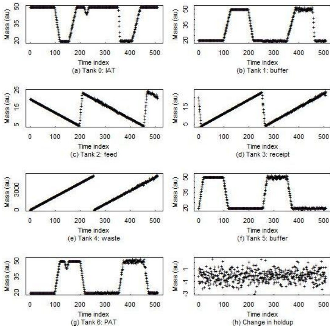
Figure 7. Example data from a 7-tank aqueous facility MBA. Some tanks are batch input, batch output (denoted B/B). Tanks that are just upstream or downstream from a separations vessel have a continuous (C) mode. (a) Input accountability tank; (b) Buffer tank; (c) Feed tank; (d) Receipt tank; (e) Waste tank; (f) Buffer tank; (g) Output accountability tank; (h) Change in holdup.
