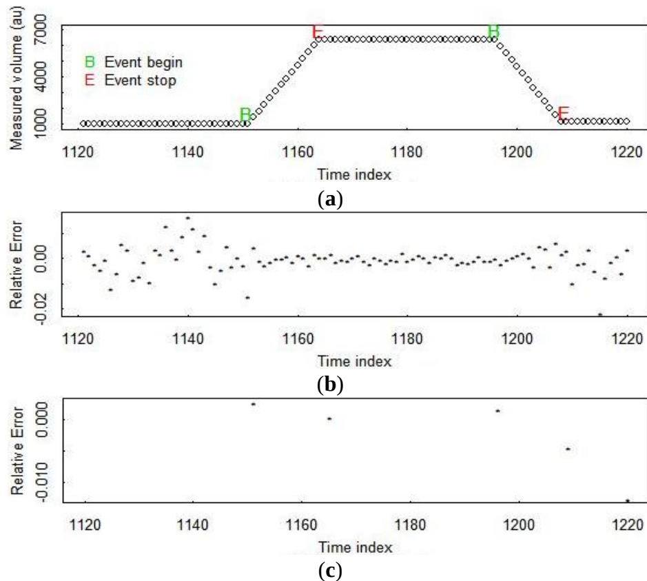
Figure 3. (a) The measured volume in a tank during a receive, wait, ship cycle; (b) PM residuals for bulk volume using option 1 PM; (c) PM residuals for bulk volume using option 2 PM. In PM option 1, residuals are generated on a fixed time schedule. In PM option 2, residuals are generated at the end of each “wait” and “transfer” mode, and transfer-mode residuals compare the bulk volume change in the shipper tank to the corresponding change in the receiver tank.
