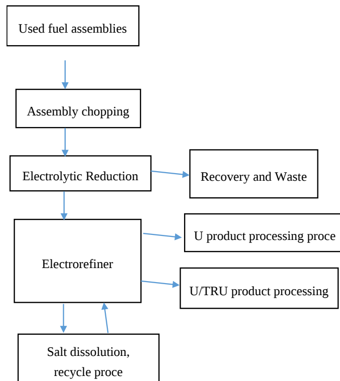
Figure 1. Generic electrochemical reprocessing facility with key activities shown.
