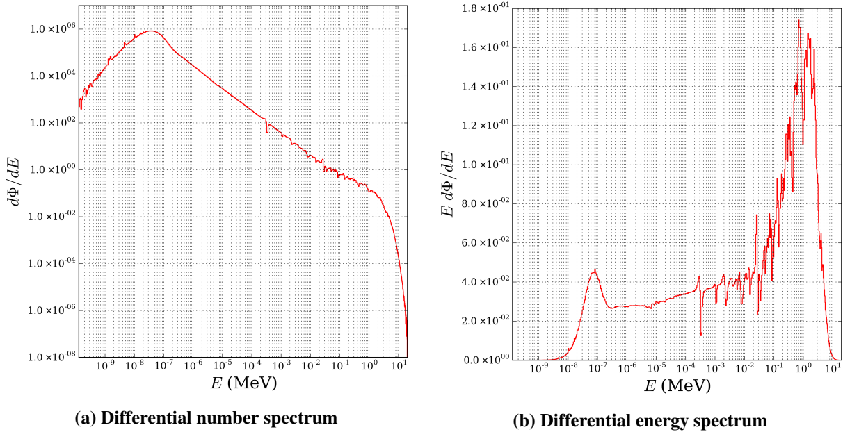
Figure 3. Calculated free-field spectrum in the ACRR central cavity.
