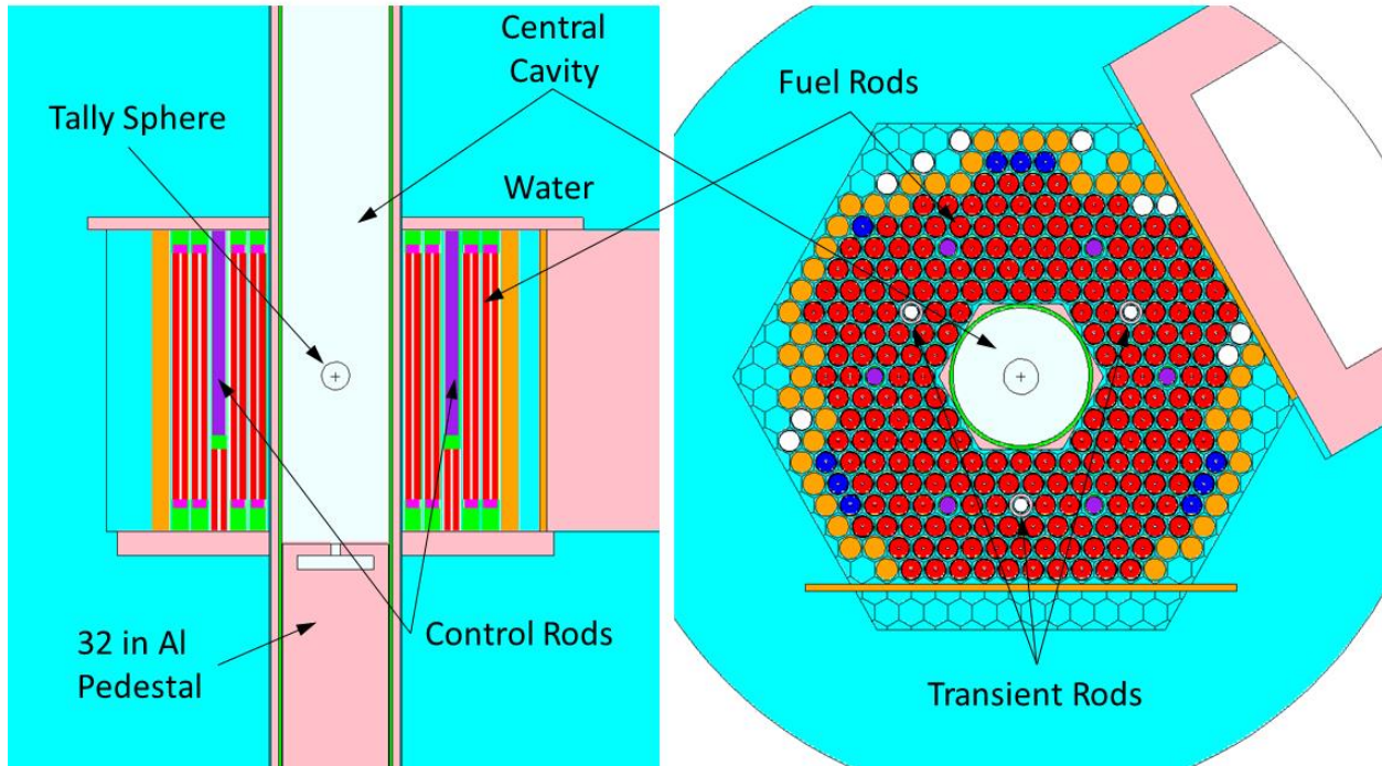
Figure 2. MCNP model of the ACRR and the central cavity with the 32-inch pedestal.
