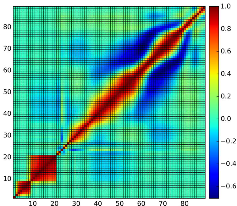
Figure 4. “A priori” energy dependent relative correlation matrix.
