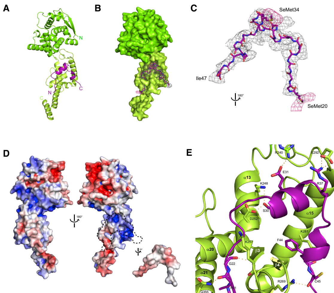
Figure 3. The Complex Structure of \Delta\text{NP}_{\text{NTD}} and NPBP Reveals Extensive Intermolecular Interactions
