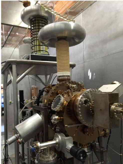
Figure 3: Back end of the gun showing the corona ring and the limiting resistor network.
