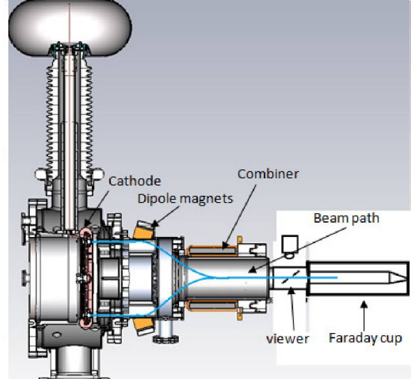
Figure 1: Schematic diagram of the gun.
