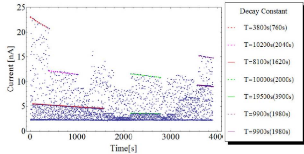
Figure 7: Two beam operation decay curve.
