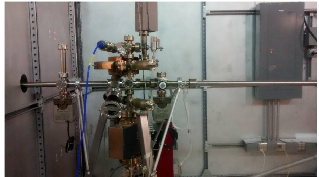
Figure 2: The transfer line, cathode preparation chamber and long manipulator, as shown from left to right.
