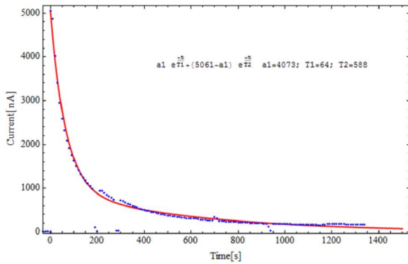
Figure 5: Single beam lifetime curve.
