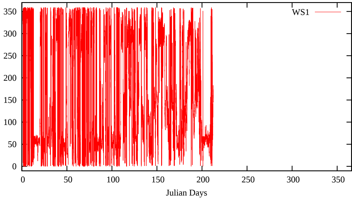
Station 000001 Eyak, AK 26.5m - Wind Directions - 2009
