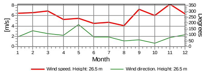
— Wind speed. Height: 26.5 m — Wind direction. Height: 26.5 m
