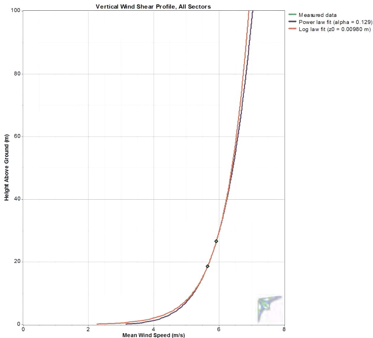
Figure 11B: Wind Shear – 19m and 26m
