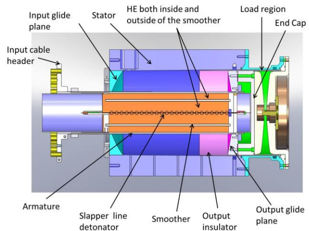
Figure 1. Baseline Ranchero configuration with 43 cm detonation system and an imploding liner load. For the minimum inductance load, the stator is connected to the output glide plane with a plate contoured to match the current joints shown here.
