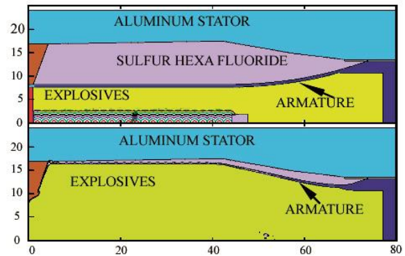
Figure 3. 2-D Hydrodynamic calculation of Ranchero S concept. There is no output glide plane in this design, and the armature is supported by full detonation pressure near the output. The first frame ( t=0 ) shows the initial contours and slapper initiation points, and the second frame ( t=34.5\mu\text{s} ) shows the contours as the armature approaches the stator. First armature motion is \sim 10\mu\text{s} . Inductance at first motion is \sim 86 nH, and at frame two is \sim 9 nH.
