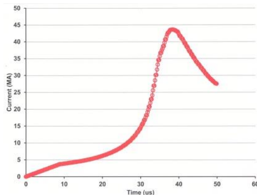
Figure 9. Current computed for 5 mm thick liner experiment. Seed current is provided by a 9.3 \mu\text{s} ramp to 3.75 MA in this calculation.
