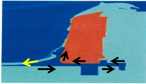
Figure 2. Result from an MHD simulation of the Ranchero experiment which had a peak current of 76 MA. The red is the output glide plane, the light blue regions are FCG conductors, the upper dark blue region is the detonation by-products, and the lower dark blue area has \text{SF}_6 in the collapsing void and load. Current flows along the surfaces enclosing the collapsing void and load as shown by the arrows. The curved conductor at the glide plane is the armature, and the aneurism is seen where the armature adjoins the glide plane. This aneurism adds parasitic inductance to the system, and the very thin armature section adds resistance and will ultimately fuse.
