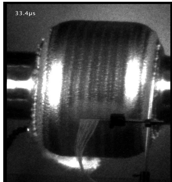
Figure 6. Framing camera record of armature expansion driven by 19.4 cm long 9501 initiated on 18 mm centers at the midplane of the HE cylinder. The 167 mm diameter, 6 mm thick annealed Al armature has expanded by a factor of two in this frame, and it is in good condition for flux compression.
