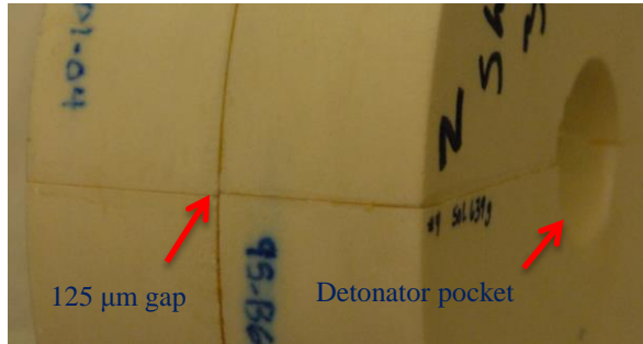
Figure 7. Armature charge with two 30 mm long 9501 half-cylinders glued together to create cylinders, and two of these glued together to make a 60 mm long cylinder. The detonator pockets were bored to different depths so that the middle of the 18 mm detonator spacing was offset by 3 mm from the glue joint. All glue joints were \sim 50 \mu\text{m} thick, but a machining error left an extra gap of 125 \mu\text{m} at this compound joint, and it is seen to rupture in the dynamic record.
