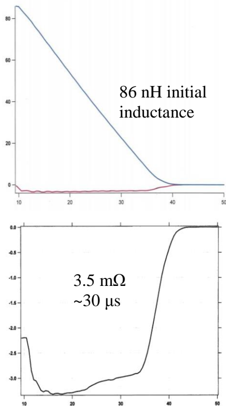
Figure 4. L and dL/dt for the FCG in fig. 3. Operation time is from about 10 μs to ~40 μs.
