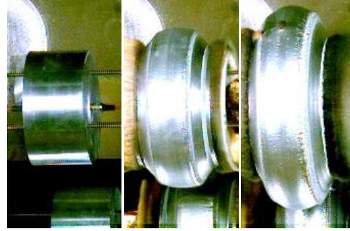
Figure 8. One static and two dynamic images of an expanding 6 mm thick 167 mm diameter Al armature driven by the charge in Fig. 6. The armature is initially 94 mm long, and there are polycarbonate spacers 17 mm long to hold the HE in place and locate the detonators. Evidence of all glue joints is seen in the middle frame, but the only rupture is in the upper compound joint where a machining flaw created a 125 \mu\text{m} flaw. The compound joint with no flaw, seen in the mirror view, is occluded in the last frame, and no data was obtained at this degree of expansion.
