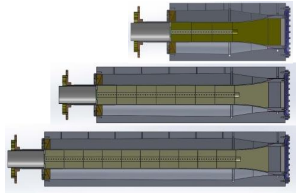
Figure 5. Family of Ranchero S generators using 43 cm, 100 cm, or 144 cm detonation systems. Initial inductances are approximately 86 nH, 170 nH, and 225 nH respectively.
