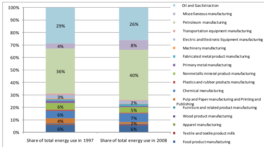
Figure 30: Manufacturing Subsector Shares of Total Final California Industry Energy Use, 1997 and 2008
