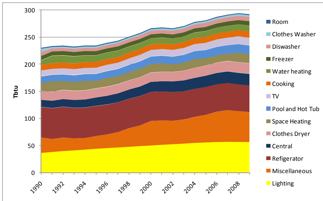
Figure 56: Final Energy Use for Residential Natural Gas End Uses (TBtu)
