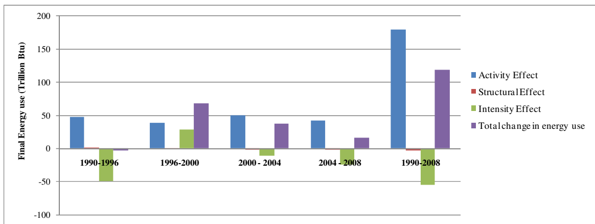
Figure 49: Decomposition Analysis Using Floor Space Activity Variable
