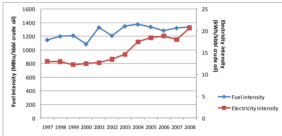
Figure 40: Total Final Energy Intensity of the California Oil and Gas Extraction Sector
