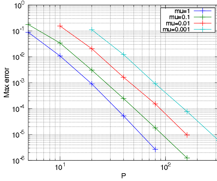
Figure 4: Max error in the numerical evolution of the Rayleigh surface wave after one period, as function of the number of grid points per wave length, P_r . The different curves correspond to \mu = 1 (blue), \mu = 0.1 (green), \mu = 0.01 (red), and \mu = 0.001 (cyan).
