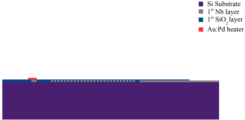
Figure 4.3: Au:Pd layer for the persistent current switch heater.
