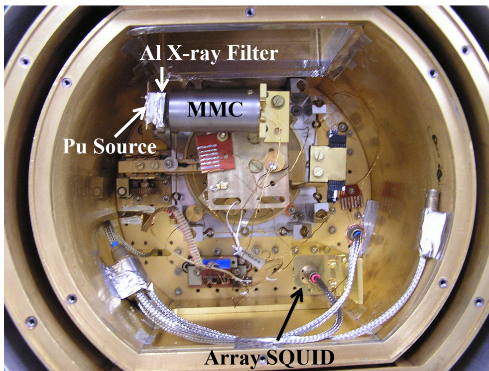
Figure 7.24: MMC installed in cryostat at LLNL for measurements of the mixed isotope plutonium source with Al X-ray filter.
