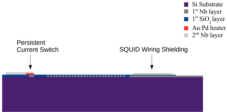
Figure 4.4: Nb layer for heater connections and SQUID wiring shielding.
