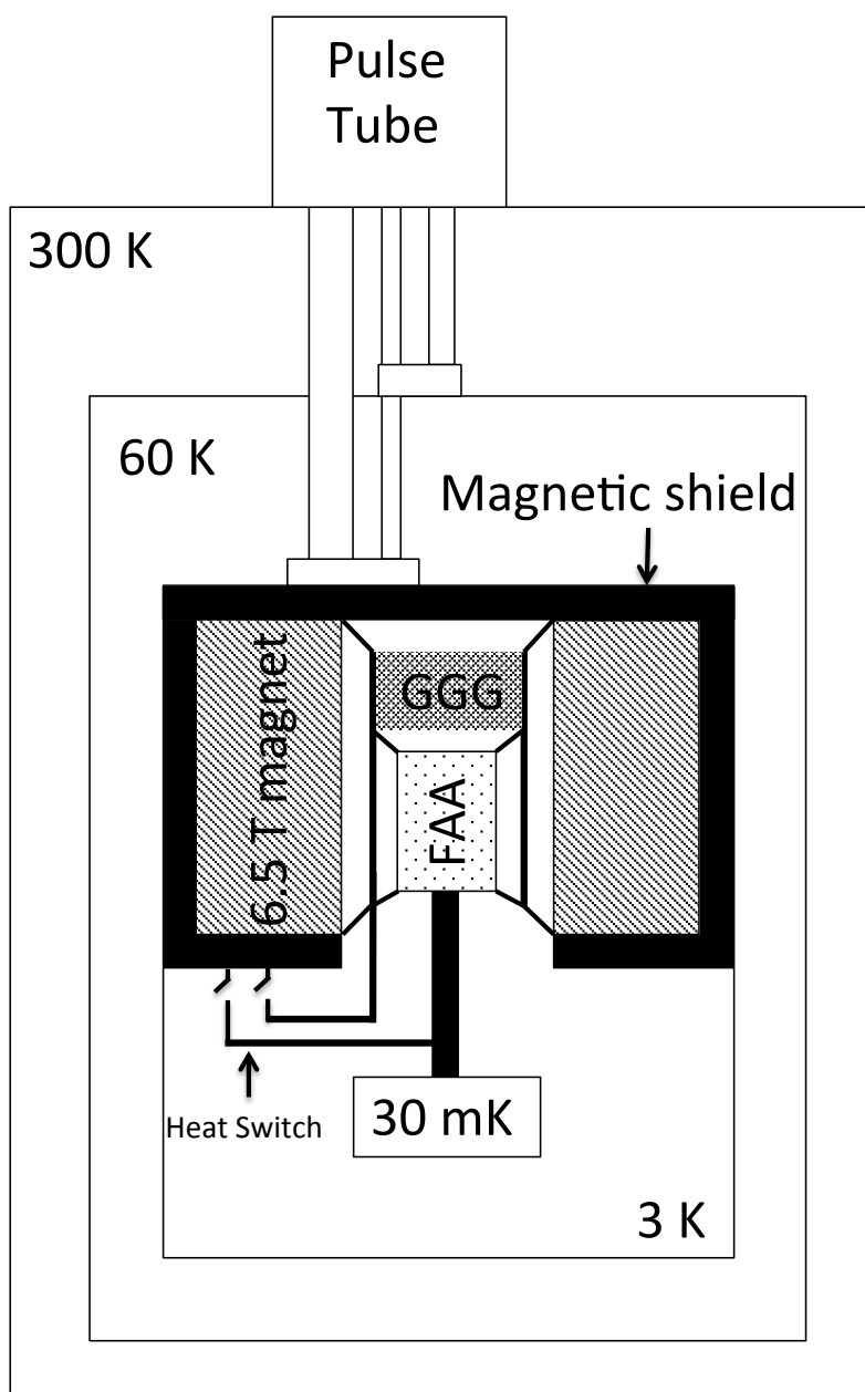
Figure 5.1: Conceptual drawing of a pulse-tube cooled two-stage ADR.
