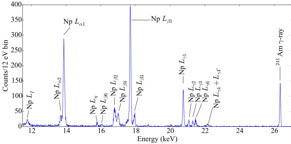
Figure 7.7: MMC X-ray spectrum from ^{241}Am taken at the University of Heidelberg.
