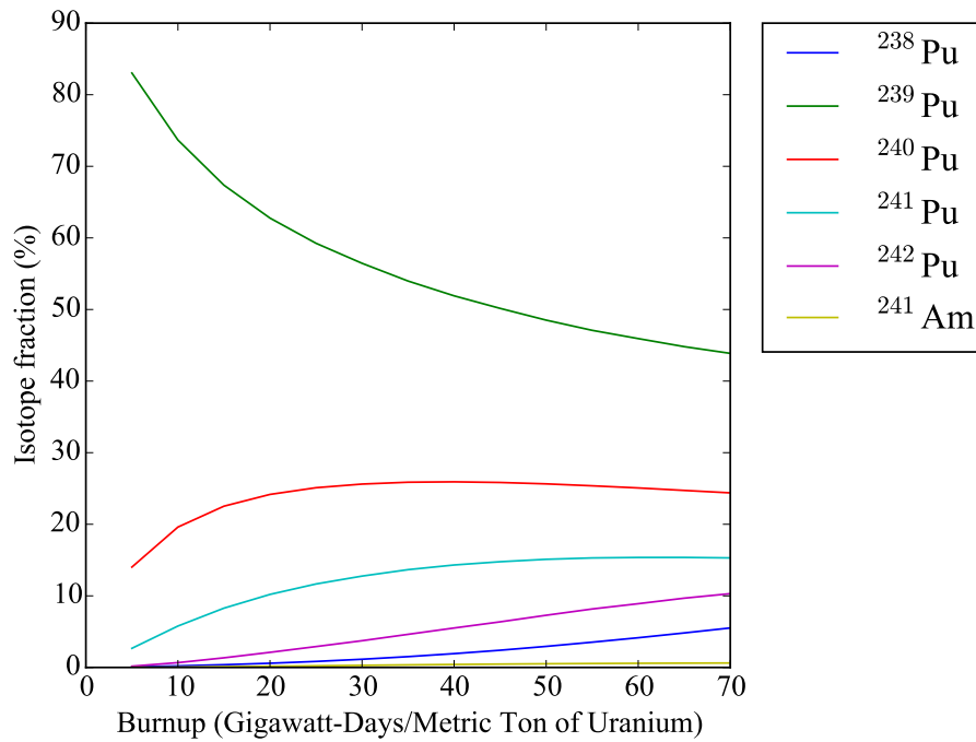
Figure 2.2: A plot of Pu concentration as a function of burn-up in a PWR calculated using CAIN [27].
