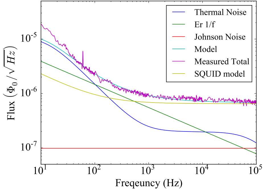
Figure 7.14: Comparison of model noise with measured noise spectrum.
