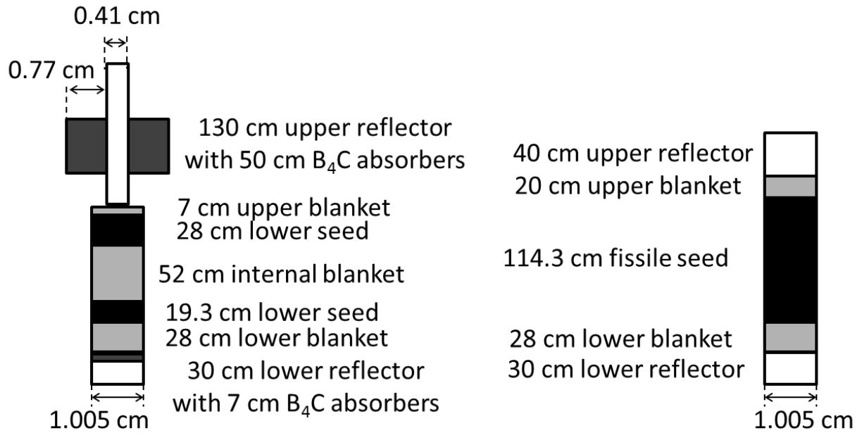
Figure 16 Layout of the RBWR-Th using Hitachi T/H correlations versus RBWR-AC fuel rod design
