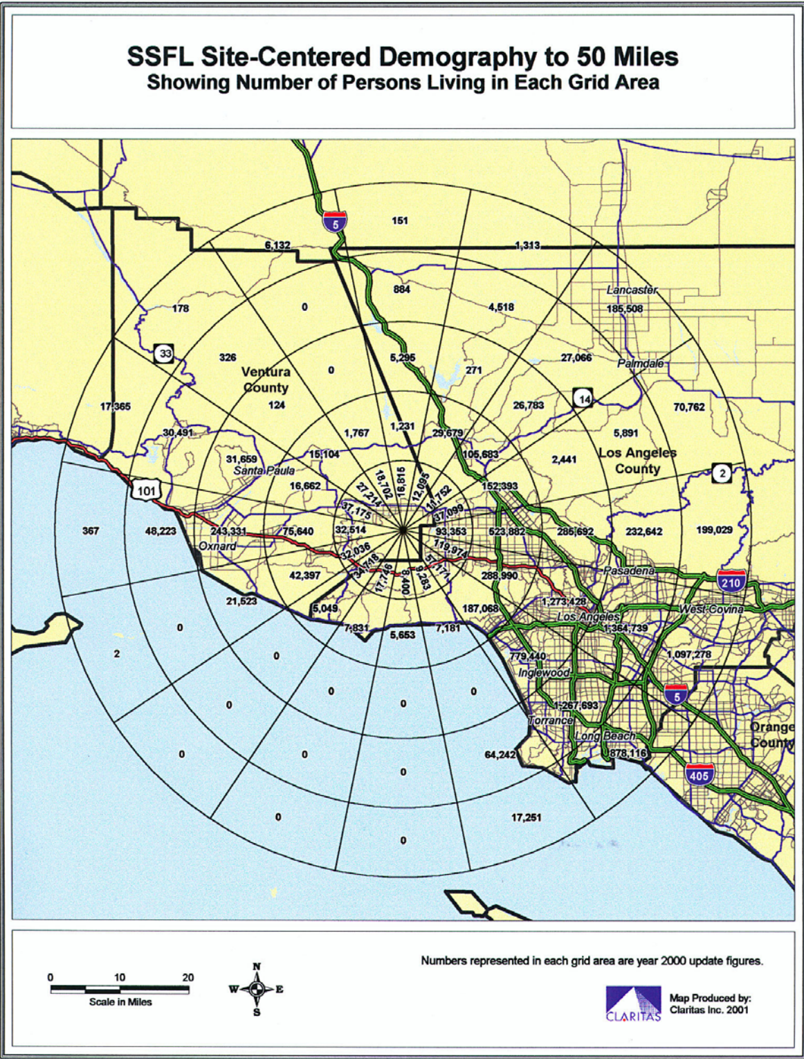
Figure 5-3. Demographic Data Within 50 miles (80 km) of SSFL
