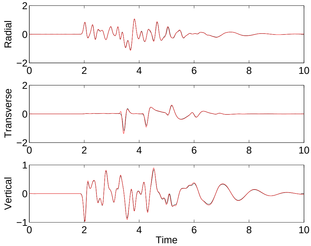
Figure 6: Solution of the LOH.3 test problem at reciever # 10. The black line is the semi-analytical solution, and the red line shows the numerical solutions with n = 3 mechanisms.
