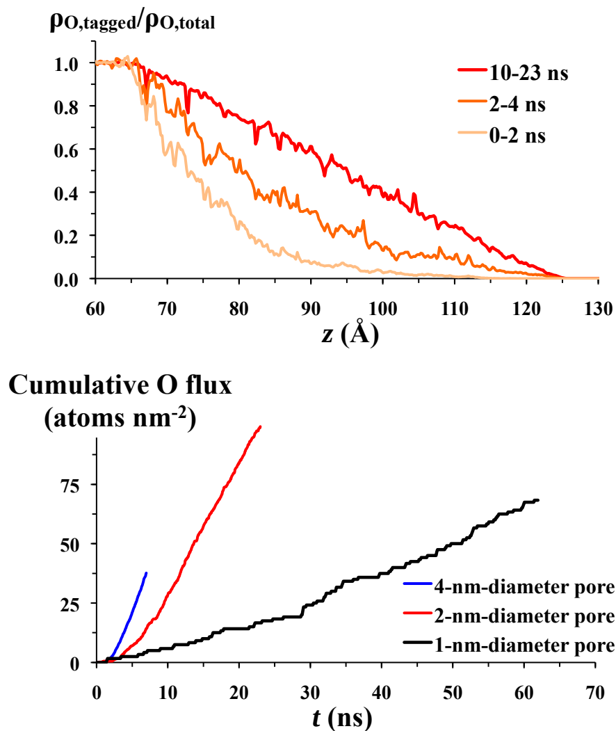
Figure 5. Upper graph: average density distribution of “tagged” water O atoms (normalized to the average density of water O atoms, averaged over both z directions, and plotted as a function of z) during several time intervals after the beginning of the 2 nm diameter nanopore simulation. Lower graph: cumulative breakthrough flux of tagged water O atoms diffusing through 1, 2, and 4 nm diameter nanopores (averaged over both directions, normalized to pore cross-section area) plotted as a function of time since the beginning of the MD simulation.
