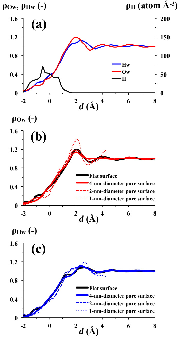
Figure 3. (a) Average density of silanol H (in black), Ow (in red), and Hw atoms (in blue) as a function of distance from the curved surface of the 2 nm diameter pore, calculated for z = 75 to 115 Å. (b) Comparison of the average Ow density ( \rho_{Ow} ) profiles on flat surfaces (calculated for r = 23.0 to 31.2 Å in the 4 nm diameter pore simulations) and on curved nanopore surfaces ( z = 75 to 115 Å). (c) Same as Fig. 3b for \rho_{Hw} .
