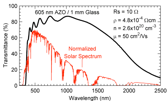
Fig. 1. Transmittance of an AZO film on glass.
