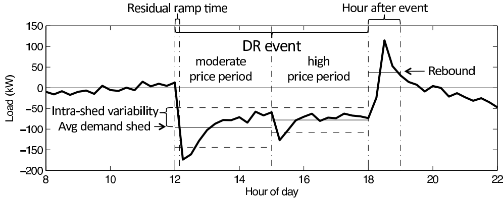
Figure 2.15: Several DR parameters shown on the furniture store’s DR residual (from Figure 2.14). ©2011 IEEE
