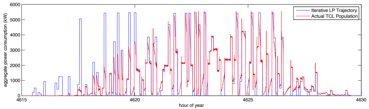
Figure 5.6: TCL population tracking performance: 1,000 air conditioners.
