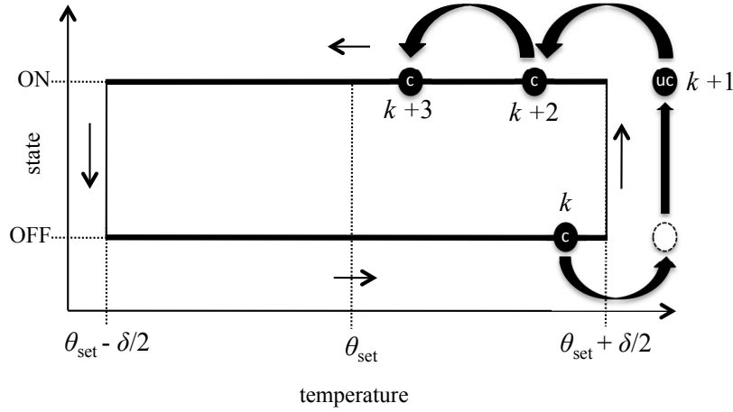
Figure 5.1: A cooling TCLs temperature dead-band and motion in discrete time.
