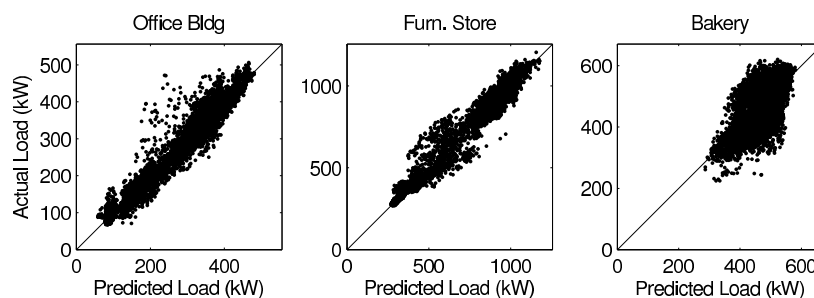
Figure 2.11: Actual versus predicted load scatter plots. Data shown are from May-Sept 2008. Significant outliers visible in the plot for the office building result from the model's inability to accurately predict the morning start-up. ©2011 IEEE
