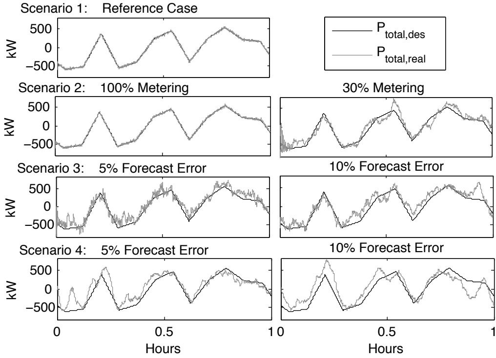
Figure 4.7: Tracking performance for Scenarios 1–3 ( N_{\text{bin}}=40 , Controller 1) and Scenario 4 ( N_{\text{bin}}=2 ) with N_{\text{TCL}}=1,000 .
